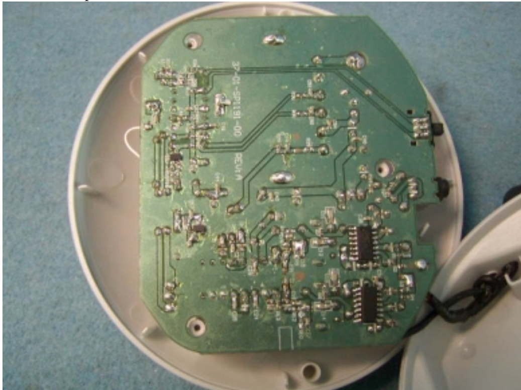
SP1291 internal photo
