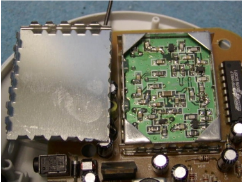
solder side
