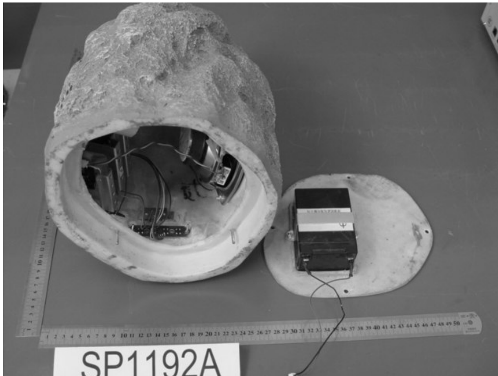
SP1192A internal photo
