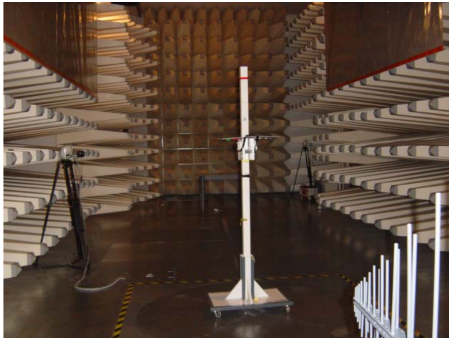
Set-up for Radiation Emission
