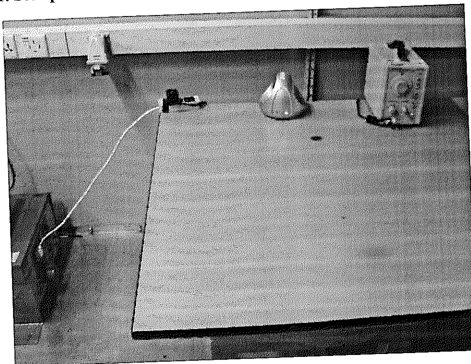
Photograph 1: Set-up for Conducted Emission on AC Mains
