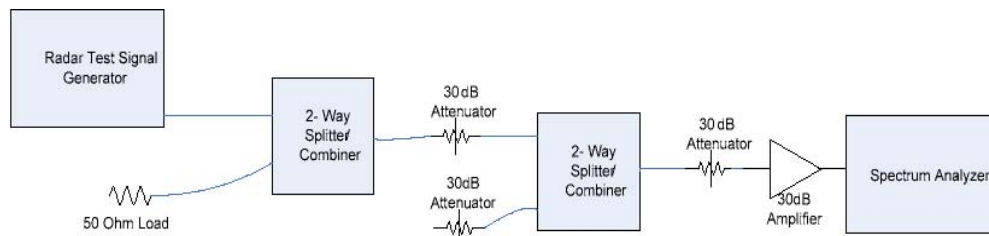
Conducted Calibration Setup
