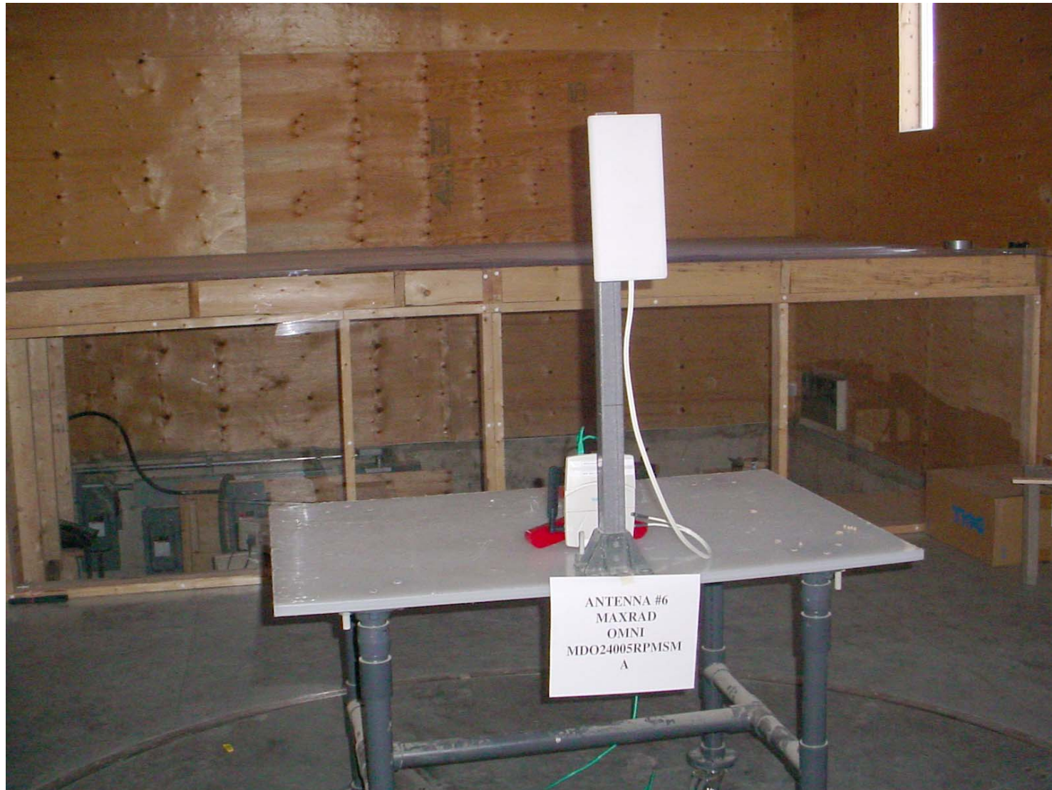
Photo #6a: HiPath Wireless Access Point with Maxrad Omni, 2 Inputs External Antenna Model: MDO24005PTRPMSMA, 5.2 dBi gain
