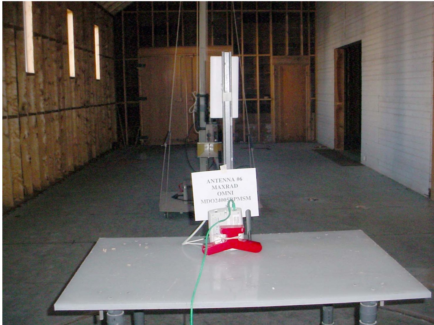
Photo #6b: HiPath Wireless Access Point with Maxrad Omni, 2 Inputs External Antenna Model: MDO24005PTRPMSMA, 5.2 dBi gain
