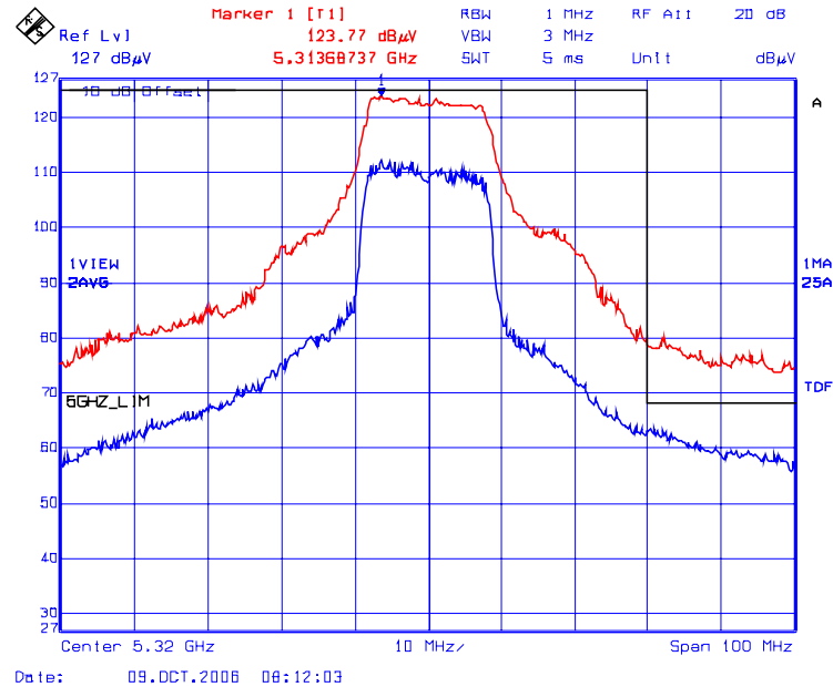
Plot 6.2.5.1.3.4 Upper Band-Edge Transmitter Radiated Emissions @ 3 Meters, Vertical Polarization Frequency: 5320 MHz; Power Setting: 18.0dBm
