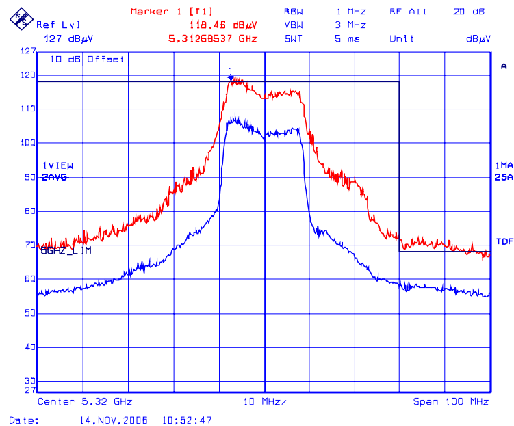
Plot 6.2.5.1.4.4 Upper Band-Edge Transmitter Radiated Emissions @ 3 Meters, Vertical Polarization Frequency: 5320 MHz; Power Setting: 18.0dBm
