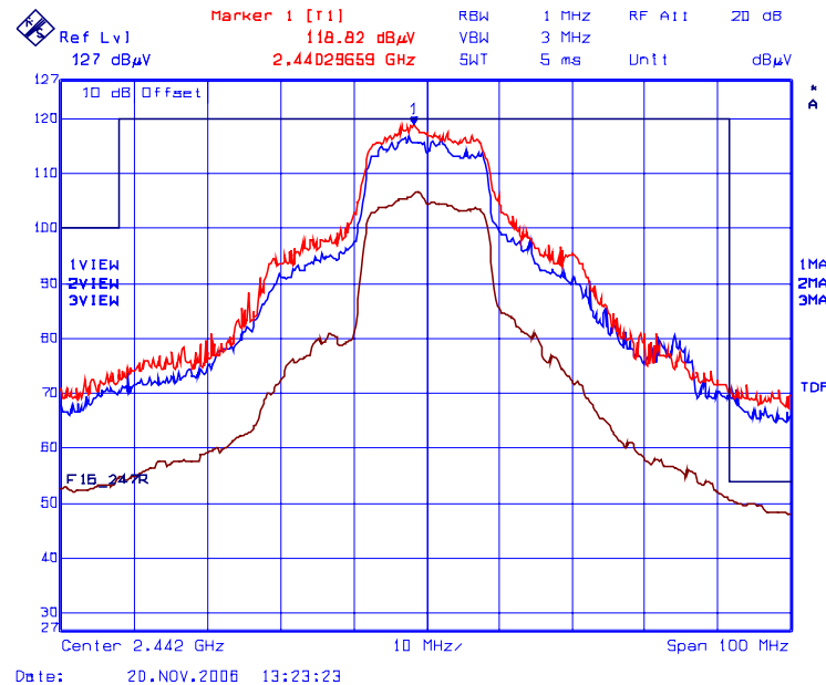
Plot 5.2.4.1.12.14 Upper Band-Edge Transmitter Radiated Emissions @ 3 Meters, Vertical Polarization Frequency: 2442 MHz, Power Setting: 20.0dBm
