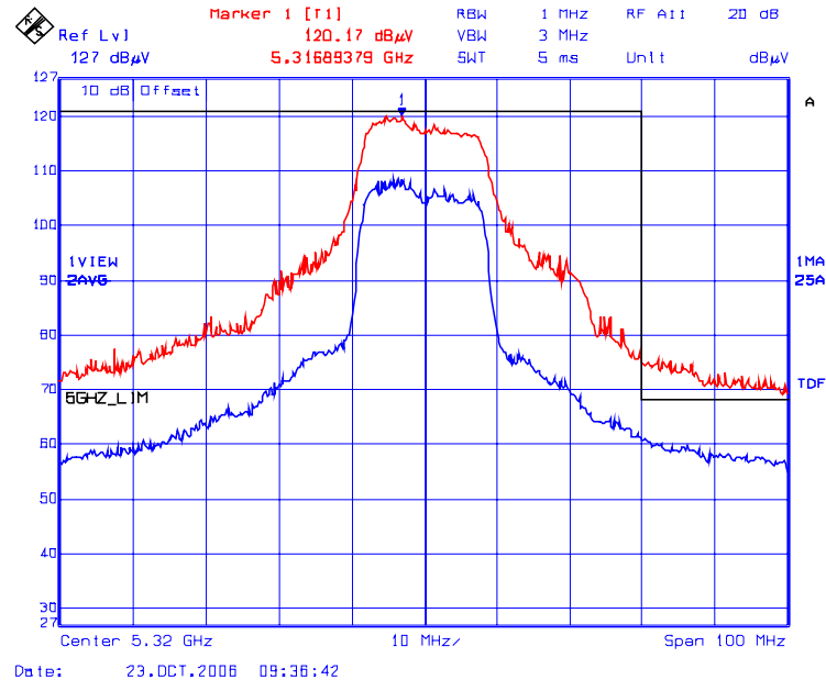
Plot 6.2.5.1.1.4 Upper Band-Edge Transmitter Radiated Emissions @ 3 Meters, Vertical Polarization Frequency: 5320 MHz; Power Setting: 18.0dBm
