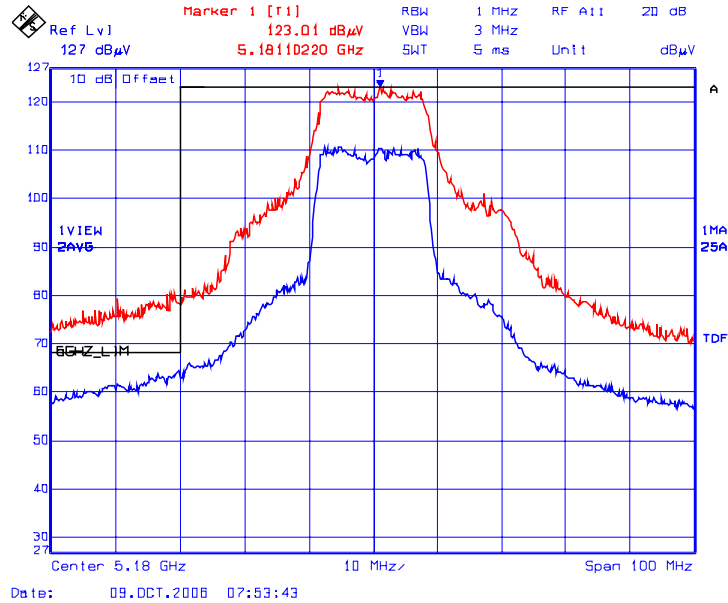
Plot 6.2.5.1.3.2 Lower Band-Edge Transmitter Radiated Emissions @ 3 Meters, Vertical Polarization
