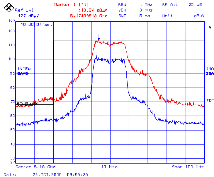
Plot 6.2.5.1.1.2 Lower Band-Edge Transmitter Radiated Emissions @ 3 Meters, Vertical Polarization
