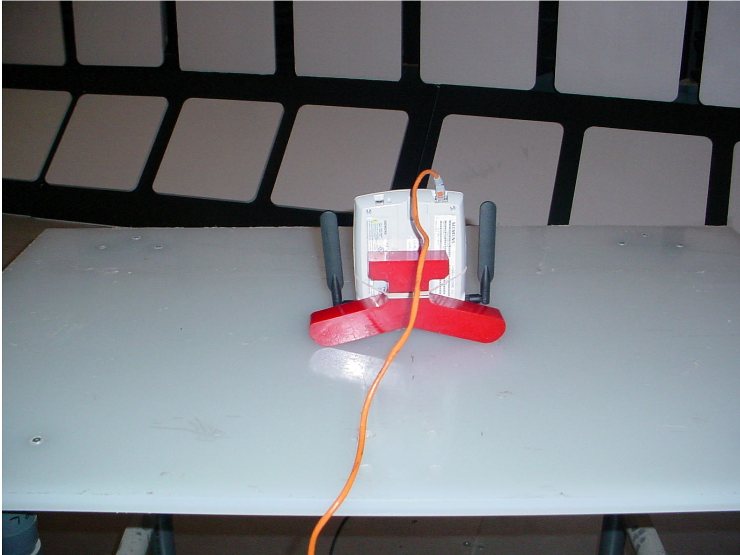
Photo #5: HiPath Wireless Access Point with external antennas – Test Orthogonal Position #2
