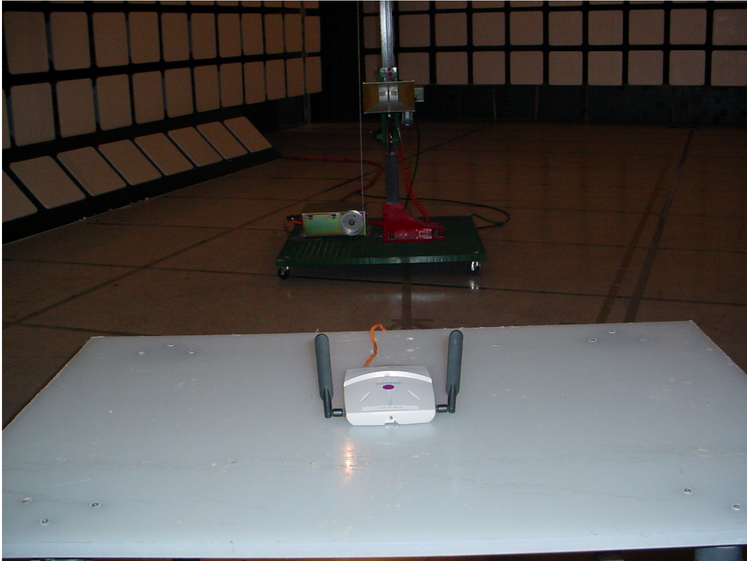
Photo #6: HiPath Wireless Access Point with external antennas – Test Orthogonal Position #3
