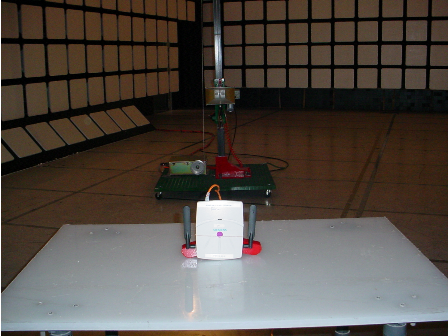
Photo #4: HiPath Wireless Access Point with external antennas – Test Orthogonal Position #1
