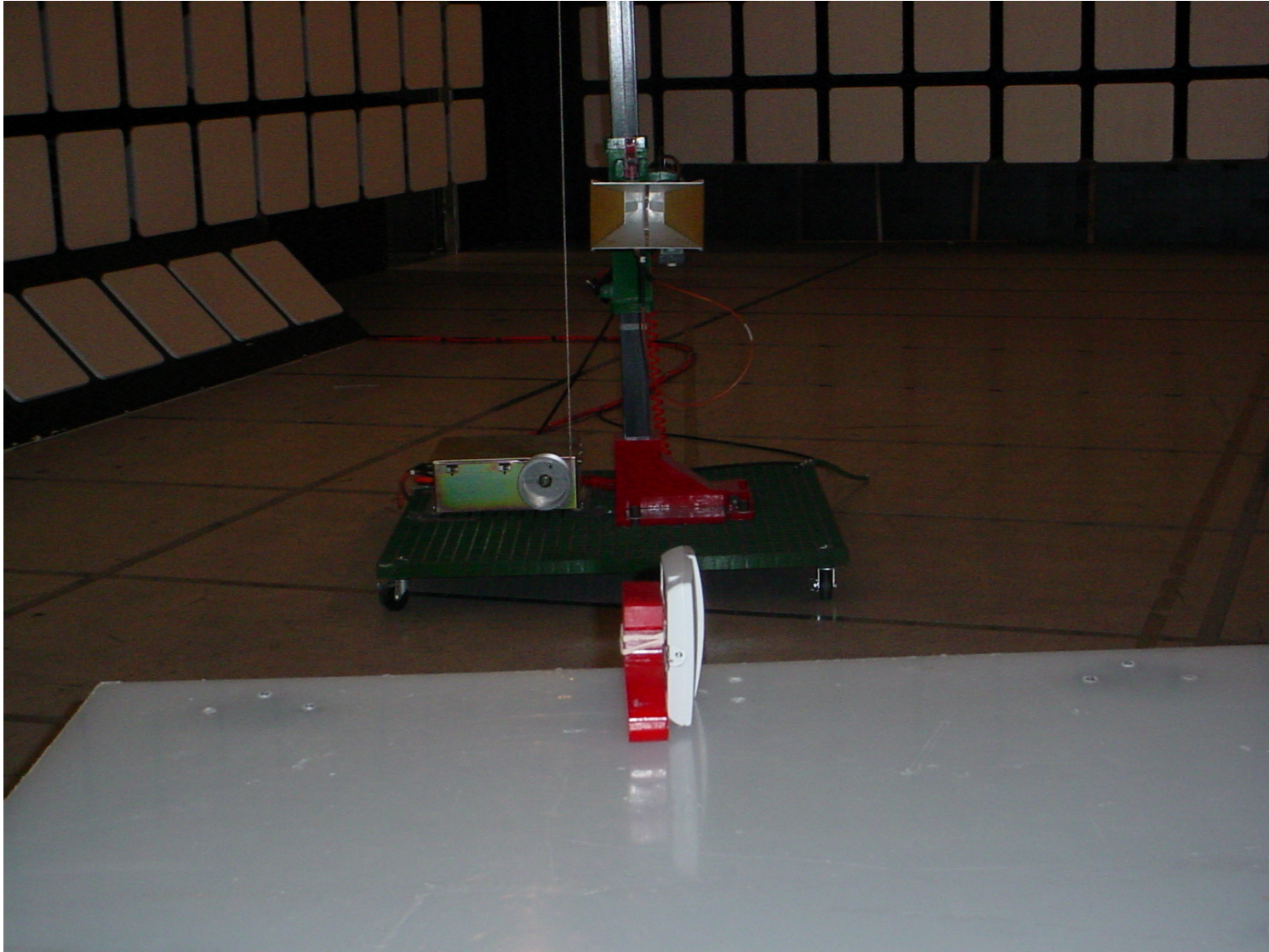
Photo #3: HiPath Wireless Access Point with internal antennas – Test Orthogonal Position #3
