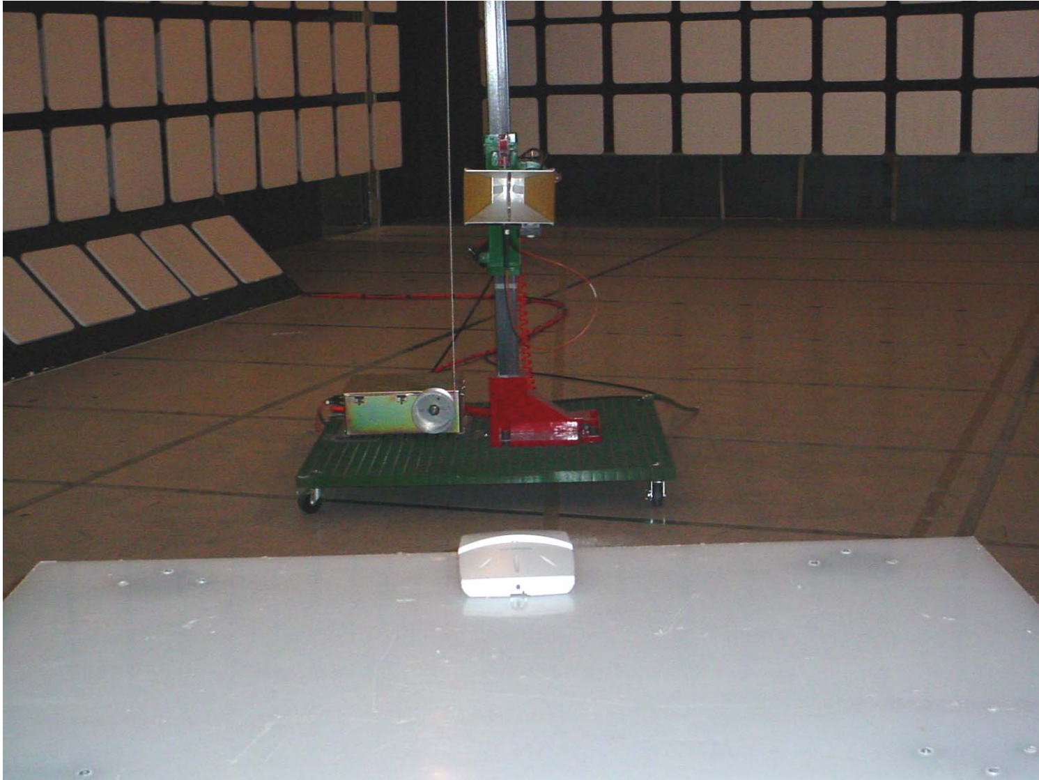
Photo #1: HiPath Wireless Access Point with internal antennas – Test Orthogonal Position #1
