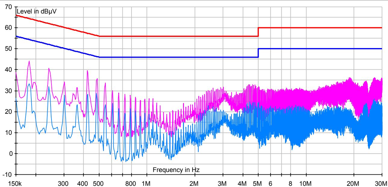
Worst case measurement result of 802.11n HT20 modulation
