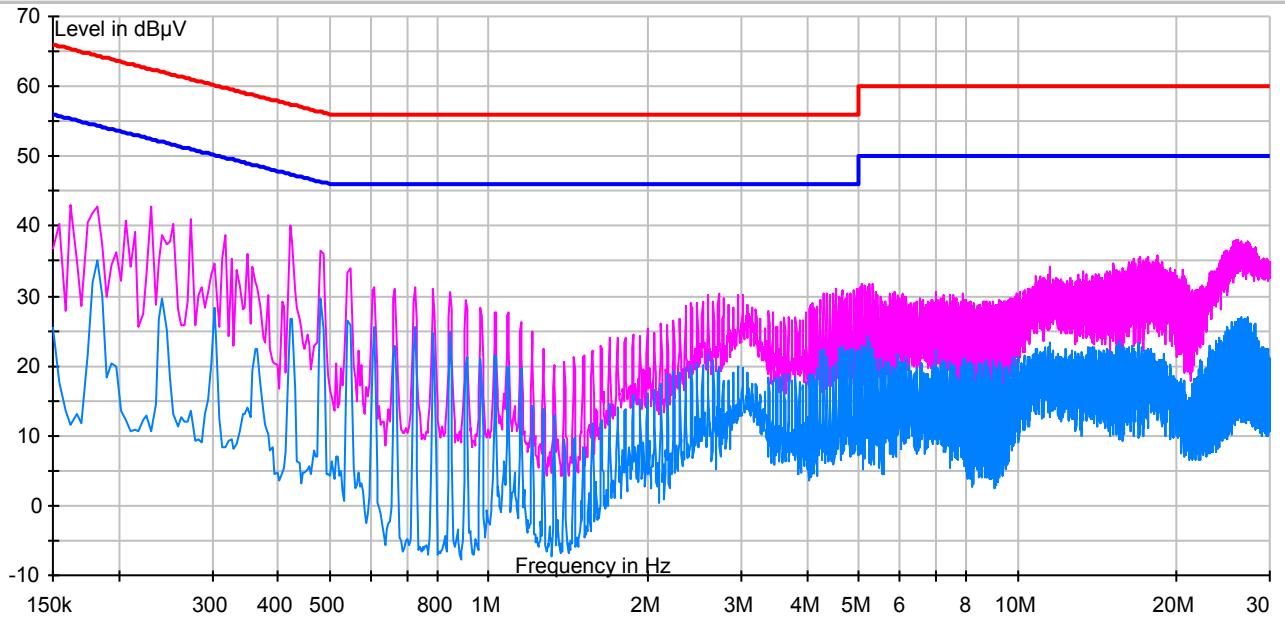
Worst case measurement result of 802.11b modulation
