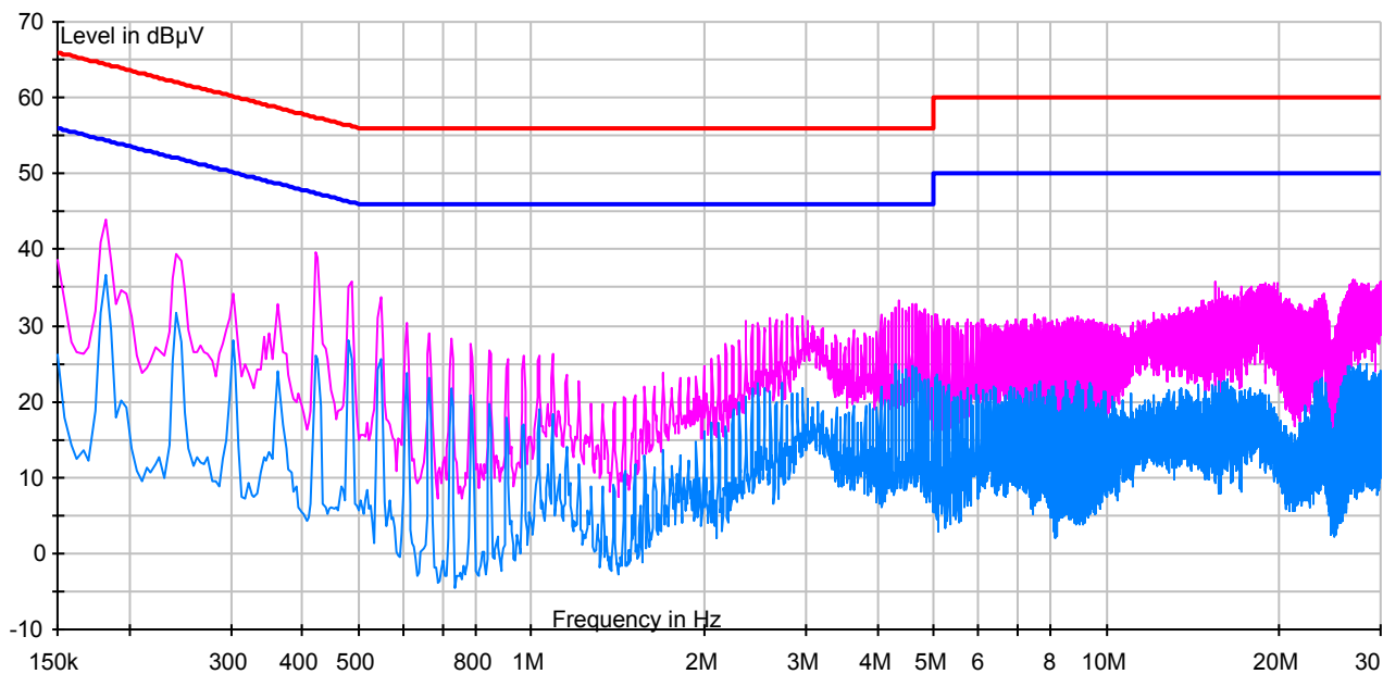
Worst case measurement result of 802.11n HT40 modulation
