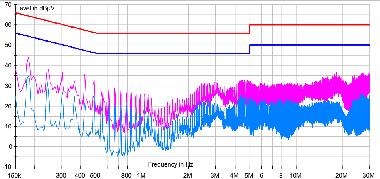
Worst case measurement result of 802.11g modulation
