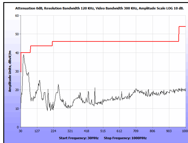
Plot 248. Co-location, Radiated Spurious Emissions, PIFA, 802.11n 20 MHz, 2412 & 5785 MHz, 30 MHz – 1 GHz
