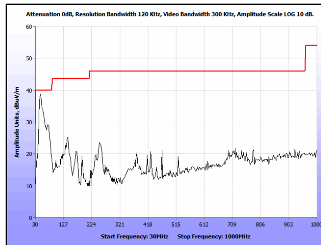
Plot 272. Co-location, Radiated Spurious Emissions, PIFA, 802.11n 20 MHz, 2462 & 5300 MHz, 30 MHz – 1 GHz
