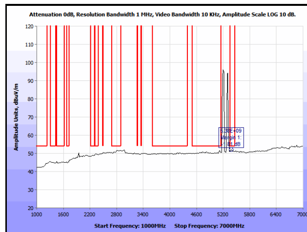
Plot 289. Co-location, Radiated Spurious Emissions, PIFA, 802.11n 20 MHz, 5200 & 5300 MHz, 1 GHz – 7 GHz, Average
