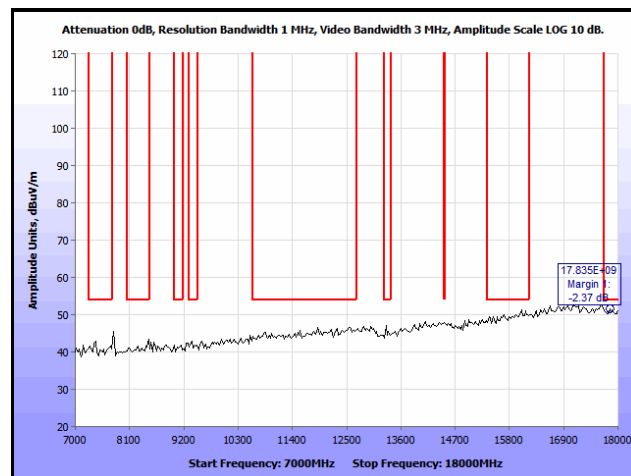
Plot 259. Co-location, Radiated Spurious Emissions, PIFA, 802.11n 20 MHz, 2437 & 5300 MHz, 7 GHz – 18 GHz, Peak
