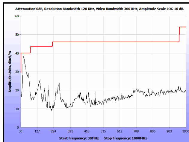
Plot 232. Co-location, Radiated Spurious Emissions, PIFA, 802.11n 20 MHz, 2437 & 2462 MHz, 30 MHz – 1 GHz
