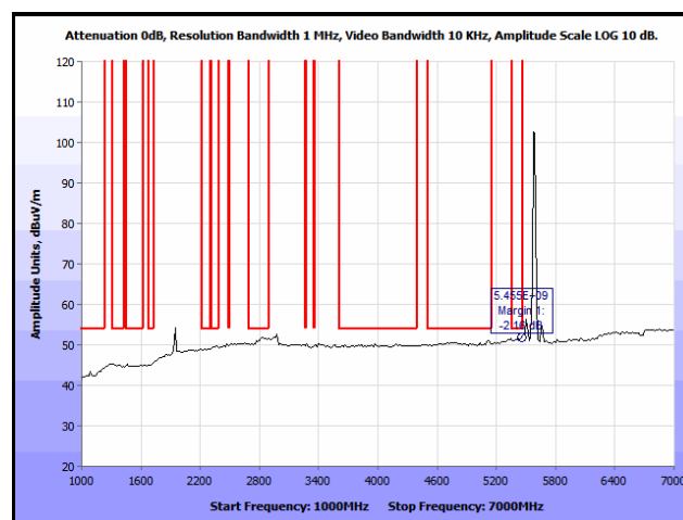
Plot 313. Co-location, Radiated Spurious Emissions, PIFA, 802.11n 20 MHz, 5580 & 5580 MHz, 1 GHz – 7 GHz, Average
