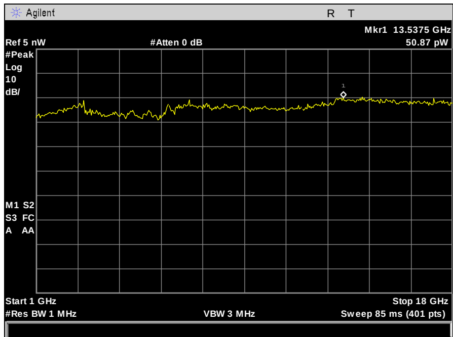
Plot 517. Receiver Spurious Emission, 1 GHz – 18 GHz, Port 1
