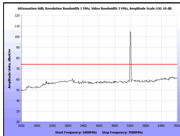
Plot 286. Co-location, Radiated Spurious Emissions, PIFA, 802.11n 20 MHz, 5200 & 5200 MHz, 1 GHz – 7 GHz, Peak
