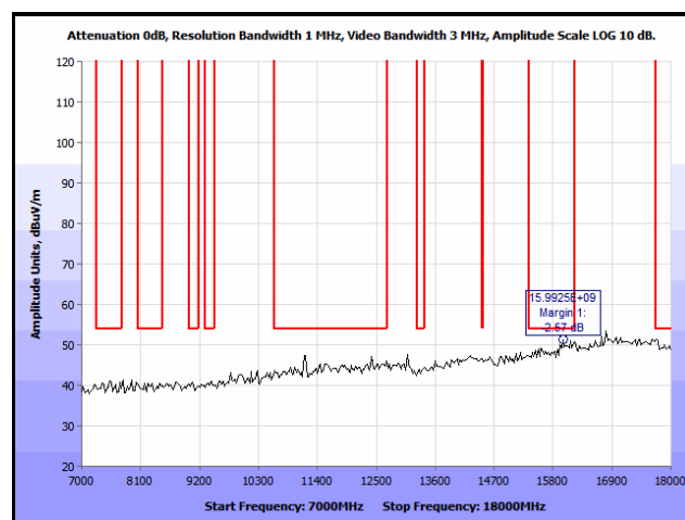
Plot 319. Co-location, Radiated Spurious Emissions, PIFA, 802.11n 20 MHz, 5580 & 5785 MHz, 7 GHz – 18 GHz, Peak
