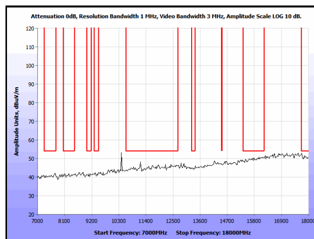
Plot 295. Co-location, Radiated Spurious Emissions, PIFA, 802.11n 20 MHz, 5200 & 5580 MHz, 7 GHz – 18 GHz, Peak
