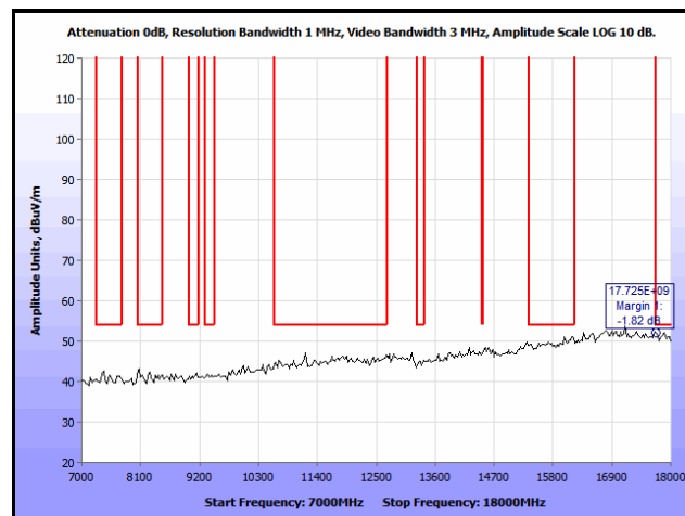
Plot 247. Co-location, Radiated Spurious Emissions, PIFA, 802.11n 20 MHz, 2412 & 5580 MHz, 7 GHz – 18 GHz, Peak
