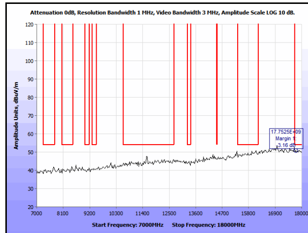
Plot 323. Co-location, Radiated Spurious Emissions, PIFA, 802.11n 20 MHz, 5785 & 5785 MHz, 7 GHz – 18 GHz, Peak
