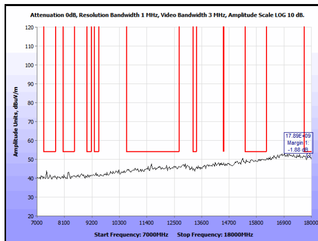
Plot 283. Co-location, Radiated Spurious Emissions, PIFA, 802.11n 20 MHz, 2462 & 5785 MHz, 7 GHz – 18 GHz, Peak
