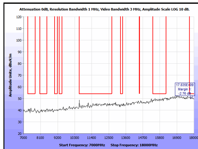
Plot 307. Co-location, Radiated Spurious Emissions, PIFA, 802.11n 20 MHz, 5300 & 5580 MHz, 7 GHz – 18 GHz, Peak
