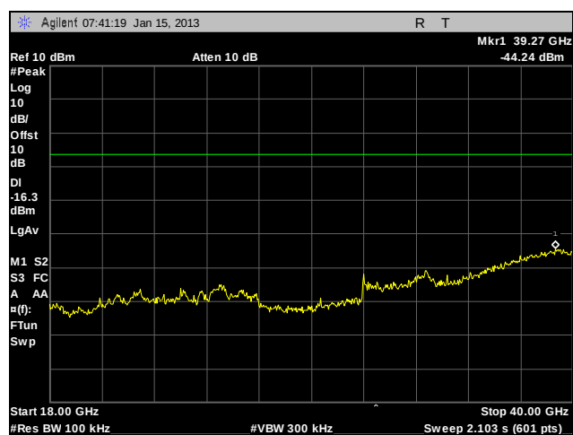
Plot 419. Conducted Spurious Emissions, 802.11n 40 MHz, 5795 MHz, High Channel, Port 2, 18 GHz - 40 GHz
