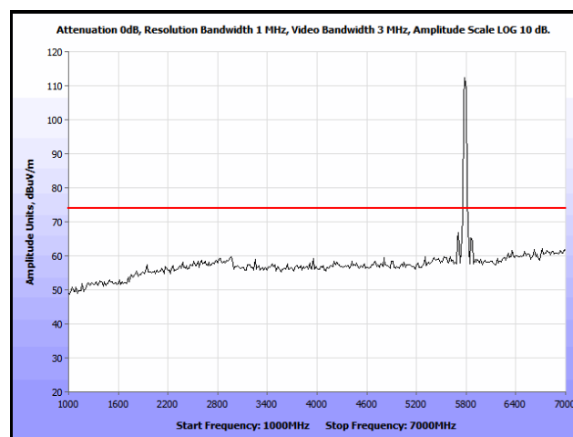
Plot 322. Co-location, Radiated Spurious Emissions, PIFA, 802.11n 20 MHz, 5785 & 5785 MHz, 1 GHz – 7 GHz, Peak
