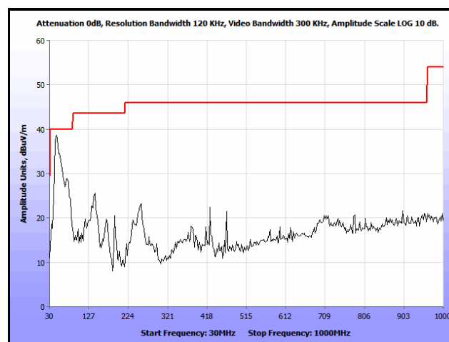
Plot 280. Co-location, Radiated Spurious Emissions, PIFA, 802.11n 20 MHz, 2462 & 5785 MHz, 30 MHz – 1 GHz
