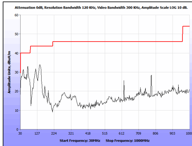
Plot 127. Radiated Spurious Emissions, 802.11n 80 MHz, 30 MHz – 1 GHz, 7 dBi Patch
