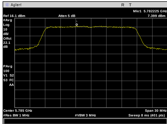
Plot 66. Power Spectral Density, Mid Channel, 802.11n 20 MHz, Port 3
