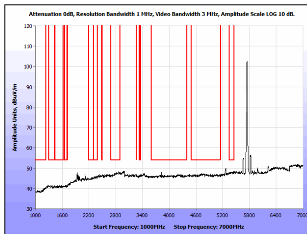
Plot 132. Radiated Spurious Emissions, 802.11a, Low Channel, 1 GHz – 7 GHz, Average, Ceiling
