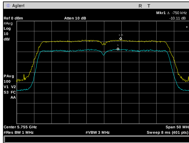
Plot 89. Peak Excursion Ratio, Low Channel, 802.11n 40 MHz, Port 1
