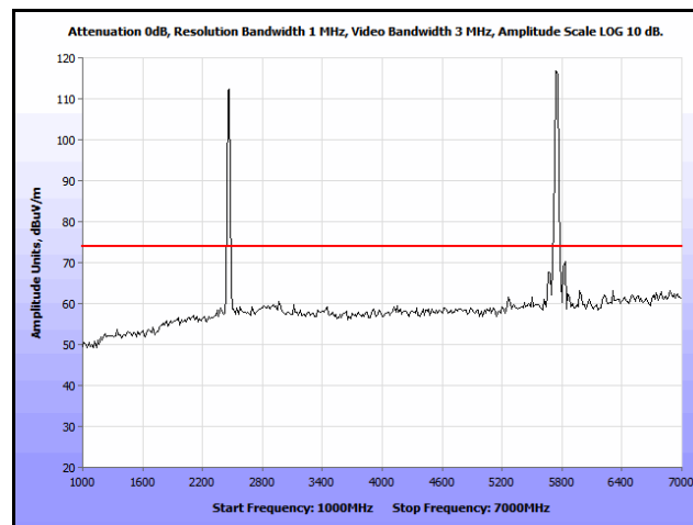
Plot 265. Co-location, Radiated Spurious Emissions, Patch, 802.11n 20 MHz, 2462 & 5785 MHz, 1 GHz – 7 GHz, Peak
