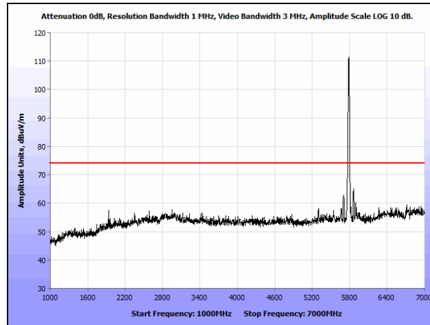
Plot 173. Radiated Spurious Emissions, 802.11a, Mid Channel, 1 GHz – 7 GHz, Peak, Omni
