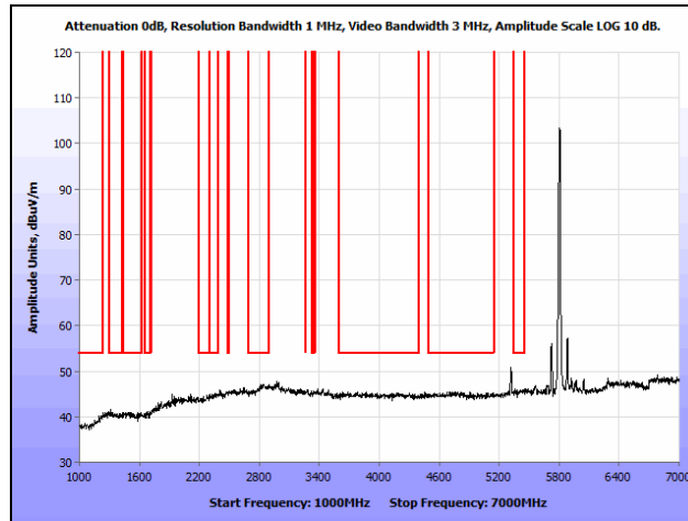
Plot 176. Radiated Spurious Emissions, 802.11a, High Channel, 1 GHz – 7 GHz, Average, Omni
