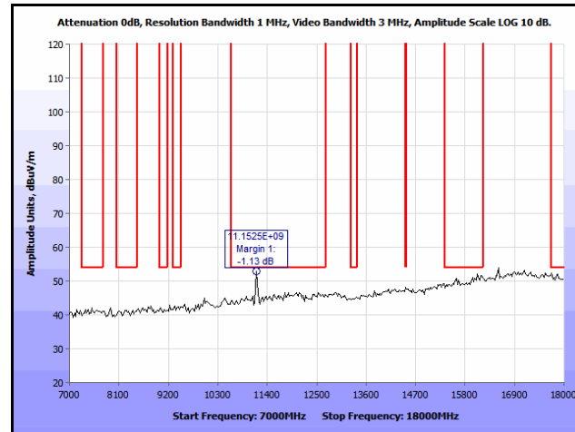
Plot 242. Co-location, Radiated Spurious Emissions, Omni, 802.11n 20 MHz, 5200 & 5785 MHz, 7 GHz – 18 GHz, Peak
