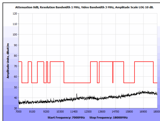
Plot 190. Radiated Spurious Emissions, 802.11n 20 MHz, High Channel, 7 GHz – 18 GHz, Omni
