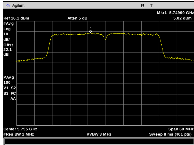
Plot 72. Power Spectral Density, Low Channel, 802.11n 40 MHz, Port 3
