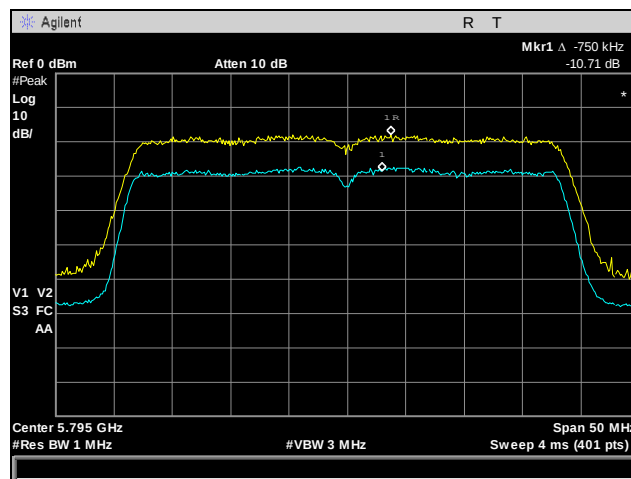
Plot 92. Peak Excursion Ratio, High Channel, 802.11n 40 MHz, Port 1
