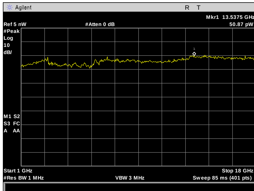
Plot 280. Receiver Spurious Emission, 1 GHz – 18 GHz, Port 1
