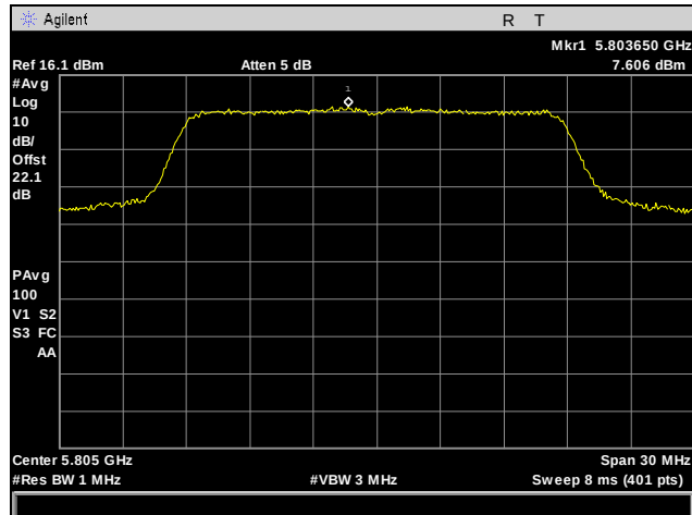
Plot 61. Power Spectral Density, High Channel, 802.11n 20 MHz, Port 1
