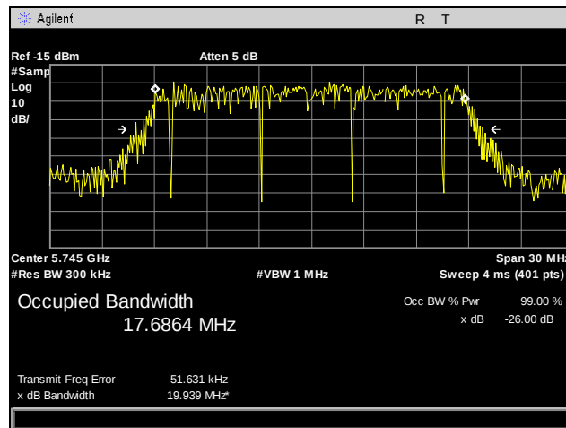
Plot 44. 99% Occupied Bandwidth, 802.11n 20 MHz, Port 3, Low Channel
