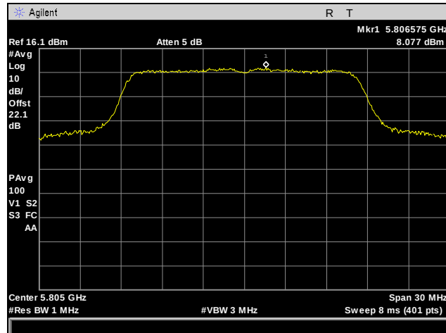
Plot 58. Power Spectral Density, High Channel, 802.11a
