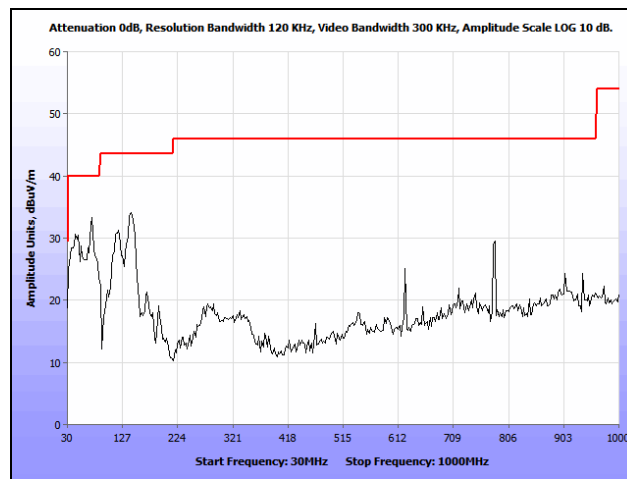
Plot 123. Radiated Spurious Emissions, 802.11n 40 MHz, High Channel, 30 MHz – 1 GHz, 7 dBi Patch
