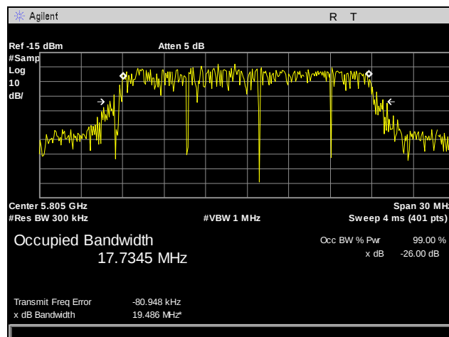
Plot 46. 99% Occupied Bandwidth, 802.11n 20 MHz, Port 3, High Channel
