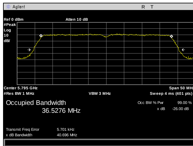
Plot 27. 26 dB Occupied Bandwidth, 802.11n 40 MHz, Port 1, High Channel
