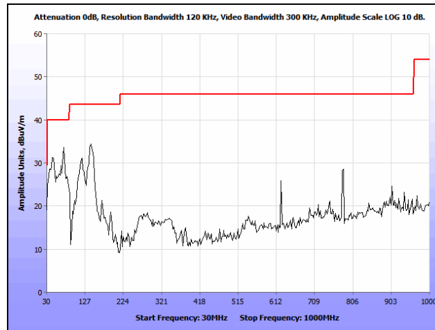
Plot 95. Radiated Spurious Emissions, 802.11a, Low Channel, 30 MHz – 1 GHz, 7 dBi Patch
