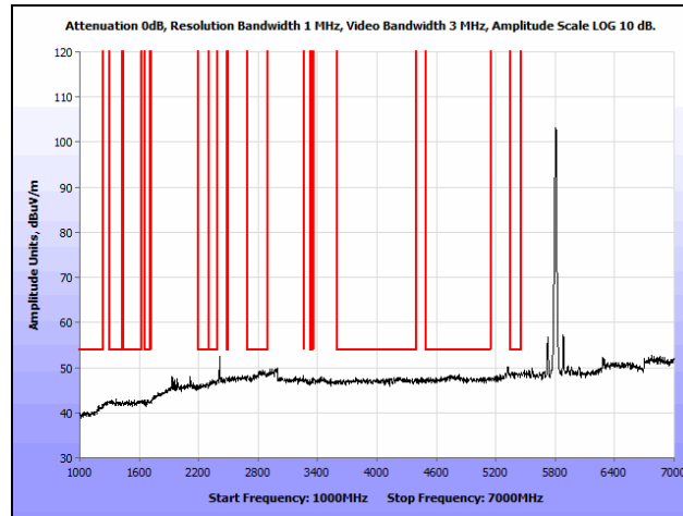
Plot 140. Radiated Spurious Emissions, 802.11a, High Channel, 1 GHz – 7 GHz, Average, Ceiling
