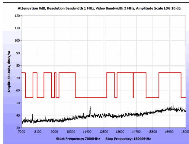
Plot 162. Radiated Spurious Emissions, 802.11n 40 MHz, High Channel, 7 GHz – 18 GHz, Ceiling
