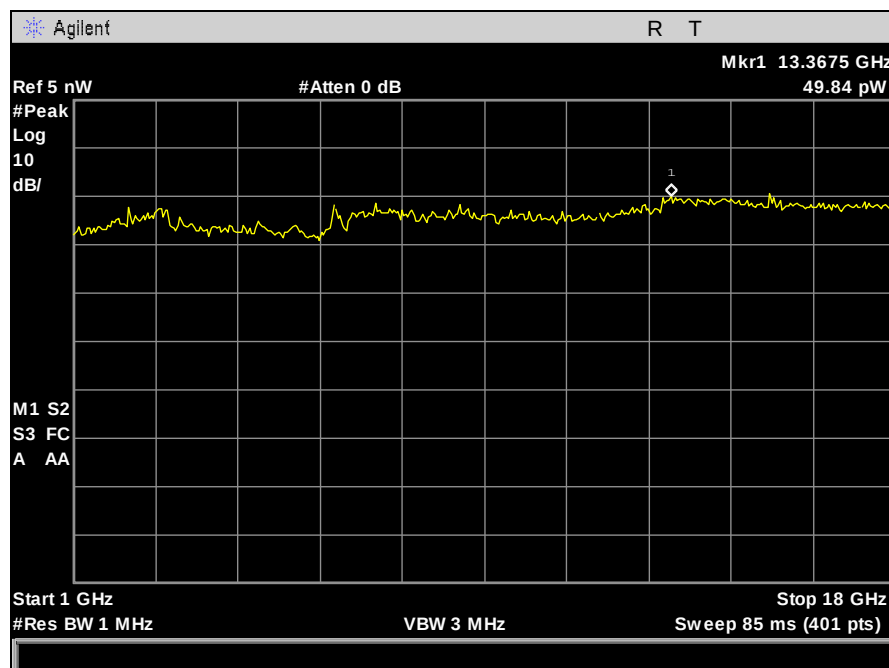
Plot 284. Receiver Spurious Emission, 1 GHz – 18 GHz, Port 3
