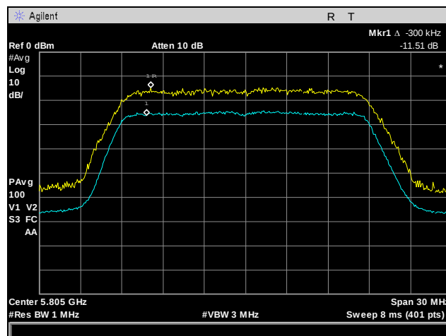
Plot 88. Peak Excursion Ratio, High Channel, 802.11n 20 MHz, Port 3
