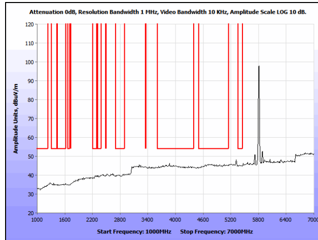
Plot 104. Radiated Spurious Emissions, 802.11a, High Channel, 1 GHz – 7 GHz, Average, 7 dBi Patch
