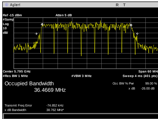
Plot 50. 99% Occupied Bandwidth, 802.11n 40 MHz, Port 2, High Channel
