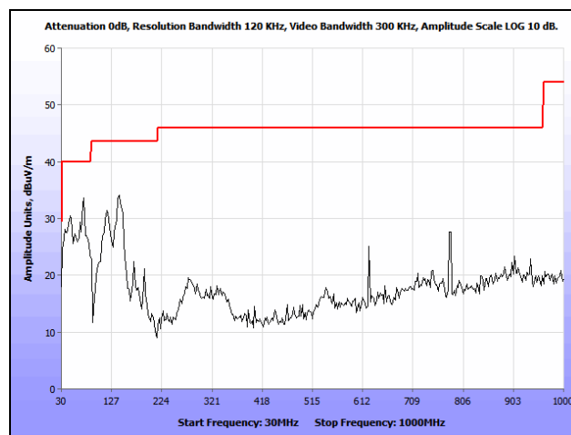
Plot 115. Radiated Spurious Emissions, 802.11n 20 MHz, High Channel, 30 MHz – 1 GHz, 7 dBi Patch
