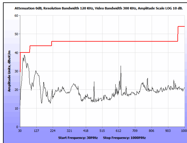
Plot 147. Radiated Spurious Emissions, 802.11n 20 MHz, Mid Channel, 30 MHz – 1 GHz, Ceiling
