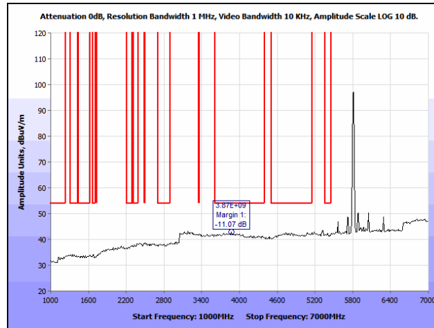
Plot 116. Radiated Spurious Emissions, 802.11n 20 MHz, High Channel, 1 GHz – 7 GHz, Average, 7 dBi Patch
