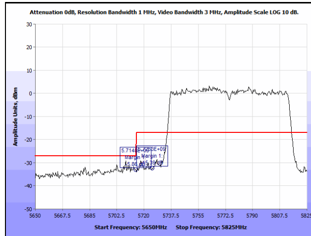
Plot 209. Radiated Band Edge, 802.11n 80 MHz, 7 dBi Patch Antenna (Band Edge @ 5725 & 5715 MHz)
