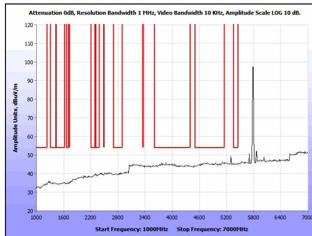
Plot 100. Radiated Spurious Emissions, 802.11a, Mid Channel, 1 GHz – 7 GHz, Average, 7 dBi Patch
