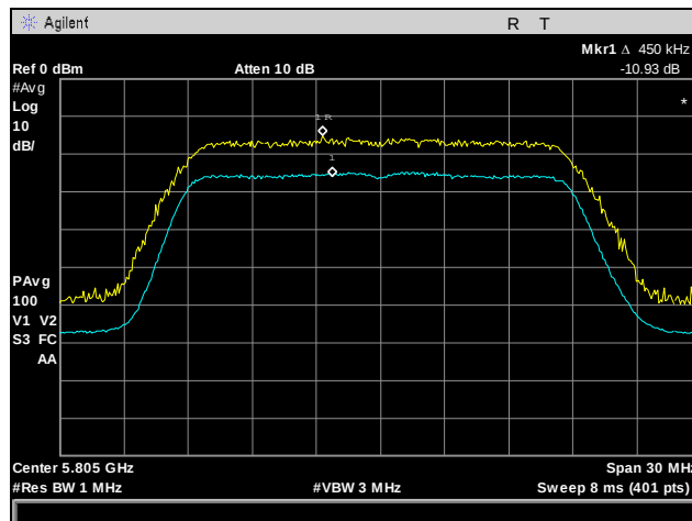
Plot 82. Peak Excursion Ratio, High Channel, 802.11n 20 MHz, Port 1
