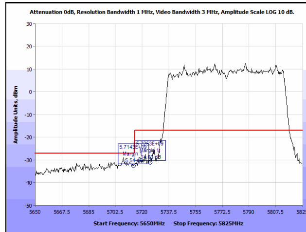
Plot 225. Radiated Band Edge, 802.11n 80 MHz, Omni Antenna (Band Edge @ 5725 & 5715 MHz)
