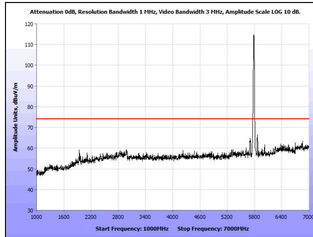
Plot 149. Radiated Spurious Emissions, 802.11n 20 MHz, Mid Channel, 1 GHz – 7 GHz, Peak, Ceiling
