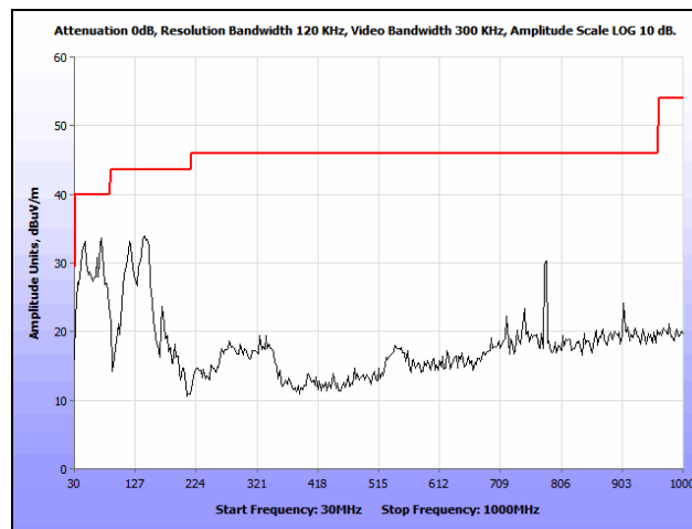
Plot 171. Radiated Spurious Emissions, 802.11a, Mid Channel, 30 MHz – 1 GHz, Omni
