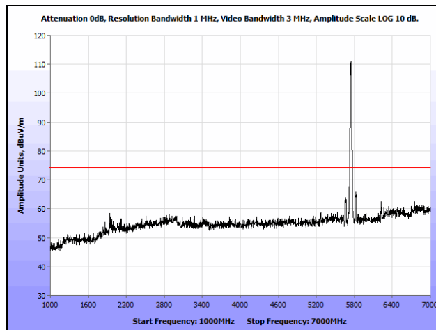
Plot 133. Radiated Spurious Emissions, 802.11a, Low Channel, 1 GHz – 7 GHz, Peak, Ceiling
