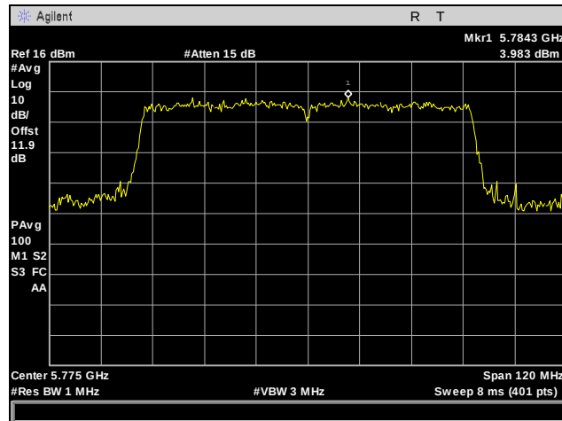
Plot 75. Power Spectral Density, 802.11n 80MHz, Port 2
