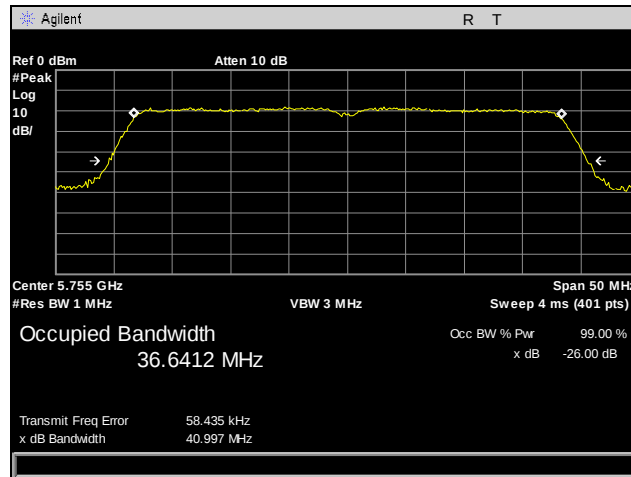
Plot 28. 26 dB Occupied Bandwidth, 802.11n 40 MHz, Port 2, Low Channel
