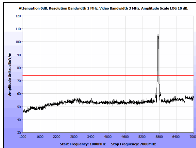
Plot 193. Radiated Spurious Emissions, 802.11n 40 MHz, Low Channel, 1 GHz – 7 GHz, Peak, Omni
