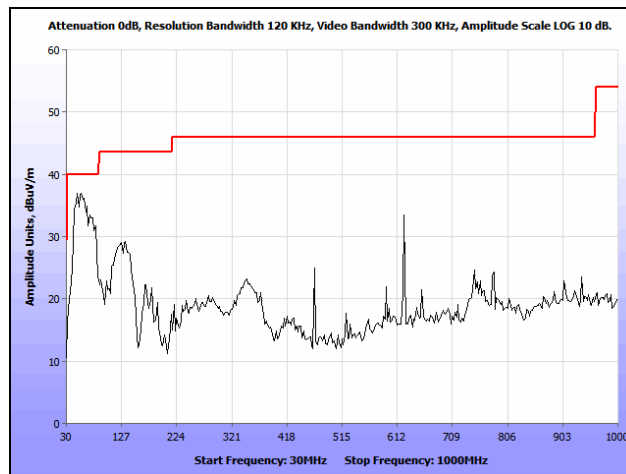
Plot 139. Radiated Spurious Emissions, 802.11a, High Channel, 30 MHz – 1 GHz, Ceiling
