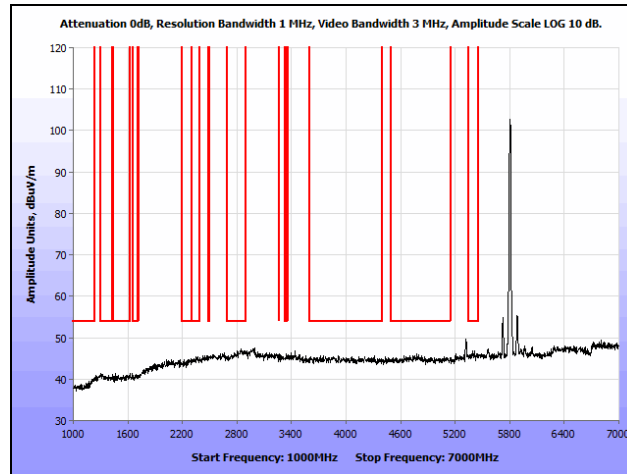
Plot 188. Radiated Spurious Emissions, 802.11n 20 MHz, High Channel, 1 GHz – 7 GHz, Average, Omni
