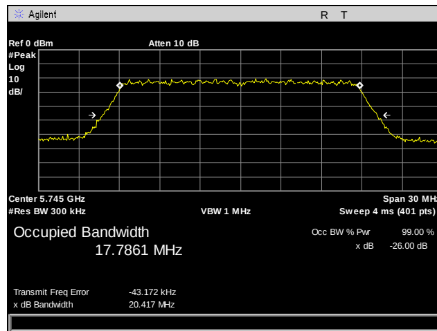
Plot 20. 26 dB Occupied Bandwidth, 802.11n 20 MHz, Port 2, Low Channel
