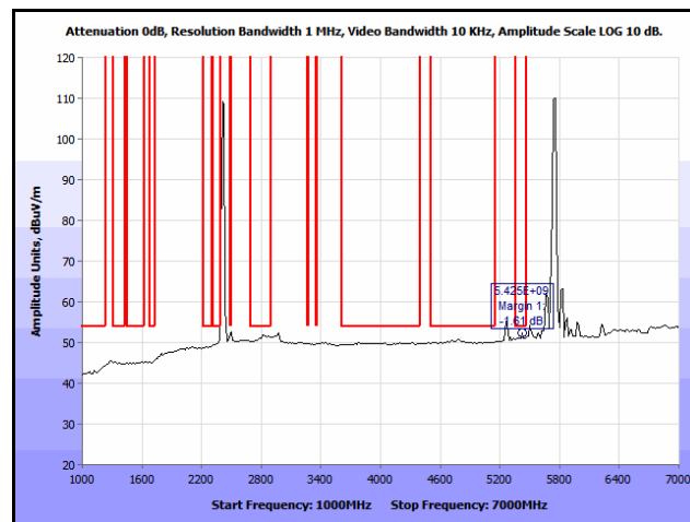
Plot 256. Co-location, Radiated Spurious Emissions, Patch, 802.11n 20 MHz, 2412 & 5785 MHz, 1 GHz – 7 GHz, Average
