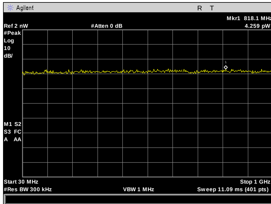
Plot 283. Receiver Spurious Emission, 30 MHz – 1 GHz, Port 3
