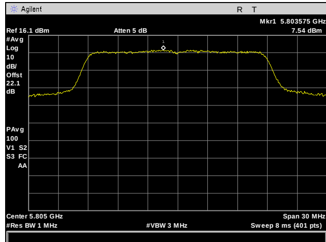
Plot 67. Power Spectral Density, High Channel, 802.11n 20 MHz, Port 3
