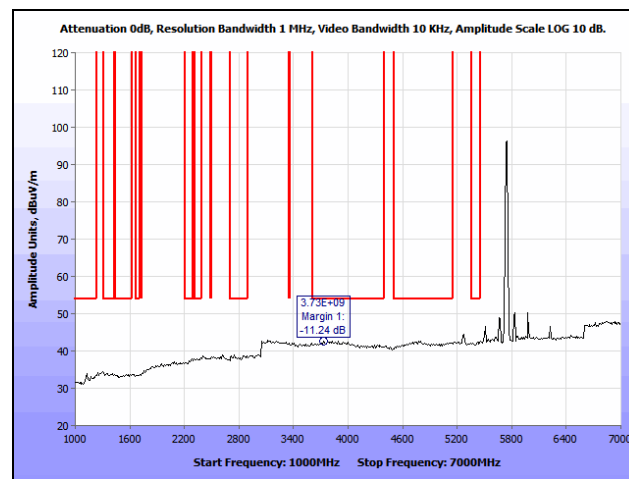
Plot 108. Radiated Spurious Emissions, 802.11n 20 MHz, Low Channel, 1 GHz – 7 GHz, Average, 7 dBi Patch
