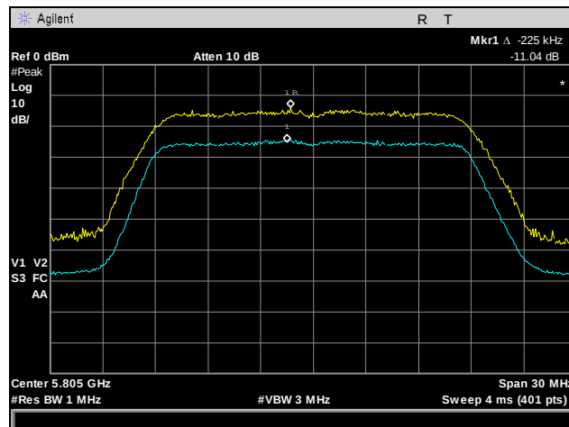
Plot 85. Peak Excursion Ratio, High Channel, 802.11n 20 MHz, Port 2
