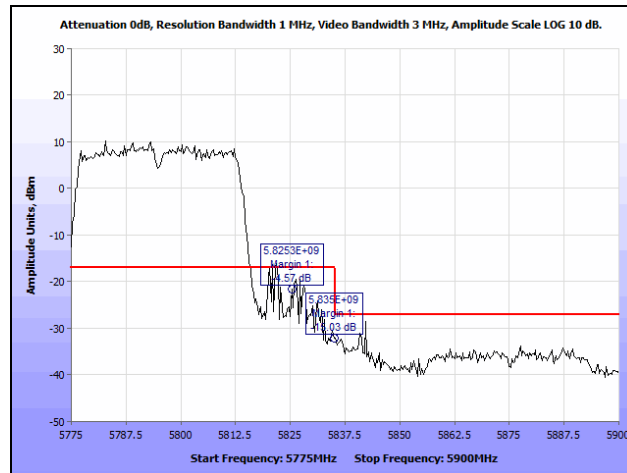
Plot 216. Radiated Band Edge, 802.11n 40 MHz, High Channel, Ceiling Antenna (Band Edge @ 5825 & 5835 MHz)
