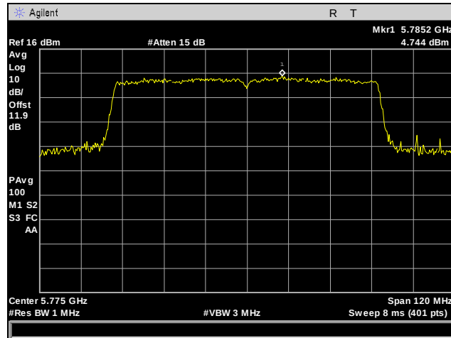
Plot 74. Power Spectral Density, 802.11n 80MHz, Port 1
