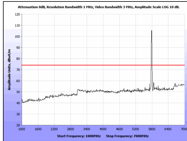
Plot 113. Radiated Spurious Emissions, 802.11n 20 MHz, Mid Channel, 1 GHz – 7 GHz, Peak, 7 dBi Patch
