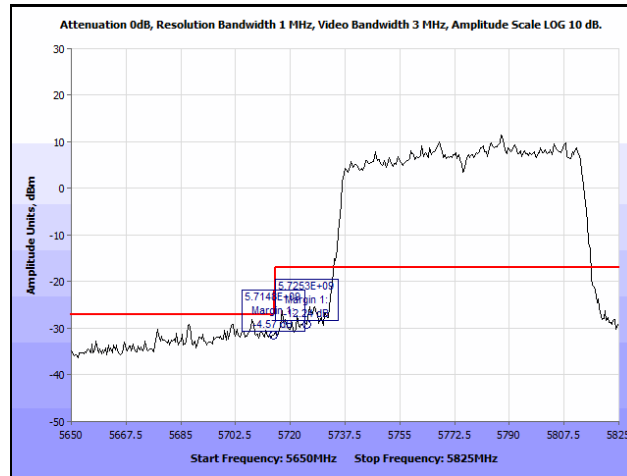
Plot 217. Radiated Band Edge, 802.11n 80 MHz, Ceiling Antenna (Band Edge @ 5725 & 5715 MHz)
