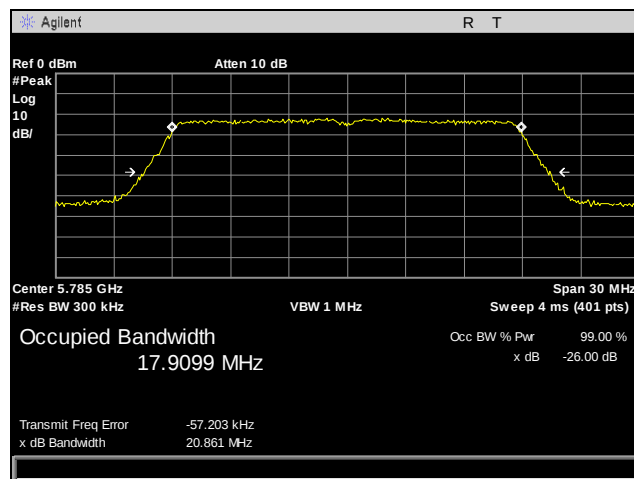
Plot 18. 26 dB Occupied Bandwidth, 802.11n 20 MHz, Port 1, Mid Channel
