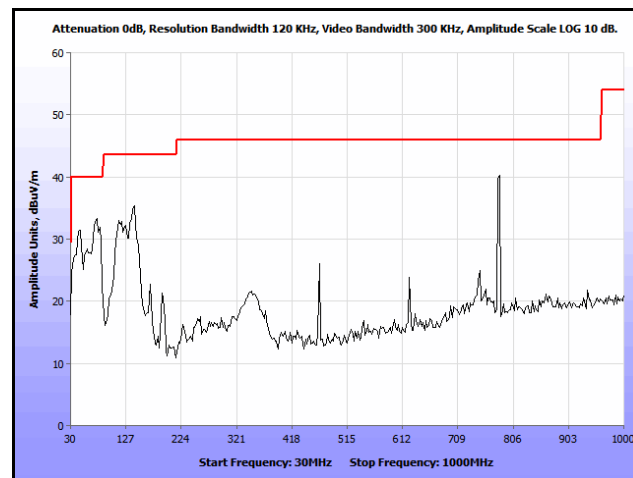
Plot 243. Co-location, Radiated Spurious Emissions, Omni, 802.11n 20 MHz, 5300 & 5785 MHz, 30 MHz – 1 GHz
