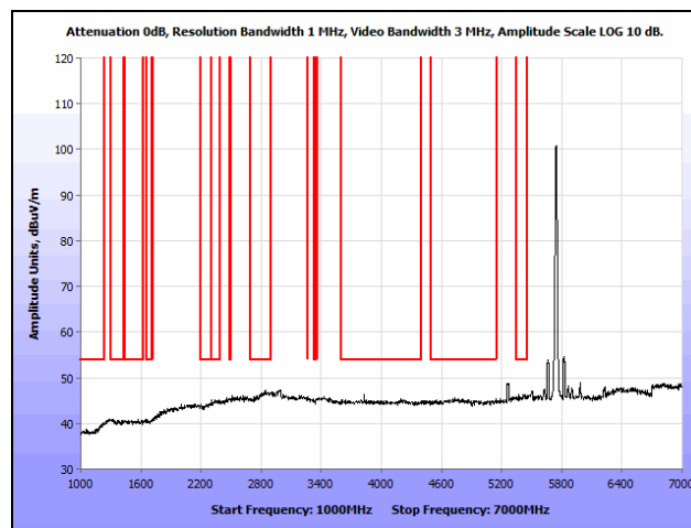
Plot 180. Radiated Spurious Emissions, 802.11n 20 MHz, Low Channel, 1 GHz – 7 GHz, Average, Omni
