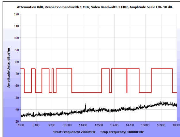
Plot 186. Radiated Spurious Emissions, 802.11n 20 MHz, Mid Channel, 7 GHz – 18 GHz, Omni
