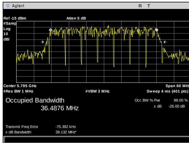
Plot 48. 99% Occupied Bandwidth, 802.11n 40 MHz, Port 1, High Channel
