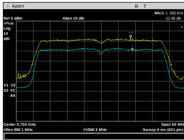
Plot 93. Peak Excursion Ratio, Low Channel, 802.11n 40 MHz, Port 3
