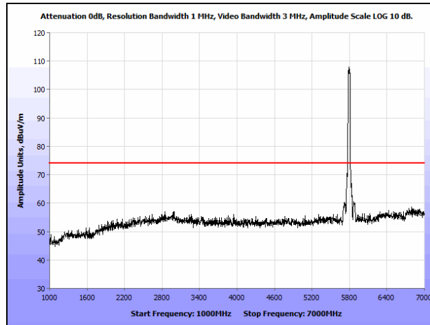
Plot 197. Radiated Spurious Emissions, 802.11n 40 MHz, High Channel, 1 GHz – 7 GHz, Peak, Omni
