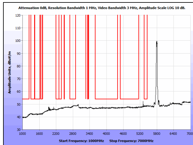
Plot 160. Radiated Spurious Emissions, 802.11n 40 MHz, High Channel, 1 GHz – 7 GHz, Average, Ceiling
