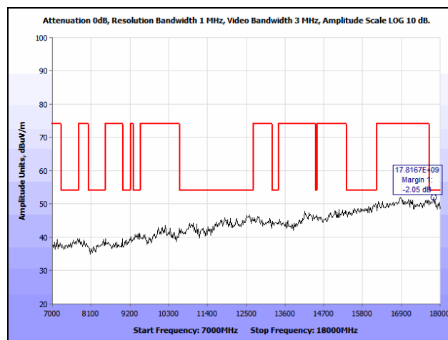
Plot 118. Radiated Spurious Emissions, 802.11n 20 MHz, High Channel, 7 GHz – 18 GHz, 7 dBi Patch
