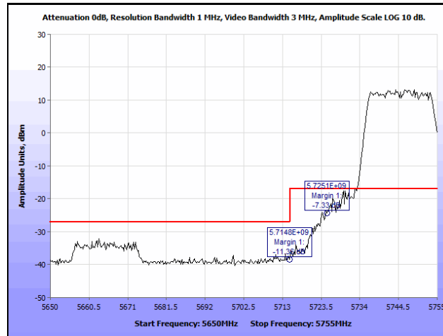
Plot 213. Radiated Band Edge, 802.11n 20 MHz, Low Channel, Ceiling Antenna (Band Edge @ 5715 & 5725 MHz)
