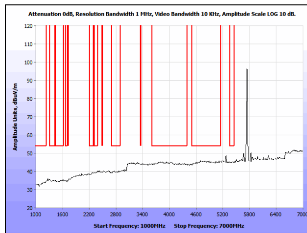
Plot 96. Radiated Spurious Emissions, 802.11a, Low Channel, 1 GHz – 7 GHz, Average, 7 dBi Patch
