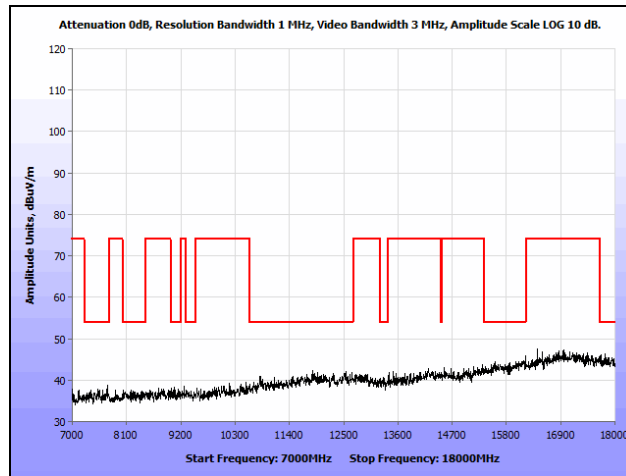
Plot 138. Radiated Spurious Emissions, 802.11a, Mid Channel, 7 GHz – 18 GHz, Ceiling
