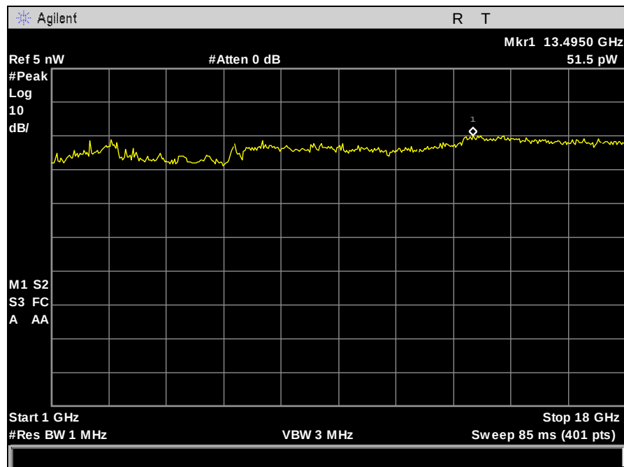
Plot 282. Receiver Spurious Emission, 1 GHz – 18 GHz, Port 2
