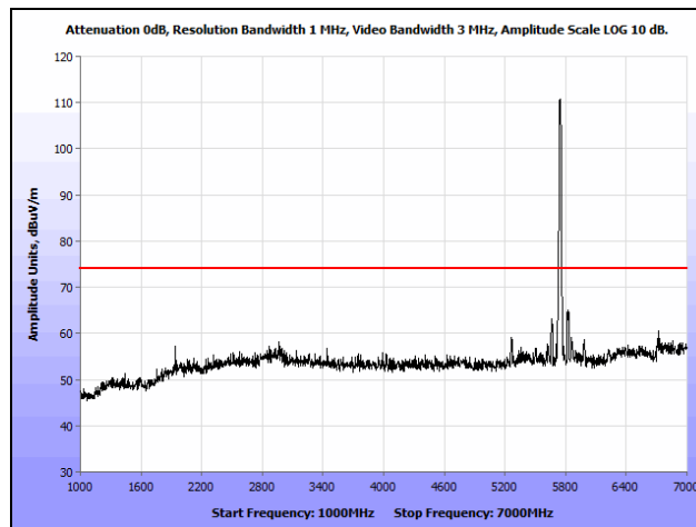
Plot 169. Radiated Spurious Emissions, 802.11a, Low Channel, 1 GHz – 7 GHz, Peak, Omni
