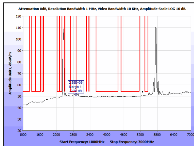
Plot 260. Co-location, Radiated Spurious Emissions, Patch, 802.11n 20 MHz, 2437 & 5785 MHz, 1 GHz – 7 GHz, Average
