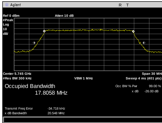
Plot 14. 26 dB Occupied Bandwidth, 802.11a, Port 1, Low Channel
