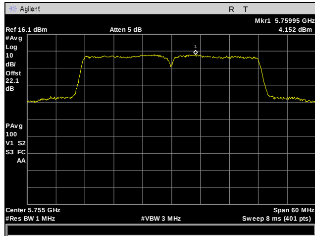
Plot 70. Power Spectral Density, Low Channel, 802.11n 40 MHz, Port 2
