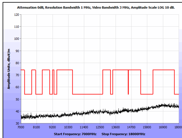
Plot 178. Radiated Spurious Emissions, 802.11a, High Channel, 7 GHz – 18 GHz, Omni
