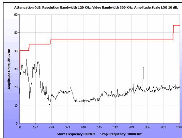
Plot 175. Radiated Spurious Emissions, 802.11a, High Channel, 30 MHz – 1 GHz, Omni
