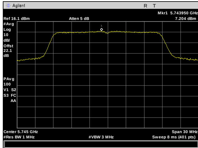
Plot 59. Power Spectral Density, Low Channel, 802.11n 20 MHz, Port 1
