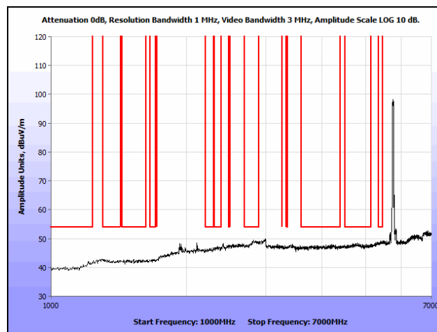
Plot 156. Radiated Spurious Emissions, 802.11n 40 MHz, Low Channel, 1 GHz – 7 GHz, Average, Ceiling
