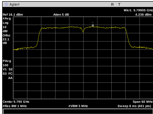
Plot 71. Power Spectral Density, High Channel, 802.11n 40 MHz, Port 2
