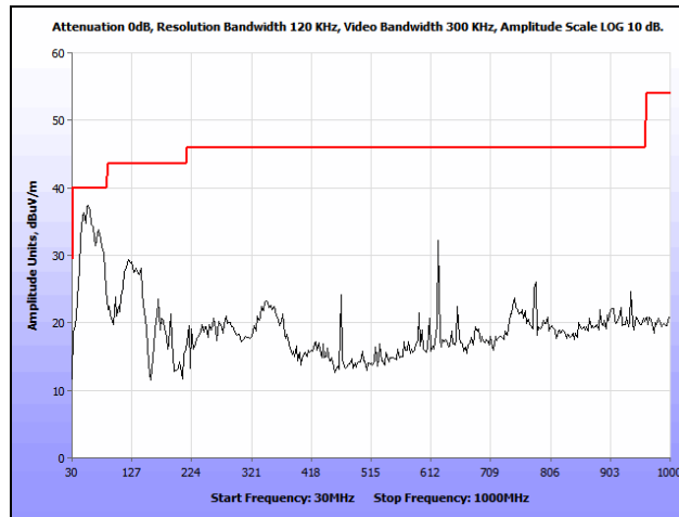
Plot 143. Radiated Spurious Emissions, 802.11n 20 MHz, Low Channel, 30 MHz – 1 GHz, Ceiling
