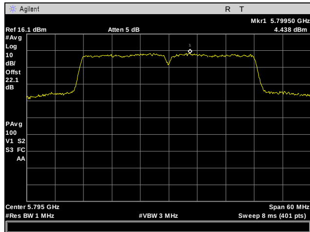
Plot 73. Power Spectral Density, High Channel, 802.11n 40 MHz, Port 3
