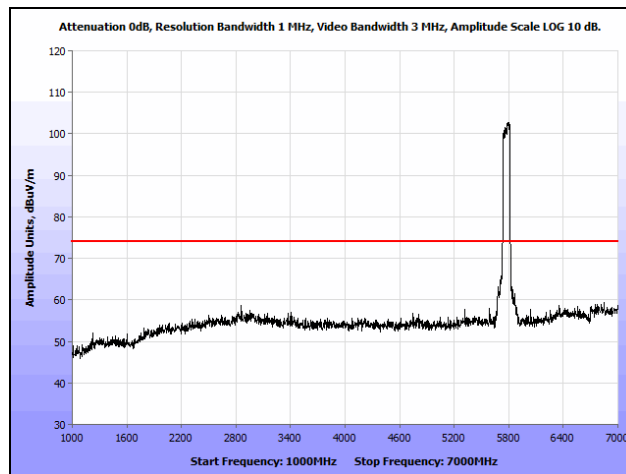
Plot 201. Radiated Spurious Emissions, 802.11n 80 MHz, Low Channel, 1 GHz – 7 GHz, Peak, Omni
