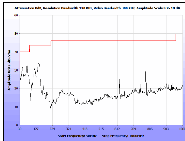
Plot 111. Radiated Spurious Emissions, 802.11n 20 MHz, Mid Channel, 30 MHz – 1 GHz, 7 dBi Patch
