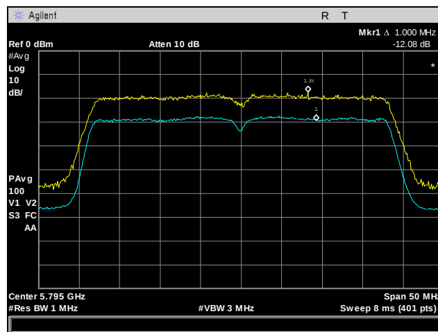
Plot 94. Peak Excursion Ratio, High Channel, 802.11n 40 MHz, Port 3
