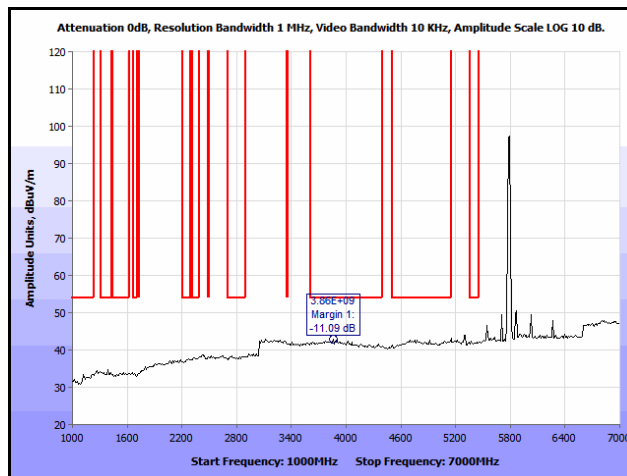
Plot 112. Radiated Spurious Emissions, 802.11n 20 MHz, Mid Channel, 1 GHz – 7 GHz, Average, 7 dBi Patch
