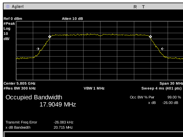
Plot 19. 26 dB Occupied Bandwidth, 802.11n 20 MHz, Port 1, High Channel
