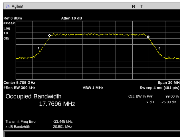
Plot 21. 26 dB Occupied Bandwidth, 802.11n 20 MHz, Port 2, Mid Channel
