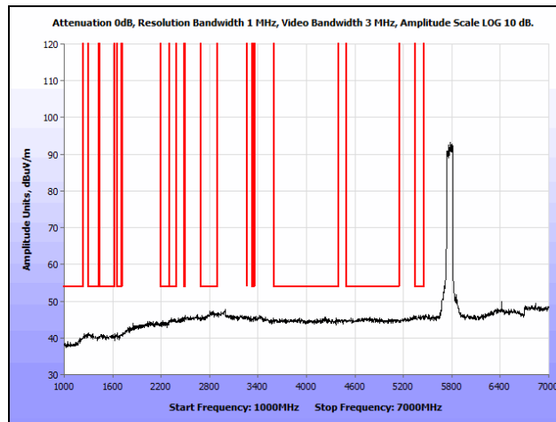
Plot 200. Radiated Spurious Emissions, 802.11n 80 MHz, Low Channel, 1 GHz – 7 GHz, Average, Omni
