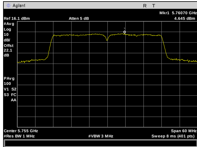
Plot 68. Power Spectral Density, Low Channel, 802.11n 40 MHz, Port 1
