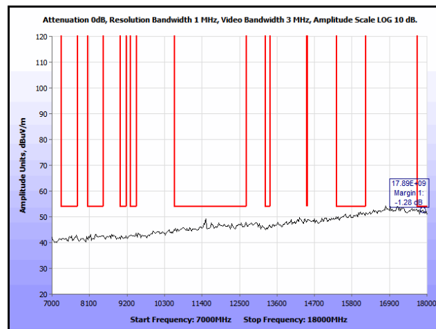
Plot 266. Co-location, Radiated Spurious Emissions, Patch, 802.11n 20 MHz, 2462 & 5785 MHz, 7 GHz – 18 GHz, Peak
