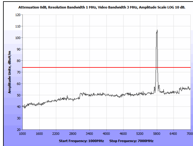
Plot 125. Radiated Spurious Emissions, 802.11n 40 MHz, High Channel, 1 GHz – 7 GHz, Peak, 7 dBi Patch
