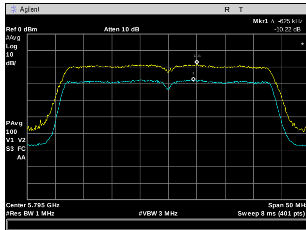
Plot 90. Peak Excursion Ratio, High Channel, 802.11n 40 MHz, Port 1
