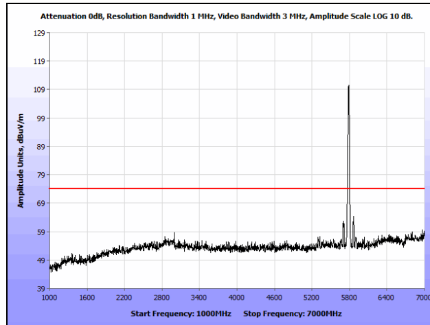
Plot 185. Radiated Spurious Emissions, 802.11n 20 MHz, Mid Channel, 1 GHz – 7 GHz, Peak, Omni
