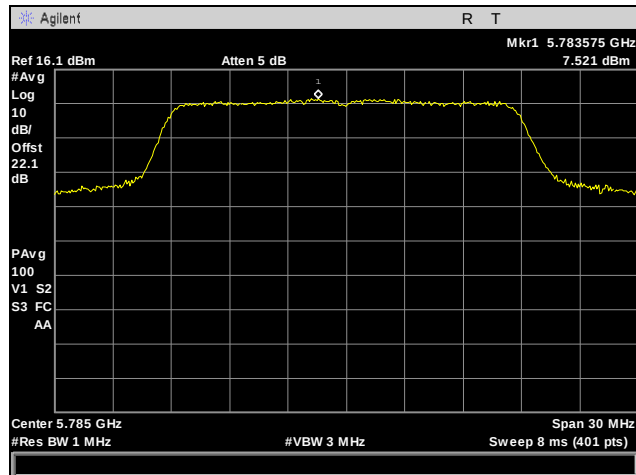
Plot 60. Power Spectral Density, Mid Channel, 802.11n 20 MHz, Port 1
