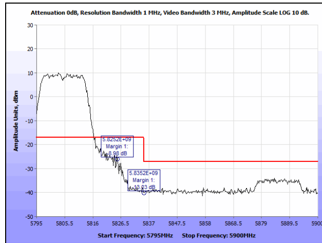
Plot 212. Radiated Band Edge, 802.11a, High Channel, Ceiling Antenna (Band Edge @ 5825 & 5835 MHz)
