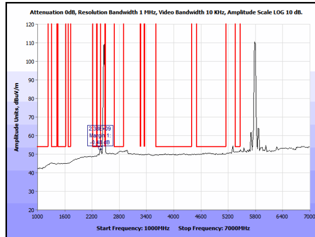
Plot 264. Co-location, Radiated Spurious Emissions, Patch, 802.11n 20 MHz, 2462 & 5785 MHz, 1 GHz – 7 GHz, Average
