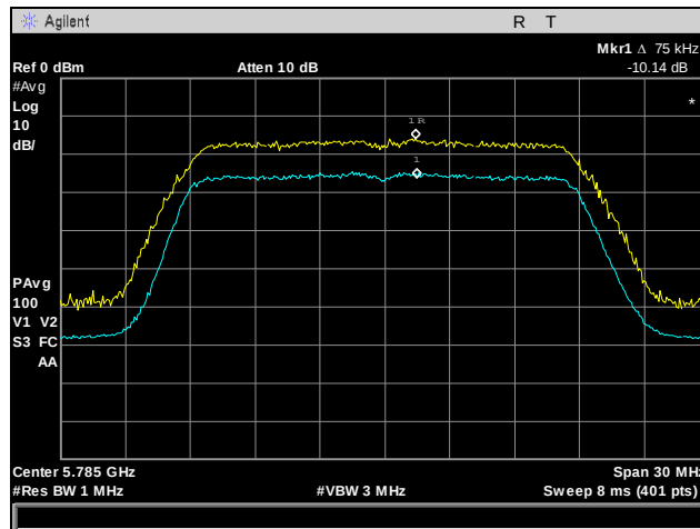
Plot 81. Peak Excursion Ratio, Mid Channel, 802.11n 20 MHz, Port 1
