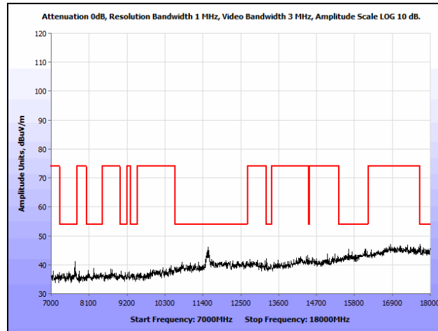
Plot 166. Radiated Spurious Emissions, 802.11n 80 MHz, Low Channel, 7 GHz – 18 GHz, Ceiling
