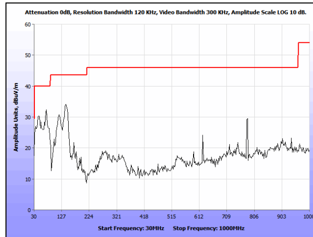
Plot 107. Radiated Spurious Emissions, 802.11n 20 MHz, Low Channel, 30 MHz – 1 GHz, 7 dBi Patch
