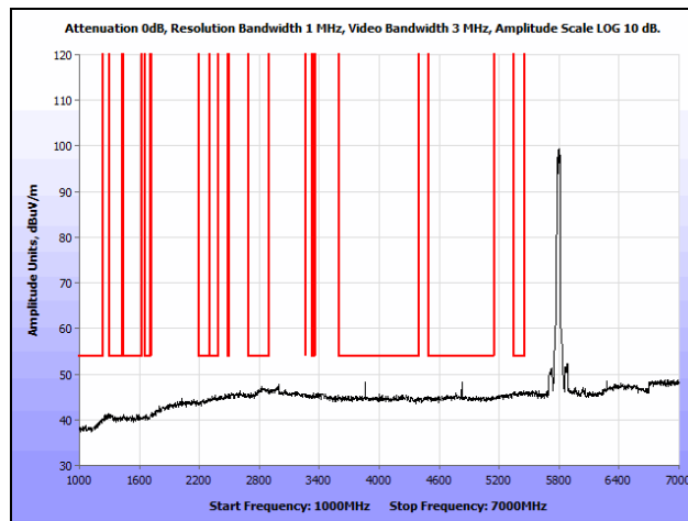
Plot 196. Radiated Spurious Emissions, 802.11n 40 MHz, High Channel, 1 GHz – 7 GHz, Average, Omni
