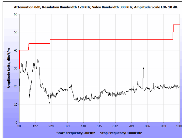
Plot 199. Radiated Spurious Emissions, 802.11n 80 MHz, Low Channel, 30 MHz – 1 GHz, Omni
