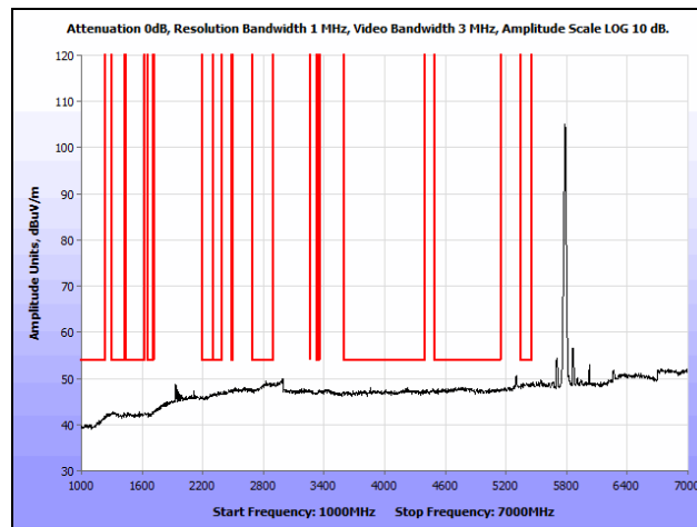
Plot 148. Radiated Spurious Emissions, 802.11n 20 MHz, Mid Channel, 1 GHz – 7 GHz, Average, Ceiling
