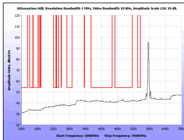
Plot 120. Radiated Spurious Emissions, 802.11n 40 MHz, Low Channel, 1 GHz – 7 GHz, Average, 7 dBi Patch
