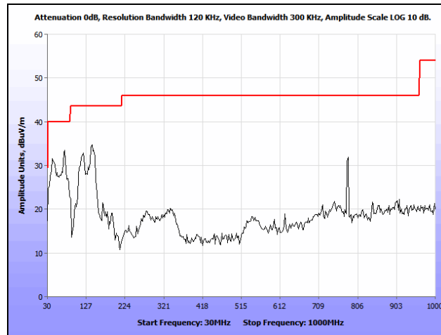
Plot 191. Radiated Spurious Emissions, 802.11n 40 MHz, Low Channel, 30 MHz – 1 GHz, Omni
