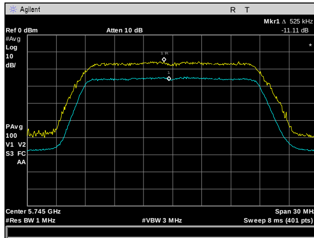
Plot 80. Peak Excursion Ratio, Low Channel, 802.11n 20 MHz, Port 1
