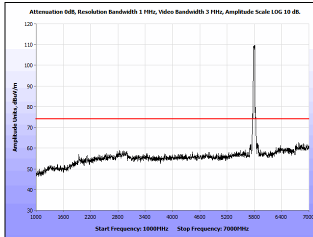
Plot 161. Radiated Spurious Emissions, 802.11n 40 MHz, High Channel, 1 GHz – 7 GHz, Peak, Ceiling
