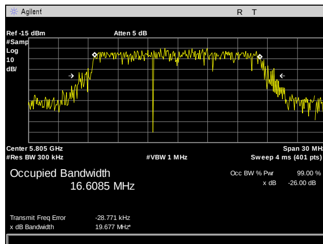
Plot 37. 99% Occupied Bandwidth, 802.11a, Port 1, High Channel
