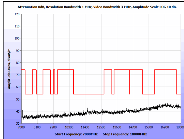
Plot 202. Radiated Spurious Emissions, 802.11n 80 MHz, Low Channel, 7 GHz – 18 GHz, Omni
