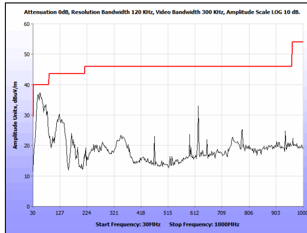
Plot 135. Radiated Spurious Emissions, 802.11a, Mid Channel, 30 MHz – 1 GHz, Ceiling
