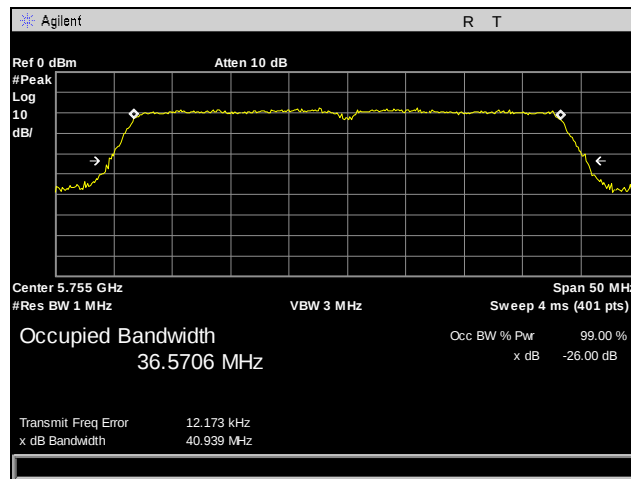
Plot 30. 26 dB Occupied Bandwidth, 802.11n 40 MHz, Port 3, Low Channel
