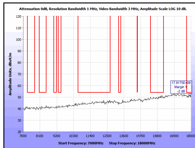
Plot 262. Co-location, Radiated Spurious Emissions, Patch, 802.11n 20 MHz, 2437 & 5785 MHz, 7 GHz – 18 GHz, Peak
