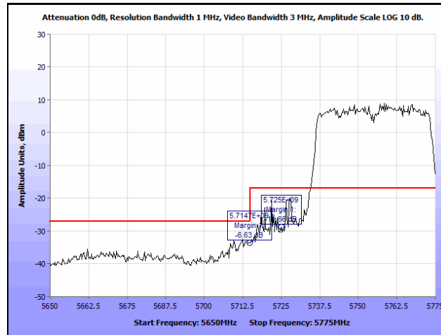
Plot 215. Radiated Band Edge, 802.11n 40 MHz, Low Channel, Ceiling Antenna (Band Edge @ 5715 & 5725 MHz)
