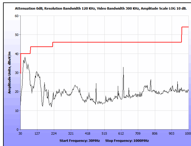
Plot 159. Radiated Spurious Emissions, 802.11n 40 MHz, High Channel, 30 MHz – 1 GHz, Ceiling
