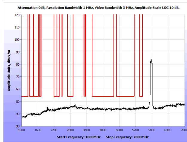
Plot 128. Radiated Spurious Emissions, 802.11n 80 MHz, 1 GHz – 7 GHz, Average, 7 dBi Patch
