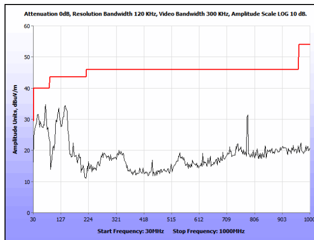
Plot 183. Radiated Spurious Emissions, 802.11n 20 MHz, Mid Channel, 30 MHz – 1 GHz, Omni
