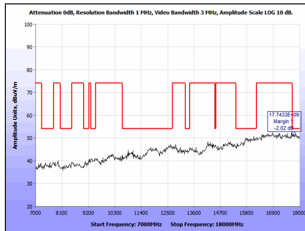
Plot 106. Radiated Spurious Emissions, 802.11a, High Channel, 7 GHz – 18 GHz, 7 dBi Patch
