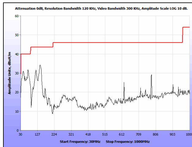
Plot 99. Radiated Spurious Emissions, 802.11a, Mid Channel, 30 MHz – 1 GHz, 7 dBi Patch
