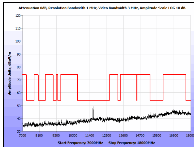
Plot 154. Radiated Spurious Emissions, 802.11n 20 MHz, High Channel, 7 GHz – 18 GHz, Ceiling
