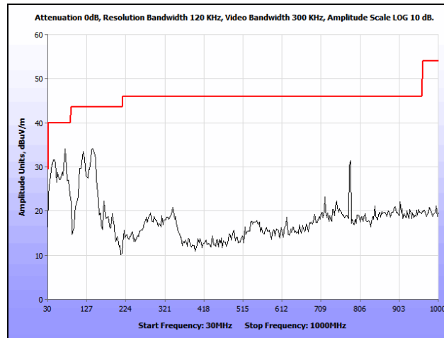
Plot 179. Radiated Spurious Emissions, 802.11n 20 MHz, Low Channel, 30 MHz – 1 GHz, Omni
