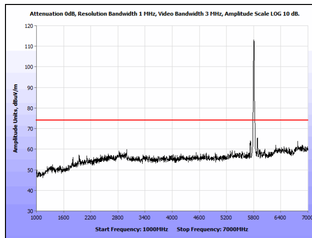
Plot 153. Radiated Spurious Emissions, 802.11n 20 MHz, High Channel, 1 GHz – 7 GHz, Peak, Ceiling
