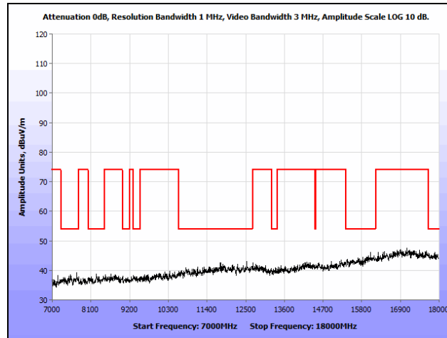
Plot 130. Radiated Spurious Emissions, 802.11n 80 MHz, 7 GHz – 18 GHz, 7 dBi
