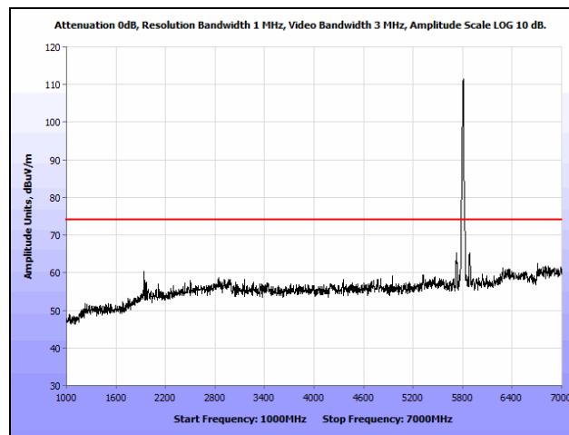
Plot 141. Radiated Spurious Emissions, 802.11a, High Channel, 1 GHz – 7 GHz, Peak, Ceiling
