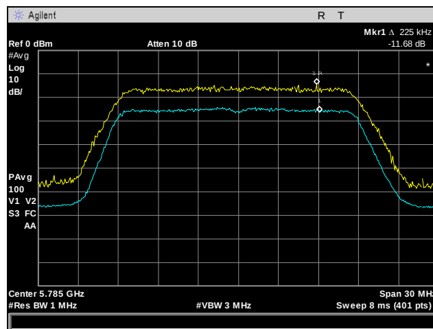
Plot 87. Peak Excursion Ratio, Mid Channel, 802.11n 20 MHz, Port 3
