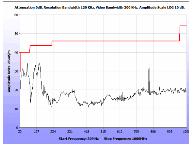
Plot 195. Radiated Spurious Emissions, 802.11n 40 MHz, High Channel, 30 MHz – 1 GHz, Omni
