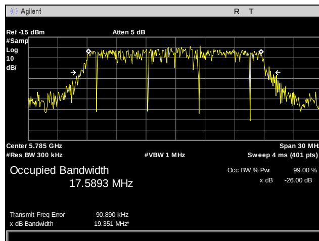
Plot 45. 99% Occupied Bandwidth, 802.11n 20 MHz, Port 3, Mid Channel
