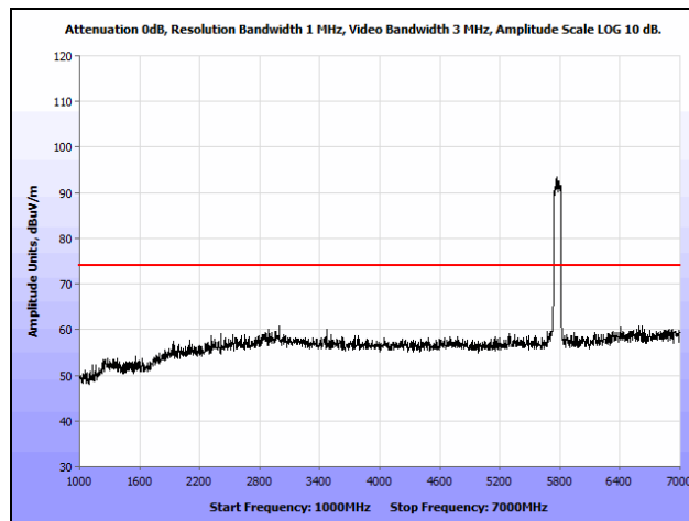
Plot 129. Radiated Spurious Emissions, 802.11n 80 MHz, 1 GHz – 7 GHz, Peak, 7 dBi Patch
