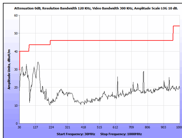
Plot 103. Radiated Spurious Emissions, 802.11a, High Channel, 30 MHz – 1 GHz, 7 dBi Patch
