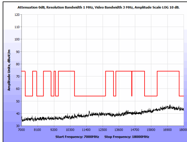
Plot 198. Radiated Spurious Emissions, 802.11n 40 MHz, High Channel, 7 GHz – 18 GHz, Omni
