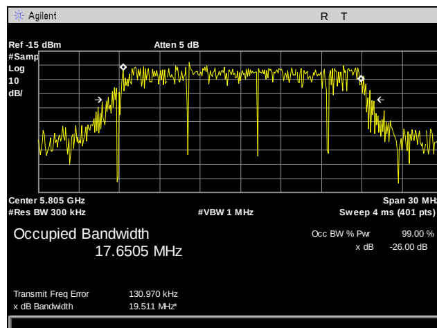
Plot 43. 99% Occupied Bandwidth, 802.11n 20 MHz, Port 2, High Channel
