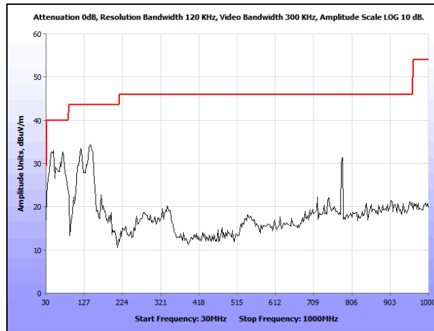
Plot 167. Radiated Spurious Emissions, 802.11a, Low Channel, 30 MHz – 1 GHz, Omni
