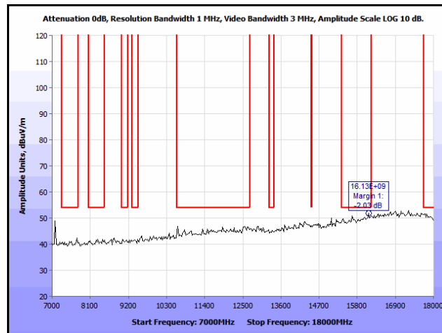
Plot 246. Co-location, Radiated Spurious Emissions, Omni, 802.11n 20 MHz, 5300 & 5785 MHz, 7 GHz – 18 GHz, Peak
