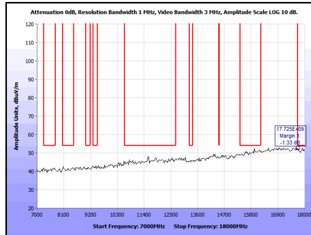
Plot 258. Co-location, Radiated Spurious Emissions, Patch, 802.11n 20 MHz, 2412 & 5785 MHz, 7 GHz – 18 GHz, Peak
