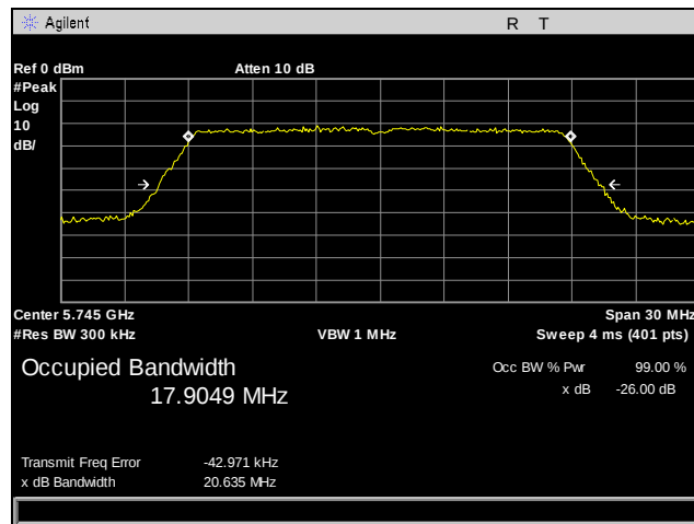
Plot 17. 26 dB Occupied Bandwidth, 802.11n 20 MHz, Port 1, Low Channel
