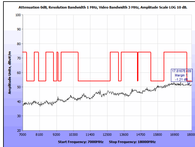
Plot 98. Radiated Spurious Emissions, 802.11a, Low Channel, 7 GHz – 18 GHz, 7 dBi Patch
