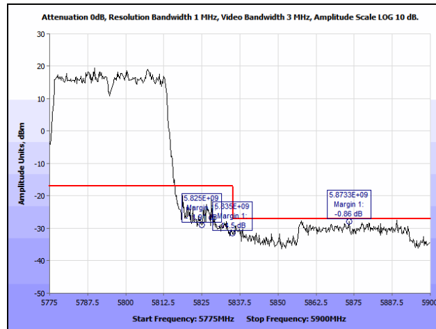
Plot 208. Radiated Band Edge, 802.11n 40 MHz, High Channel, 7 dBi Patch Antenna (Band Edge @ 5825 & 5835 MHz)
