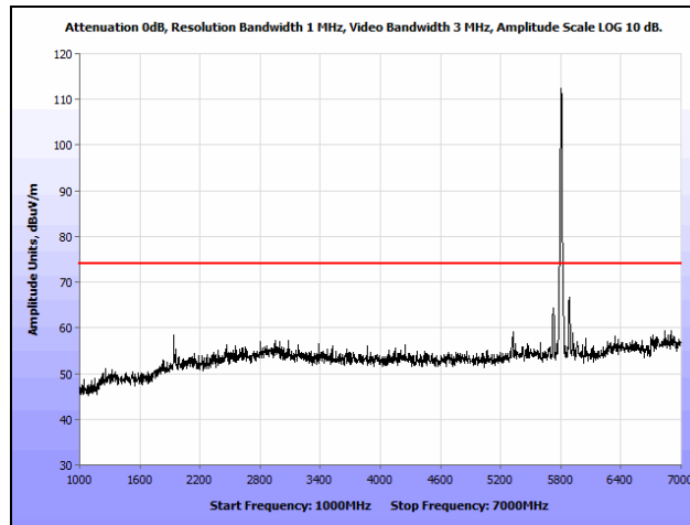
Plot 177. Radiated Spurious Emissions, 802.11a, High Channel, 1 GHz – 7 GHz, Peak, Omni
