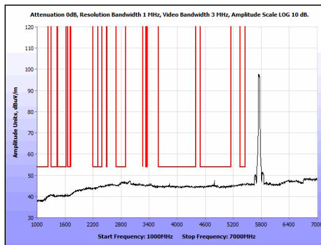
Plot 192. Radiated Spurious Emissions, 802.11n 40 MHz, Low Channel, 1 GHz – 7 GHz, Average, Omni
