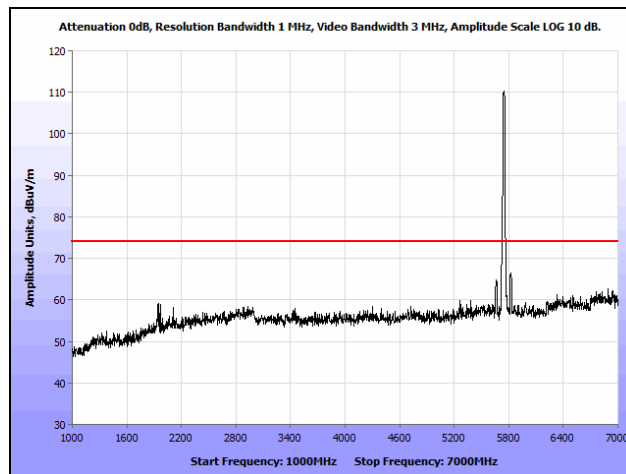
Plot 145. Radiated Spurious Emissions, 802.11n 20 MHz, Low Channel, 1 GHz – 7 GHz, Peak, Ceiling
