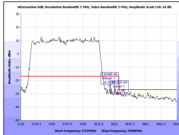
Plot 226. Radiated Band Edge, 802.11n 80 MHz, Omni Antenna (Band Edge @ 5835 & 5825 MHz)
