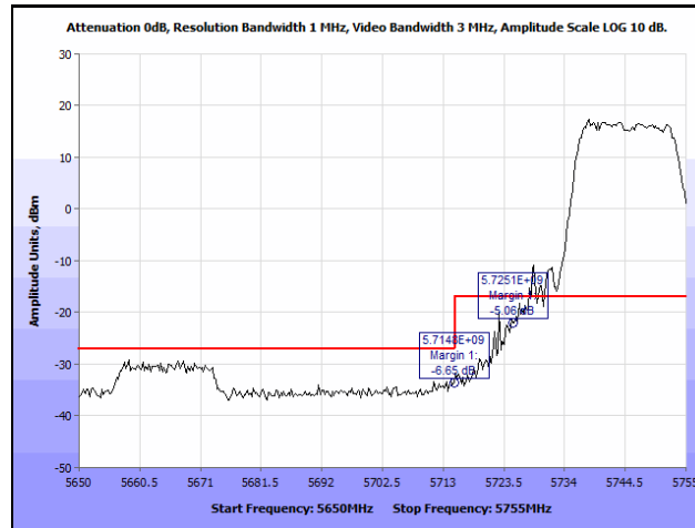
Plot 219. Radiated Band Edge, 802.11a, Low Channel, Omni Antenna (Band Edge @ 5715 & 5725 MHz)
