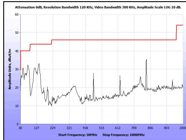
Plot 255. Co-location, Radiated Spurious Emissions, Patch, 802.11n 20 MHz, 2412 & 5785 MHz, 30 MHz – 1 GHz
