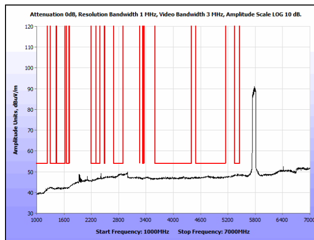
Plot 164. Radiated Spurious Emissions, 802.11n 80 MHz, Low Channel, 1 GHz – 7 GHz, Average, Ceiling
