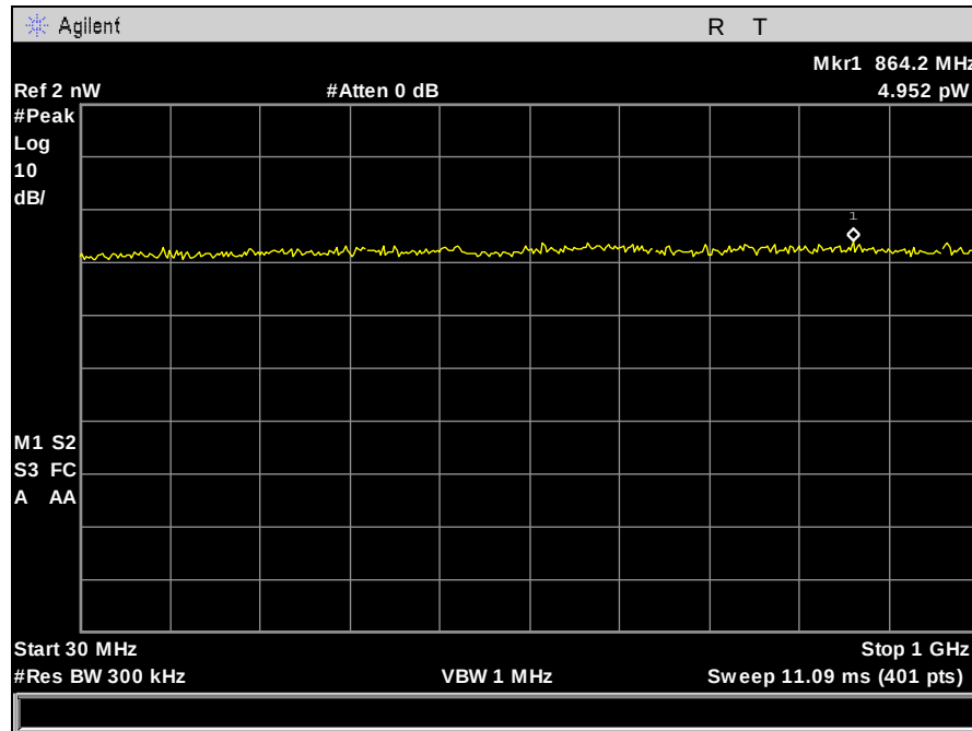
Plot 279. Receiver Spurious Emission, 30 MHz – 1 GHz, Port 1
