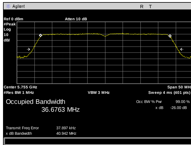
Plot 26. 26 dB Occupied Bandwidth, 802.11n 40 MHz, Port 1, Low Channel
