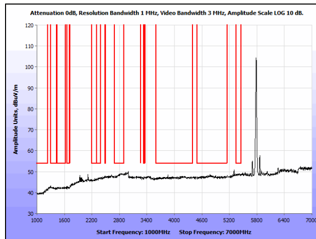
Plot 136. Radiated Spurious Emissions, 802.11a, Mid Channel, 1 GHz – 7 GHz, Average, Ceiling
