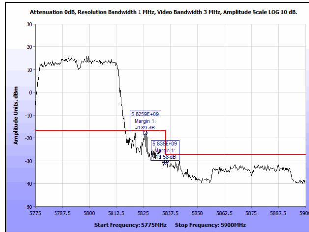
Plot 224. Radiated Band Edge, 802.11n 40 MHz, High Channel, Omni Antenna (Band Edge @ 5825 & 5835 MHz)
