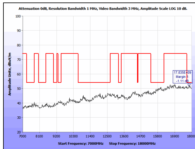
Plot 102. Radiated Spurious Emissions, 802.11a, Mid Channel, 7 GHz – 18 GHz, 7 dBi Patch
