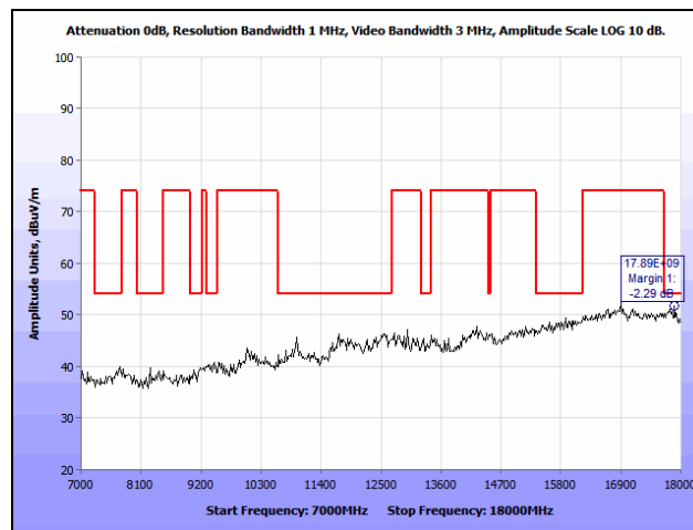
Plot 114. Radiated Spurious Emissions, 802.11n 20 MHz, Mid Channel, 7 GHz – 18 GHz, 7 dBi Patch
