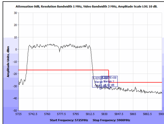
Plot 210. Radiated Band Edge, 802.11n 80 MHz, 7 dBi Patch Antenna (Band Edge @ 5825 & 5835 MHz)
