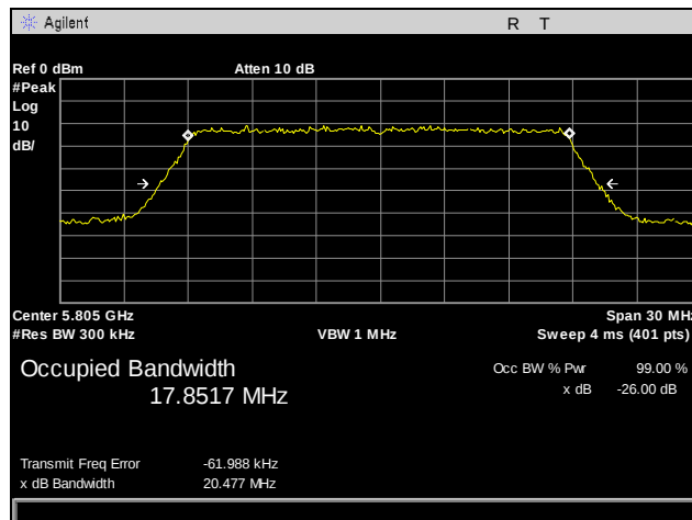
Plot 16. 26 dB Occupied Bandwidth, 802.11a, Port 1, High Channel
