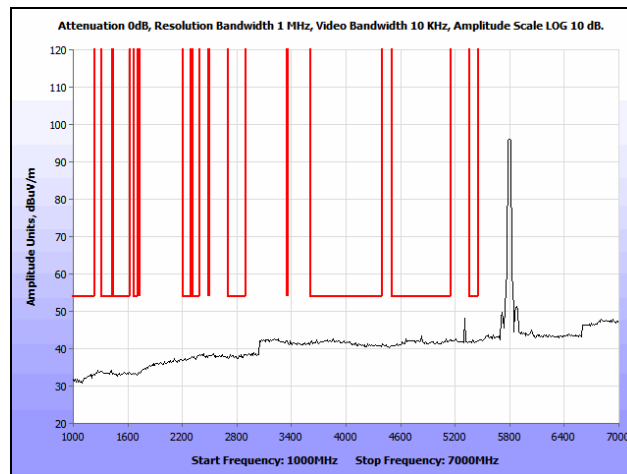
Plot 124. Radiated Spurious Emissions, 802.11n 40 MHz, High Channel, 1 GHz – 7 GHz, Average, 7 dBi Patch
