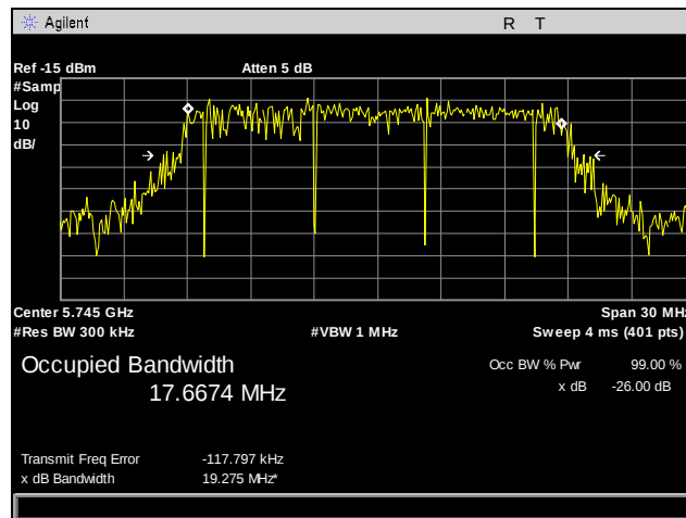
Plot 41. 99% Occupied Bandwidth, 802.11n 20 MHz, Port 2, Low Channel
