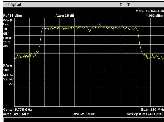
Plot 76. Power Spectral Density, 802.11n 80MHz, Port 3
