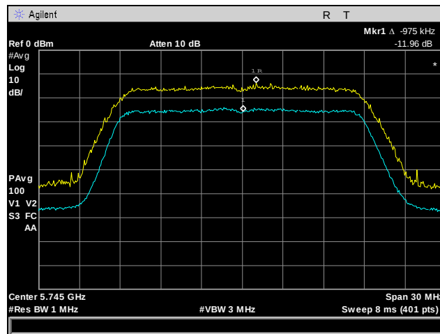
Plot 86. Peak Excursion Ratio, Low Channel, 802.11n 20 MHz, Port 3
