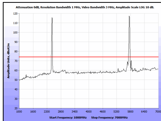
Plot 257. Co-location, Radiated Spurious Emissions, Patch, 802.11n 20 MHz, 2412 & 5785 MHz, 1 GHz – 7 GHz, Peak
