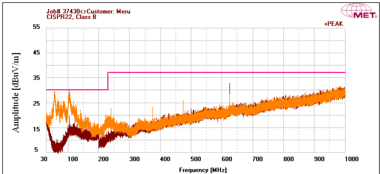
Plot 7. Radiated Emissions, 30 MHz - 1 GHz, CISPR Limits, AC-DC Power Supply
