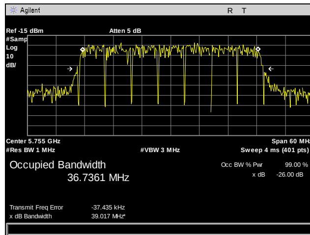
Plot 51. 99% Occupied Bandwidth, 802.11n 40 MHz, Port 3, Low Channel
