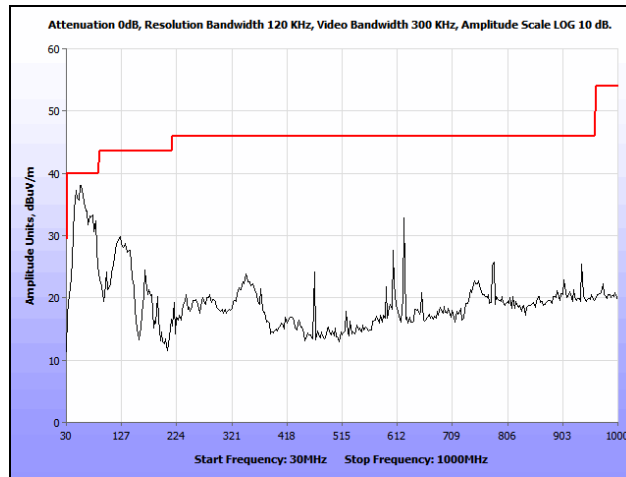
Plot 131. Radiated Spurious Emissions, 802.11a, Low Channel, 30 MHz – 1 GHz, Ceiling
