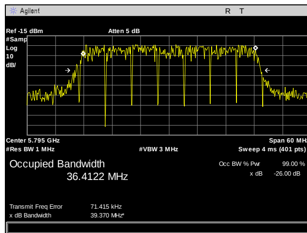
Plot 52. 99% Occupied Bandwidth, 802.11n 40 MHz, Port 3, High Channel
