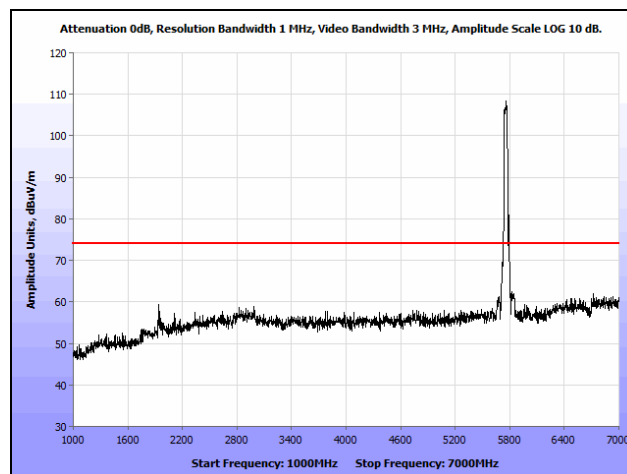
Plot 157. Radiated Spurious Emissions, 802.11n 40 MHz, Low Channel, 1 GHz – 7 GHz, Peak, Ceiling
