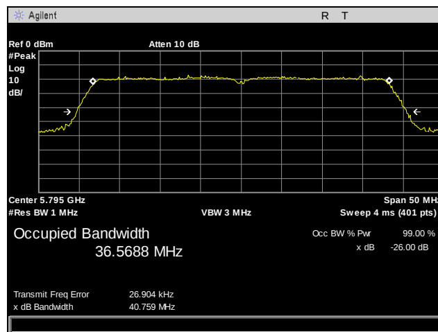
Plot 31. 26 dB Occupied Bandwidth, 802.11n 40 MHz, Port 3, High Channel
