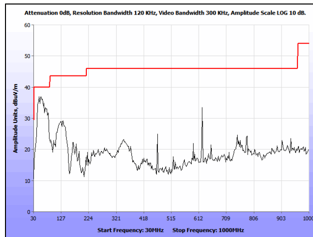
Plot 151. Radiated Spurious Emissions, 802.11n 20 MHz, High Channel, 30 MHz – 1 GHz, Ceiling
