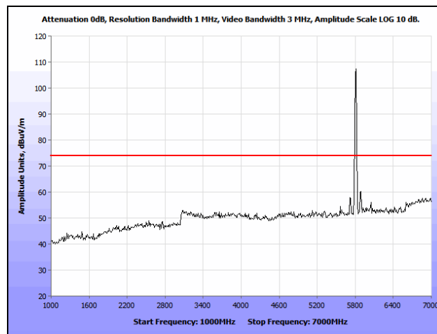
Plot 117. Radiated Spurious Emissions, 802.11n 20 MHz, High Channel, 1 GHz – 7 GHz, Peak, 7 dBi Patch
