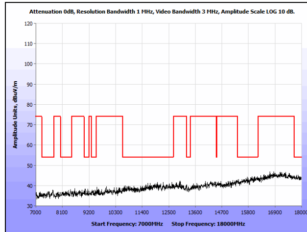
Plot 170. Radiated Spurious Emissions, 802.11a, Low Channel, 7 GHz – 18 GHz, Omni
