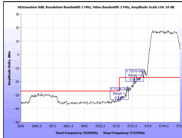
Plot 221. Radiated Band Edge, 802.11n 20 MHz, Low Channel, Omni Antenna (Band Edge @ 5715 & 5725 MHz)
