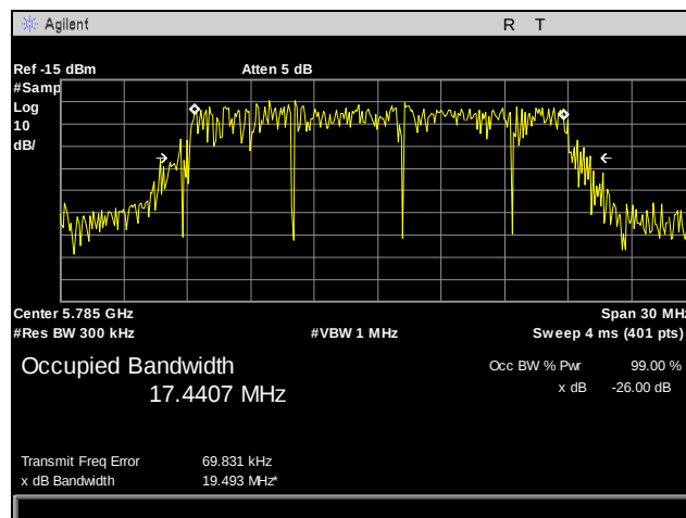
Plot 42. 99% Occupied Bandwidth, 802.11n 20 MHz, Port 2, Mid Channel
