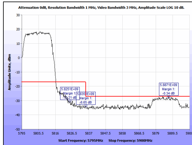
Plot 204. Radiated Band Edge, 802.11a, High Channel, 7 dBi Patch Antenna (Band Edge @ 5825 & 5835 MHz)
