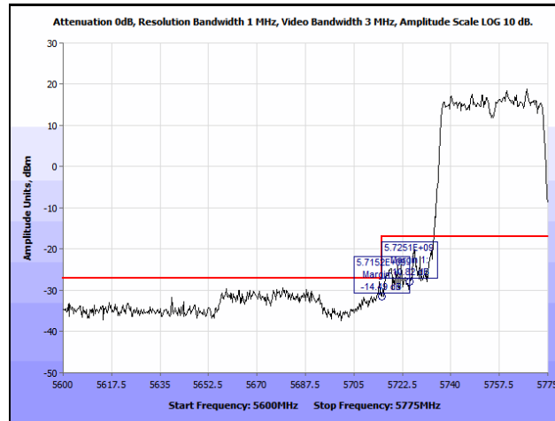
Plot 207. Radiated Band Edge, 802.11n 40 MHz, Low Channel, 7 dBi Patch Antenna (Band Edge @ 5715 & 5725 MHz)
