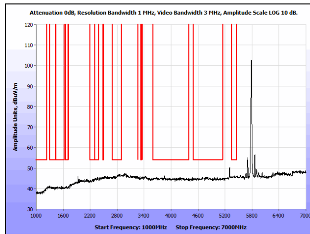
Plot 172. Radiated Spurious Emissions, 802.11a, Mid Channel, 1 GHz – 7 GHz, Average, Omni
