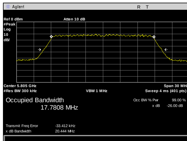
Plot 22. 26 dB Occupied Bandwidth, 802.11n 20 MHz, Port 2, High Channel
