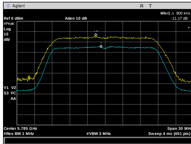
Plot 84. Peak Excursion Ratio, Mid Channel, 802.11n 20 MHz, Port 2
