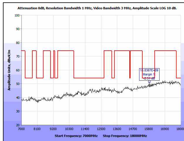
Plot 126. Radiated Spurious Emissions, 802.11n 40 MHz, High Channel, 7 GHz – 18 GHz, 7 dBi Patch
