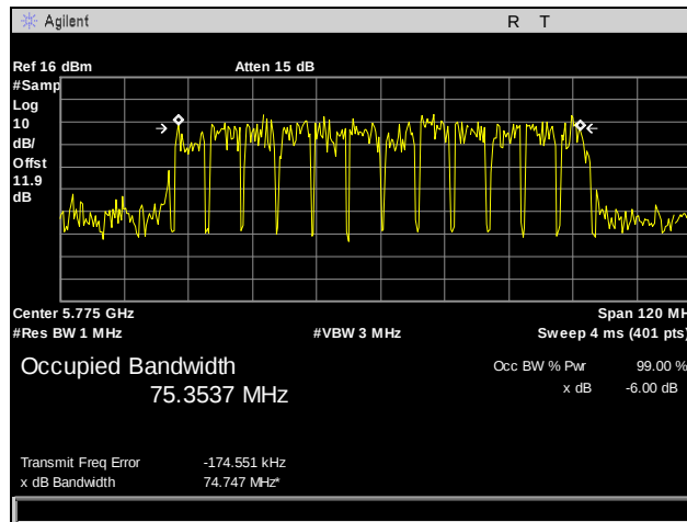
Plot 54. 99% Occupied Bandwidth, 802.11n 40 MHz, Port 2
