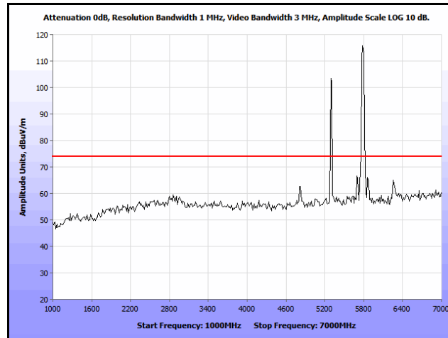
Plot 245. Co-location, Radiated Spurious Emissions, Omni, 802.11n 20 MHz, 5300 & 5785 MHz, 1 GHz – 7 GHz, Peak
