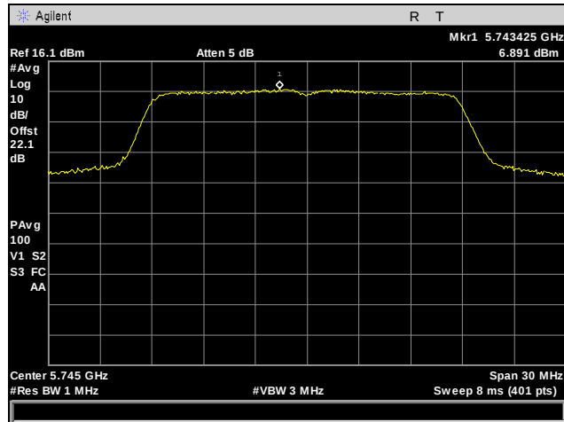
Plot 62. Power Spectral Density, Low Channel, 802.11n 20 MHz, Port 2
