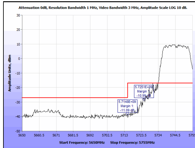
Plot 211. Radiated Band Edge, 802.11a, Low Channel, Ceiling Antenna (Band Edge @ 5715 & 5725 MHz)
