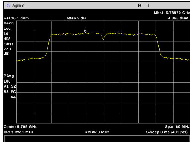
Plot 69. Power Spectral Density, High Channel, 802.11n 40 MHz, Port 1
