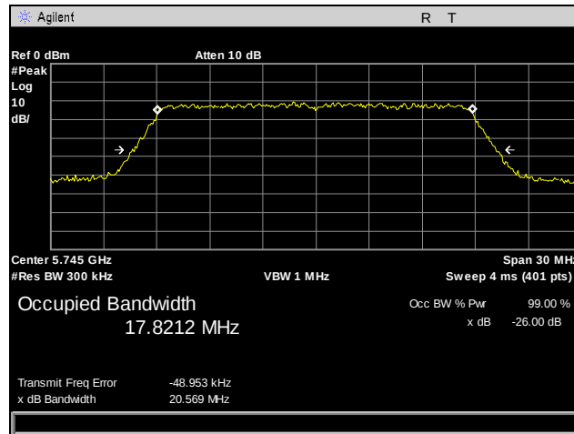
Plot 23. 26 dB Occupied Bandwidth, 802.11n 20 MHz, Port 3, Low Channel
