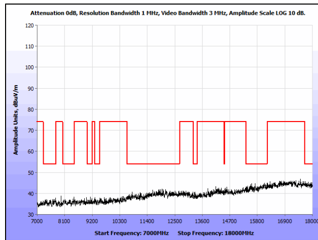
Plot 142. Radiated Spurious Emissions, 802.11a, High Channel, 7 GHz – 18 GHz, Ceiling
