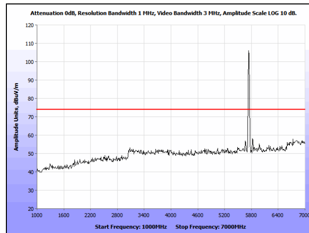
Plot 109. Radiated Spurious Emissions, 802.11n 20 MHz, Low Channel, 1 GHz – 7 GHz, Peak, 7 dBi Patch
