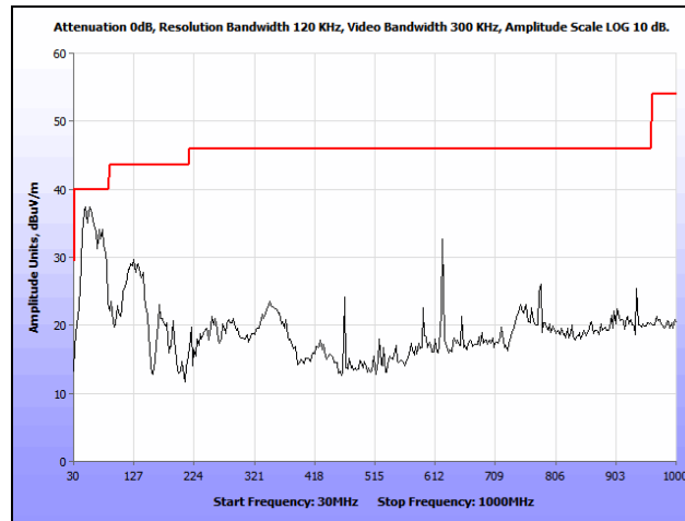
Plot 163. Radiated Spurious Emissions, 802.11n 80 MHz, Low Channel, 30 MHz – 1 GHz, Ceiling
