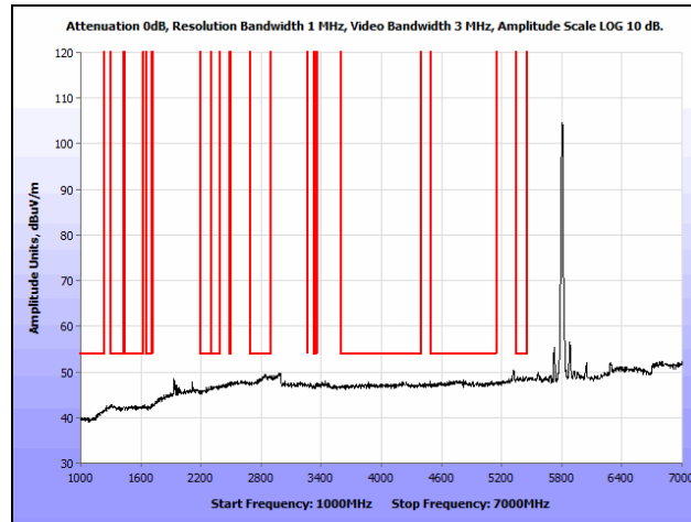
Plot 152. Radiated Spurious Emissions, 802.11n 20 MHz, High Channel, 1 GHz – 7 GHz, Average, Ceiling
