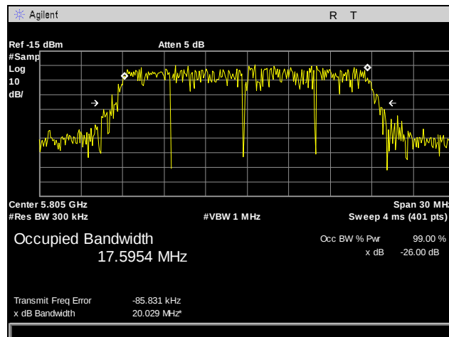
Plot 40. 99% Occupied Bandwidth, 802.11n 20 MHz, Port 1, High Channel
