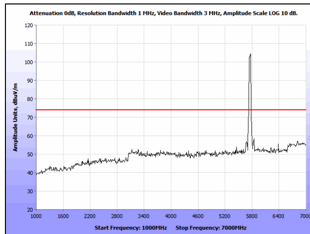
Plot 121. Radiated Spurious Emissions, 802.11n 40 MHz, Low Channel, 1 GHz – 7 GHz, Peak, 7 dBi Patch
