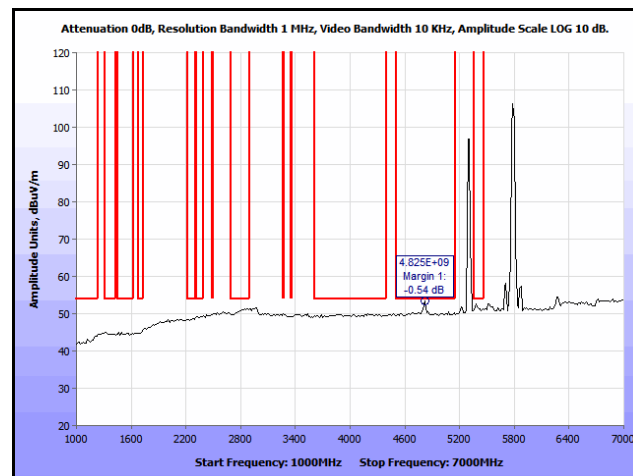
Plot 244. Co-location, Radiated Spurious Emissions, Omni, 802.11n 20 MHz, 5300 & 5785 MHz, 1 GHz – 7 GHz, Average
