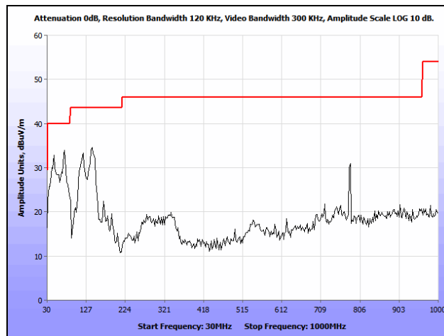
Plot 187. Radiated Spurious Emissions, 802.11n 20 MHz, High Channel, 30 MHz – 1 GHz, Omni
