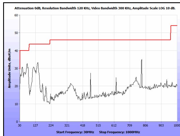
Plot 263. Co-location, Radiated Spurious Emissions, Patch, 802.11n 20 MHz, 2462 & 5785 MHz, 30 MHz – 1 GHz
