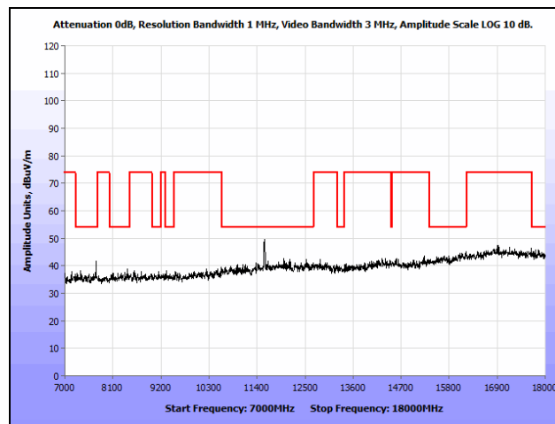
Plot 150. Radiated Spurious Emissions, 802.11n 20 MHz, Mid Channel, 7 GHz – 18 GHz, Ceiling
