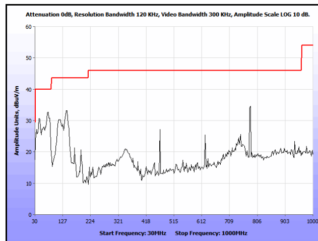
Plot 259. Co-location, Radiated Spurious Emissions, Patch, 802.11n 20 MHz, 2437 & 5785 MHz, 30 MHz – 1 GHz
