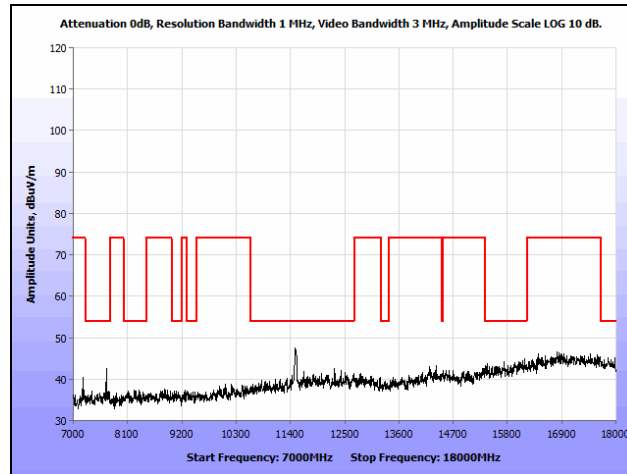
Plot 158. Radiated Spurious Emissions, 802.11n 40 MHz, Low Channel, 7 GHz – 18 GHz, Ceiling
