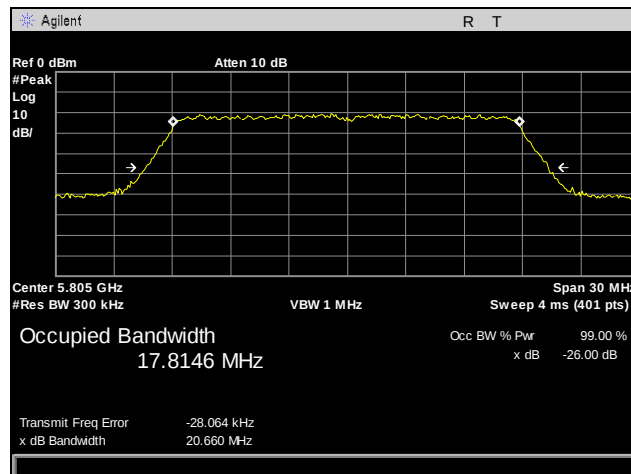
Plot 25. 26 dB Occupied Bandwidth, 802.11n 20 MHz, Port 3, High Channel
