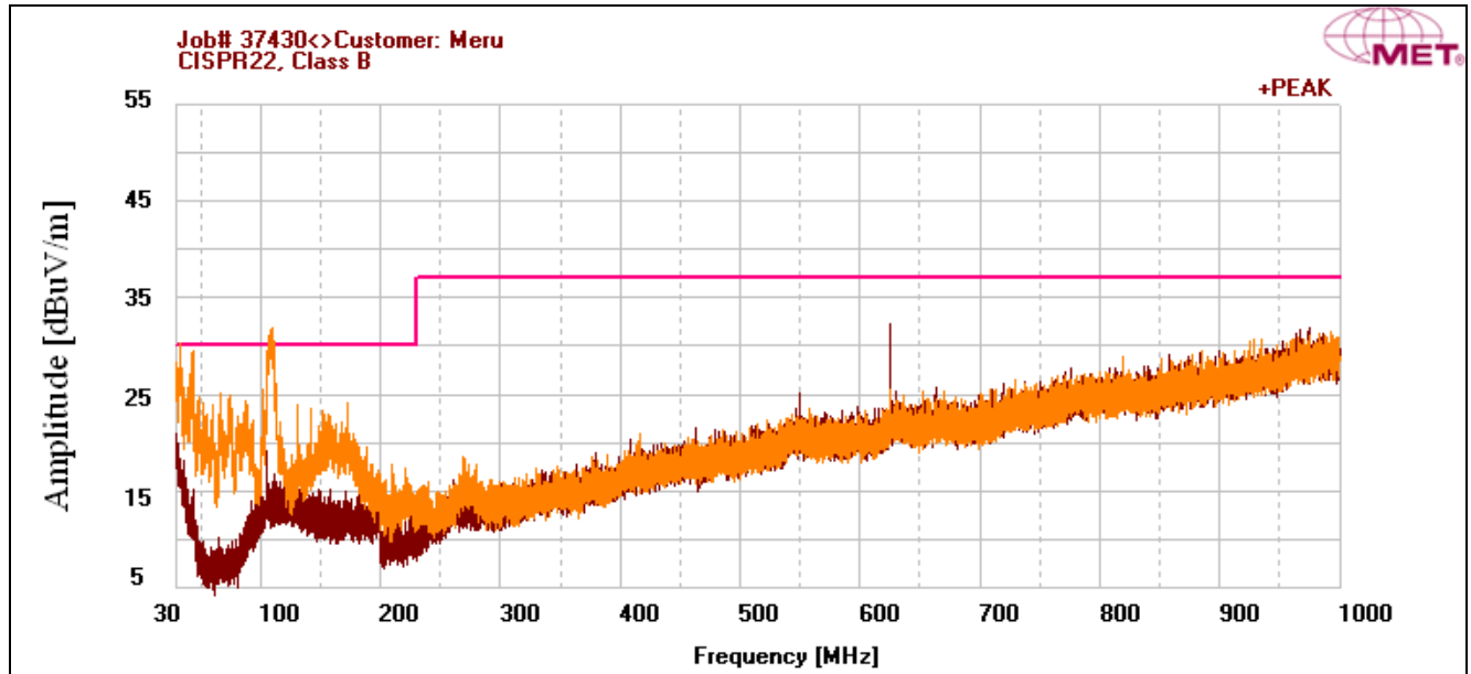
Plot 8. Radiated Emissions, 30 MHz - 1 GHz, CISPR Limits, PoE
