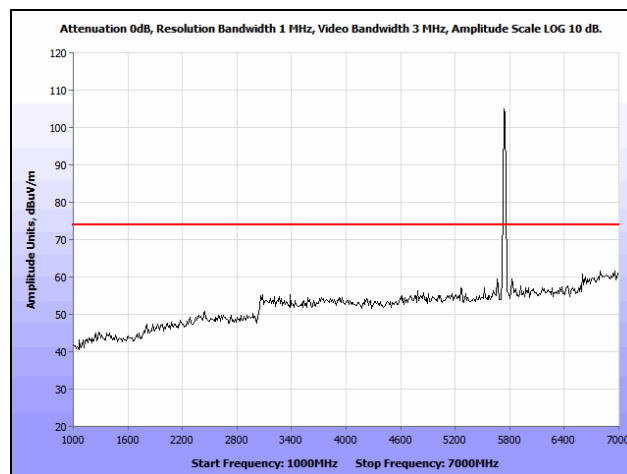
Plot 97. Radiated Spurious Emissions, 802.11a, Low Channel, 1 GHz – 7 GHz, Peak, 7 dBi Patch
