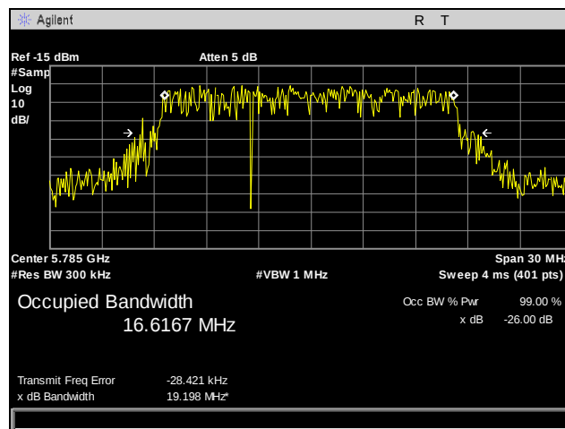
Plot 36. 99% Occupied Bandwidth, 802.11a, Port 1, Mid Channel
