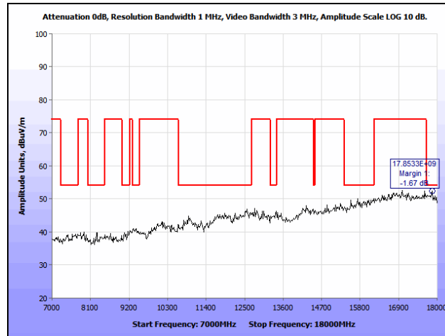
Plot 110. Radiated Spurious Emissions, 802.11n 20 MHz, Low Channel, 7 GHz – 18 GHz, 7 dBi Patch
