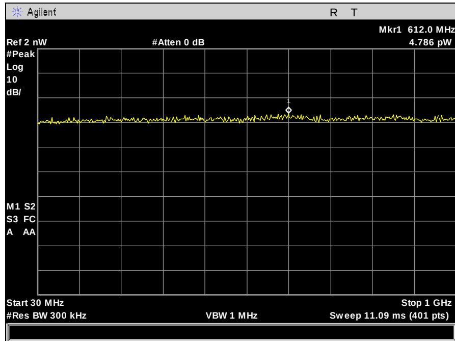
Plot 281. Receiver Spurious Emission, 30 MHz – 1 GHz, Port 2
