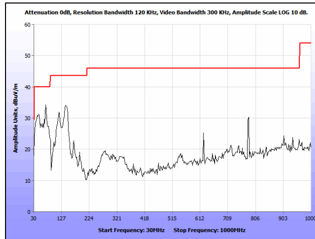
Plot 119. Radiated Spurious Emissions, 802.11n 40 MHz, Low Channel, 30 MHz – 1 GHz, 7 dBi Patch
