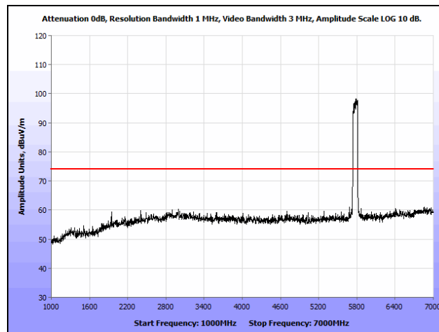
Plot 165. Radiated Spurious Emissions, 802.11n 80 MHz, Low Channel, 1 GHz – 7 GHz, Peak, Ceiling
