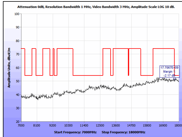
Plot 122. Radiated Spurious Emissions, 802.11n 40 MHz, Low Channel, 7 GHz – 18 GHz, 7 dBi Patch
