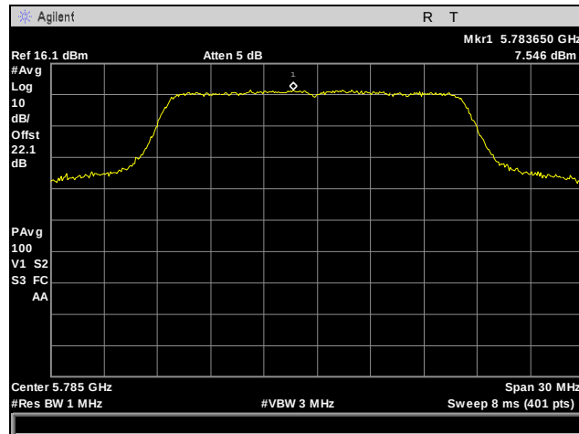
Plot 57. Power Spectral Density, Mid Channel, 802.11a
