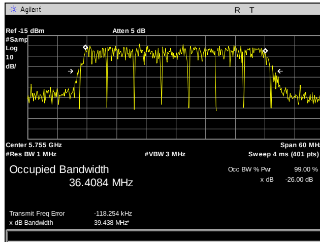
Plot 49. 99% Occupied Bandwidth, 802.11n 40 MHz, Port 2, Low Channel
