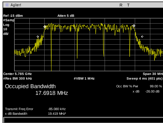
Plot 39. 99% Occupied Bandwidth, 802.11n 20 MHz, Port 1, Mid Channel
