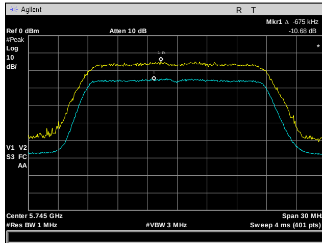
Plot 83. Peak Excursion Ratio, Low Channel, 802.11n 20 MHz, Port 2
