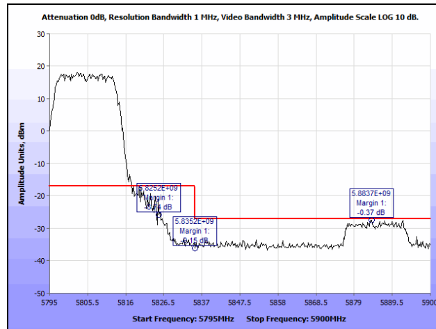
Plot 220. Radiated Band Edge, 802.11a, High Channel, Omni Antenna (Band Edge @ 5825 & 5835 MHz)
