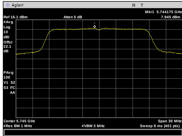
Plot 65. Power Spectral Density, Low Channel, 802.11n 20 MHz, Port 3
