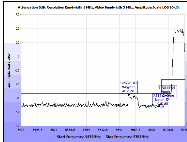
Plot 205. Radiated Band Edge, 802.11n 20 MHz, Low Channel, 7 dBi Patch Antenna (Band Edge @ 5715 & 5725 MHz)
