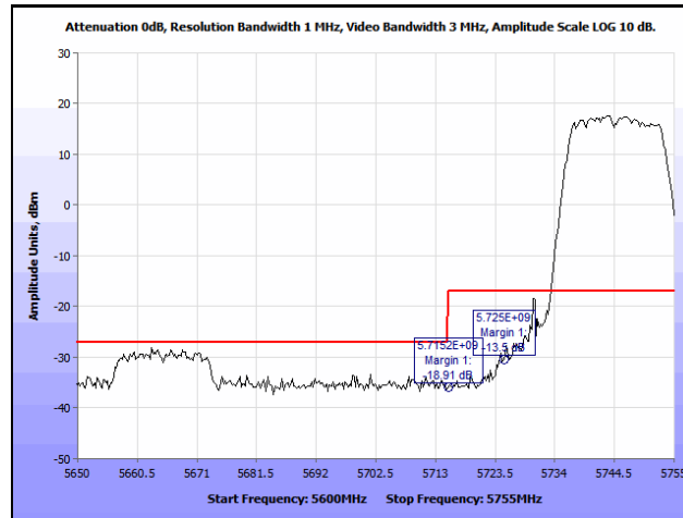
Plot 203. Radiated Band Edge, 802.11a, Low Channel, 7 dBi Patch Antenna (Band Edge @ 5715 & 5725 MHz)
