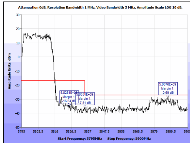
Plot 206. Radiated Band Edge, 802.11n 20 MHz, High Channel, 7 dBi Patch Antenna (Band Edge @ 5825 & 5835 MHz)
