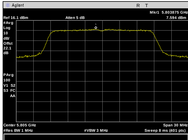
Plot 64. Power Spectral Density, High Channel, 802.11n 20 MHz, Port 2
