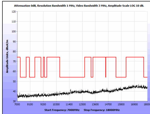
Plot 194. Radiated Spurious Emissions, 802.11n 40 MHz, Low Channel, 7 GHz – 18 GHz, Omni
