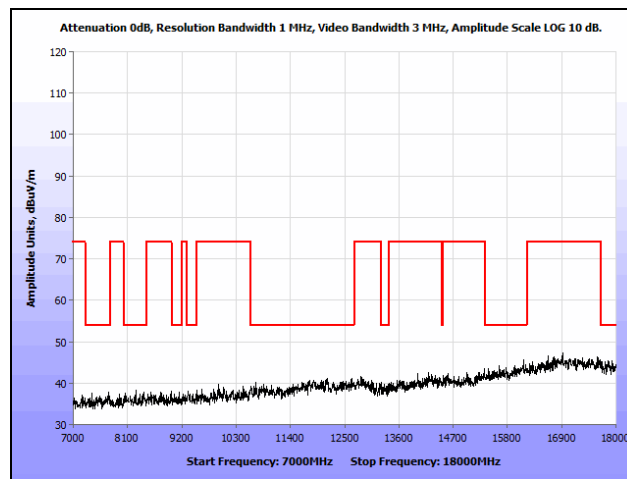
Plot 174. Radiated Spurious Emissions, 802.11a, Mid Channel, 7 GHz – 18 GHz, Omni
