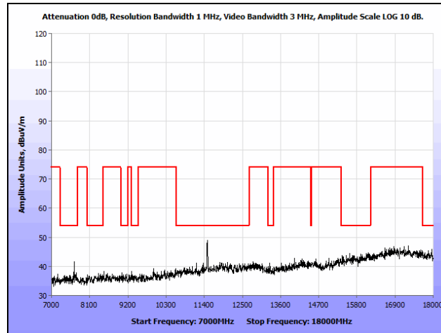
Plot 146. Radiated Spurious Emissions, 802.11n 20 MHz, Low Channel, 7 GHz – 18 GHz, Ceiling
