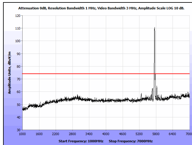
Plot 181. Radiated Spurious Emissions, 802.11n 20 MHz, Low Channel, 1 GHz – 7 GHz, Peak, Omni
