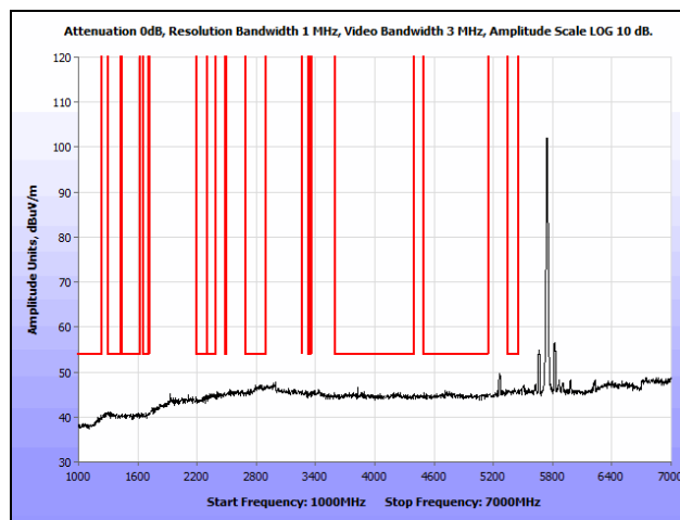
Plot 168. Radiated Spurious Emissions, 802.11a, Low Channel, 1 GHz – 7 GHz, Average, Omni
