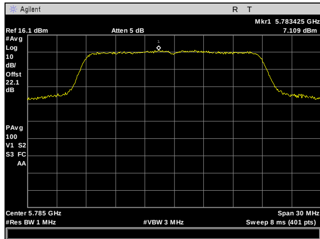
Plot 63. Power Spectral Density, Mid Channel, 802.11n 20 MHz, Port 2
