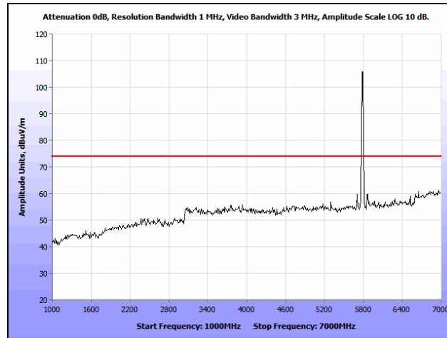
Plot 101. Radiated Spurious Emissions, 802.11a, Mid Channel, 1 GHz – 7 GHz, Peak, 7 dBi Patch
