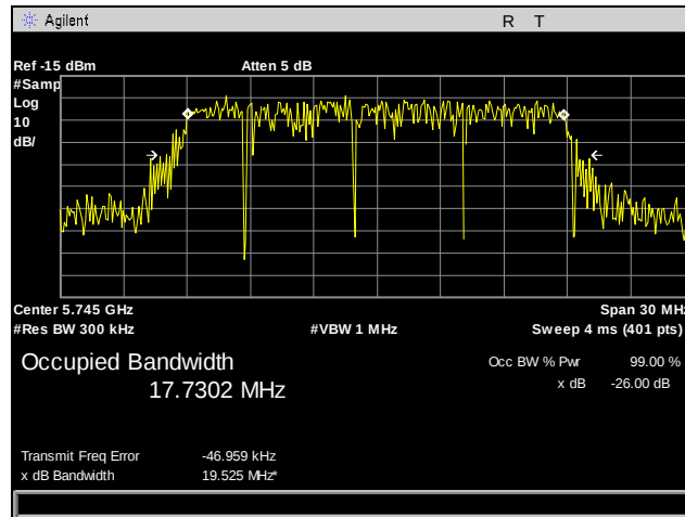
Plot 38. 99% Occupied Bandwidth, 802.11n 20 MHz, Port 1, Low Channel
