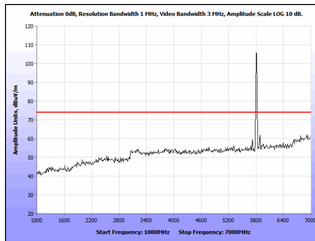
Plot 105. Radiated Spurious Emissions, 802.11a, High Channel, 1 GHz – 7 GHz, Peak, 7 dBi Patch
