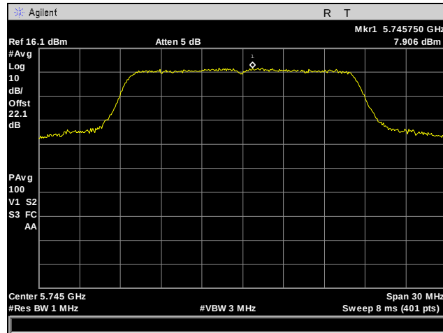
Plot 56. Power Spectral Density, Low Channel, 802.11a
