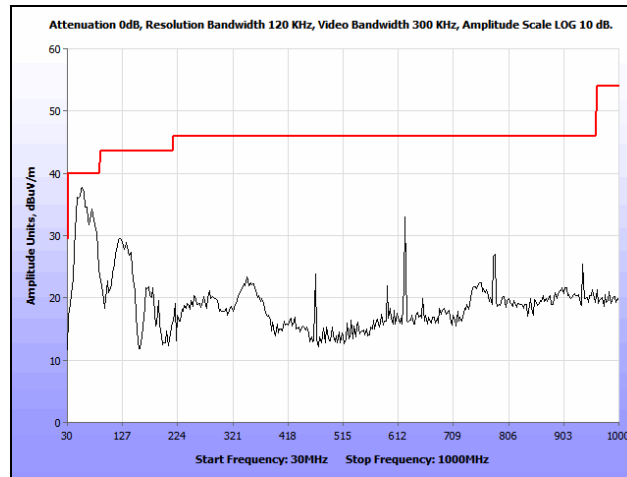
Plot 155. Radiated Spurious Emissions, 802.11n 40 MHz, Low Channel, 30 MHz – 1 GHz, Ceiling
