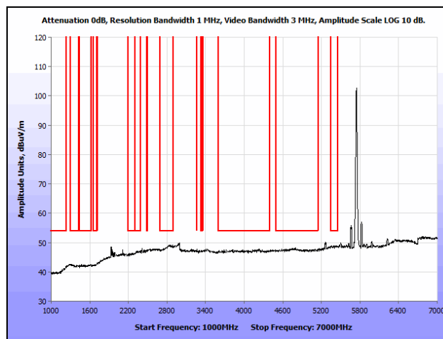
Plot 144. Radiated Spurious Emissions, 802.11n 20 MHz, Low Channel, 1 GHz – 7 GHz, Average, Ceiling
