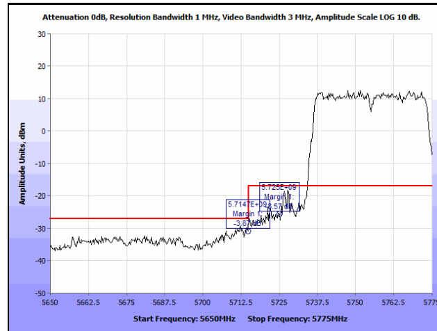
Plot 223. Radiated Band Edge, 802.11n 40 MHz, Low Channel, Omni Antenna (Band Edge @ 5715 & 5725 MHz)
