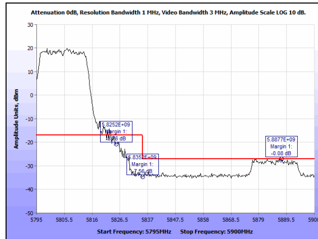
Plot 222. Radiated Band Edge, 802.11n 20 MHz, High Channel, Omni Antenna (Band Edge @ 5825 & 5835 MHz)
