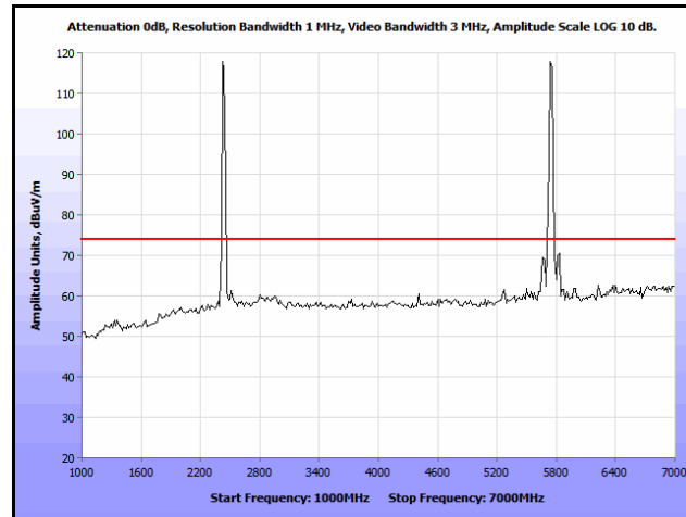
Plot 261. Co-location, Radiated Spurious Emissions, Patch, 802.11n 20 MHz, 2437 & 5785 MHz, 1 GHz – 7 GHz, Peak
