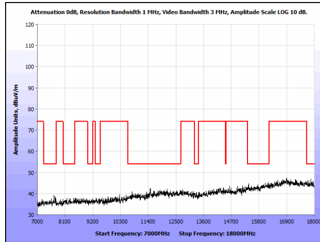
Plot 134. Radiated Spurious Emissions, 802.11a, Low Channel, 7 GHz – 18 GHz, Ceiling
