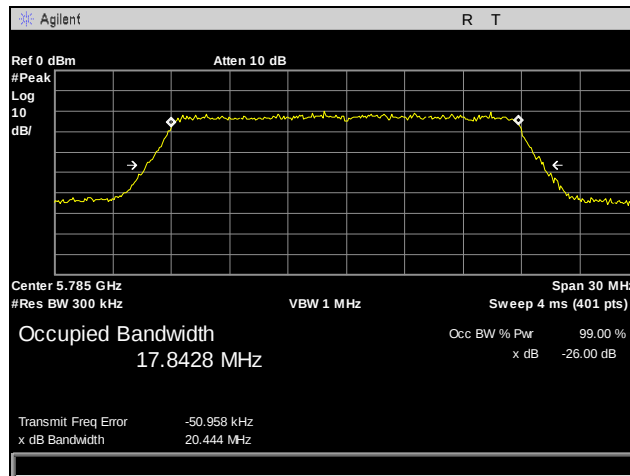
Plot 15. 26 dB Occupied Bandwidth, 802.11a, Port 1, Mid Channel
