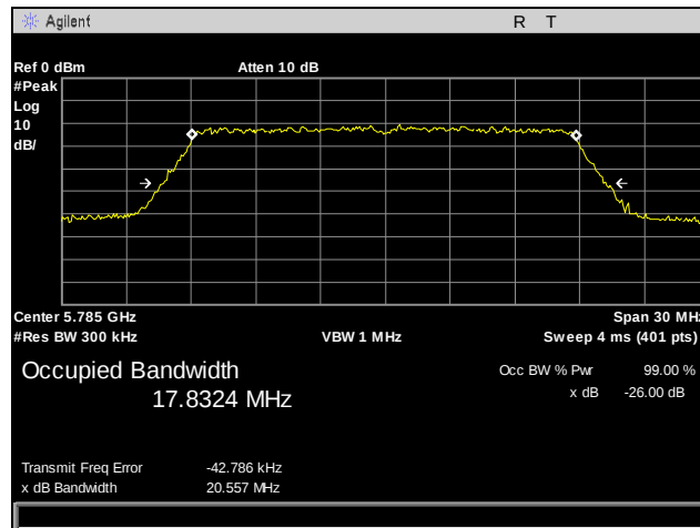
Plot 24. 26 dB Occupied Bandwidth, 802.11n 20 MHz, Port 3, Mid Channel
