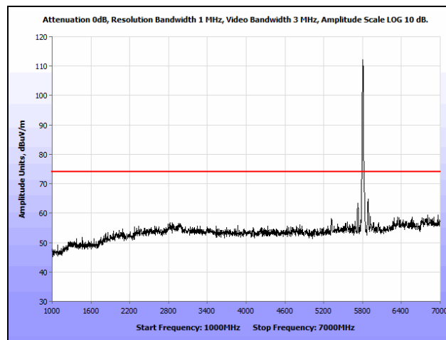
Plot 189. Radiated Spurious Emissions, 802.11n 20 MHz, High Channel, 1 GHz – 7 GHz, Peak, Omni
