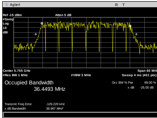
Plot 47. 99% Occupied Bandwidth, 802.11n 40 MHz, Port 1, Low Channel
