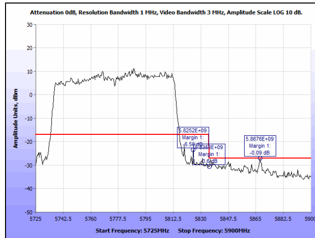
Plot 218. Radiated Band Edge, 802.11n 80 MHz, Ceiling Antenna (Band Edge @ 5825 & 5835 MHz)
