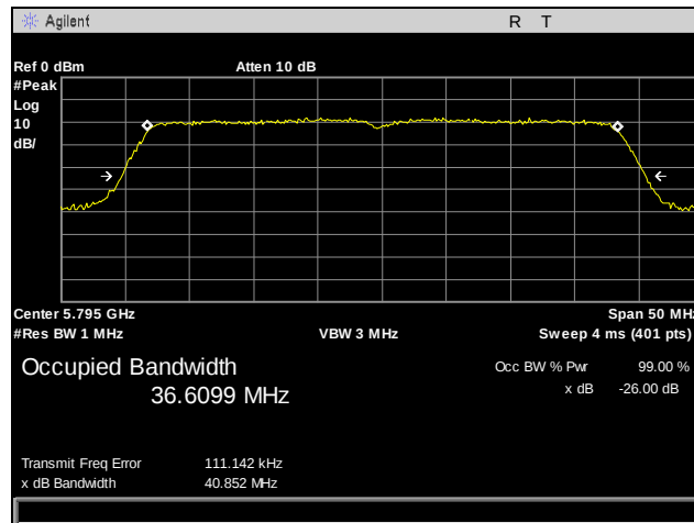
Plot 29. 26 dB Occupied Bandwidth, 802.11n 40 MHz, Port 2, High Channel
