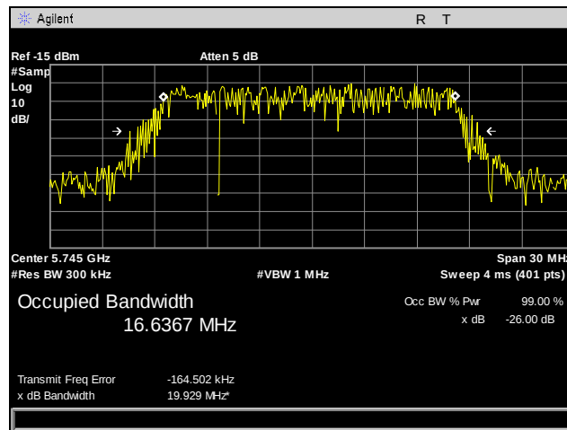
Plot 35. 99% Occupied Bandwidth, 802.11a, Port 1, Low Channel
