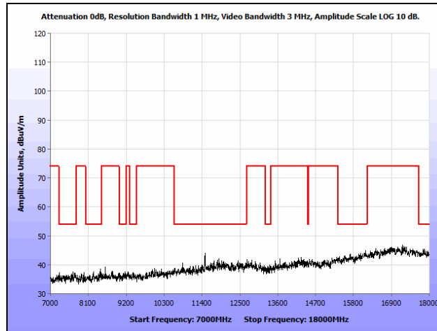
Plot 182. Radiated Spurious Emissions, 802.11n 20 MHz, Low Channel, 7 GHz – 18 GHz, Omni
