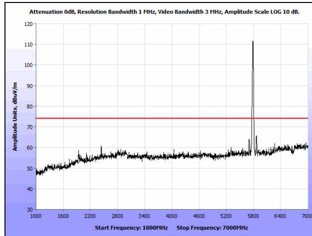
Plot 137. Radiated Spurious Emissions, 802.11a, Mid Channel, 1 GHz – 7 GHz, Peak, Ceiling
