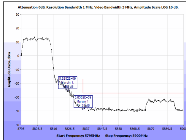
Plot 214. Radiated Band Edge, 802.11n 20 MHz, High Channel, Ceiling Antenna (Band Edge @ 5825 & 5835 MHz)
