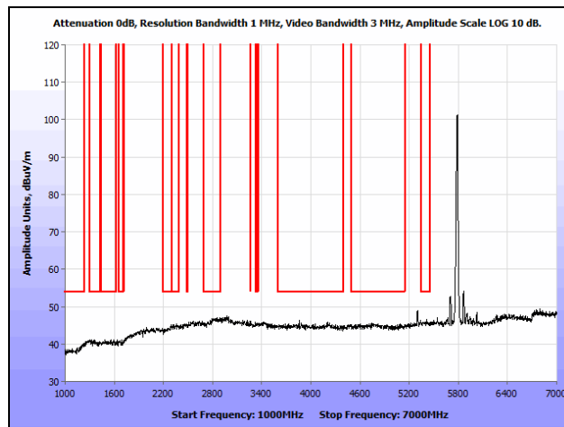
Plot 184. Radiated Spurious Emissions, 802.11n 20 MHz, Mid Channel, 1 GHz – 7 GHz, Average, Omni
