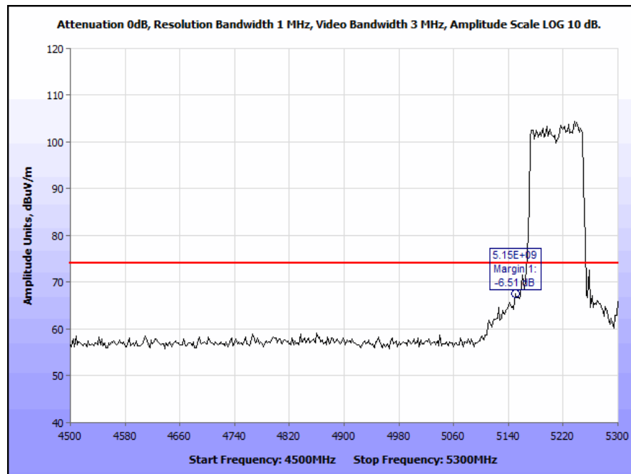
Plot 253. Restricted Band Edge, Omni Antenna, 802.11n 80 MHz, 5210 MHz @ 5150 MHz Edge, Peak
