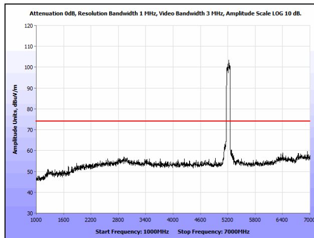
Plot 204. Radiated Spurious Emissions, 802.11n 80 MHz, Low Channel, 1 GHz – 7 GHz, Peak, Omni
