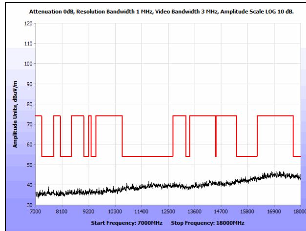
Plot 133. Radiated Spurious Emissions, 802.11n 80 MHz, 7 GHz – 18 GHz, 7 dBi
