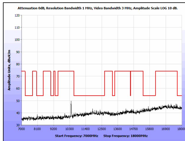
Plot 153. Radiated Spurious Emissions, 802.11n 20 MHz, Mid Channel, 7 GHz – 18 GHz, Ceiling
