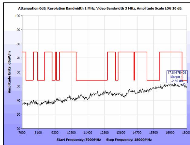
Plot 105. Radiated Spurious Emissions, 802.11a, Mid Channel, 7 GHz – 18 GHz, 7 dBi Patch
