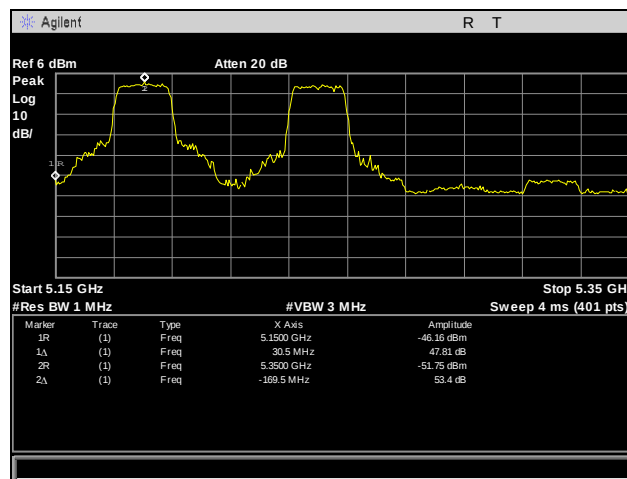
Plot 295. Frequency Stability, 5150 – 5250 MHz, -20°C, 120 V
