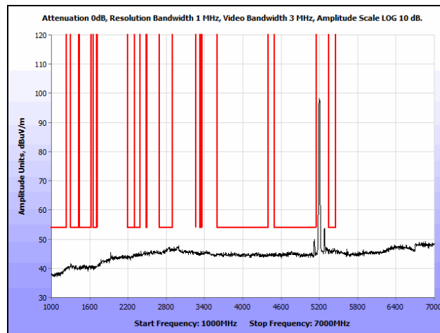
Plot 175. Radiated Spurious Emissions, 802.11a, Mid Channel, 1 GHz – 7 GHz, Average, Omni
