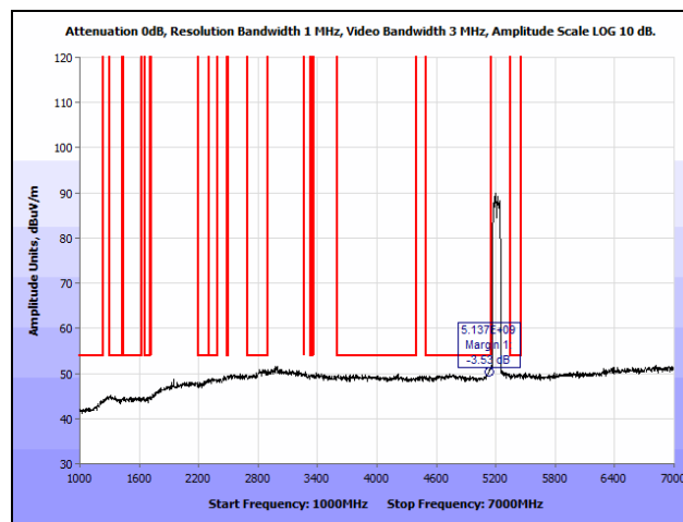
Plot 131. Radiated Spurious Emissions, 802.11n 80 MHz, 1 GHz – 7 GHz, Average, 7 dBi Patch
