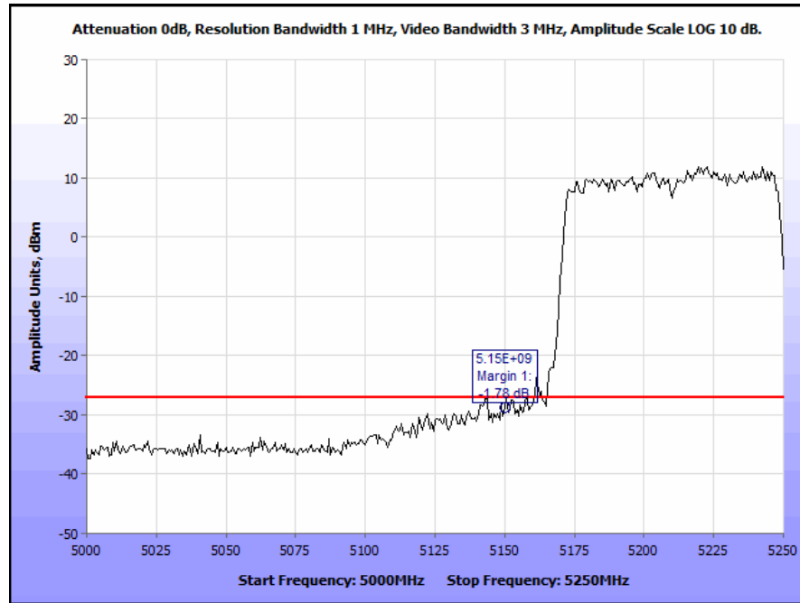
Plot 228. Radiated Band Edge 802.11n 80 MHz, Omni Antenna (Band Edge @ 5150 MHz)
