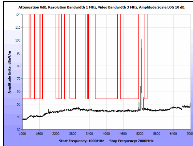
Plot 179. Radiated Spurious Emissions, 802.11a, High Channel, 1 GHz – 7 GHz, Average, Omni
