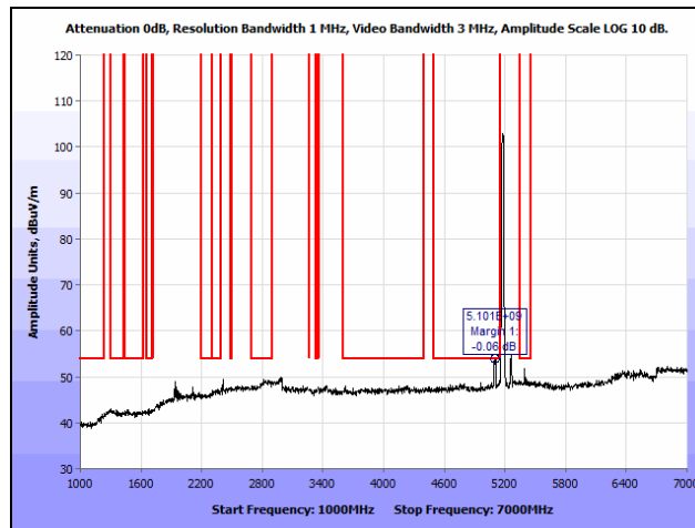
Plot 147. Radiated Spurious Emissions, 802.11n 20 MHz, Low Channel, 1 GHz – 7 GHz, Average, Ceiling
