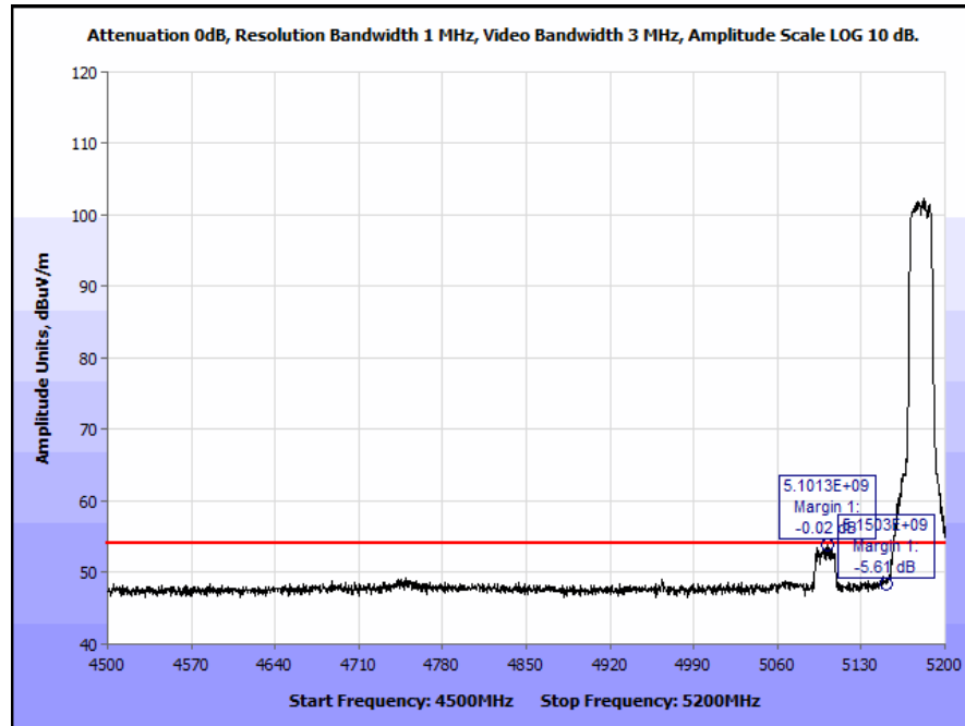
Plot 240. Restricted Band Edge, Ceiling Antenna, 802.11n 20 MHz, 5180 MHz High @ 5150 MHz Edge, Average
