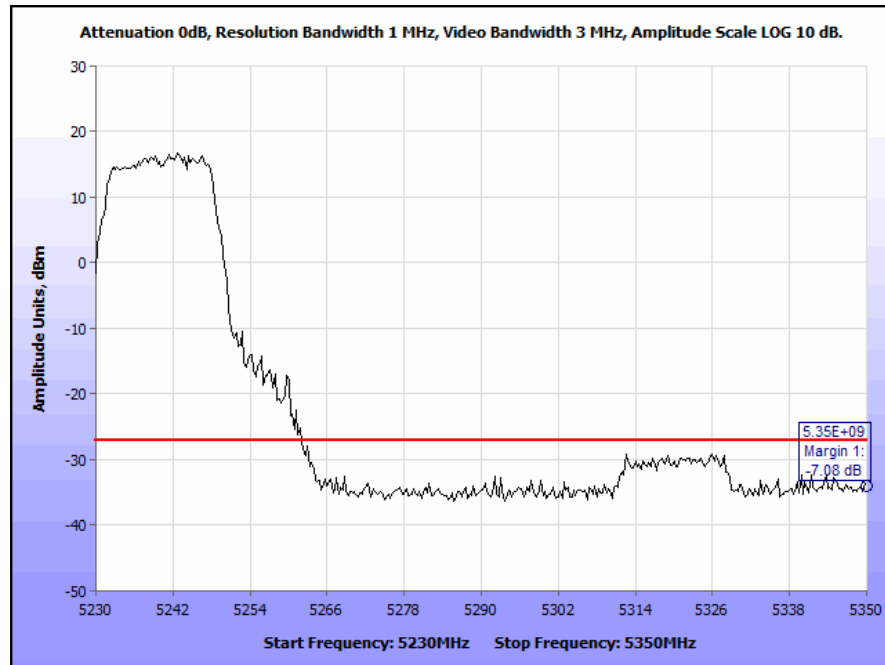
Plot 223. Radiated Band Edge 802.11a, High Channel, Omni Antenna (Band Edge @ 5350 MHz)
