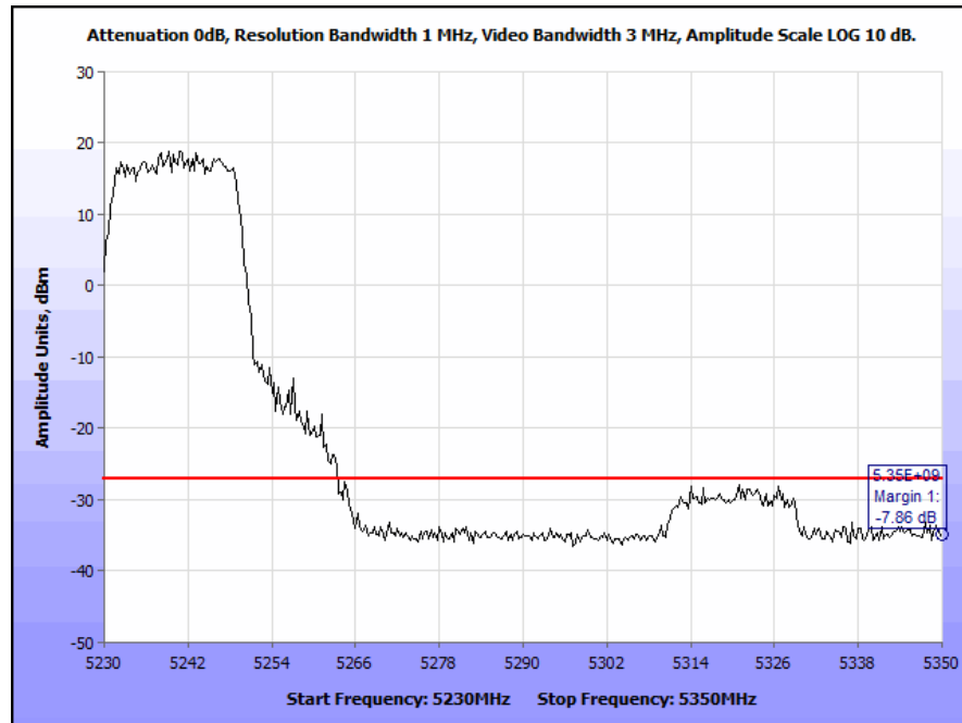
Plot 225. Radiated Band Edge 802.11n 20 MHz, High Channel, Omni Antenna (Band Edge @ 5350 MHz)
