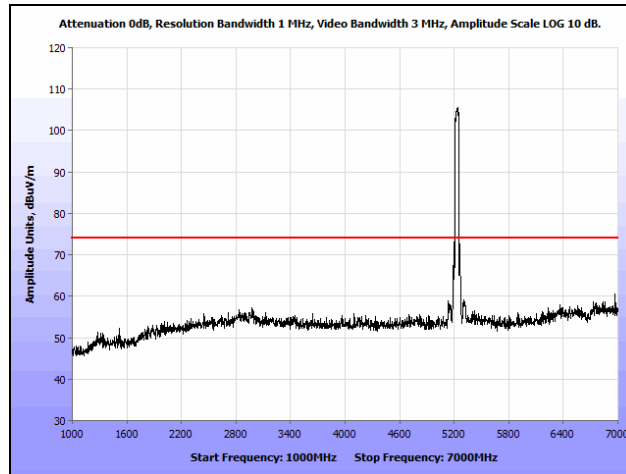
Plot 200. Radiated Spurious Emissions, 802.11n 40 MHz, High Channel, 1 GHz – 7 GHz, Peak, Omni
