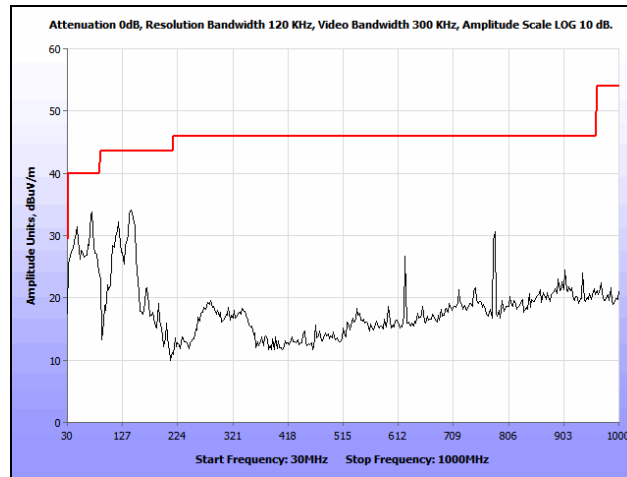
Plot 110. Radiated Spurious Emissions, 802.11n 20 MHz, Low Channel, 30 MHz – 1 GHz, 7 dBi Patch
