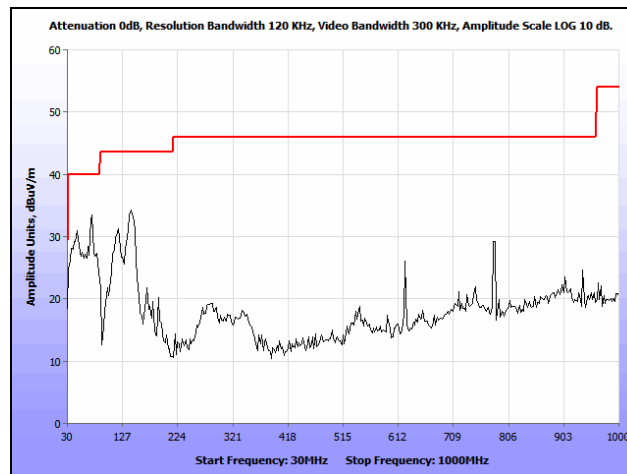
Plot 118. Radiated Spurious Emissions, 802.11n 20 MHz, High Channel, 30 MHz – 1 GHz, 7 dBi Patch
