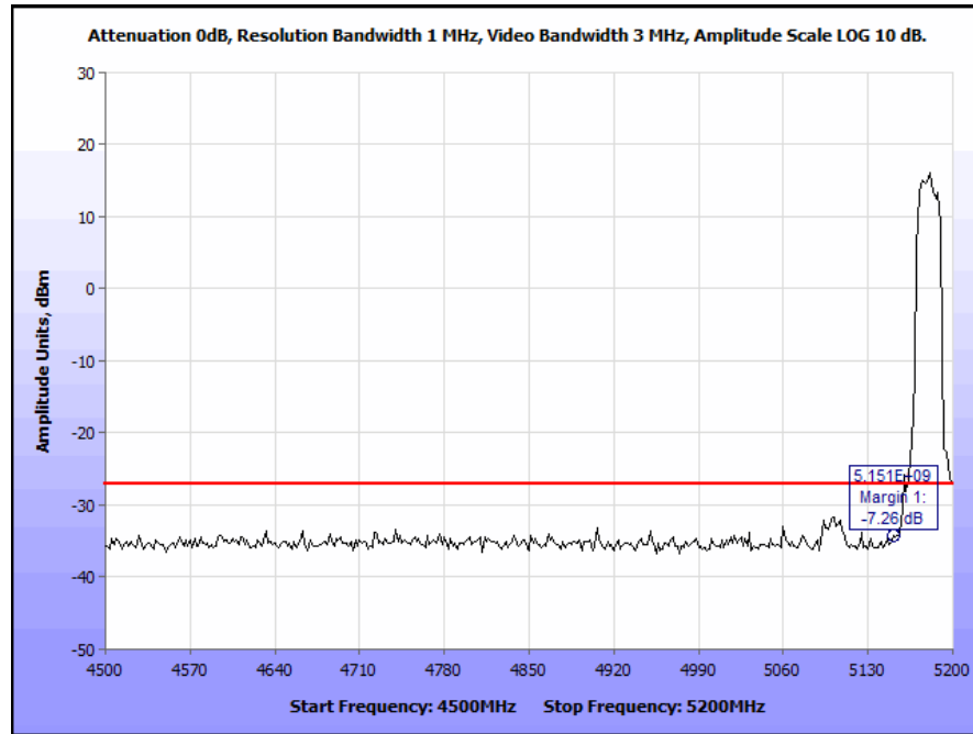
Plot 224. Radiated Band Edge 802.11n 20 MHz, Low Channel, Omni Antenna (Band Edge @ 5150 MHz)
