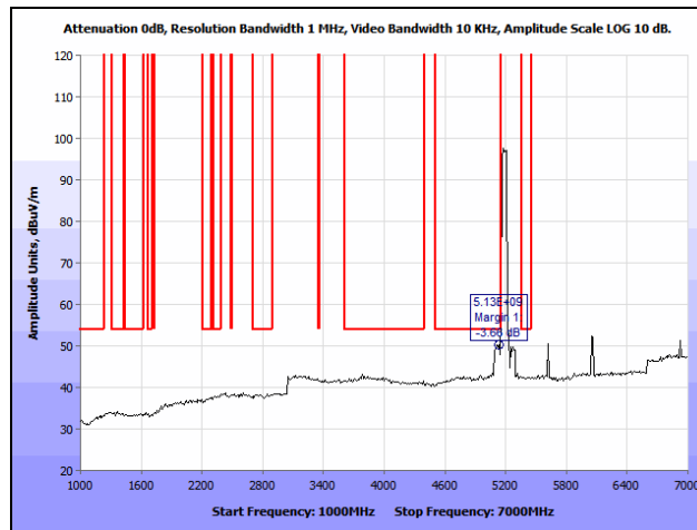
Plot 123. Radiated Spurious Emissions, 802.11n 40 MHz, Low Channel, 1 GHz – 7 GHz, Average, 7 dBi Patch
