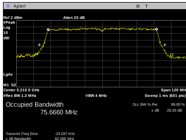
Plot 34. 26 dB Occupied Bandwidth, 802.11n 80 MHz, Port 3
