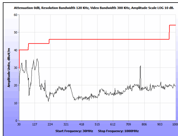
Plot 198. Radiated Spurious Emissions, 802.11n 40 MHz, High Channel, 30 MHz – 1 GHz, Omni
