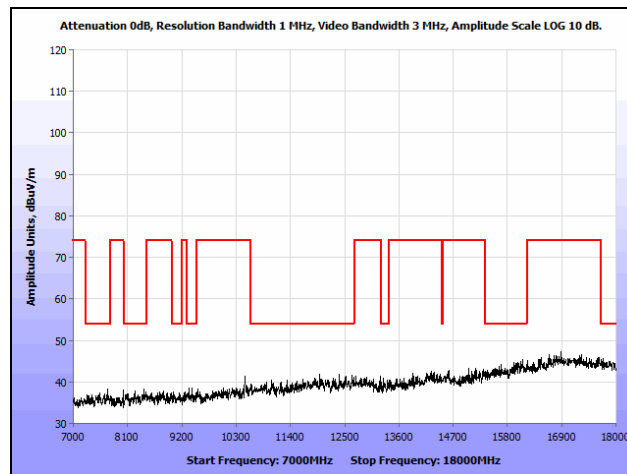
Plot 181. Radiated Spurious Emissions, 802.11a, High Channel, 7 GHz – 18 GHz, Omni
