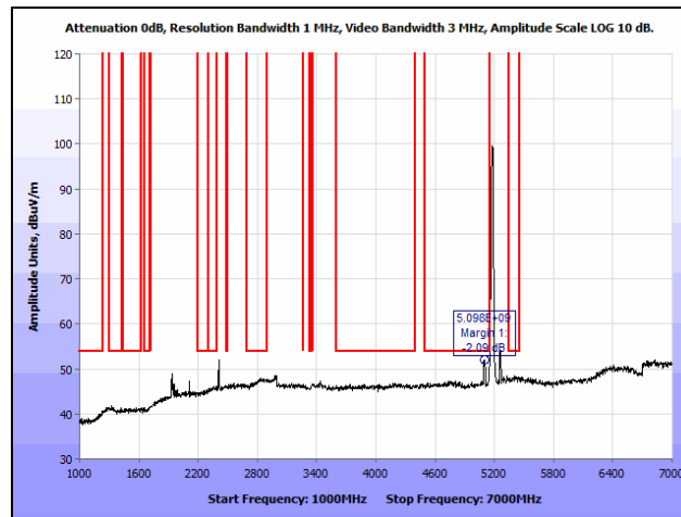
Plot 135. Radiated Spurious Emissions, 802.11a, Low Channel, 1 GHz – 7 GHz, Average, Ceiling
