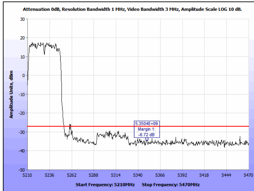
Plot 211. Radiated Band Edge 802.11n 40 MHz, High Channel, 7 dBi Patch Antenna (Band Edge @ 5350 MHz)
