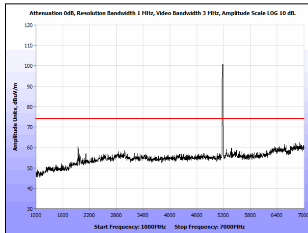
Plot 136. Radiated Spurious Emissions, 802.11a, Low Channel, 1 GHz – 7 GHz, Peak, Ceiling
