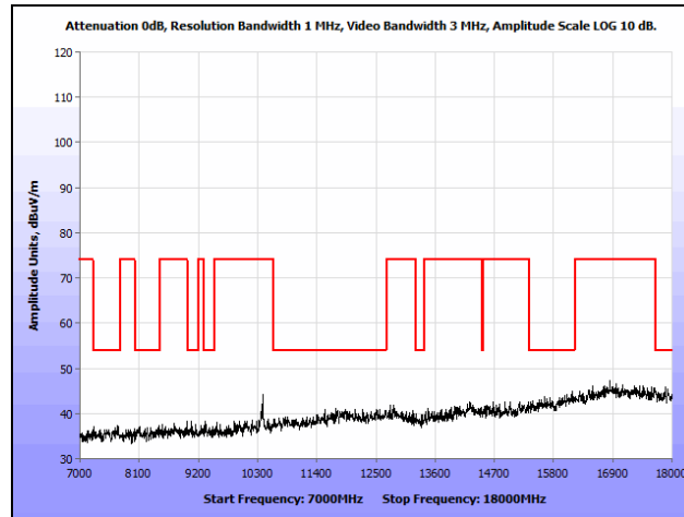
Plot 197. Radiated Spurious Emissions, 802.11n 40 MHz, Low Channel, 7 GHz – 18 GHz, Omni
