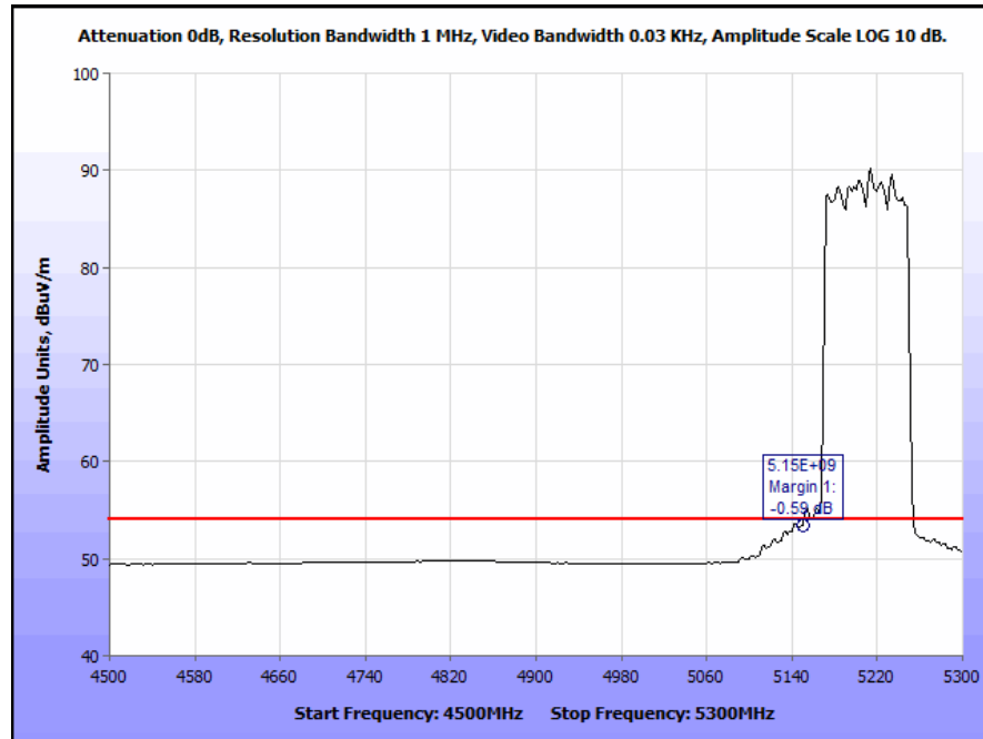
Plot 236. Restricted Band Edge, Patch Antenna, 802.11n 80 MHz, 5210 MHz @ 5150 MHz Edge, Average
