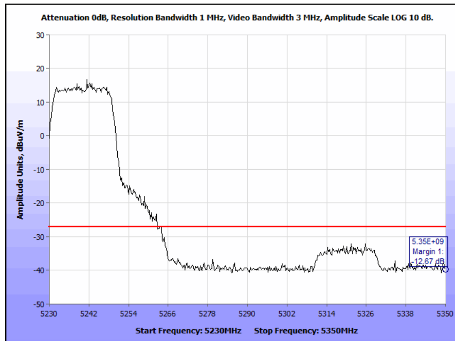
Plot 217. Radiated Band Edge 802.11n 20 MHz, High Channel, Ceiling Antenna (Band Edge @ 5350 MHz)
