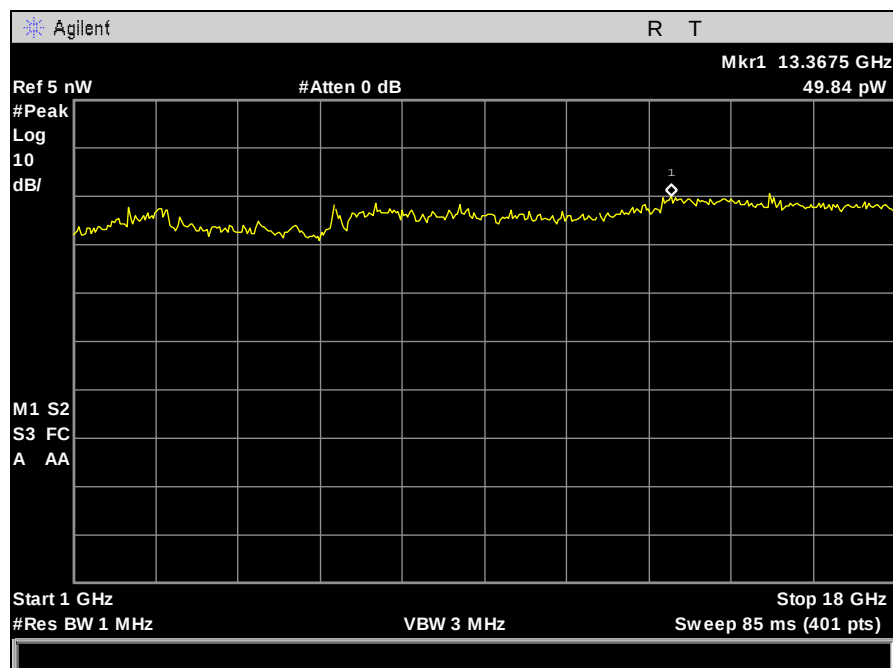
Plot 311. Receiver Spurious Emission, 1 GHz – 18 GHz, Port 3
