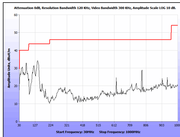
Plot 114. Radiated Spurious Emissions, 802.11n 20 MHz, Mid Channel, 30 MHz – 1 GHz, 7 dBi Patch
