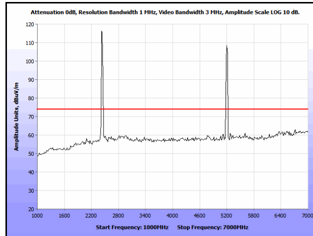
Plot 288. Co-location, Radiated Spurious Emissions, Patch, 802.11n 20 MHz, 2437 & 5200 MHz, 1 GHz – 7 GHz, Peak
