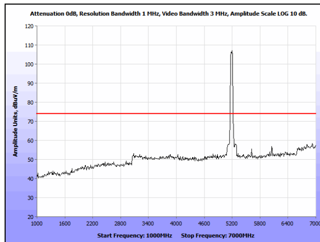
Plot 124. Radiated Spurious Emissions, 802.11n 40 MHz, Low Channel, 1 GHz – 7 GHz, Peak, 7 dBi Patch
