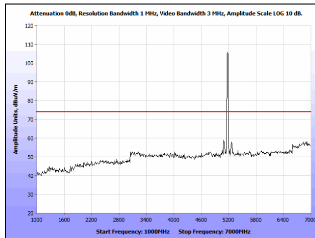
Plot 112. Radiated Spurious Emissions, 802.11n 20 MHz, Low Channel, 1 GHz – 7 GHz, Peak, 7 dBi Patch
