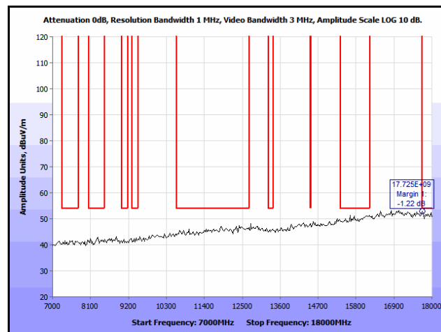
Plot 293. Co-location, Radiated Spurious Emissions, Patch, 802.11n 20 MHz, 2462 & 5200 MHz, 7 GHz – 18 GHz, Peak
