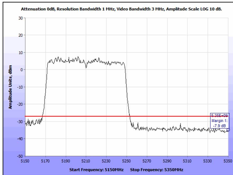
Plot 221. Radiated Band Edge 802.11n 80 MHz, Ceiling Antenna (Band Edge @ 5350 MHz)
