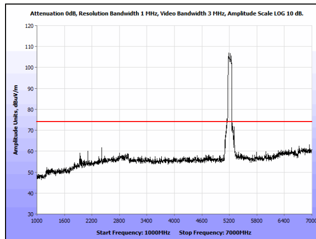
Plot 168. Radiated Spurious Emissions, 802.11n 80 MHz, Low Channel, 1 GHz – 7 GHz, Peak, Ceiling
