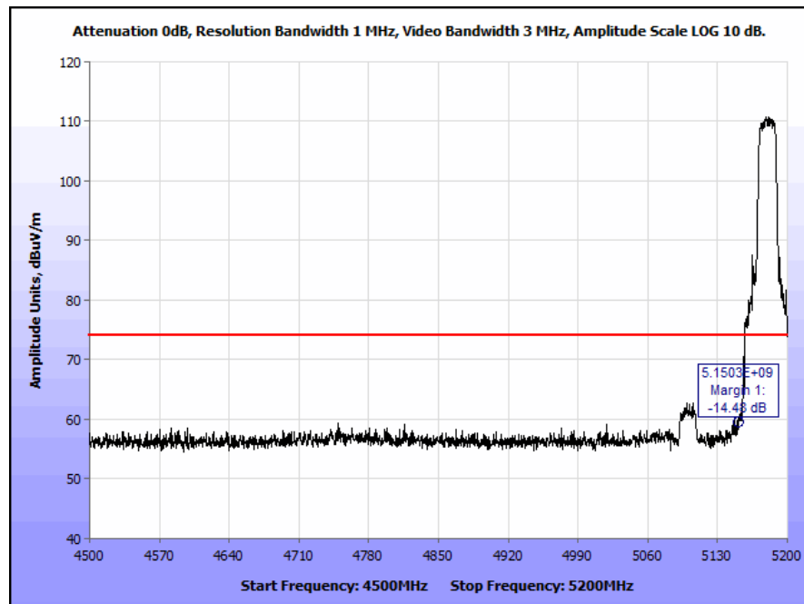
Plot 239. Restricted Band Edge, Ceiling Antenna, 802.11a 20 MHz, 5180 MHz, High @ 5150 MHz Edge, Peak
