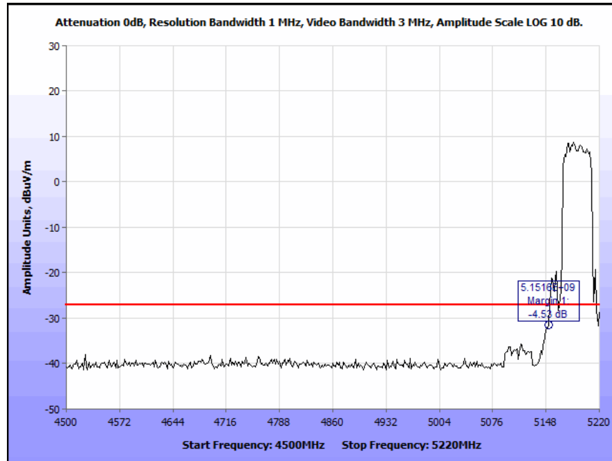
Plot 218. Radiated Band Edge 802.11n 40 MHz, Low Channel, Ceiling Antenna (Band Edge @ 5150 MHz)
