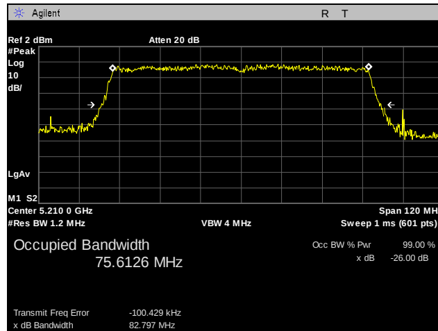
Plot 32. 26 dB Occupied Bandwidth, 802.11n 80 MHz, Port 1
