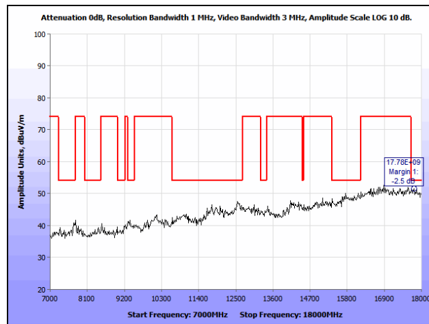
Plot 109. Radiated Spurious Emissions, 802.11a, High Channel, 7 GHz – 18 GHz, 7 dBi Patch
