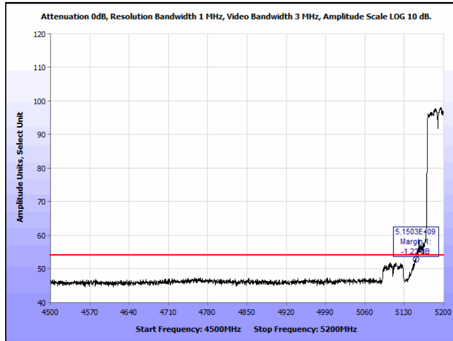
Plot 250. Restricted Band Edge, Omni Antenna, 802.11n 40 MHz, 5190 MHz Low @ 5150 MHz Edge, Average
