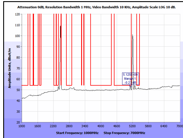
Plot 291. Co-location, Radiated Spurious Emissions, Patch, 802.11n 20 MHz, 2462 & 5200 MHz, 1 GHz – 7 GHz, Average
