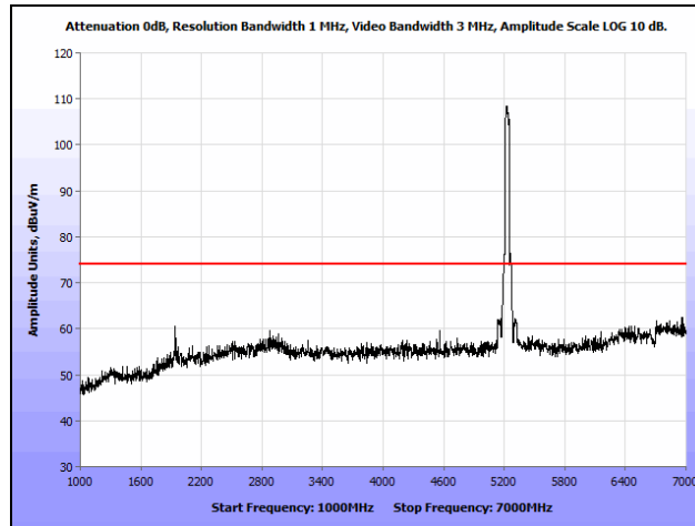
Plot 164. Radiated Spurious Emissions, 802.11n 40 MHz, High Channel, 1 GHz – 7 GHz, Peak, Ceiling
