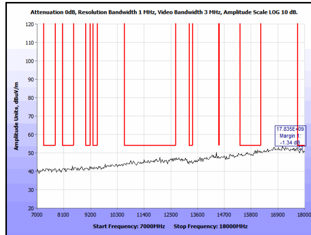
Plot 285. Co-location, Radiated Spurious Emissions, Patch, 802.11n 20 MHz, 2412 & 5200 MHz, 7 GHz – 18 GHz, Peak
