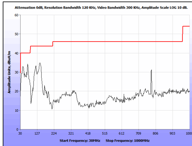
Plot 202. Radiated Spurious Emissions, 802.11n 80 MHz, Low Channel, 30 MHz – 1 GHz, Omni
