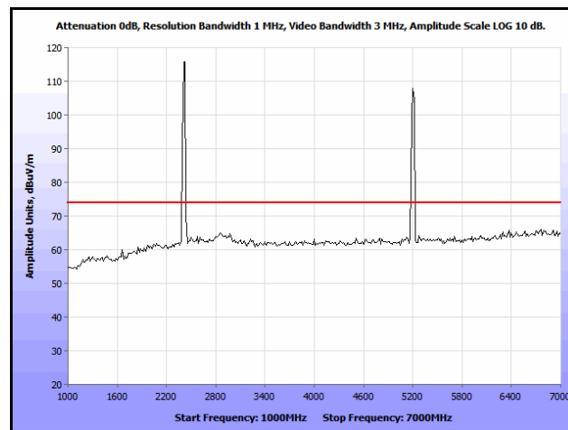
Plot 284. Co-location, Radiated Spurious Emissions, Patch, 802.11n 20 MHz, 2412 & 5200 MHz, 1 GHz – 7 GHz, Peak
