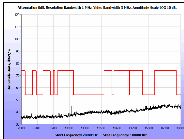
Plot 145. Radiated Spurious Emissions, 802.11a, High Channel, 7 GHz – 18 GHz, Ceiling
