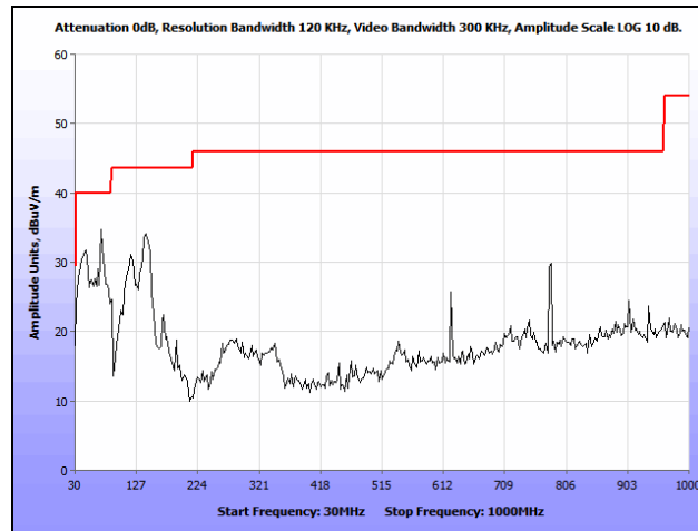
Plot 130. Radiated Spurious Emissions, 802.11n 80 MHz, 30 MHz – 1 GHz, 7 dBi Patch
