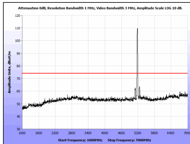
Plot 184. Radiated Spurious Emissions, 802.11n 20 MHz, Low Channel, 1 GHz – 7 GHz, Peak, Omni
