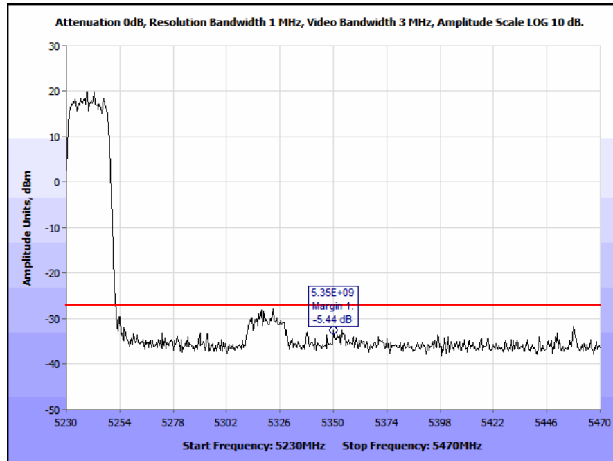
Plot 209. Radiated Band Edge 802.11n 20 MHz, High Channel, 7 dBi Patch Antenna (Band Edge @ 5350 MHz)
