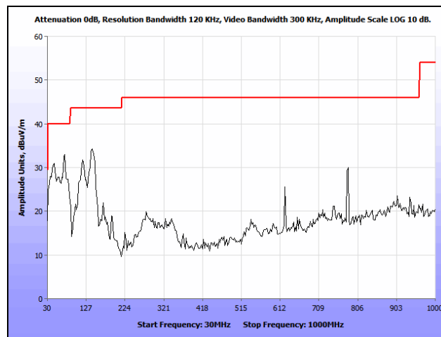
Plot 126. Radiated Spurious Emissions, 802.11n 40 MHz, High Channel, 30 MHz – 1 GHz, 7 dBi Patch
