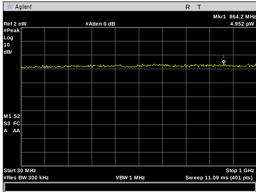
Plot 306. Receiver Spurious Emission, 30 MHz – 1 GHz, Port 1
