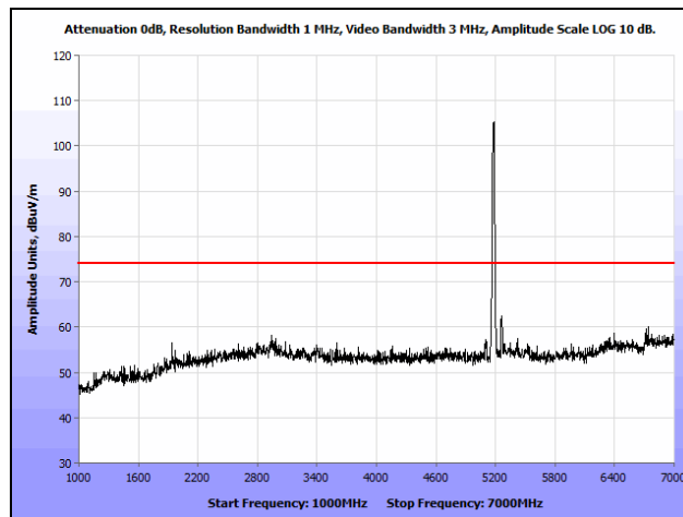
Plot 172. Radiated Spurious Emissions, 802.11a, Low Channel, 1 GHz – 7 GHz, Peak, Omni
