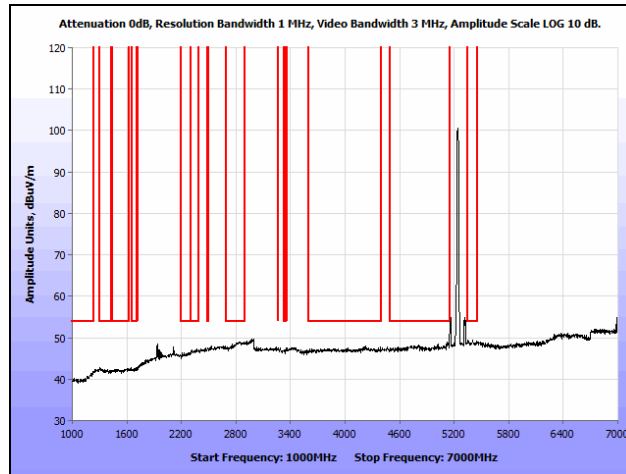
Plot 155. Radiated Spurious Emissions, 802.11n 20 MHz, High Channel, 1 GHz – 7 GHz, Average, Ceiling
