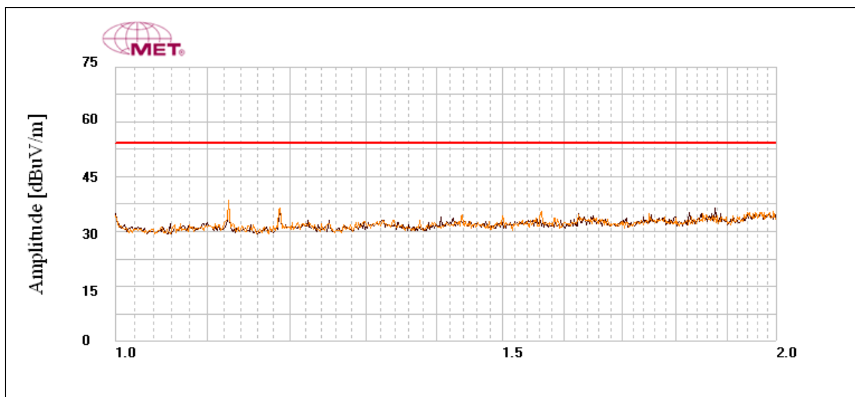
Plot 9. Radiated Emissions, Above 1 GHz
