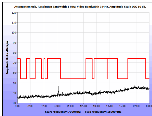
Plot 177. Radiated Spurious Emissions, 802.11a, Mid Channel, 7 GHz – 18 GHz, Omni
