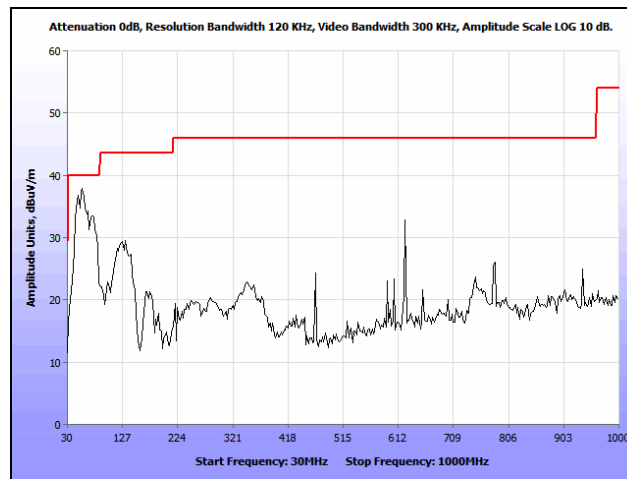
Plot 166. Radiated Spurious Emissions, 802.11n 80 MHz, Low Channel, 30 MHz – 1 GHz, Ceiling
