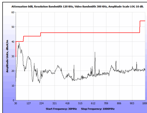
Plot 150. Radiated Spurious Emissions, 802.11n 20 MHz, Mid Channel, 30 MHz – 1 GHz, Ceiling
