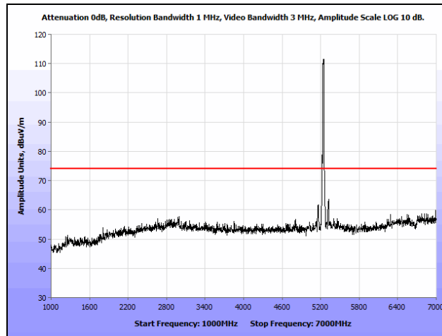
Plot 192. Radiated Spurious Emissions, 802.11n 20 MHz, High Channel, 1 GHz – 7 GHz, Peak, Omni
