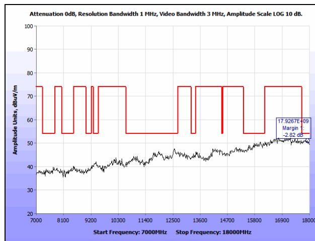
Plot 129. Radiated Spurious Emissions, 802.11n 40 MHz, High Channel, 7 GHz – 18 GHz, 7 dBi Patch
