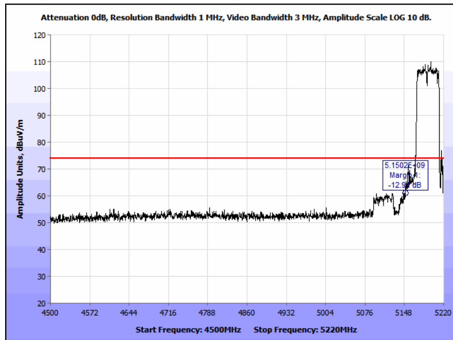
Plot 235. Restricted Band Edge, Patch Antenna, 802.11n 40 MHz, 5190 MHz, Low Channel, Peak (4.5 - 5.22 GHz Span)
