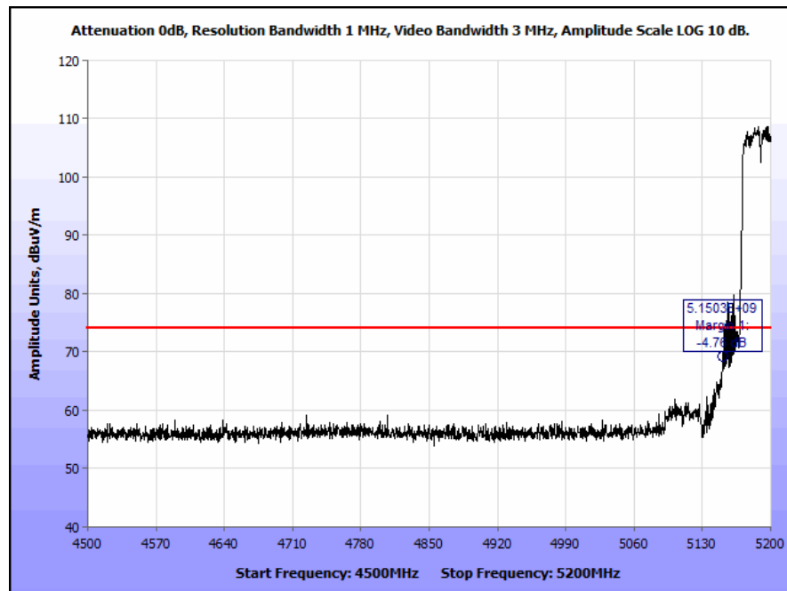
Plot 243. Restricted Band Edge, Ceiling Antenna, 802.11n 40 MHz, 5190 MHz High @ 5150 MHz Edge, Peak
