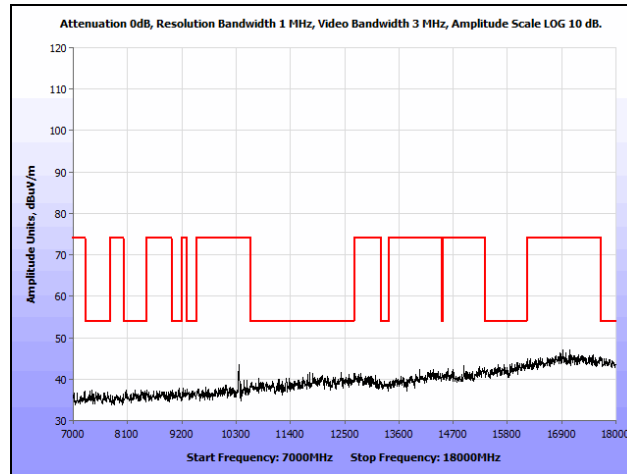
Plot 185. Radiated Spurious Emissions, 802.11n 20 MHz, Low Channel, 7 GHz – 18 GHz, Omni
