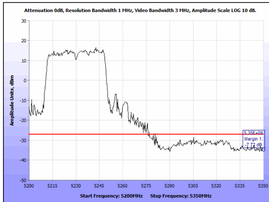
Plot 227. Radiated Band Edge 802.11n 40 MHz, High Channel, Omni Antenna (Band Edge @ 5350 MHz)
