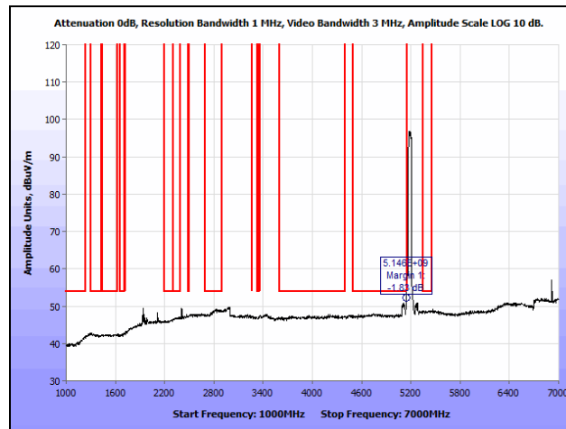
Plot 159. Radiated Spurious Emissions, 802.11n 40 MHz, Low Channel, 1 GHz – 7 GHz, Average, Ceiling
