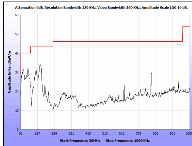
Plot 98. Radiated Spurious Emissions, 802.11a, Low Channel, 30 MHz – 1 GHz, 7 dBi Patch
