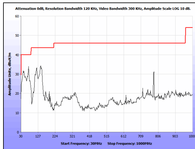
Plot 186. Radiated Spurious Emissions, 802.11n 20 MHz, Mid Channel, 30 MHz – 1 GHz, Omni
