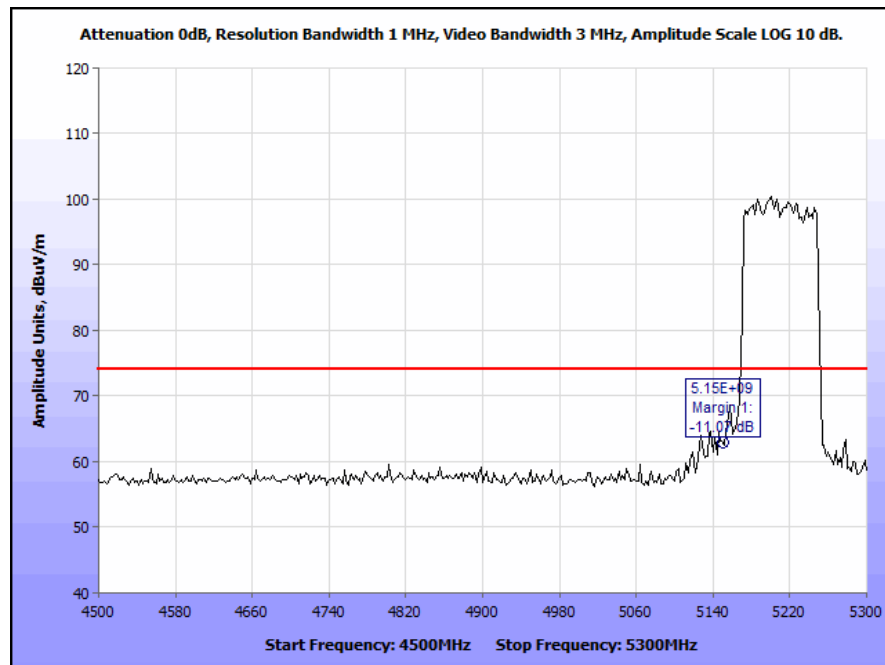
Plot 245. Restricted Band Edge, Ceiling Antenna, 802.11n 80 MHz, 5210 MHz @ 5150 MHz Edge, Peak
