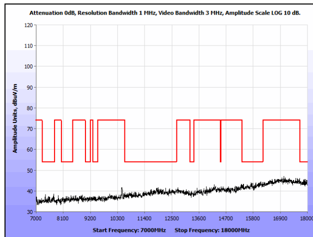
Plot 193. Radiated Spurious Emissions, 802.11n 20 MHz, High Channel, 7 GHz – 18 GHz, Omni
