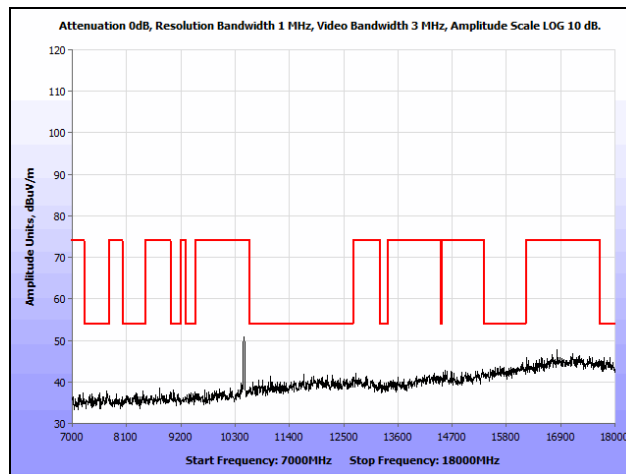
Plot 157. Radiated Spurious Emissions, 802.11n 20 MHz, High Channel, 7 GHz – 18 GHz, Ceiling
