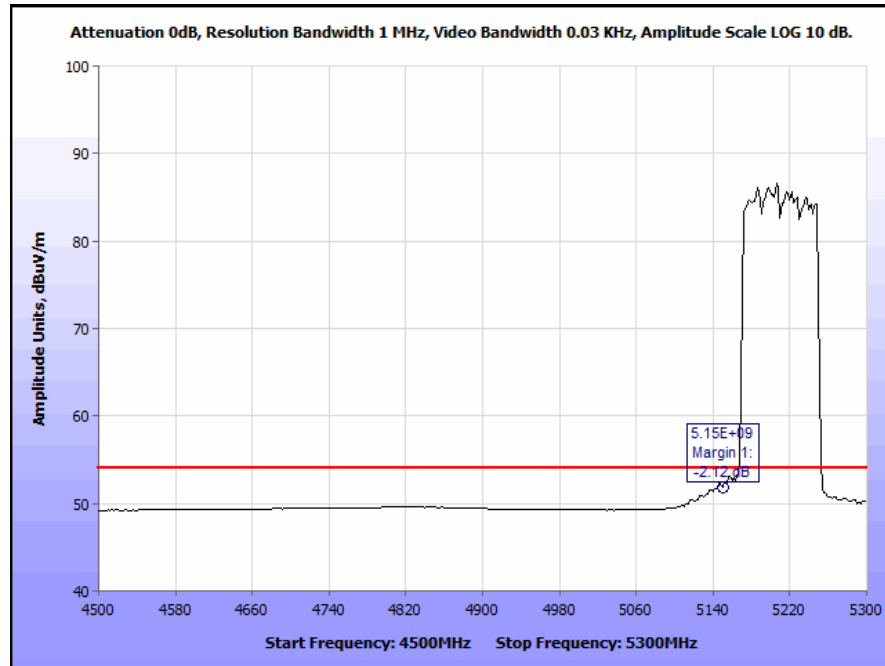
Plot 244. Restricted Band Edge, Ceiling Antenna, 802.11n 80 MHz, 5210 MHz @ 5150 MHz Edge, Average
