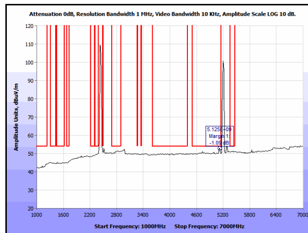
Plot 287. Co-location, Radiated Spurious Emissions, Patch, 802.11n 20 MHz, 2437 & 5200 MHz, 1 GHz – 7 GHz, Average
