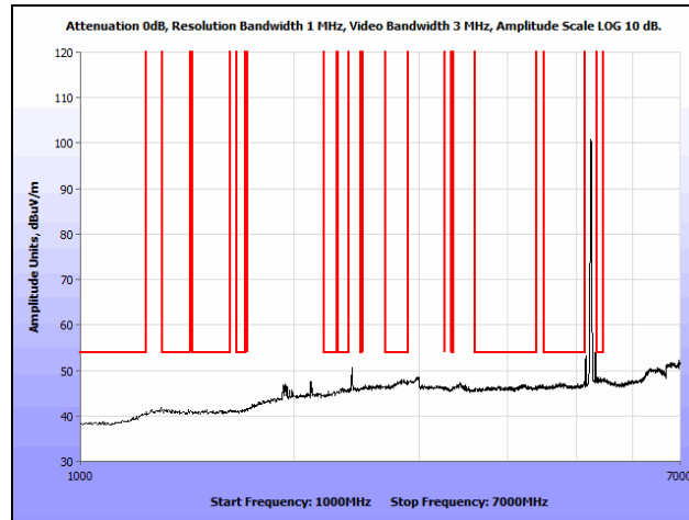
Plot 143. Radiated Spurious Emissions, 802.11a, High Channel, 1 GHz – 7 GHz, Average, Ceiling
