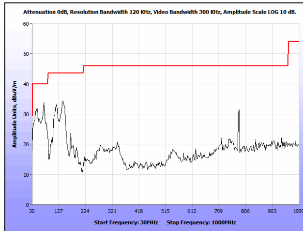
Plot 170. Radiated Spurious Emissions, 802.11a, Low Channel, 30 MHz – 1 GHz, Omni
