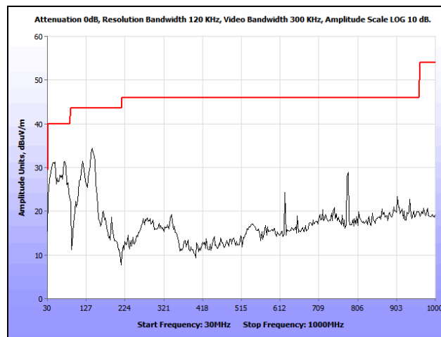
Plot 102. Radiated Spurious Emissions, 802.11a, Mid Channel, 30 MHz – 1 GHz, 7 dBi Patch
