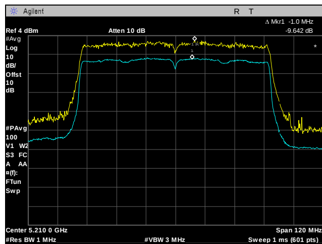
Plot 96. Peak Excursion Ratio, 802.11n 80 MHz, Port 2
