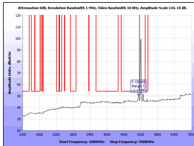
Plot 103. Radiated Spurious Emissions, 802.11a, Mid Channel, 1 GHz – 7 GHz, Average, 7 dBi Patch
