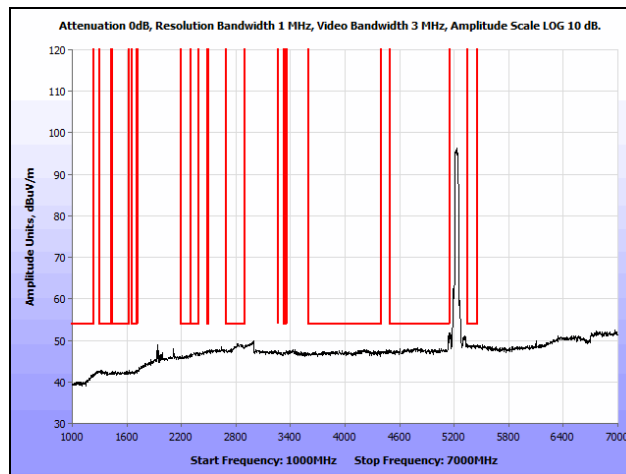
Plot 163. Radiated Spurious Emissions, 802.11n 40 MHz, High Channel, 1 GHz – 7 GHz, Average, Ceiling
