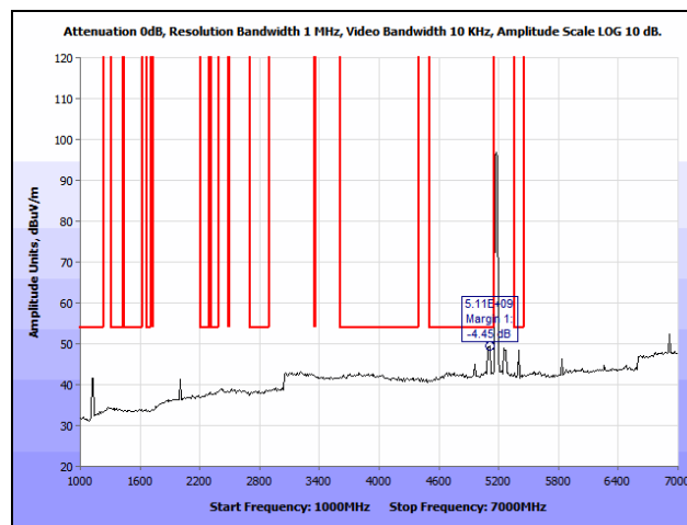
Plot 111. Radiated Spurious Emissions, 802.11n 20 MHz, Low Channel, 1 GHz – 7 GHz, Average, 7 dBi Patch
