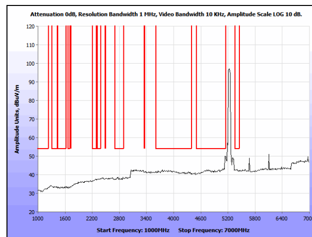
Plot 127. Radiated Spurious Emissions, 802.11n 40 MHz, High Channel, 1 GHz – 7 GHz, Average, 7 dBi Patch
