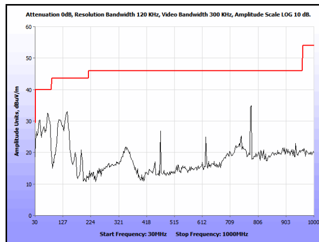
Plot 286. Co-location, Radiated Spurious Emissions, Patch, 802.11n 20 MHz, 2437 & 5200 MHz, 30 MHz – 1 GHz
