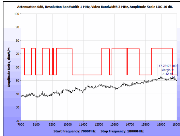
Plot 101. Radiated Spurious Emissions, 802.11a, Low Channel, 7 GHz – 18 GHz, 7 dBi Patch
