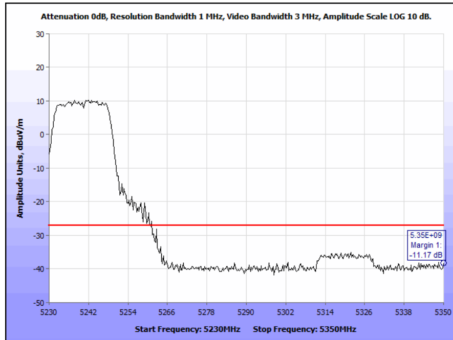
Plot 215. Radiated Band Edge 802.11a, High Channel, Ceiling Antenna (Band Edge @ 5350 MHz)
