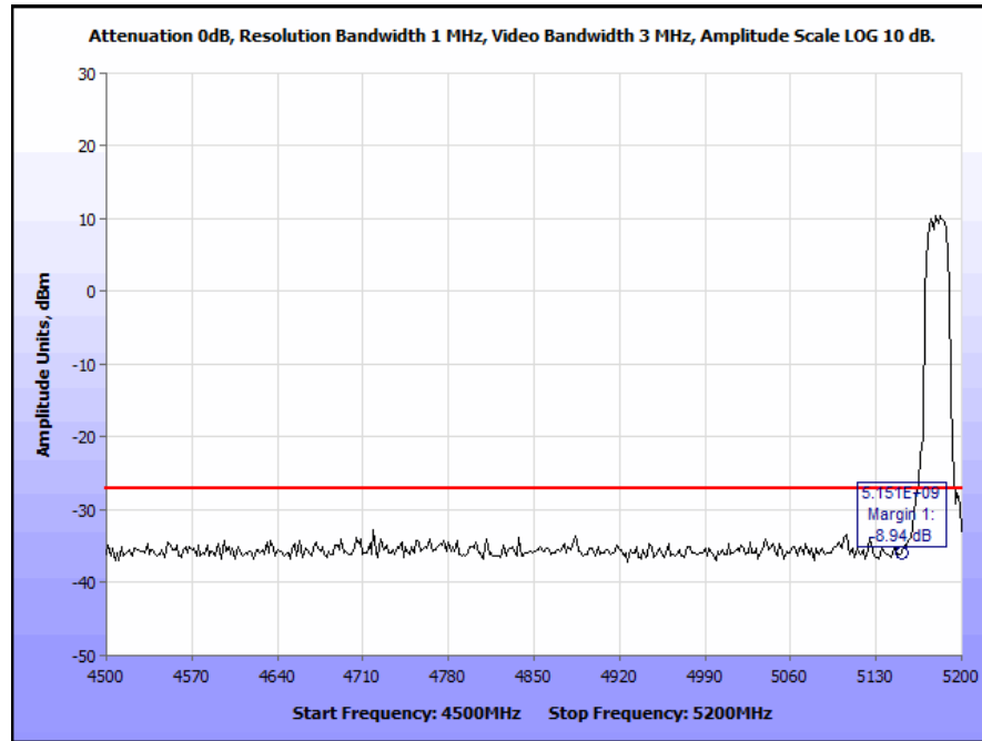
Plot 222. Radiated Band Edge 802.11a, Low Channel, Omni Antenna (Band Edge @ 5150 MHz)
