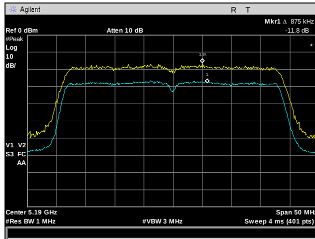
Plot 91. Peak Excursion Ratio, Low Channel, 802.11n 40 MHz, Port 2
