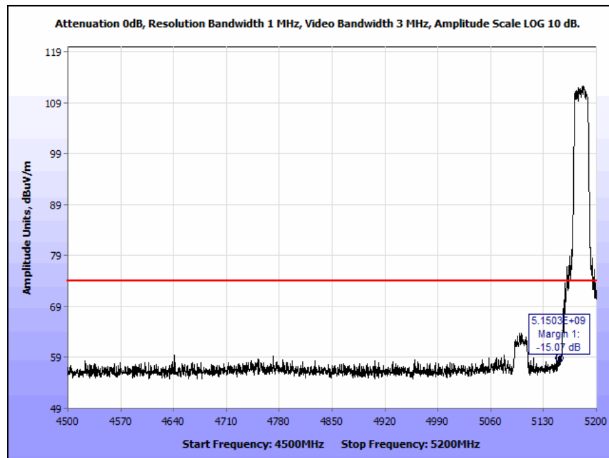
Plot 241. Restricted Band Edge, Ceiling Antenna, 802.11n 20 MHz, 5180 MHz High @ 5150 MHz Edge, Peak
