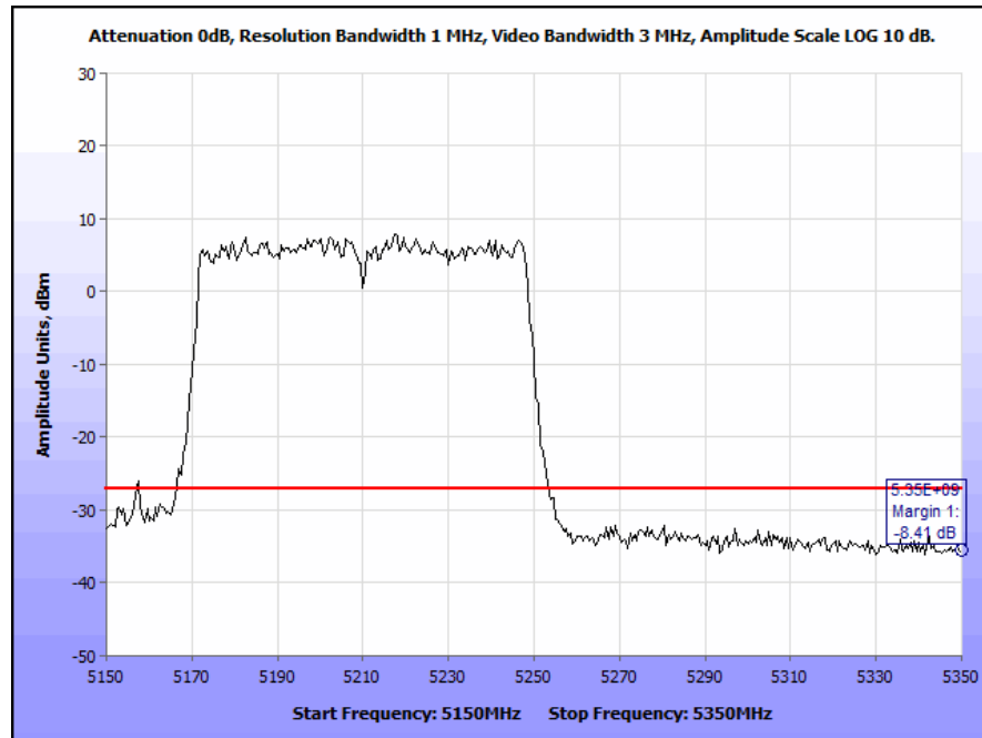
Plot 213. Radiated Band Edge 802.11n 80 MHz, 7 dBi Patch Antenna (Band Edge @ 5350 MHz)
