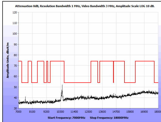
Plot 169. Radiated Spurious Emissions, 802.11n 80 MHz, Low Channel, 7 GHz – 18 GHz, Ceiling
