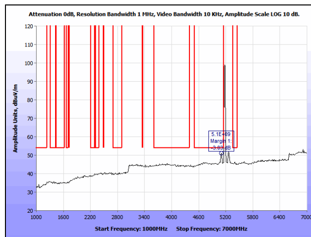
Plot 99. Radiated Spurious Emissions, 802.11a, Low Channel, 1 GHz – 7 GHz, Average, 7 dBi Patch
