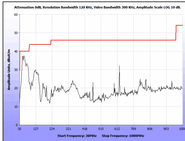
Plot 162. Radiated Spurious Emissions, 802.11n 40 MHz, High Channel, 30 MHz – 1 GHz, Ceiling
