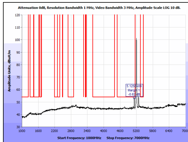
Plot 187. Radiated Spurious Emissions, 802.11n 20 MHz, Mid Channel, 1 GHz – 7 GHz, Average, Omni
