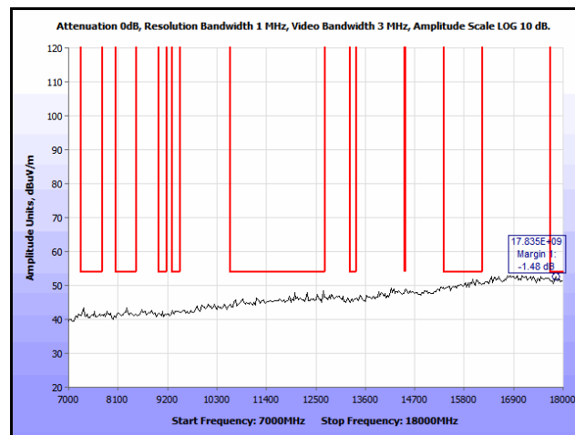
Plot 289. Co-location, Radiated Spurious Emissions, Patch, 802.11n 20 MHz, 2437 & 5200 MHz, 7 GHz – 18 GHz, Peak
