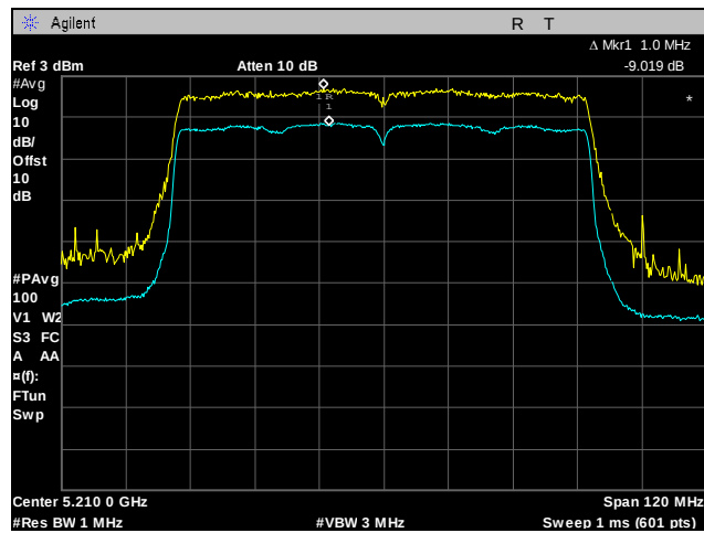
Plot 95. Peak Excursion Ratio, 802.11n 80 MHz, Port 1
