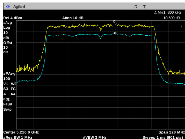
Plot 97. Peak Excursion Ratio, 802.11n 80 MHz, Port 3
