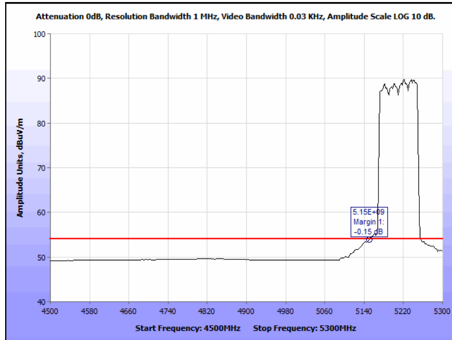
Plot 252. Restricted Band Edge, Omni Antenna, 802.11n 80 MHz, 5210 MHz @ 5150 MHz Edge, Average
