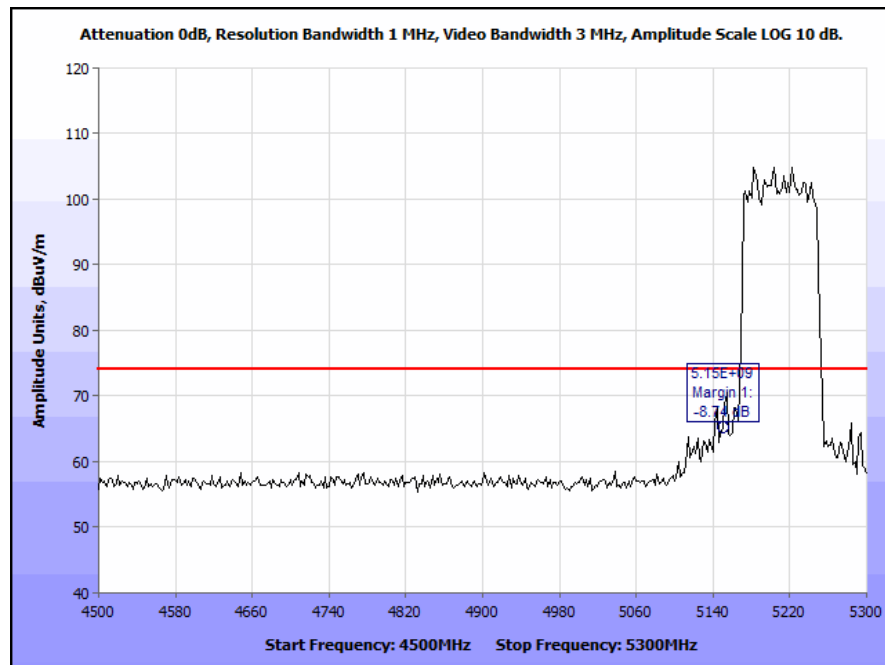
Plot 237. Restricted Band Edge, Patch Antenna, 802.11n 80 MHz, 5210 MHz @ 5150 MHz Edge, Peak
