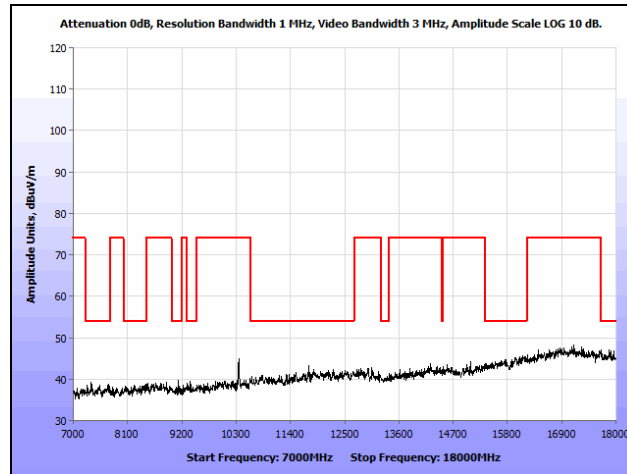
Plot 173. Radiated Spurious Emissions, 802.11a, Low Channel, 7 GHz – 18 GHz, Omni
