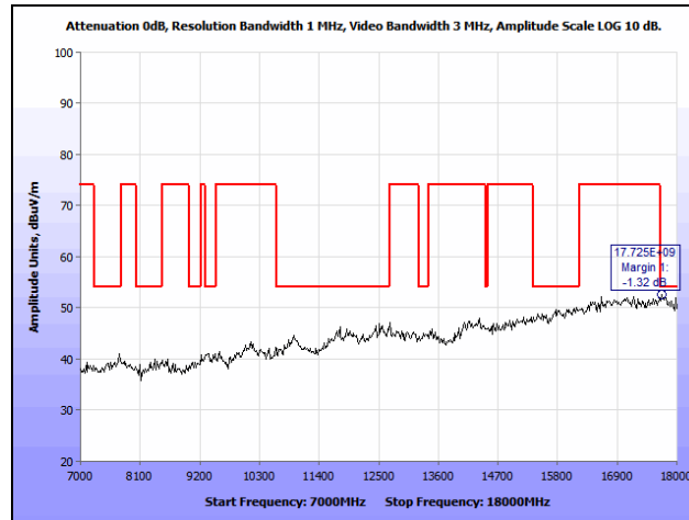
Plot 113. Radiated Spurious Emissions, 802.11n 20 MHz, Low Channel, 7 GHz – 18 GHz, 7 dBi Patch
