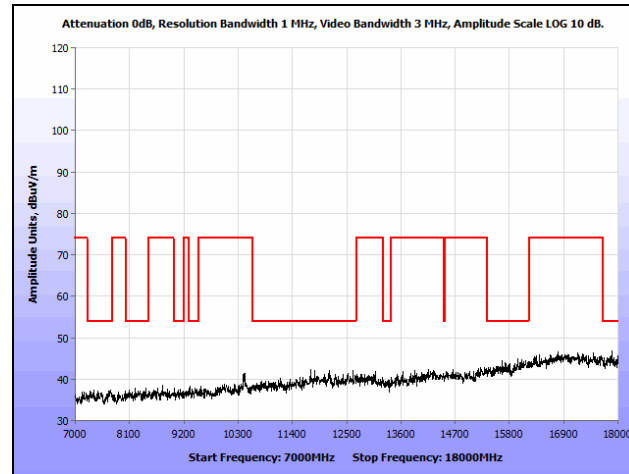
Plot 205. Radiated Spurious Emissions, 802.11n 80 MHz, Low Channel, 7 GHz – 18 GHz, Omni
