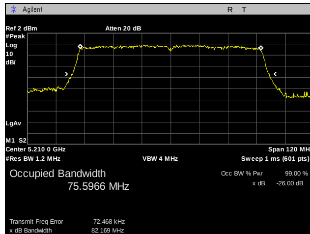
Plot 33. 26 dB Occupied Bandwidth, 802.11n 80 MHz, Port 2
