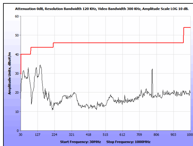
Plot 190. Radiated Spurious Emissions, 802.11n 20 MHz, High Channel, 30 MHz – 1 GHz, Omni
