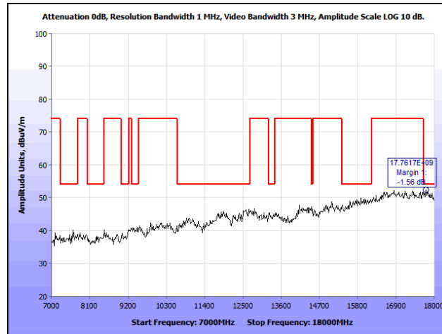
Plot 125. Radiated Spurious Emissions, 802.11n 40 MHz, Low Channel, 7 GHz – 18 GHz, 7 dBi Patch
