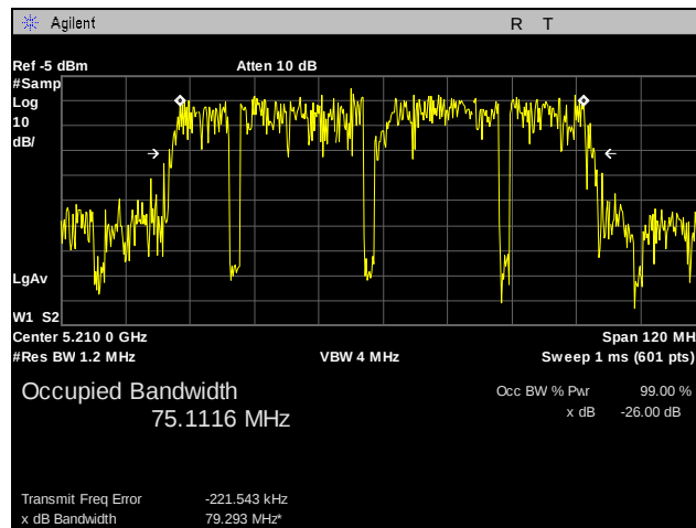
Plot 53. 99% Occupied Bandwidth, 802.11n 80 MHz, Port 1
