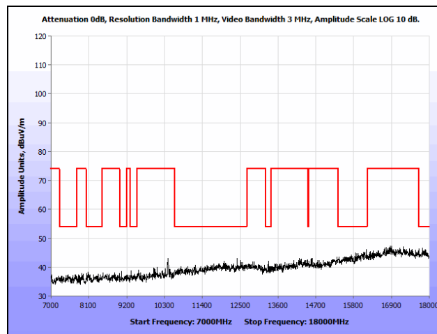
Plot 141. Radiated Spurious Emissions, 802.11a, Mid Channel, 7 GHz – 18 GHz, Ceiling
