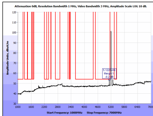
Plot 151. Radiated Spurious Emissions, 802.11n 20 MHz, Mid Channel, 1 GHz – 7 GHz, Average, Ceiling
