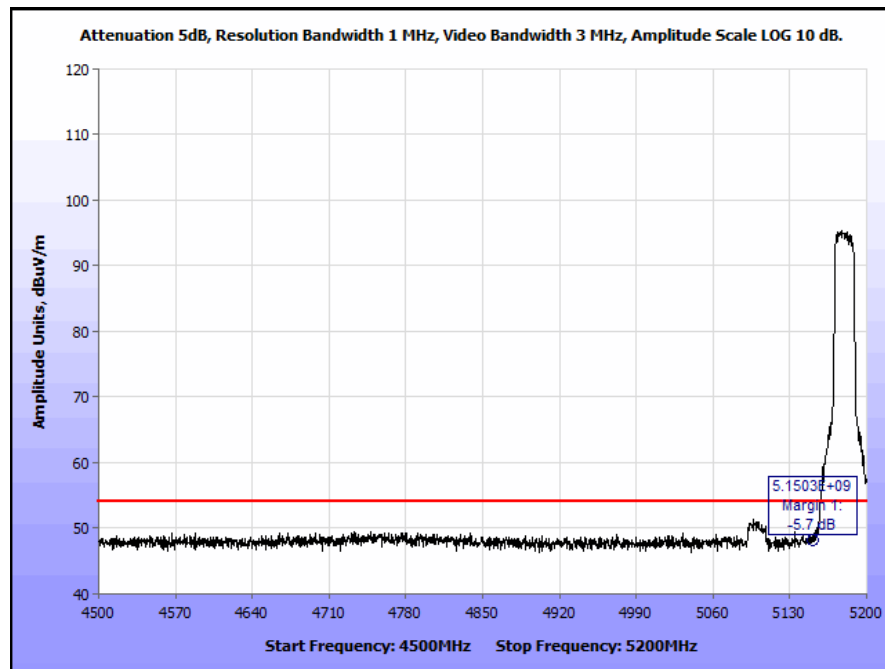
Plot 246. Restricted Band Edge, Omni Antenna, 802.11a 20 MHz, 5180 MHz Low @ 5150 MHz Edge, Average
