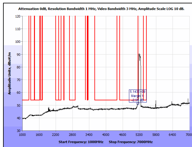
Plot 167. Radiated Spurious Emissions, 802.11n 80 MHz, Low Channel, 1 GHz – 7 GHz, Average, Ceiling
