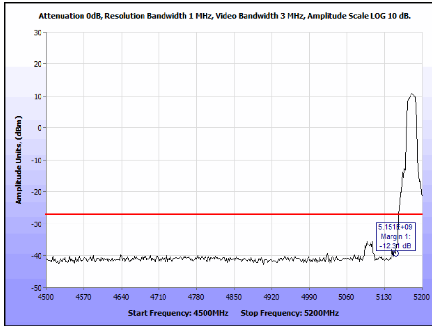
Plot 214. Radiated Band Edge 802.11a, Low Channel, Ceiling Antenna (Band Edge @ 5150 MHz)
