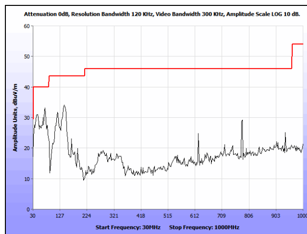
Plot 106. Radiated Spurious Emissions, 802.11a, High Channel, 30 MHz – 1 GHz, 7 dBi Patch
