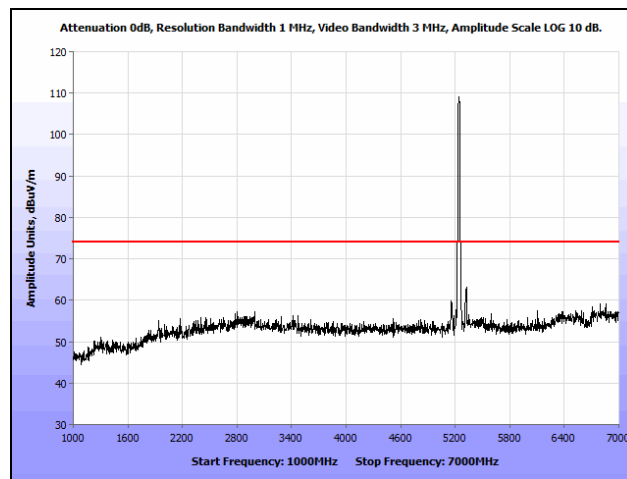
Plot 180. Radiated Spurious Emissions, 802.11a, High Channel, 1 GHz – 7 GHz, Peak, Omni
