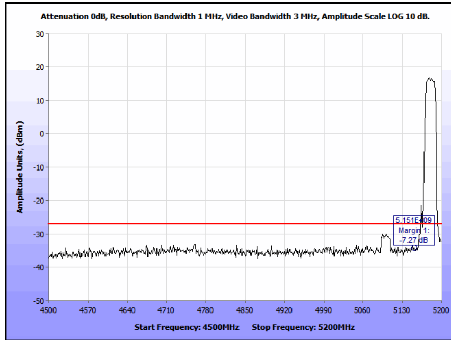
Plot 206. Radiated Band Edge 802.11a, Low Channel, 7 dBi Patch Antenna (Band Edge @ 5150 MHz)
