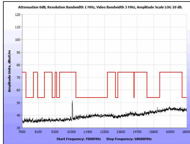
Plot 149. Radiated Spurious Emissions, 802.11n 20 MHz, Low Channel, 7 GHz – 18 GHz, Ceiling
