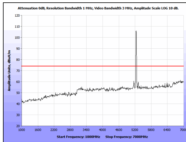
Plot 108. Radiated Spurious Emissions, 802.11a, High Channel, 1 GHz – 7 GHz, Peak, 7 dBi Patch
