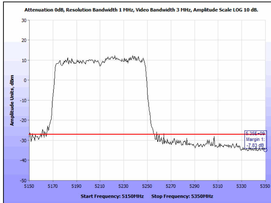
Plot 229. Radiated Band Edge 802.11n 80 MHz, Omni Antenna (Band Edge @ 5350 MHz)
