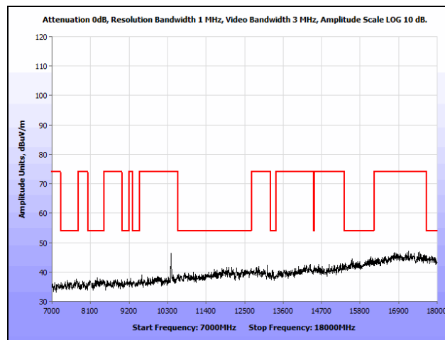
Plot 189. Radiated Spurious Emissions, 802.11n 20 MHz, Mid Channel, 7 GHz – 18 GHz, Omni
