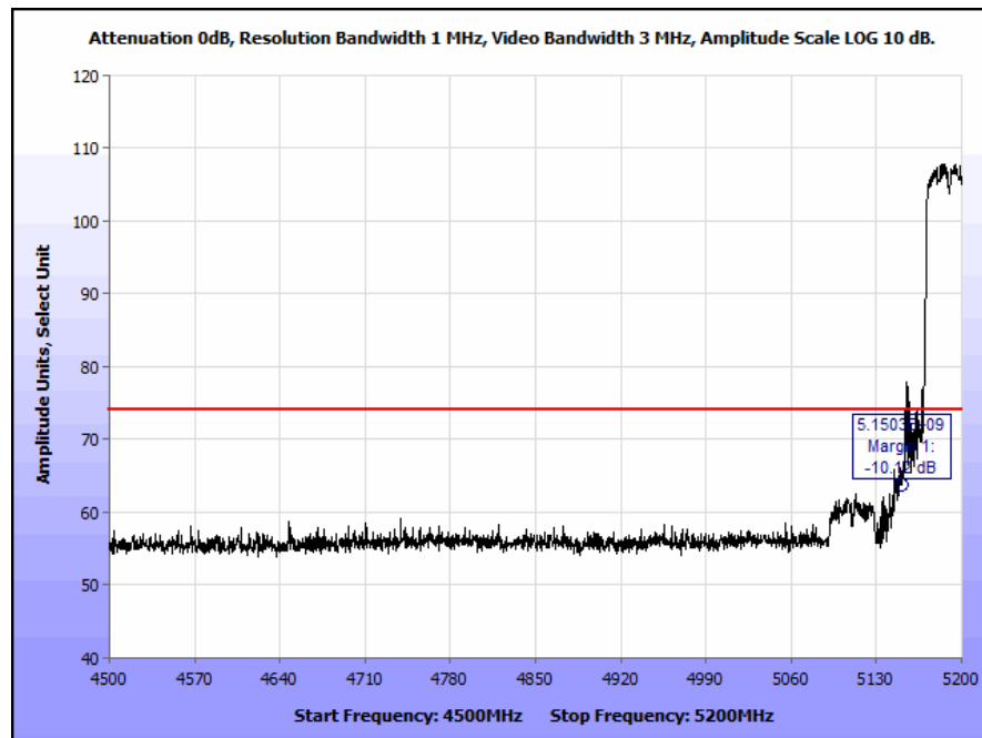
Plot 251. Restricted Band Edge, Omni Antenna, 802.11n 40 MHz, 5190 MHz Low @ 5150 MHz Edge, Peak
