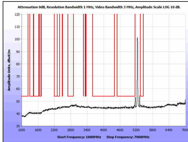
Plot 191. Radiated Spurious Emissions, 802.11n 20 MHz, High Channel, 1 GHz – 7 GHz, Average, Omni
