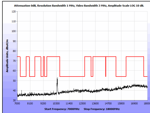
Plot 161. Radiated Spurious Emissions, 802.11n 40 MHz, Low Channel, 7 GHz – 18 GHz, Ceiling
