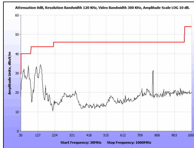
Plot 182. Radiated Spurious Emissions, 802.11n 20 MHz, Low Channel, 30 MHz – 1 GHz, Omni
