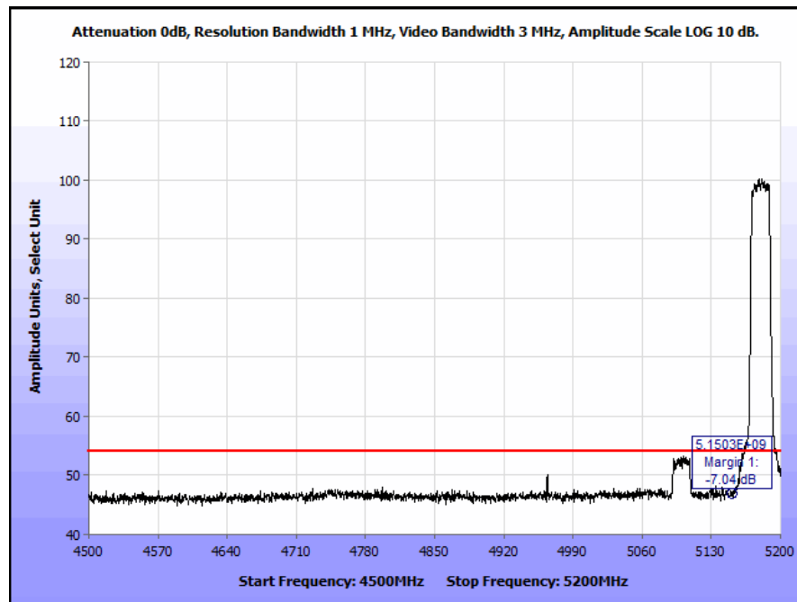
Plot 248. Restricted Band Edge, Omni Antenna, 802.11n 20 MHz, 5180 MHz Low @ 5150 MHz Edge, Average
