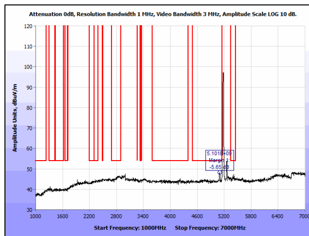
Plot 171. Radiated Spurious Emissions, 802.11a, Low Channel, 1 GHz – 7 GHz, Average, Omni
