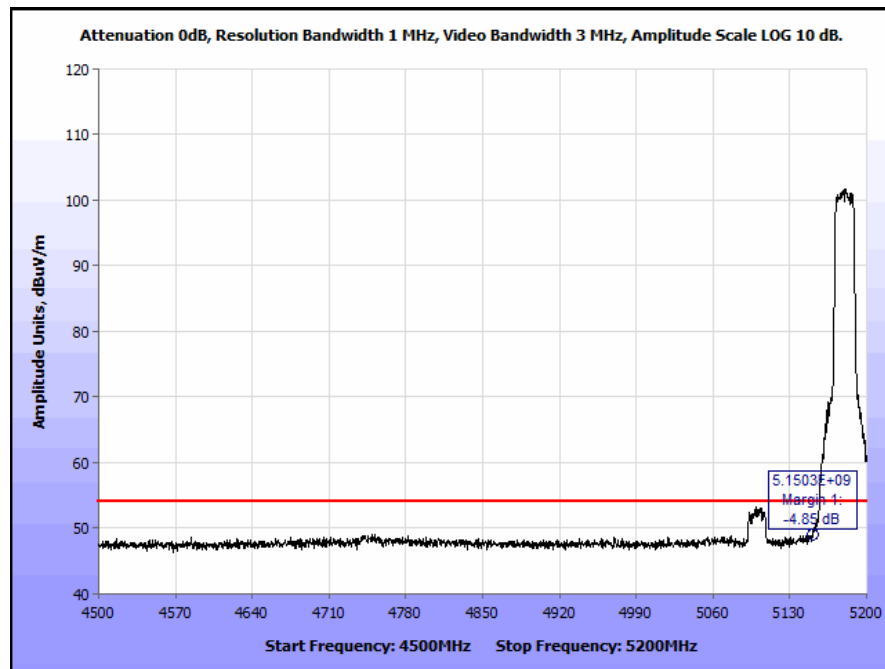
Plot 238. Restricted Band Edge, Ceiling Antenna, 802.11a 20 MHz, 5180 MHz, High @ 5150 MHz Edge, Average
