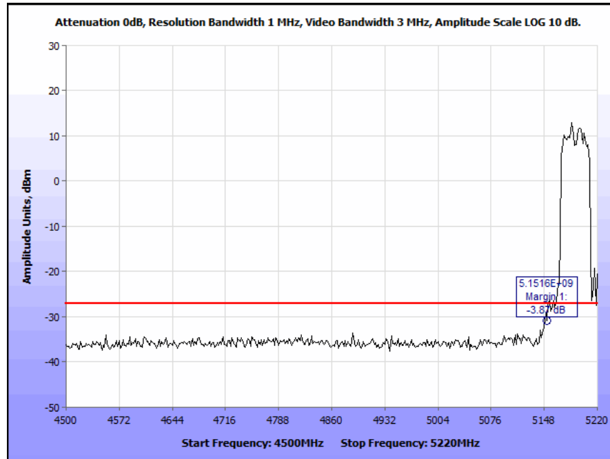
Plot 226. Radiated Band Edge 802.11n 40 MHz, Low Channel, Omni Antenna (Band Edge @ 5150 MHz)
