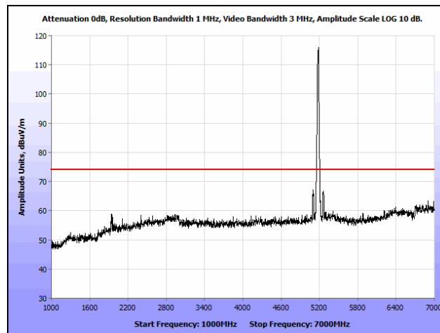
Plot 148. Radiated Spurious Emissions, 802.11n 20 MHz, Low Channel, 1 GHz – 7 GHz, Peak, Ceiling
