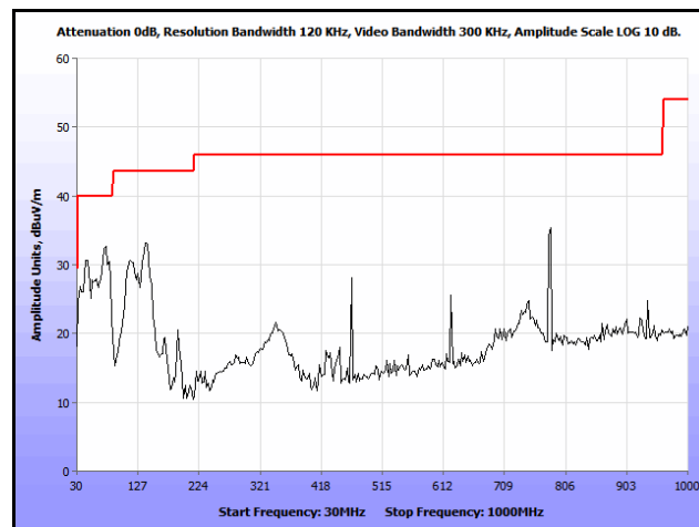
Plot 290. Co-location, Radiated Spurious Emissions, Patch, 802.11n 20 MHz, 2462 & 5200 MHz, 30 MHz – 1 GHz
