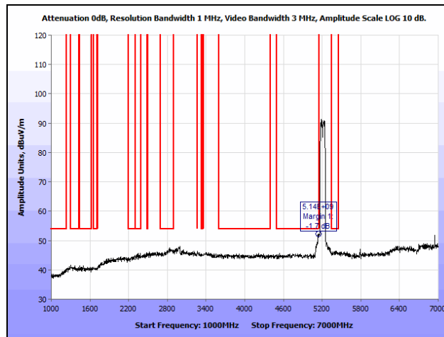
Plot 203. Radiated Spurious Emissions, 802.11n 80 MHz, Low Channel, 1 GHz – 7 GHz, Average, Omni
