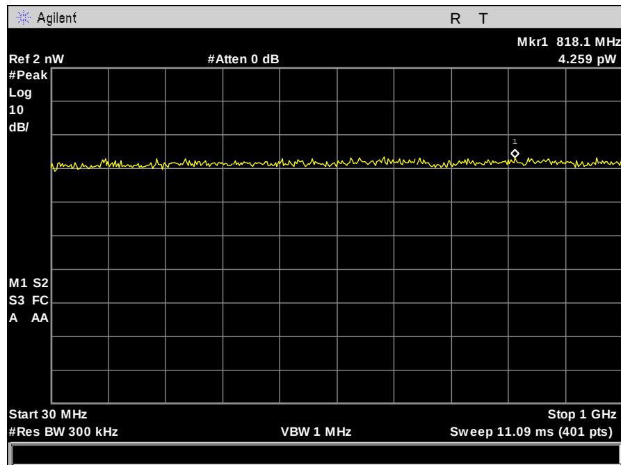
Plot 310. Receiver Spurious Emission, 30 MHz – 1 GHz, Port 3
