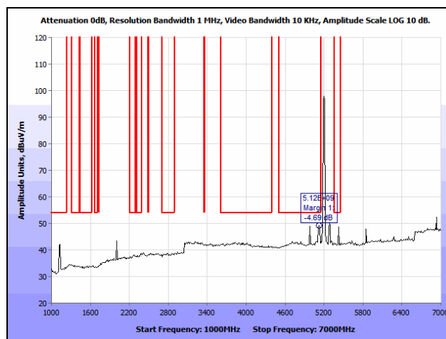
Plot 115. Radiated Spurious Emissions, 802.11n 20 MHz, Mid Channel, 1 GHz – 7 GHz, Average, 7 dBi Patch
