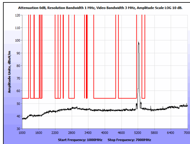
Plot 199. Radiated Spurious Emissions, 802.11n 40 MHz, High Channel, 1 GHz – 7 GHz, Average, Omni
