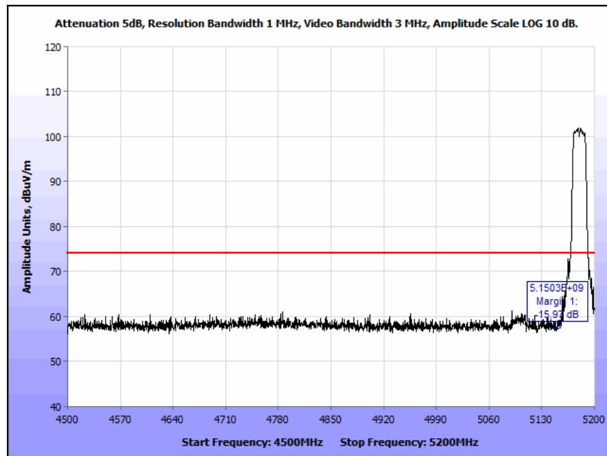
Plot 247. Restricted Band Edge, Omni Antenna, 802.11a 20 MHz, 5180 MHz Low @ 5150 MHz Edge, Peak
