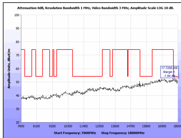
Plot 117. Radiated Spurious Emissions, 802.11n 20 MHz, Mid Channel, 7 GHz – 18 GHz, 7 dBi Patch
