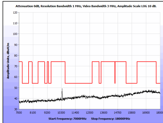
Plot 137. Radiated Spurious Emissions, 802.11a, Low Channel, 7 GHz – 18 GHz, Ceiling
