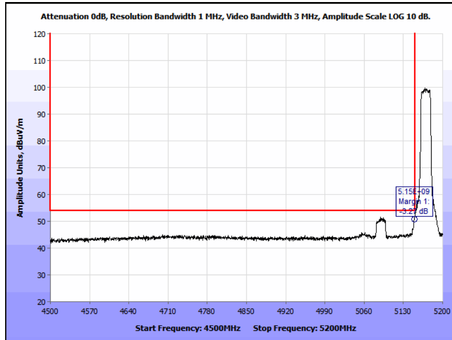
Plot 230. Restricted Band Edge, Patch Antenna, 802.11a, 5180 MHz, Low Channel, Average (4.5 - 5.2 GHz Span)
