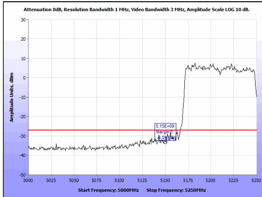
Plot 220. Radiated Band Edge 802.11n 80 MHz, Ceiling Antenna (Band Edge @ 5150 MHz)
