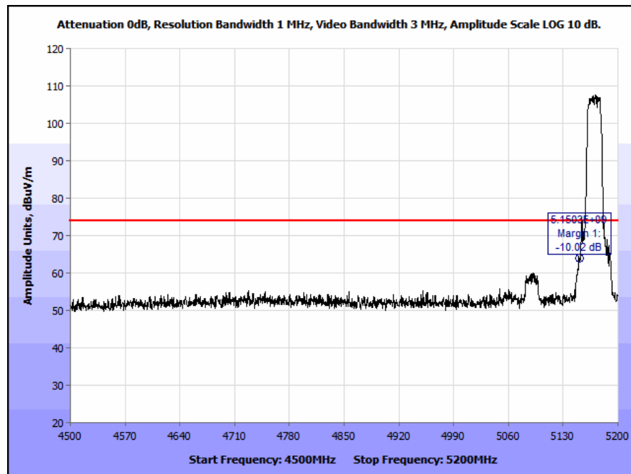
Plot 231. Restricted Band Edge, Patch Antenna, 802.11a, 5180 MHz, Low Channel, Peak (4.5 - 5.2 GHz Span)
