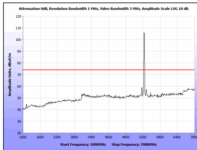
Plot 120. Radiated Spurious Emissions, 802.11n 20 MHz, High Channel, 1 GHz – 7 GHz, Peak, 7 dBi Patch
