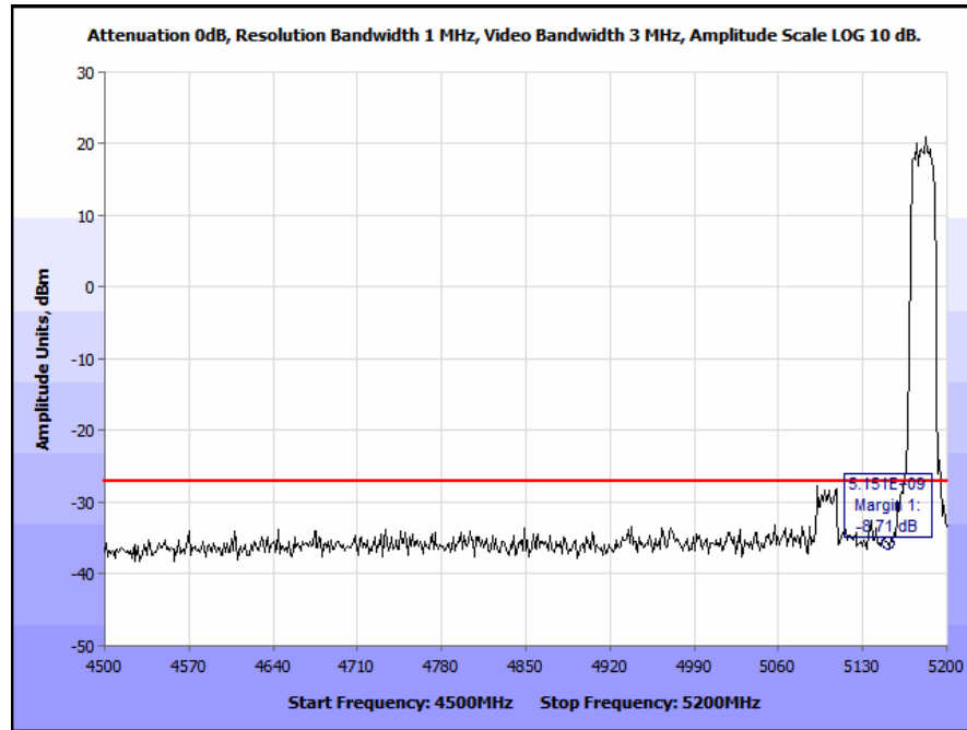
Plot 208. Radiated Band Edge 802.11n 20 MHz, Low Channel, 7 dBi Patch Antenna (Band Edge @ 5150 MHz)
