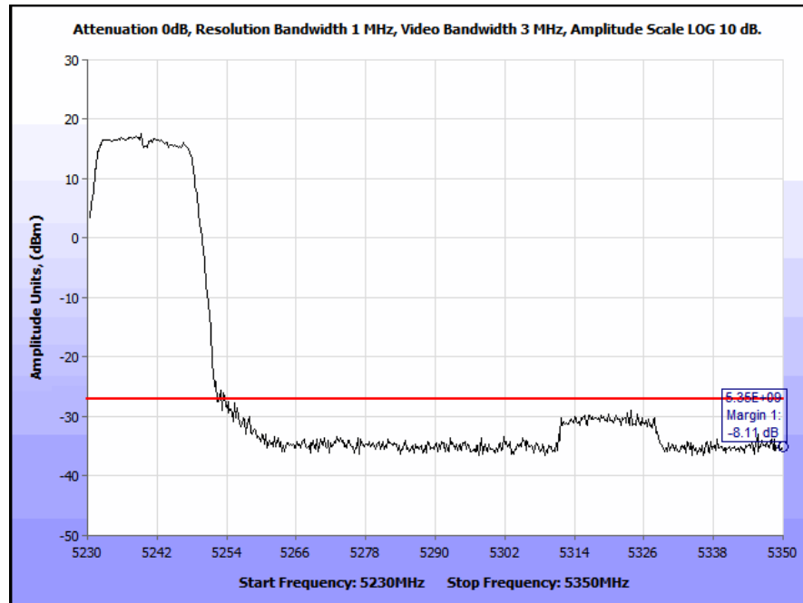
Plot 207. Radiated Band Edge 802.11a, High Channel, 7 dBi Patch Antenna (Band Edge @ 5350 MHz)
