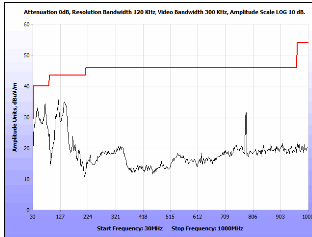
Plot 194. Radiated Spurious Emissions, 802.11n 40 MHz, Low Channel, 30 MHz – 1 GHz, Omni
