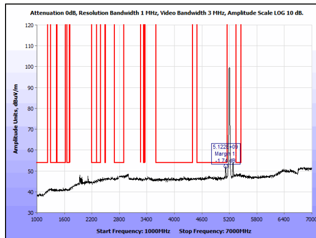
Plot 139. Radiated Spurious Emissions, 802.11a, Mid Channel, 1 GHz – 7 GHz, Average, Ceiling
