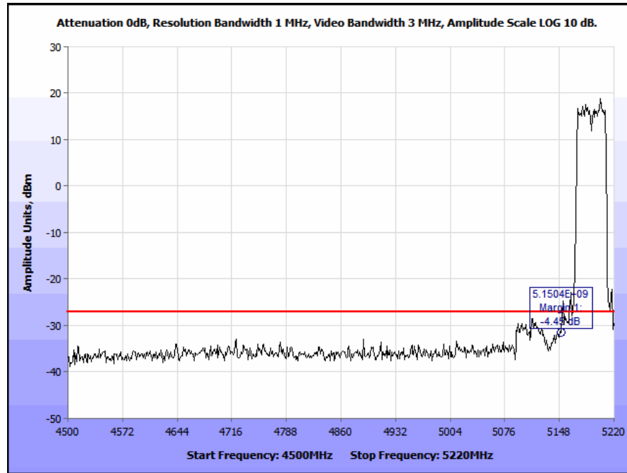
Plot 210. Radiated Band Edge 802.11n 40 MHz, Low Channel, 7 dBi Patch Antenna (Band Edge @ 5150 MHz)
