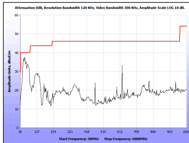
Plot 142. Radiated Spurious Emissions, 802.11a, High Channel, 30 MHz – 1 GHz, Ceiling
