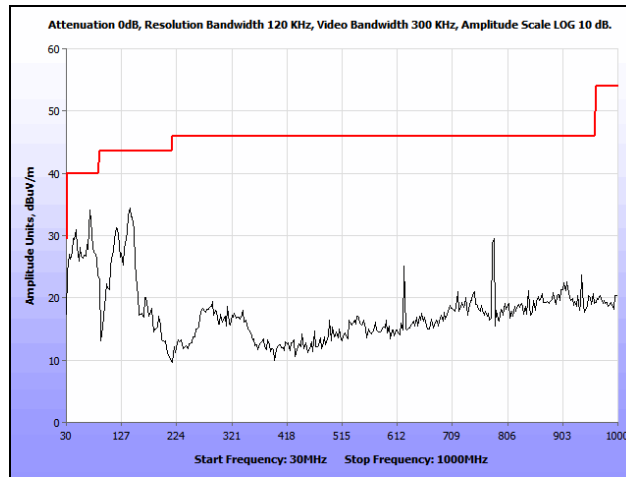
Plot 122. Radiated Spurious Emissions, 802.11n 40 MHz, Low Channel, 30 MHz – 1 GHz, 7 dBi Patch
