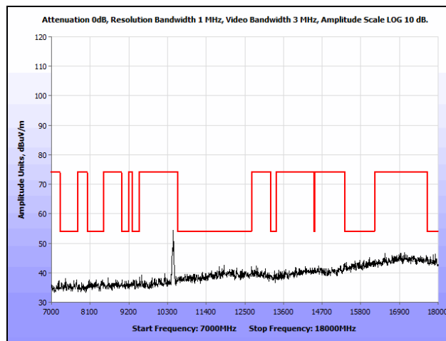
Plot 165. Radiated Spurious Emissions, 802.11n 40 MHz, High Channel, 7 GHz – 18 GHz, Ceiling
