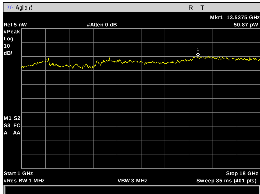
Plot 307. Receiver Spurious Emission, 1 GHz – 18 GHz, Port 1
