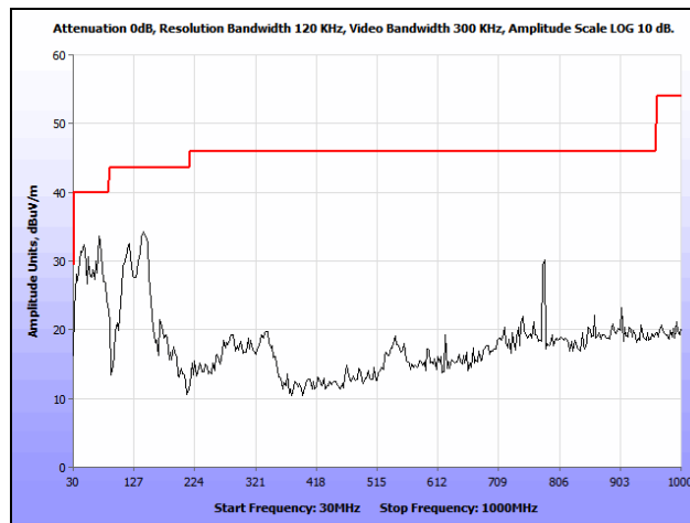
Plot 178. Radiated Spurious Emissions, 802.11a, High Channel, 30 MHz – 1 GHz, Omni
