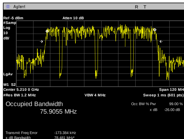
Plot 55. 99% Occupied Bandwidth, 802.11n 80 MHz, Port 3
