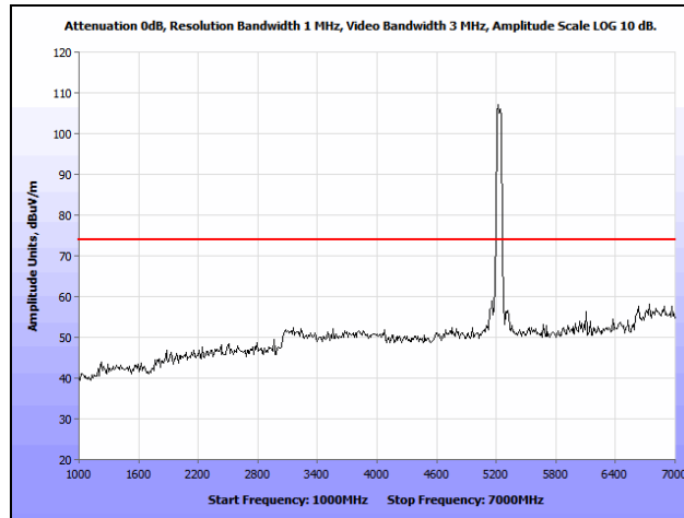
Plot 128. Radiated Spurious Emissions, 802.11n 40 MHz, High Channel, 1 GHz – 7 GHz, Peak, 7 dBi Patch
