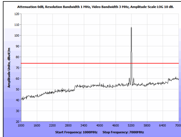
Plot 104. Radiated Spurious Emissions, 802.11a, Mid Channel, 1 GHz – 7 GHz, Peak, 7 dBi Patch
