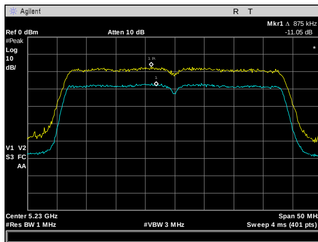
Plot 92. Peak Excursion Ratio, High Channel, 802.11n 40 MHz, Port 2
