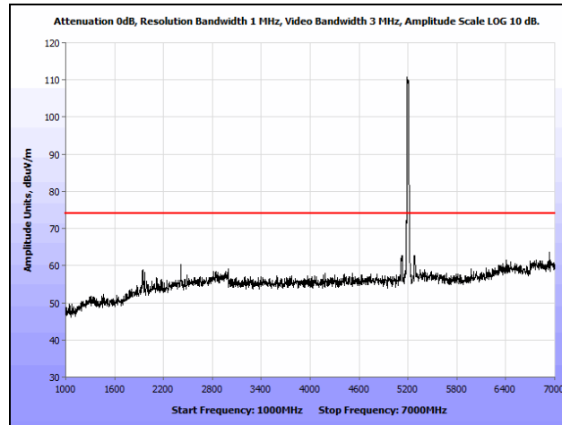
Plot 152. Radiated Spurious Emissions, 802.11n 20 MHz, Mid Channel, 1 GHz – 7 GHz, Peak, Ceiling
