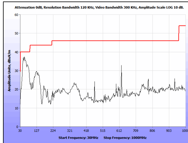
Plot 146. Radiated Spurious Emissions, 802.11n 20 MHz, Low Channel, 30 MHz – 1 GHz, Ceiling
