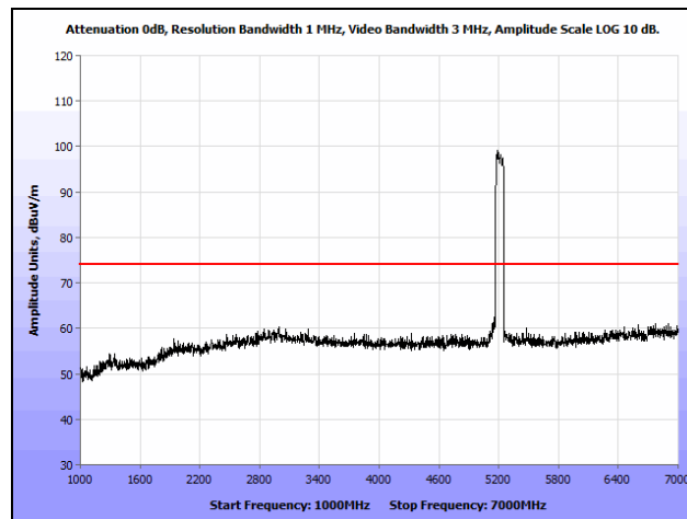
Plot 132. Radiated Spurious Emissions, 802.11n 80 MHz, 1 GHz – 7 GHz, Peak, 7 dBi Patch
