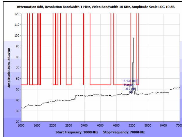
Plot 107. Radiated Spurious Emissions, 802.11a, High Channel, 1 GHz – 7 GHz, Average, 7 dBi Patch
