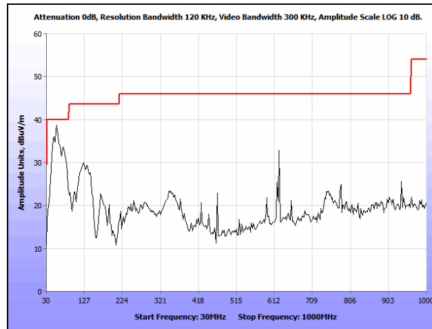
Plot 158. Radiated Spurious Emissions, 802.11n 40 MHz, Low Channel, 30 MHz – 1 GHz, Ceiling
