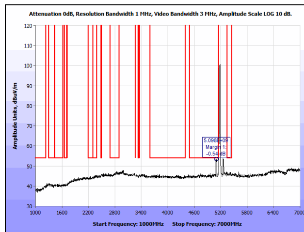
Plot 183. Radiated Spurious Emissions, 802.11n 20 MHz, Low Channel, 1 GHz – 7 GHz, Average, Omni
