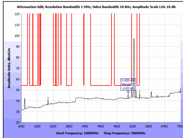
Plot 119. Radiated Spurious Emissions, 802.11n 20 MHz, High Channel, 1 GHz – 7 GHz, Average, 7 dBi Patch
