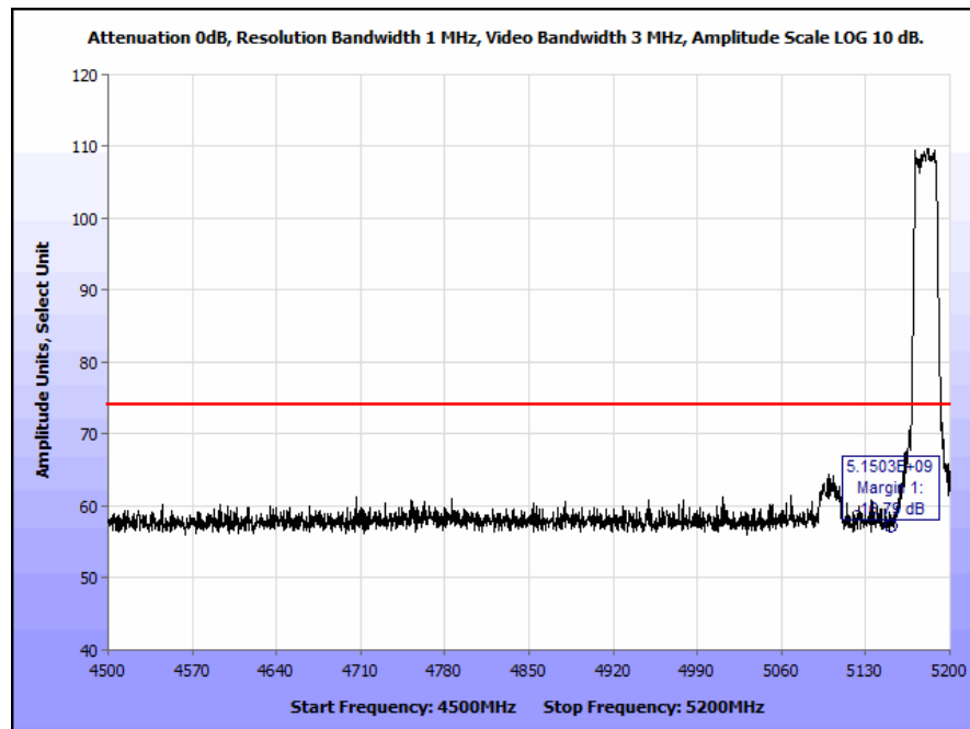
Plot 249. Restricted Band Edge, Omni Antenna, 802.11n 20 MHz, 5180 MHz Low @ 5150 MHz Edge, Peak
