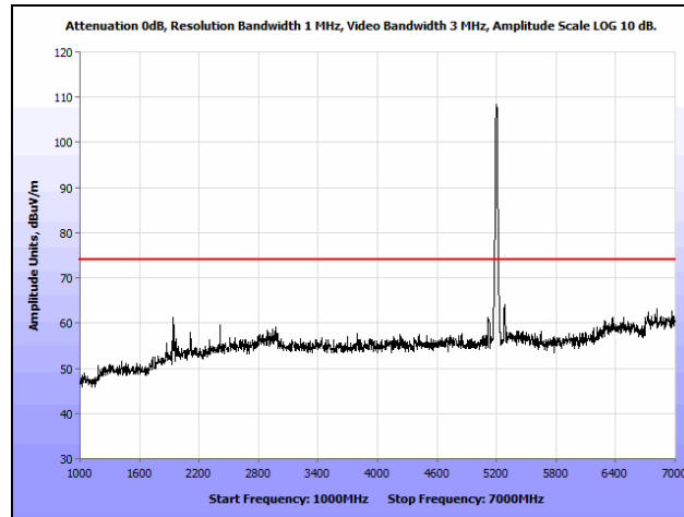
Plot 140. Radiated Spurious Emissions, 802.11a, Mid Channel, 1 GHz – 7 GHz, Peak, Ceiling
