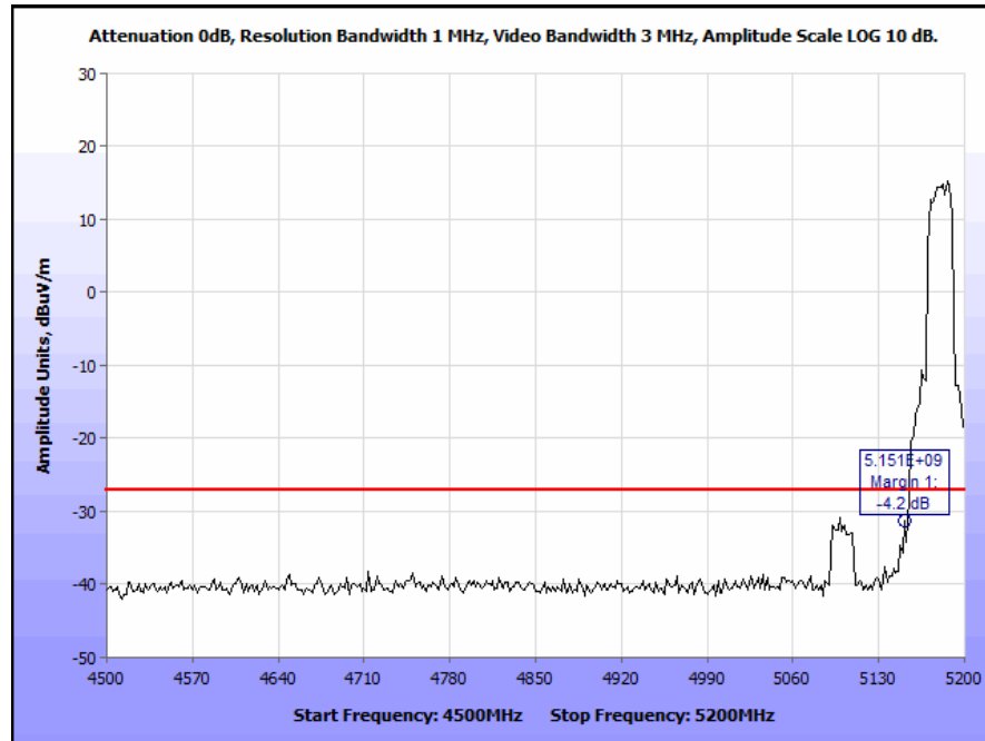
Plot 216. Radiated Band Edge 802.11n 20 MHz, Low Channel, Ceiling Antenna (Band Edge @ 5150 MHz)
