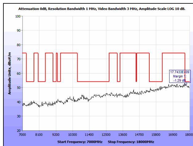
Plot 121. Radiated Spurious Emissions, 802.11n 20 MHz, High Channel, 7 GHz – 18 GHz, 7 dBi Patch
