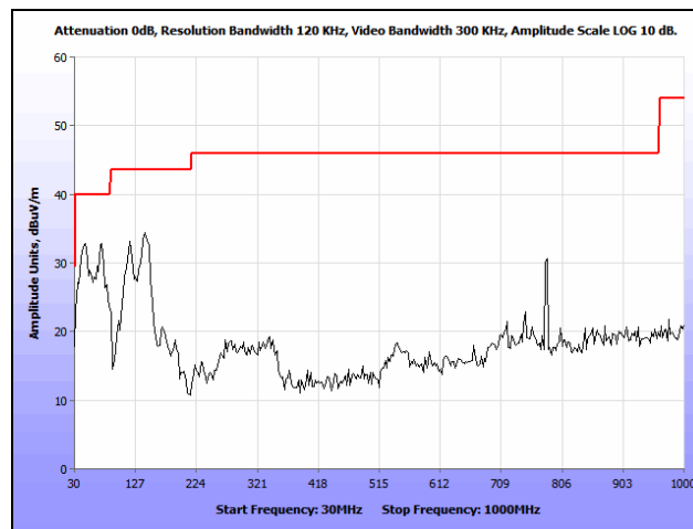
Plot 174. Radiated Spurious Emissions, 802.11a, Mid Channel, 30 MHz – 1 GHz, Omni
