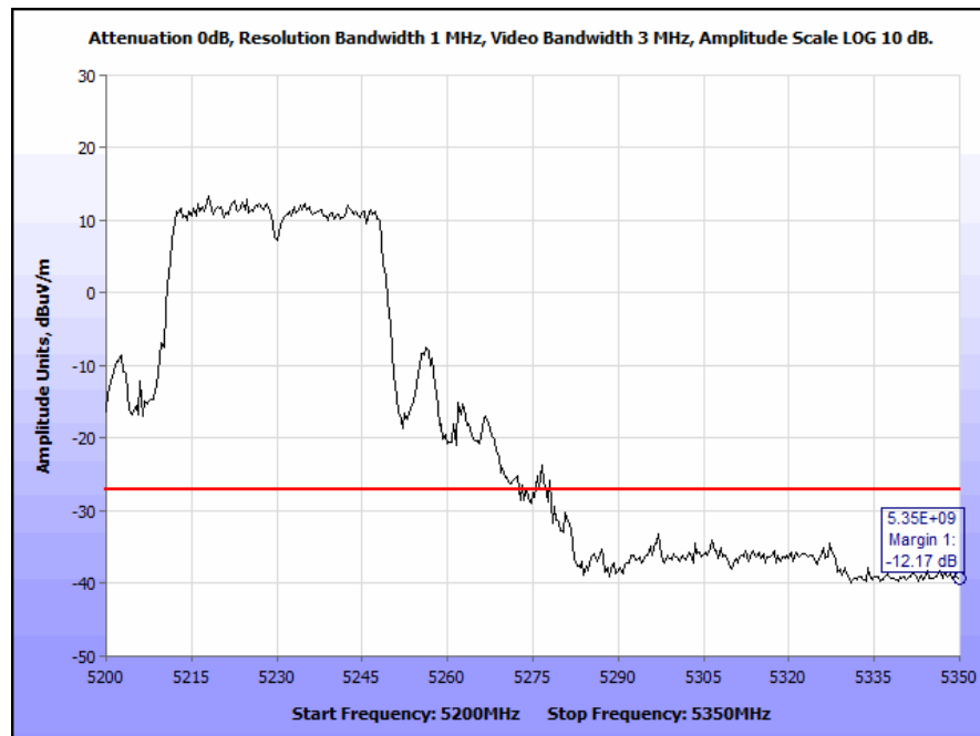
Plot 219. Radiated Band Edge 802.11n 40 MHz, High Channel, Ceiling Antenna (Band Edge @ 5350 MHz)
