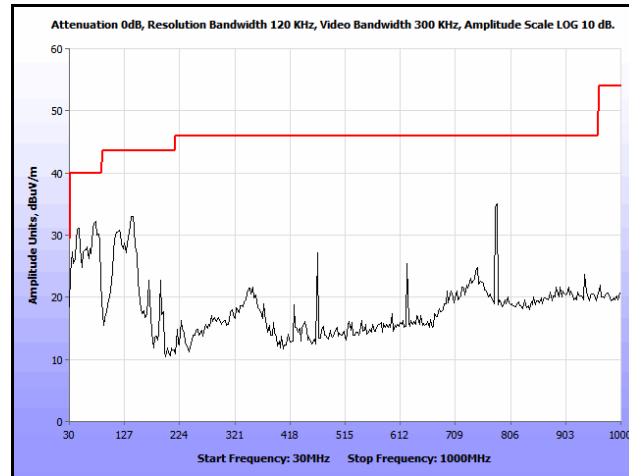
Plot 282. Co-location, Radiated Spurious Emissions, Patch, 802.11n 20 MHz, 2412 & 5200 MHz, 30 MHz – 1 GHz
