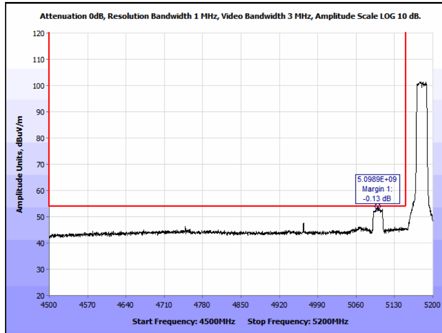
Plot 232. Restricted Band Edge, Patch Antenna, 802.11n 20 MHz, 5180 MHz, Low Channel, Average (4.5 - 5.2 GHz Span)
