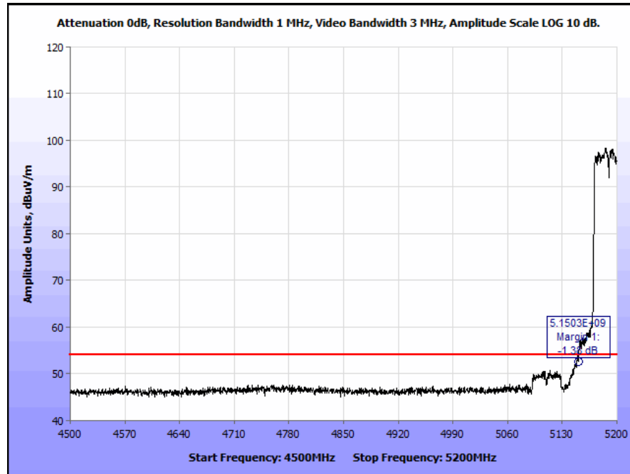
Plot 242. Restricted Band Edge, Ceiling Antenna, 802.11n 40 MHz, 5190 MHz High @ 5150 MHz Edge, Average
