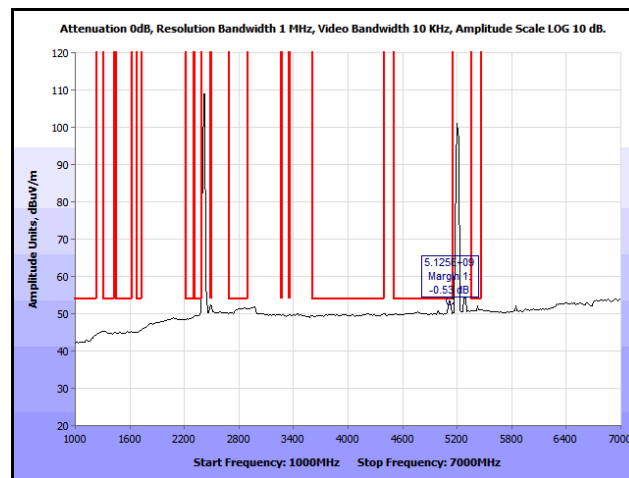
Plot 283. Co-location, Radiated Spurious Emissions, Patch, 802.11n 20 MHz, 2412 & 5200 MHz, 1 GHz – 7 GHz, Average
