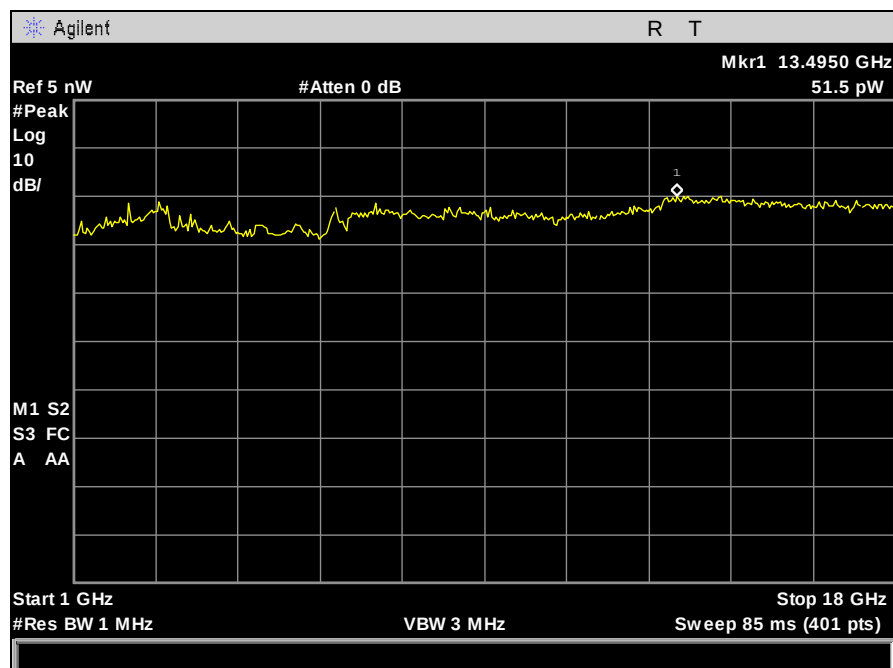
Plot 309. Receiver Spurious Emission, 1 GHz – 18 GHz, Port 2
