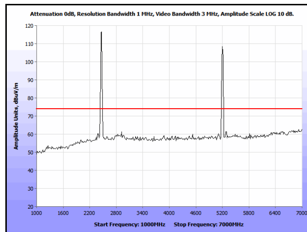
Plot 292. Co-location, Radiated Spurious Emissions, Patch, 802.11n 20 MHz, 2462 & 5200 MHz, 1 GHz – 7 GHz, Peak
