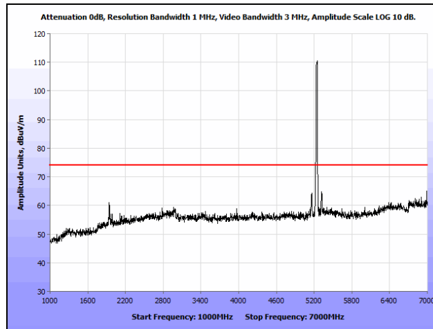
Plot 156. Radiated Spurious Emissions, 802.11n 20 MHz, High Channel, 1 GHz – 7 GHz, Peak, Ceiling
