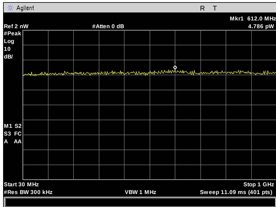
Plot 308. Receiver Spurious Emission, 30 MHz – 1 GHz, Port 2
