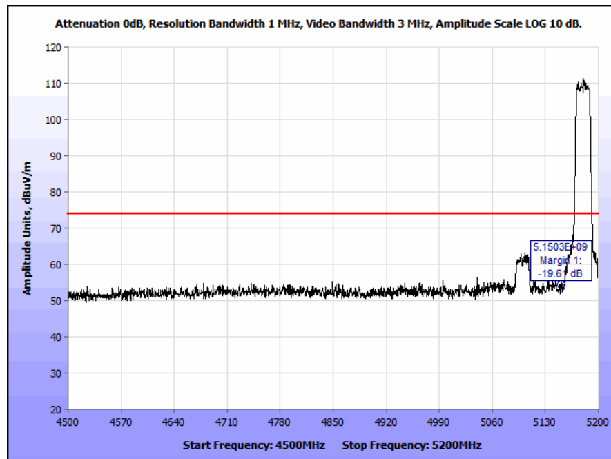
Plot 233. Restricted Band Edge, Patch Antenna, 802.11n 20 MHz, 5180 MHz, Low Channel, Peak (4.5 - 5.2 GHz Span)
