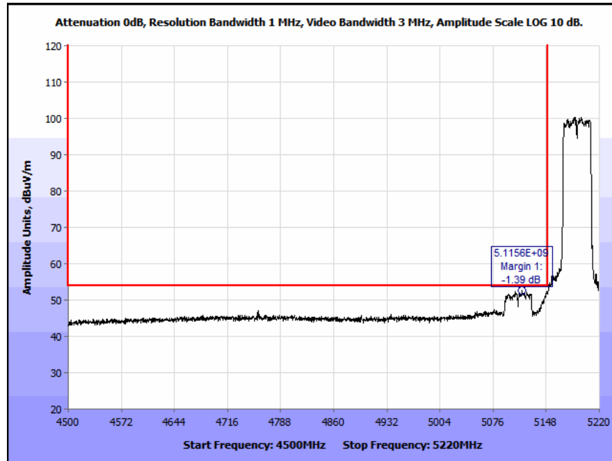
Plot 234. Restricted Band Edge, Patch Antenna, 802.11n 40 MHz, 5190 MHz Low Channel, Average (4.5 - 5.22 GHz Span)
