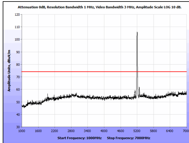
Plot 176. Radiated Spurious Emissions, 802.11a, Mid Channel, 1 GHz – 7 GHz, Peak, Omni
