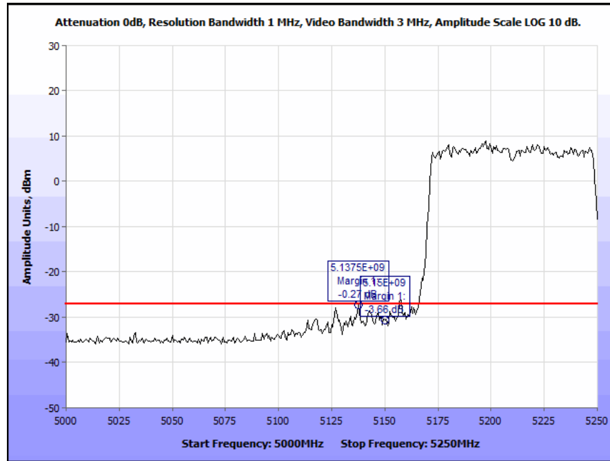
Plot 212. Radiated Band Edge 802.11n 80 MHz, 7 dBi Patch Antenna (Band Edge @ 5150 MHz)
