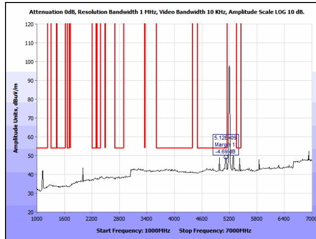
Plot 116. Radiated Spurious Emissions, 802.11n 20 MHz, Mid Channel, 1 GHz – 7 GHz, Peak, 7 dBi Patch
