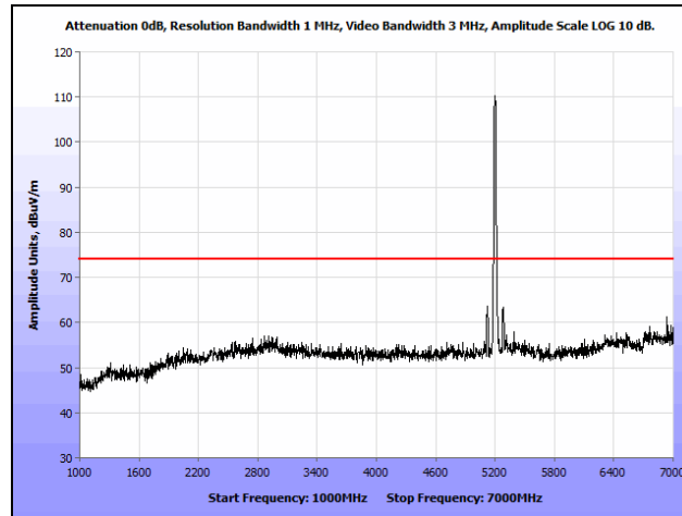
Plot 188. Radiated Spurious Emissions, 802.11n 20 MHz, Mid Channel, 1 GHz – 7 GHz, Peak, Omni
