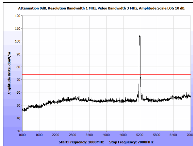
Plot 196. Radiated Spurious Emissions, 802.11n 40 MHz, Low Channel, 1 GHz – 7 GHz, Peak, Omni
