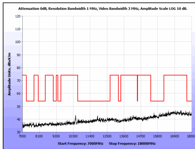
Plot 201. Radiated Spurious Emissions, 802.11n 40 MHz, High Channel, 7 GHz – 18 GHz, Omni
