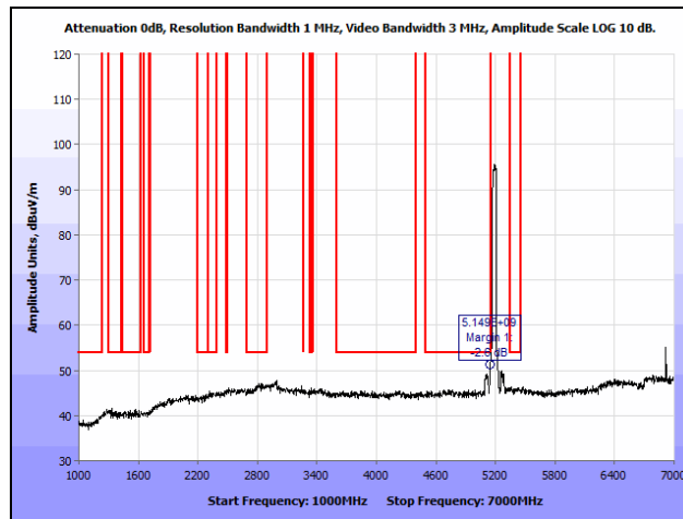
Plot 195. Radiated Spurious Emissions, 802.11n 40 MHz, Low Channel, 1 GHz – 7 GHz, Average, Omni
