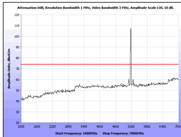
Plot 100. Radiated Spurious Emissions, 802.11a, Low Channel, 1 GHz – 7 GHz, Peak, 7 dBi Patch
