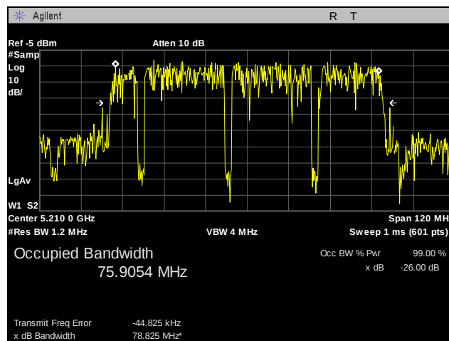
Plot 54. 99% Occupied Bandwidth, 802.11n 80 MHz, Port 2
