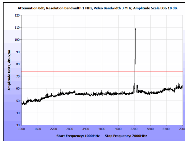
Plot 144. Radiated Spurious Emissions, 802.11a, High Channel, 1 GHz – 7 GHz, Peak, Ceiling
