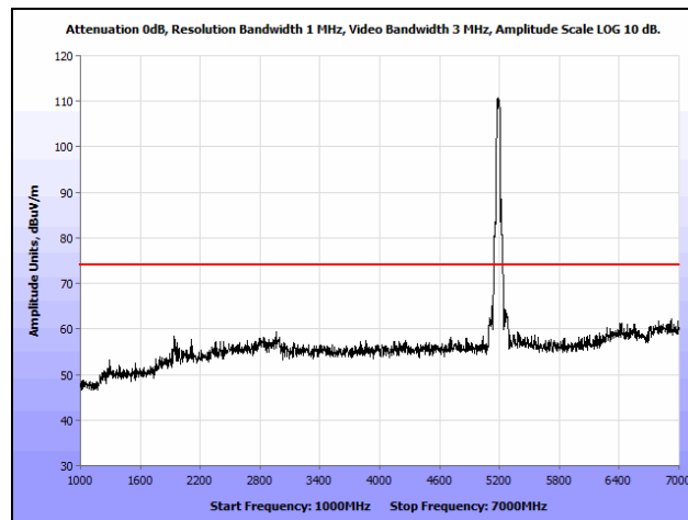
Plot 160. Radiated Spurious Emissions, 802.11n 40 MHz, Low Channel, 1 GHz – 7 GHz, Peak, Ceiling
