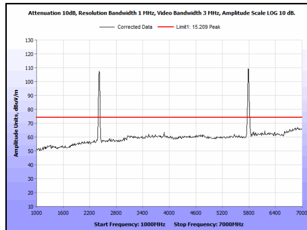
Plot 132. Radiated Spurs, Co-Location, 802.11n 20 MHz, 2412 MHz & 5785 MHz, 1 GHz – 7 GHz, Peak
