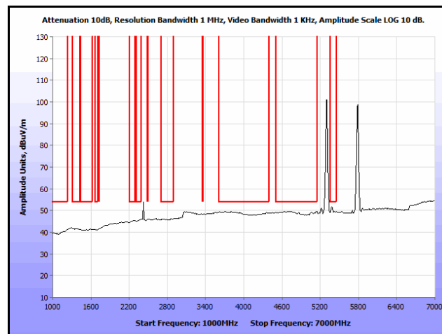
Plot 191. Radiated Spurs, Co-Location, 802.11n 20 MHz, 5300 MHz & 5785 MHz, 1 GHz – 7 GHz, Avg.
