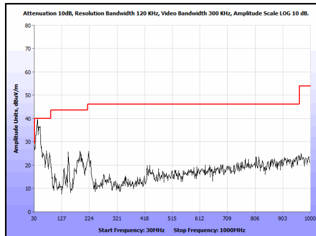
Plot 114. Radiated Spurs, Co-Location, 802.11n 20 MHz, 2462 MHz & 2462 MHz, 30 MHz – 1 GHz, Peak
