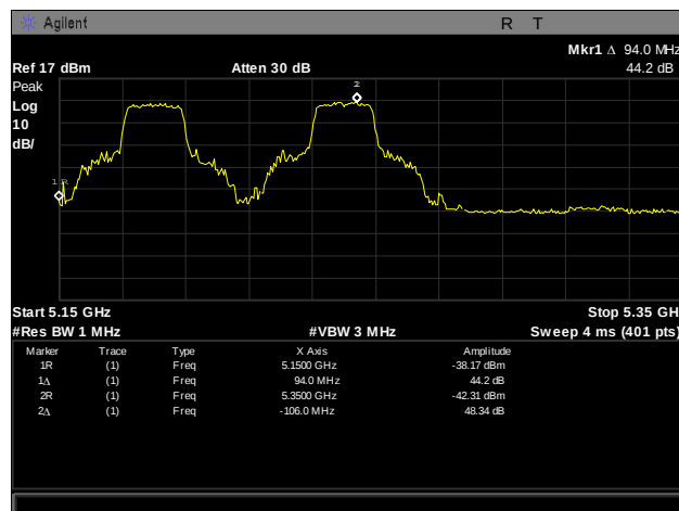
Plot 208. Frequency Stability, 5150 – 5350 MHz, -20°C, 120 V
