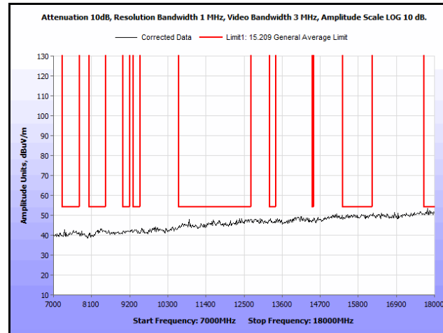
Plot 97. Radiated Spurs, Co-Location, 802.11n 20 MHz, 2412 MHz & 2412 MHz, 7 GHz – 18 GHz, Peak
