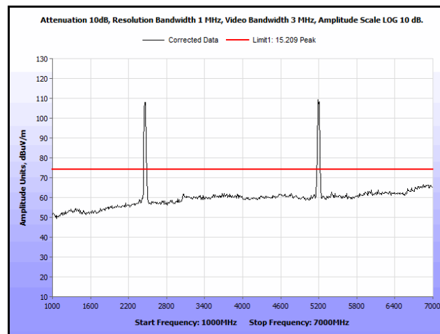
Plot 152. Radiated Spurs, Co-Location, 802.11n 20 MHz, 2462 MHz & 5200 MHz, 1 GHz – 7 GHz, Peak
