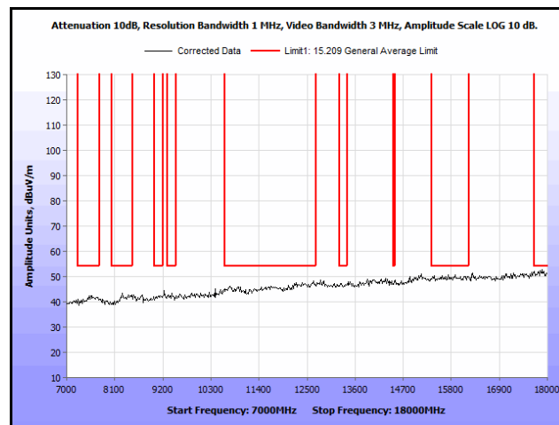
Plot 185. Radiated Spurs, Co-Location, 802.11n 20 MHz, 5300 MHz & 5300 MHz, 7 GHz – 18 GHz, Peak
