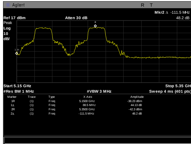
Plot 212. Frequency Stability, 5150 – 5350 MHz, 20°C, 120 V
