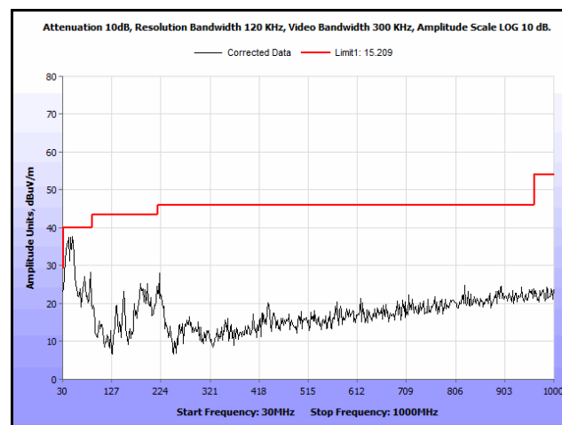
Plot 110. Radiated Spurs, Co-Location, 802.11n 20 MHz, 2437 MHz & 2462 MHz, 30 MHz – 1 GHz, Peak
