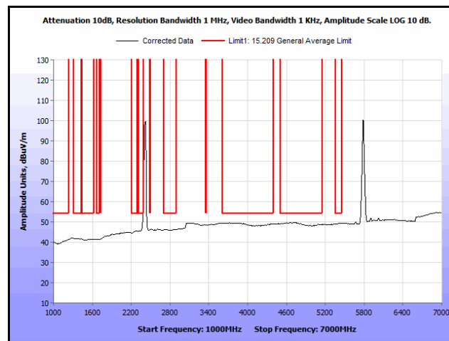
Plot 131. Radiated Spurs, Co-Location, 802.11n 20 MHz, 2412 MHz & 5785 MHz, 1 GHz – 7 GHz, Avg.
