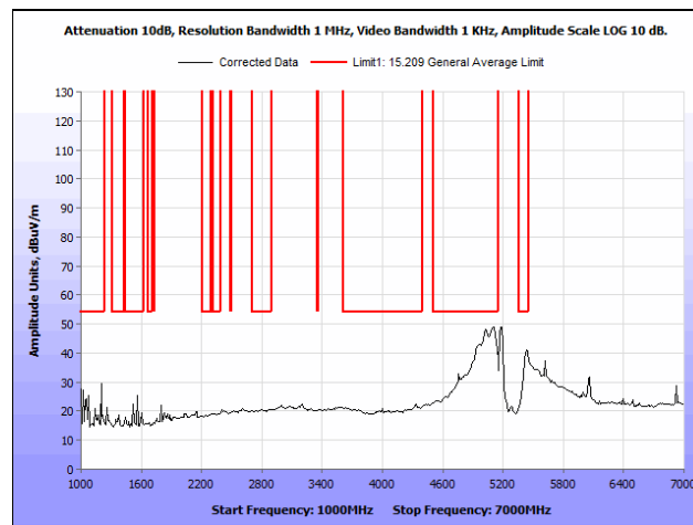
Plot 35. Radiated Spurious Emissions, 802.11a, 40 MHz, Low Channel, 1 GHz – 7 GHz, Average
