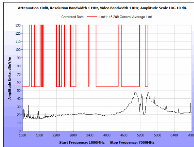
Plot 67. Radiated Spurious Emissions, 802.11n, 40 MHz, High Channel, 1 GHz – 7 GHz
