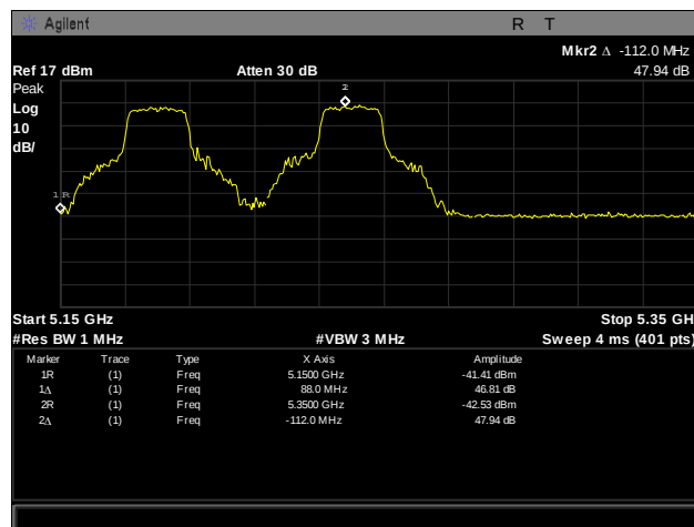
Plot 214. Frequency Stability, 5150 – 5350 MHz, 40°C, 120 V
