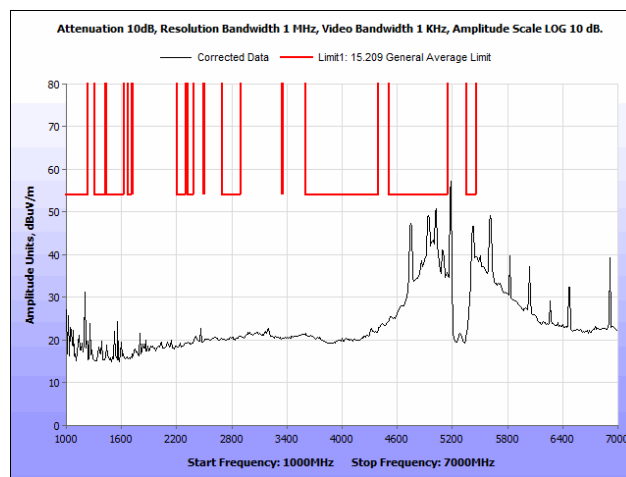
Plot 51. Radiated Spurious Emissions, 802.11n, Low Channel, 1 GHz – 7 GHz, Average
