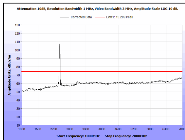
Plot 96. Radiated Spurs, Co-Location, 802.11n 20 MHz, 2412 MHz & 2412 MHz, 1 GHz – 7 GHz, Peak
