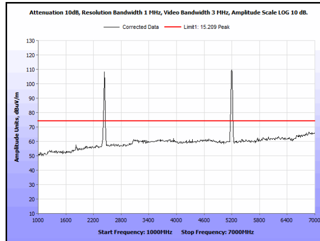
Plot 136. Radiated Spurs, Co-Location, 802.11n 20 MHz, 2437 MHz & 5200 MHz, 1 GHz – 7 GHz, Peak
