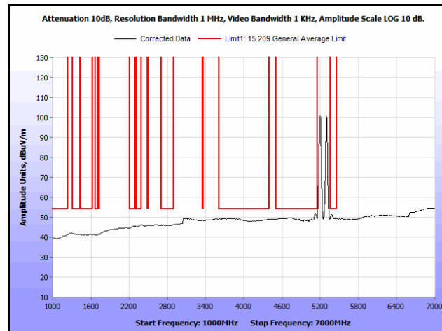
Plot 171. Radiated Spurs, Co-Location, 802.11n 20 MHz, 5200 MHz & 5300 MHz, 1 GHz – 7 GHz, Avg.
