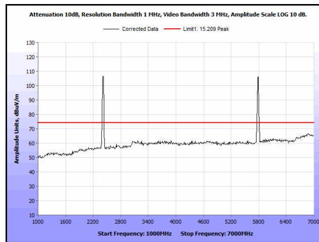
Plot 164. Radiated Spurs, Co-Location, 802.11n 20 MHz, 2462 MHz & 5785 MHz, 1 GHz – 7 GHz, Peak
