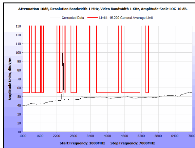
Plot 95. Radiated Spurs, Co-Location, 802.11n 20 MHz, 2412 MHz & 2412 MHz, 1 GHz – 7 GHz, Avg.
