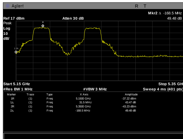
Plot 207. Frequency Stability, 5150 – 5350 MHz, -30°C, 120 V
