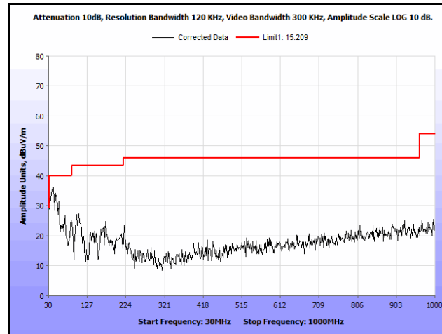
Plot 154. Radiated Spurs, Co-Location, 802.11n 20 MHz, 2462 MHz & 5300 MHz, 30 MHz – 1 GHz, Peak
