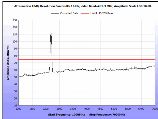
Plot 100. Radiated Spurs, Co-Location, 802.11n 20 MHz, 2412 MHz & 2437 MHz, 1 GHz – 7 GHz, Peak
