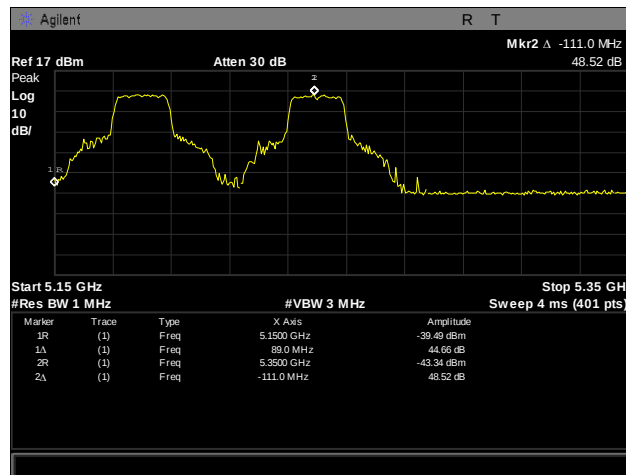
Plot 216. Frequency Stability, 5150 – 5350 MHz, 55°C, 120 V
