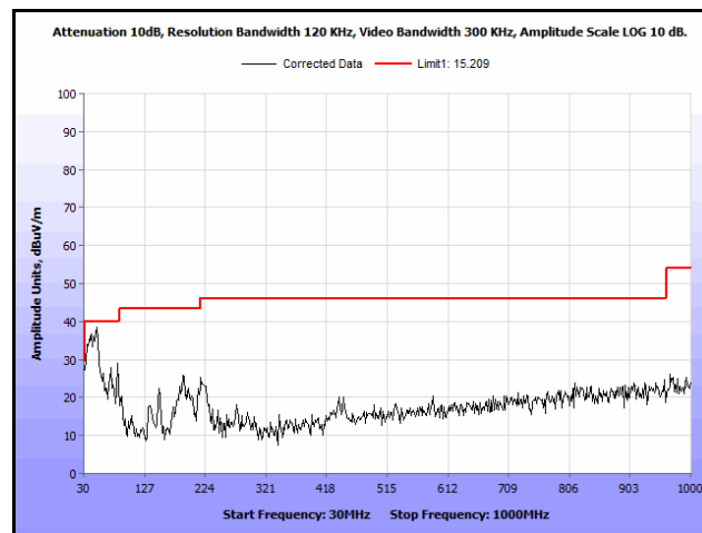
Plot 170. Radiated Spurs, Co-Location, 802.11n 20 MHz, 5200 MHz & 5300 MHz, 30 MHz – 1 GHz, Peak
