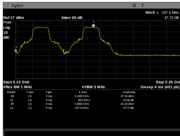
Plot 213. Frequency Stability, 5150 – 5350 MHz, 30°C, 120 V
