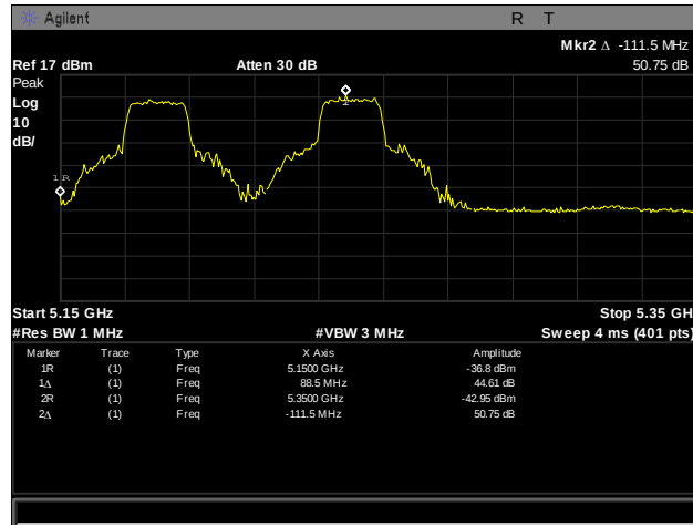
Plot 209. Frequency Stability, 5150 – 5350 MHz, -10°C, 120 V
