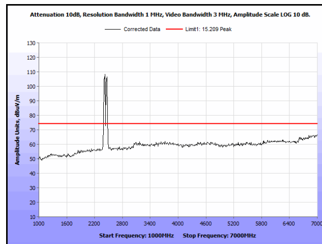
Plot 104. Radiated Spurs, Co-Location, 802.11n 20 MHz, 2412 MHz & 2462 MHz, 1 GHz – 7 GHz, Peak
