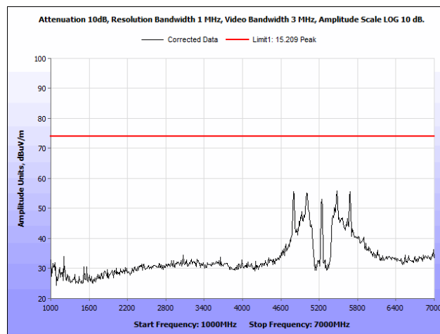
Plot 44. Radiated Spurious Emissions, 802.11a, High Channel, 1 GHz – 7 GHz, Peak
