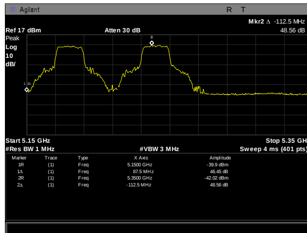
Plot 210. Frequency Stability, 5150 – 5350 MHz, 0°C, 120 V
