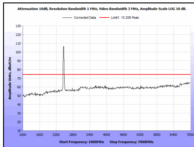
Plot 116. Radiated Spurs, Co-Location, 802.11n 20 MHz, 2462 MHz & 2462 MHz, 1 GHz – 7 GHz, Peak
