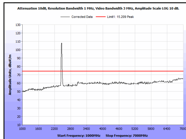
Plot 108. Radiated Spurs, Co-Location, 802.11n 20 MHz, 2437 MHz & 2437 MHz, 1 GHz – 7 GHz, Peak
