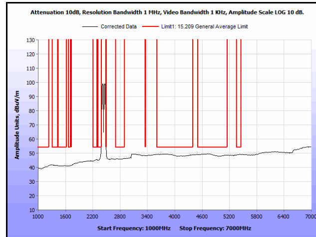
Plot 103. Radiated Spurs, Co-Location, 802.11n 20 MHz, 2412 MHz & 2462 MHz, 1 GHz – 7 GHz, Avg.
