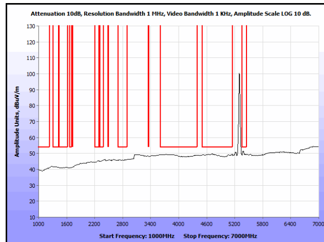
Plot 183. Radiated Spurs, Co-Location, 802.11n 20 MHz, 5300 MHz & 5300 MHz, 1 GHz – 7 GHz, Avg.
