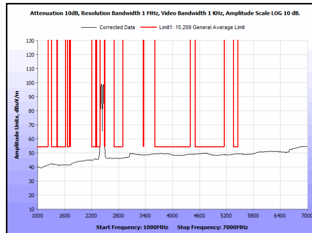
Plot 99. Radiated Spurs, Co-Location, 802.11n 20 MHz, 2412 MHz & 2437 MHz, 1 GHz – 7 GHz, Avg.
