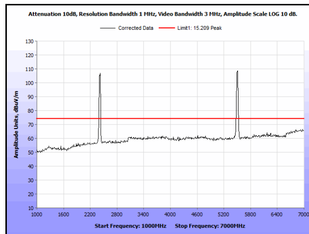
Plot 128. Radiated Spurs, Co-Location, 802.11n 20 MHz, 2412 MHz & 5580 MHz, 1 GHz – 7 GHz, Peak
