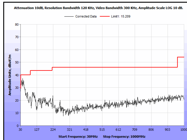
Plot 198. Radiated Spurs, Co-Location, 802.11n 20 MHz, 5580 MHz & 5785 MHz, 30 MHz – 1 GHz, Peak
