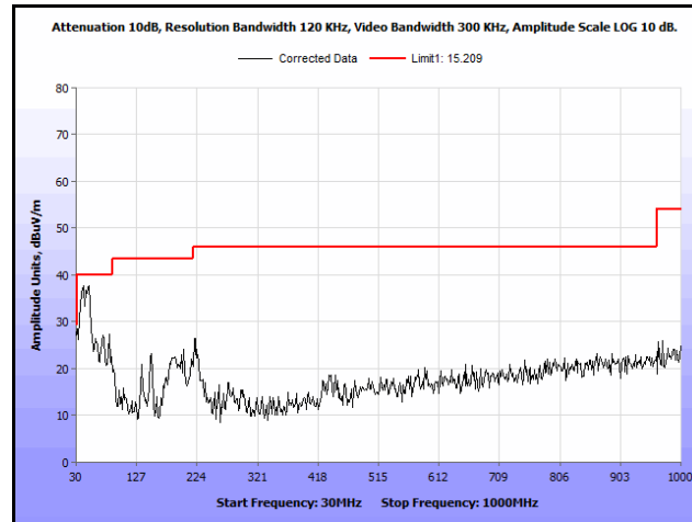
Plot 130. Radiated Spurs, Co-Location, 802.11n 20 MHz, 2412 MHz & 5785 MHz, 30 MHz – 1 GHz, Peak
