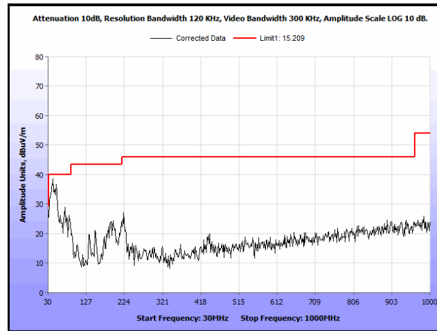
Plot 118. Radiated Spurs, Co-Location, 802.11n 20 MHz, 2412 MHz & 5200 MHz, 30 MHz – 1 GHz, Peak
