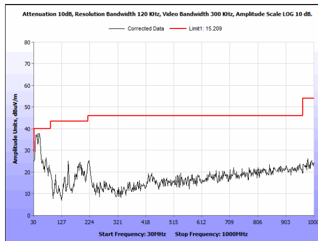
Plot 38. Radiated Spurious Emissions, 802.11a, 20 MHz, Mid Channel, 30 MHz – 1 GHz
