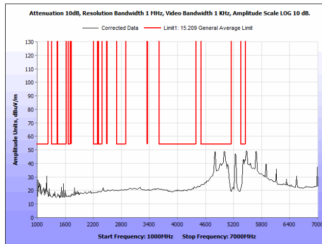
Plot 63. Radiated Spurious Emissions, 802.11n, High Channel, 1 GHz – 7 GHz, Average
