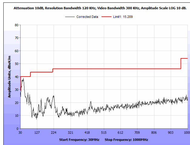
Plot 34. Radiated Spurious Emissions, 802.11a, 40 MHz, Low Channel, 30 MHz – 1 GHz
