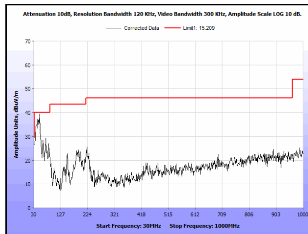
Plot 122. Radiated Spurs, Co-Location, 802.11n 20 MHz, 2412 MHz & 5300 MHz, 30 MHz – 1 GHz, Peak
