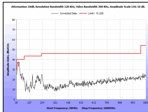
Plot 98. Radiated Spurs, Co-Location, 802.11n 20 MHz, 2412 MHz & 2437 MHz, 30 MHz – 1 GHz, Peak
