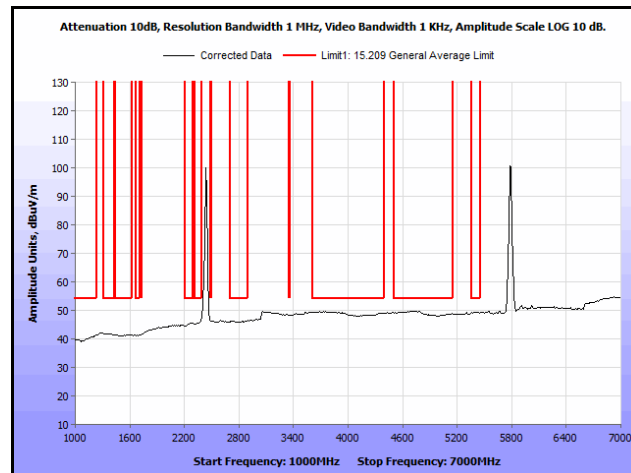
Plot 147. Radiated Spurs, Co-Location, 802.11n 20 MHz, 2437 MHz & 5785 MHz, 1 GHz – 7 GHz, Avg.
