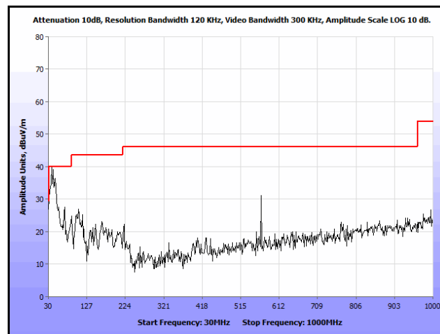
Plot 146. Radiated Spurs, Co-Location, 802.11n 20 MHz, 2437 MHz & 5785 MHz, 30 MHz – 1 GHz, Peak
