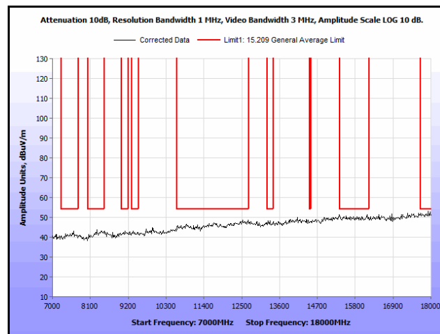
Plot 173. Radiated Spurs, Co-Location, 802.11n 20 MHz, 5200 MHz & 5300 MHz, 7 GHz – 18 GHz, Peak
