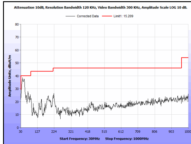
Plot 94. Radiated Spurs, Co-Location, 802.11n 20 MHz, 2412 MHz & 2412 MHz, 30 MHz – 1 GHz, Peak
