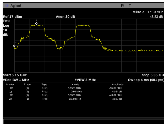
Plot 211. Frequency Stability, 5150 – 5350 MHz, 10°C, 120 V
