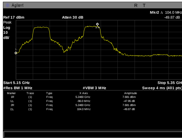
Plot 206. Frequency Stability, 5150 – 5350 MHz, -40°C, 120 V
