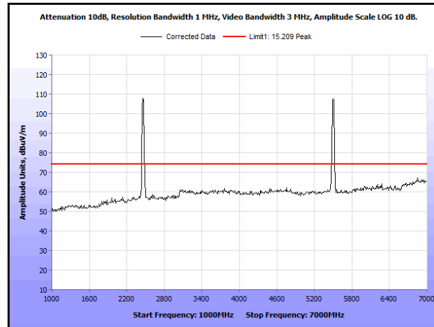
Plot 160. Radiated Spurs, Co-Location, 802.11n 20 MHz, 2462 MHz & 5580 MHz, 1 GHz – 7 GHz, Peak
