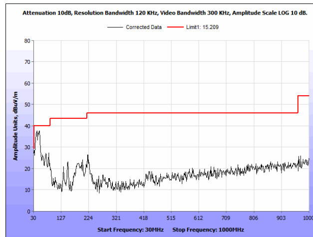
Plot 66. Radiated Spurious Emissions, 802.11n, 40 MHz, High Channel, 30 MHz – 1 GHz
