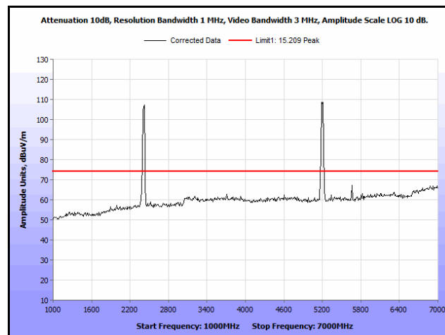
Plot 120. Radiated Spurs, Co-Location, 802.11n 20 MHz, 2412 MHz & 5200 MHz, 1 GHz – 7 GHz, Peak
