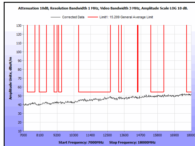
Plot 105. Radiated Spurs, Co-Location, 802.11n 20 MHz, 2412 MHz & 2462 MHz, 7 GHz – 18 GHz, Peak
