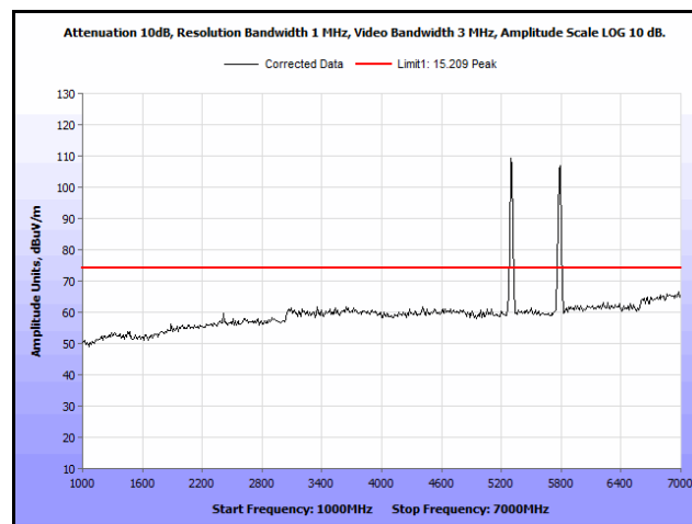
Plot 192. Radiated Spurs, Co-Location, 802.11n 20 MHz, 5300 MHz & 5785 MHz, 1 GHz – 7 GHz, Peak
