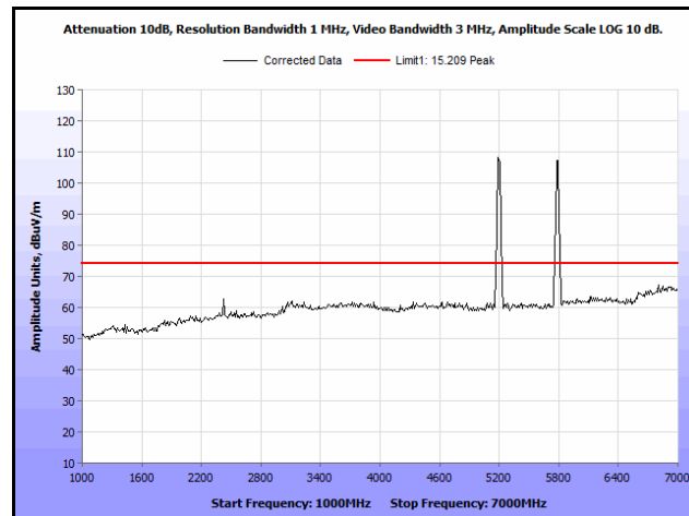
Plot 180. Radiated Spurs, Co-Location, 802.11n 20 MHz, 5200 MHz & 5785 MHz, 1 GHz – 7 GHz, Peak
