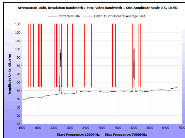
Plot 135. Radiated Spurs, Co-Location, 802.11n 20 MHz, 2437 MHz & 5200 MHz, 1 GHz – 7 GHz, Avg.
