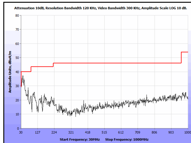
Plot 138. Radiated Spurs, Co-Location, 802.11n 20 MHz, 2437 MHz & 5300 MHz, 30 MHz – 1 GHz, Peak
