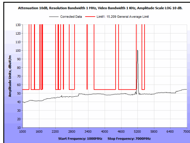
Plot 167. Radiated Spurs, Co-Location, 802.11n 20 MHz, 5200 MHz & 5200 MHz, 1 GHz – 7 GHz, Avg.
