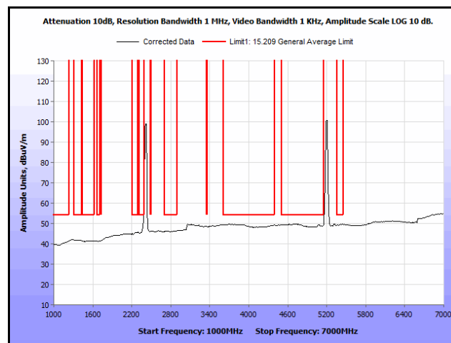
Plot 119. Radiated Spurs, Co-Location, 802.11n 20 MHz, 2412 MHz & 5200 MHz, 1 GHz – 7 GHz, Avg.
