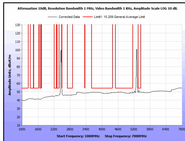
Plot 155. Radiated Spurs, Co-Location, 802.11n 20 MHz, 2462 MHz & 5300 MHz, 1 GHz – 7 GHz, Avg.
