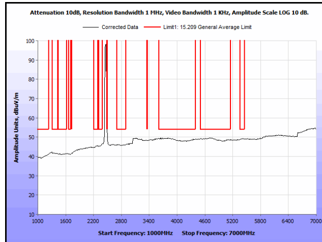
Plot 115. Radiated Spurs, Co-Location, 802.11n 20 MHz, 2462 MHz & 2462 MHz, 1 GHz – 7 GHz, Avg.
