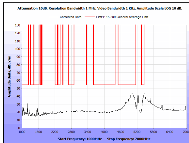
Plot 47. Radiated Spurious Emissions, 802.11a, 40 MHz, High Channel, 1 GHz – 7 GHz, Average
