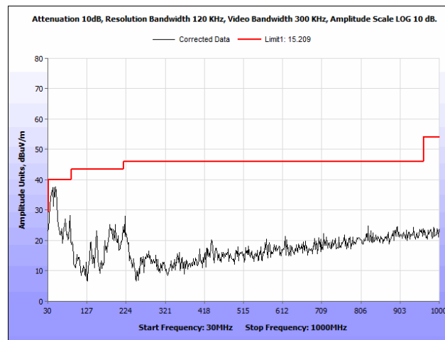
Plot 46. Radiated Spurious Emissions, 802.11a, 40 MHz, High Channel, 30 MHz – 1 GHz
