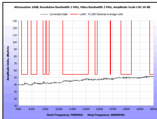
Plot 113. Radiated Spurs, Co-Location, 802.11n 20 MHz, 2437 MHz & 2462 MHz, 7 GHz – 18 GHz, Peak
