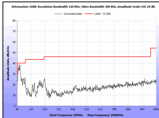
Plot 102. Radiated Spurs, Co-Location, 802.11n 20 MHz, 2412 MHz & 2462 MHz, 30 MHz – 1 GHz, Peak
