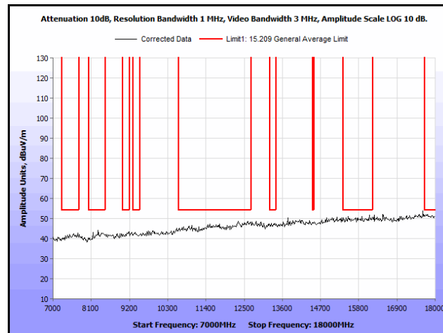
Plot 177. Radiated Spurs, Co-Location, 802.11n 20 MHz, 5200 MHz & 5580 MHz, 7 GHz – 18 GHz, Peak
