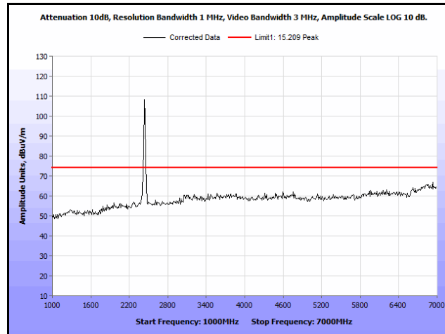
Plot 112. Radiated Spurs, Co-Location, 802.11n 20 MHz, 2437 MHz & 2462 MHz, 1 GHz – 7 GHz, Peak
