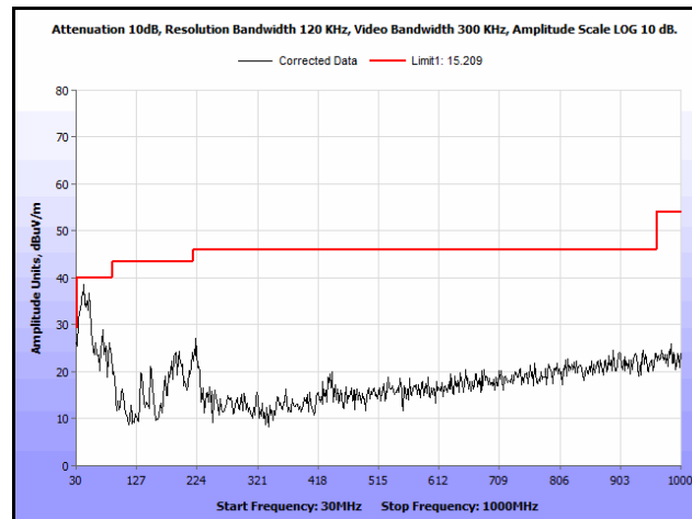
Plot 174. Radiated Spurs, Co-Location, 802.11n 20 MHz, 5200 MHz & 5580 MHz, 30 MHz – 1 GHz, Peak
