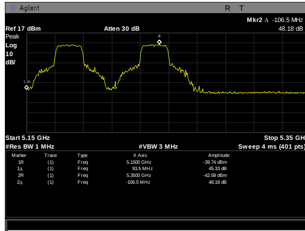
Plot 215. Frequency Stability, 5150 – 5350 MHz, 50°C, 120 V
