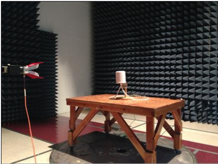
Photograph 8. Radiated Spurious Emissions, Test Setup, Above 1 GHz, Omni Antenna
