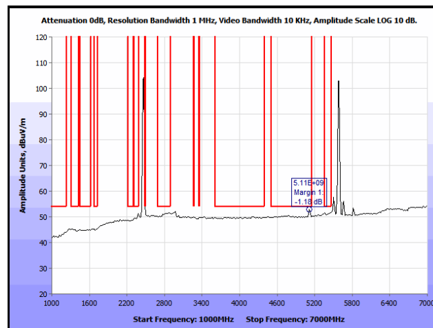
Plot 576. Co-location, Radiated Spurious Emissions, Patch, 802.11n 20 MHz, 2462 & 5580 MHz, 1 GHz – 7 GHz, Average
