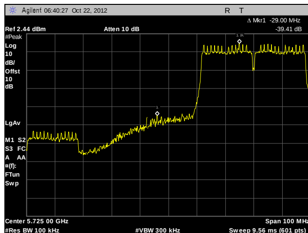
Plot 718. Conducted Band Edge, 802.11n 40 MHz, 5755 MHz Low Channel, Port 1
