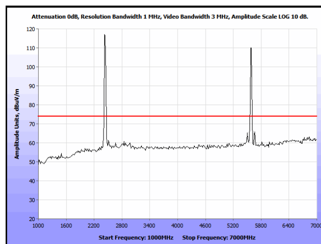
Plot 561. Co-location, Radiated Spurious Emissions, Patch, 802.11n 20 MHz, 2437 & 5580 MHz, 1 GHz – 7 GHz, Peak
