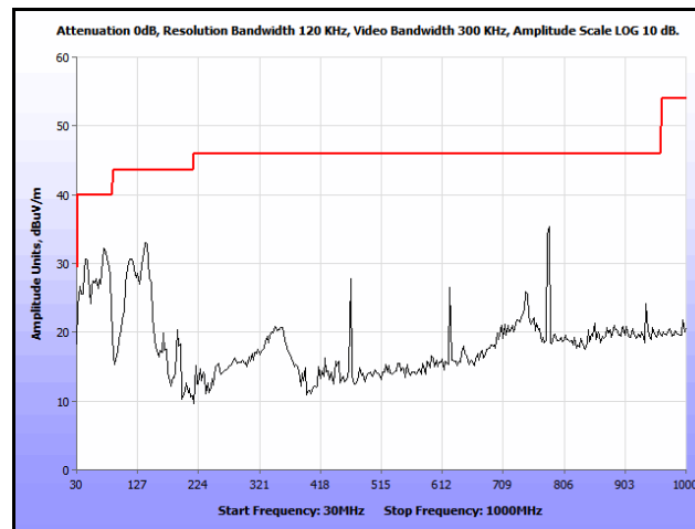
Plot 547. Co-location, Radiated Spurious Emissions, Patch, 802.11n 20 MHz, 2412 & 5785 MHz, 30 MHz – 1 GHz
