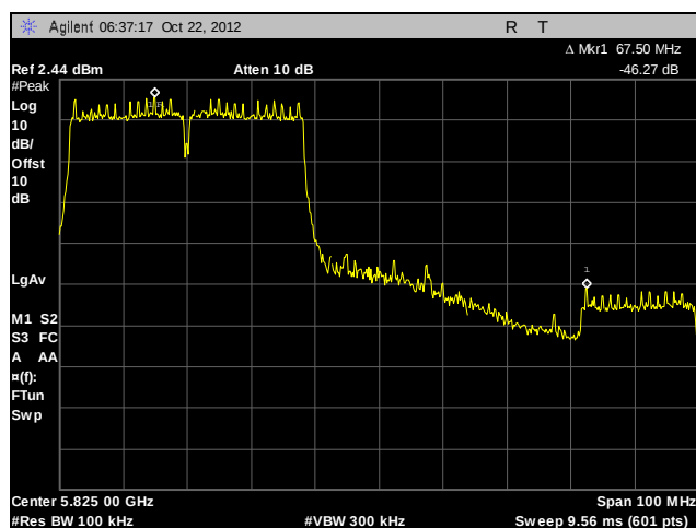
Plot 723. Conducted Band Edge, 802.11n 40 MHz, 5795 MHz, High Channel, Port 3
