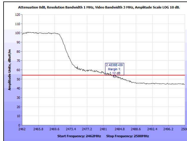
Plot 381. Restricted Band Edge, Omni Antenna, 802.11n 20 MHz, 2462 MHz @ 2483.5 MHz, Average
