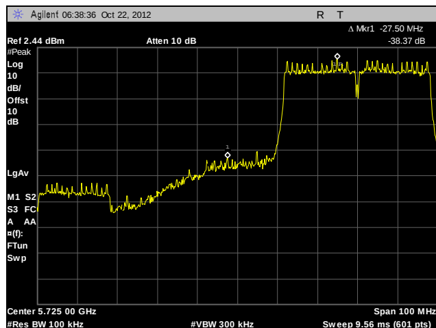
Plot 722. Conducted Band Edge, 802.11n 40 MHz, 5755 MHz, Low Channel, Port 3
