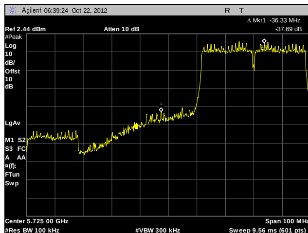
Plot 720. Conducted Band Edge, 802.11n 40 MHz, 5755 MHz, Low Channel, Port 2
