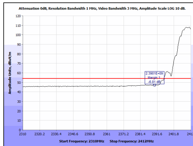
Plot 391. Restricted Band Edge, Patch Antenna, 802.11b 20 MHz, 2412 MHz @ 2390 MHz, Average
