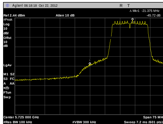
Plot 712. Conducted Band Edge, 802.11n 20 MHz, 5745 MHz, Low Channel, Port 1
