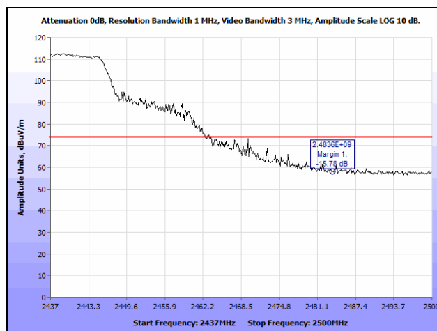
Plot 380. Restricted Band Edge, Omni Antenna, 802.11n 20 MHz, 2437 MHz @ 2483.5 MHz, Peak, Channel 6
