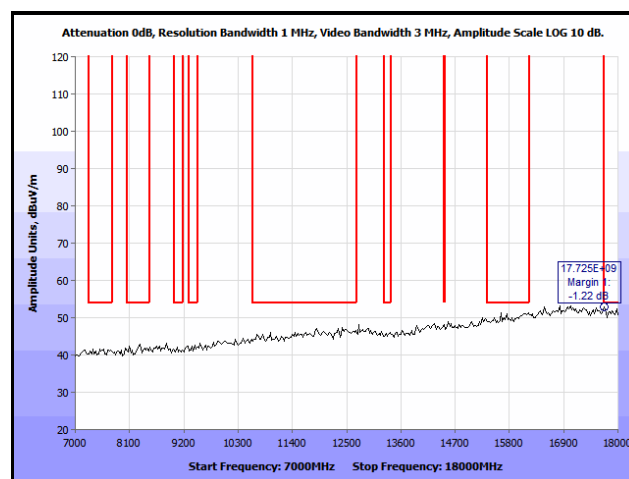
Plot 570. Co-location, Radiated Spurious Emissions, Patch, 802.11n 20 MHz, 2462 & 5200 MHz, 7 GHz – 18 GHz, Peak
