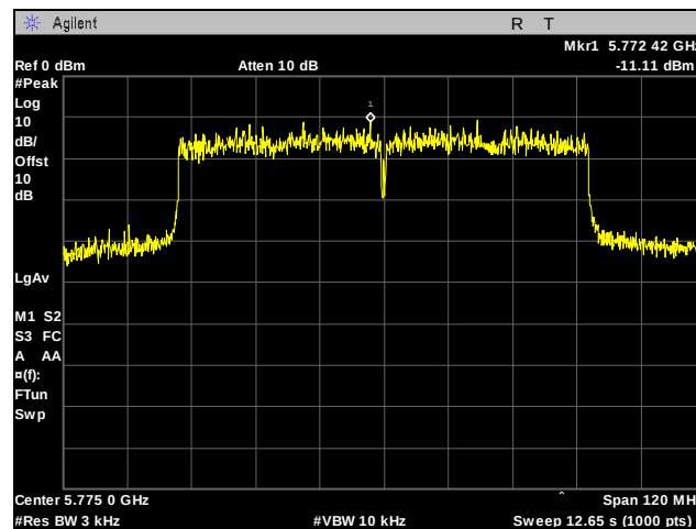
Plot 772. Power Spectral Density, 802.11n 80 MHz, 5775 MHz, Port 1
