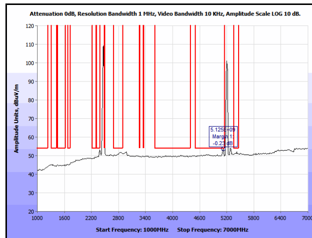
Plot 568. Co-location, Radiated Spurious Emissions, Patch, 802.11n 20 MHz, 2462 & 5200 MHz, 1 GHz – 7 GHz, Average
