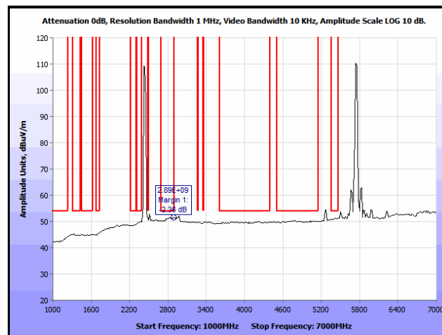
Plot 564. Co-location, Radiated Spurious Emissions, Patch, 802.11n 20 MHz, 2437 & 5785 MHz, 1 GHz – 7 GHz, Average
