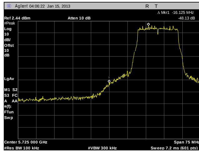
Plot 710. Conducted Band Edge, 802.11a 20 MHz, 5745 MHz, Low Channel, Port 1
