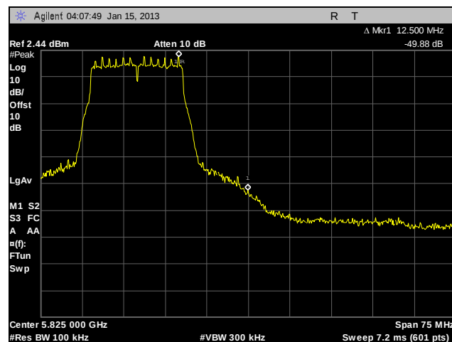
Plot 711. Conducted Band Edge, 802.11a 20 MHz, 5805 MHz, High Channel, Port 1
