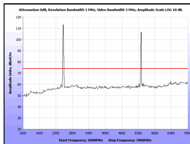
Plot 485. Co-location, Radiated Spurious Emissions, Omni, 802.11n 20 MHz, 2462 & 5300 MHz, 1 GHz – 7 GHz, Peak
