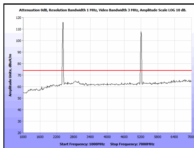
Plot 537. Co-location, Radiated Spurious Emissions, Patch, 802.11n 20 MHz, 2412 & 5200 MHz, 1 GHz – 7 GHz, Peak
