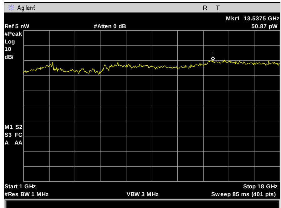
Plot 776. Receiver Spurious Emission, 1 GHz – 18 GHz, Port 1
