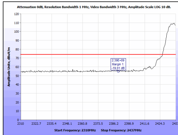
Plot 378. Restricted Band Edge, Omni Antenna, 802.11n 20 MHz, 2437 MHz @ 2390 MHz, Peak, Channel 6
