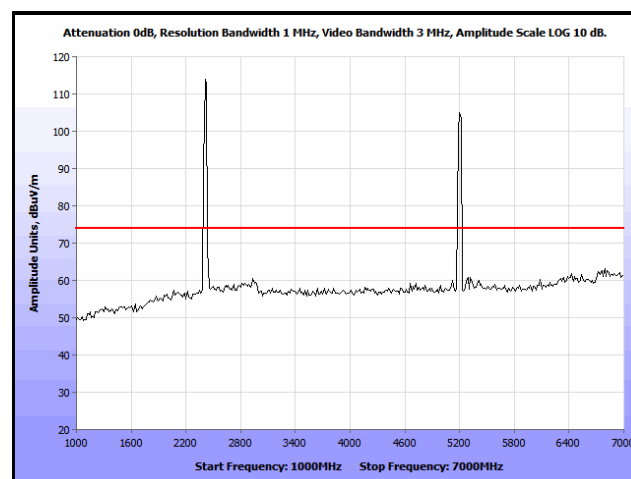
Plot 449. Co-location, Radiated Spurious Emissions, Omni, 802.11n 20 MHz, 2412 & 5200 MHz, 1 GHz – 7 GHz, Peak
