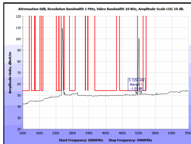
Plot 552. Co-location, Radiated Spurious Emissions, Patch, 802.11n 20 MHz, 2437 & 5200 MHz, 1 GHz – 7 GHz, Average
