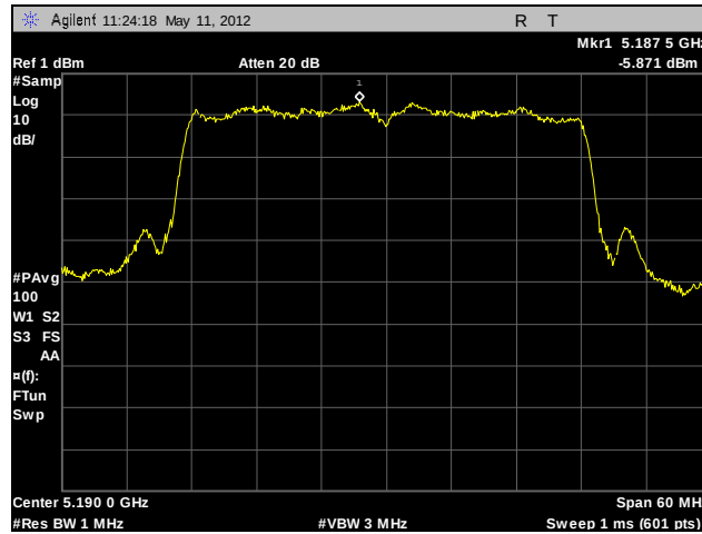
Plot 76. Power Spectral Density, Low Channel, 802.11n 40 MHz (A4)
