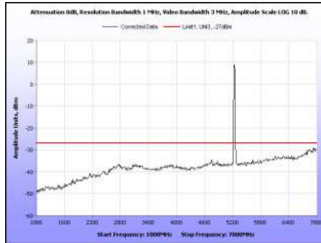
Plot 121. Radiated Spurious Emissions, 802.11n 20 MHz, High Channel, 1 GHz – 7 GHz
