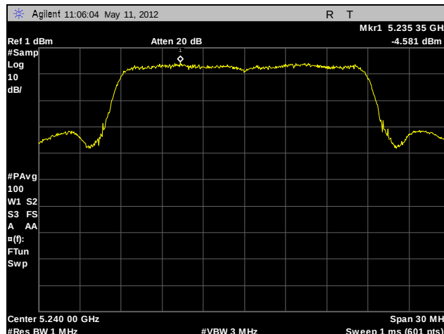
Plot 75. Power Spectral Density, High Channel, 802.11n 20 MHz (A6)
