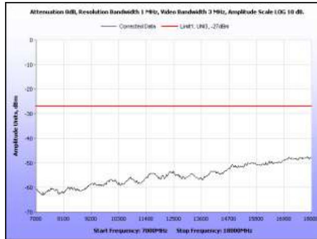
Plot 130. Radiated Spurious Emissions, 802.11n 40 MHz, High Channel, 7 GHz – 18 GHz
