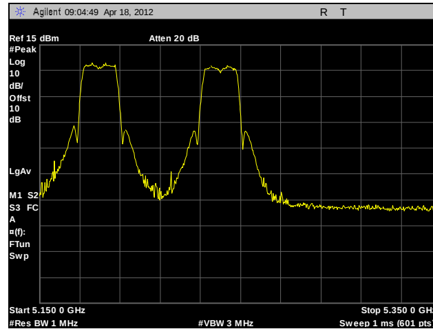
Plot 150. Frequency Stability, 5150 – 5250 MHz, 20°C, 120 V
