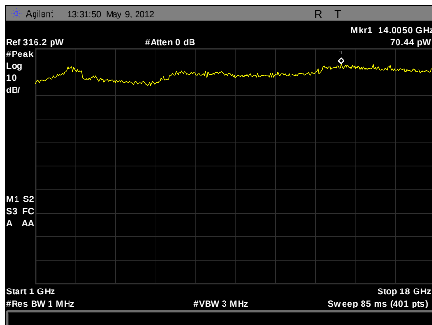
Plot 161. Receiver Spurious Emission, 1 GHz – 18 GHz (Port 3)
