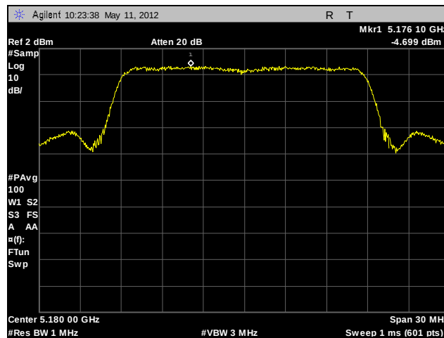
Plot 67. Power Spectral Density, Low Channel, 802.11n 20 MHz (A4)
