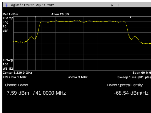
Plot 63. RF Power Output, High Channel, 802.11n 40 MHz (A6)
