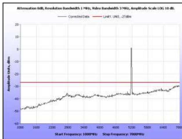
Plot 101. Radiated Spurious Emissions, 802.11a, Low Channel, 1 GHz – 7 GHz
