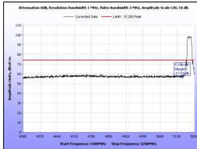
Plot 139. Radiated Band Edge, 802.11a, Low Channel, Peak
