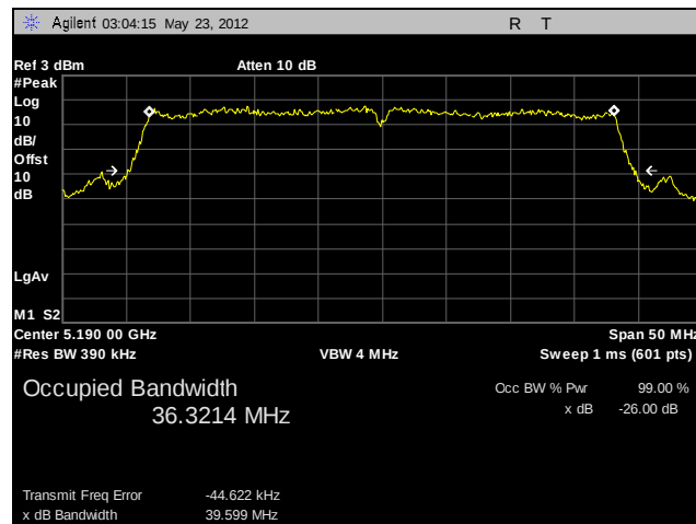
Plot 22. 26 dB Occupied Bandwidth, Low Channel, 802.11n 40 MHz (A4)
