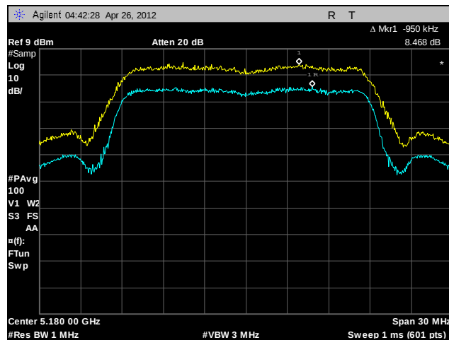
Plot 88. Peak Excursion Ratio, Low Channel, 802.11n 20 MHz (A5)
