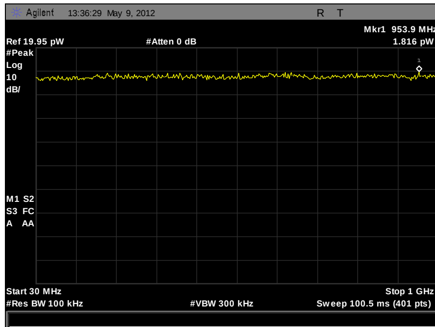
Plot 156. Receiver Spurious Emission, 30 MHz – 1 GHz (Port 1)
