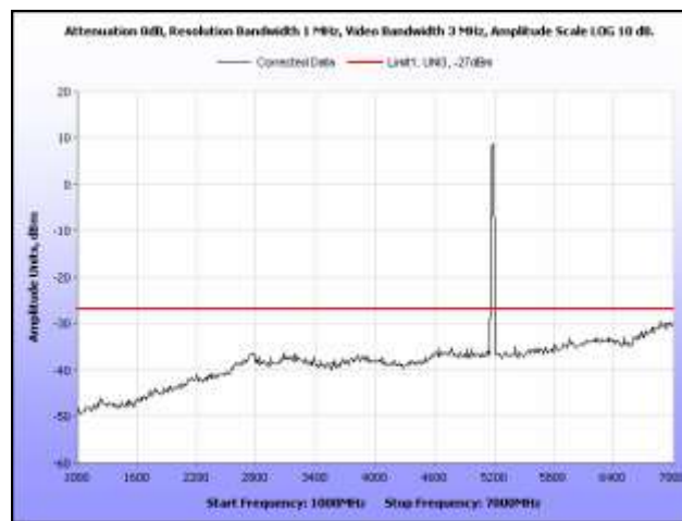
Plot 113. Radiated Spurious Emissions, 802.11n 20 MHz, Low Channel, 1 GHz – 7 GHz
