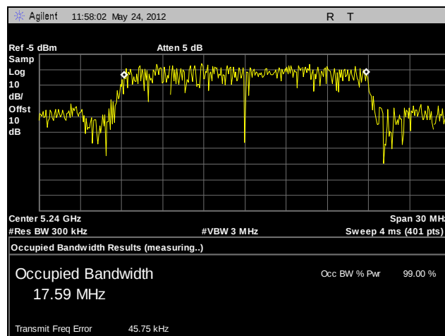
Plot 39. 99% Occupied Bandwidth, High Channel, 802.11n 20 MHz (A6)
