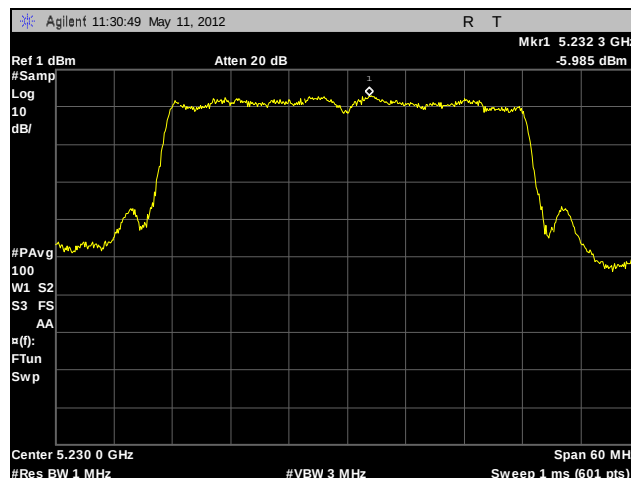
Plot 80. Power Spectral Density, High Channel, 802.11n 40 MHz (A5)
