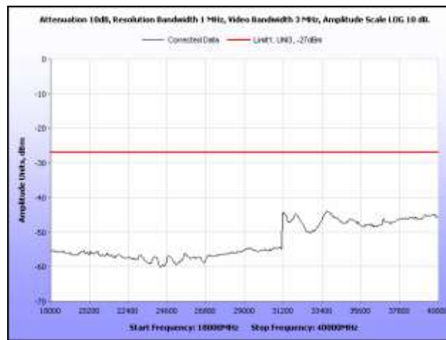
Plot 131. Radiated Spurious Emissions, 802.11n 40 MHz, High Channel, 18 GHz – 40 GHz
