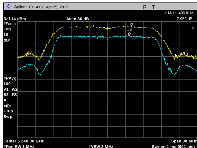
Plot 84. Peak Excursion Ratio, High Channel, 802.11a
