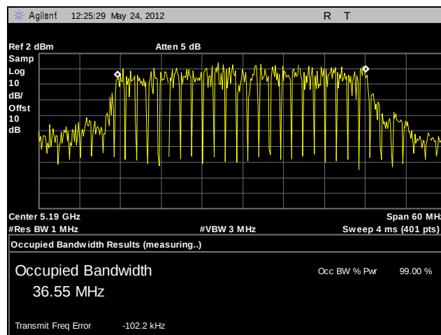
Plot 41. 99% Occupied Bandwidth, Low Channel, 802.11n 40 MHz (A5)
