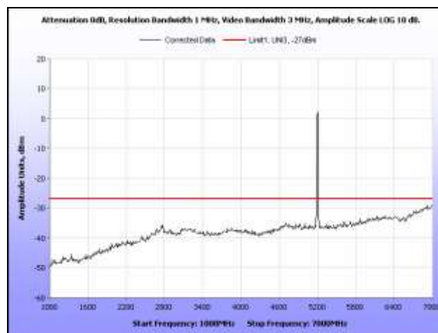
Plot 105. Radiated Spurious Emissions, 802.11a, Mid Channel, 1 GHz – 7 GHz
