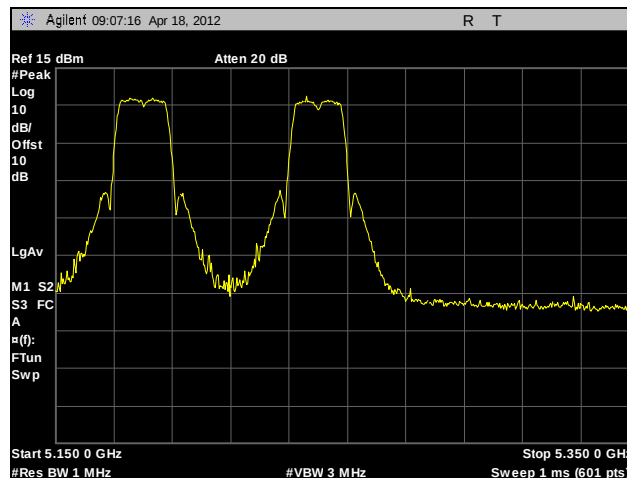
Plot 149. Frequency Stability, 5150 – 5250 MHz, 20°C, 108 V
