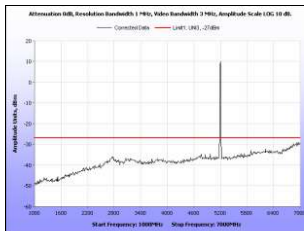
Plot 117. Radiated Spurious Emissions, 802.11n 20 MHz, Mid Channel, 1 GHz – 7 GHz
