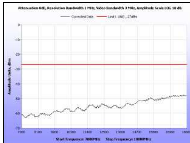
Plot 114. Radiated Spurious Emissions, 802.11n 20 MHz, Low Channel, 7 GHz – 18 GHz
