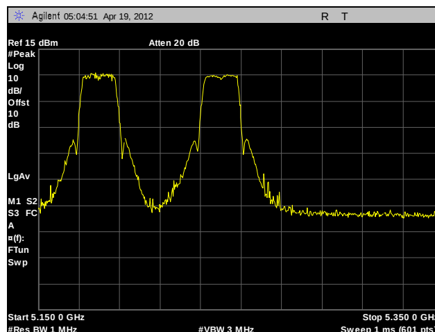
Plot 146. Frequency Stability, 5150 – 5250 MHz, -10°C, 120 V
