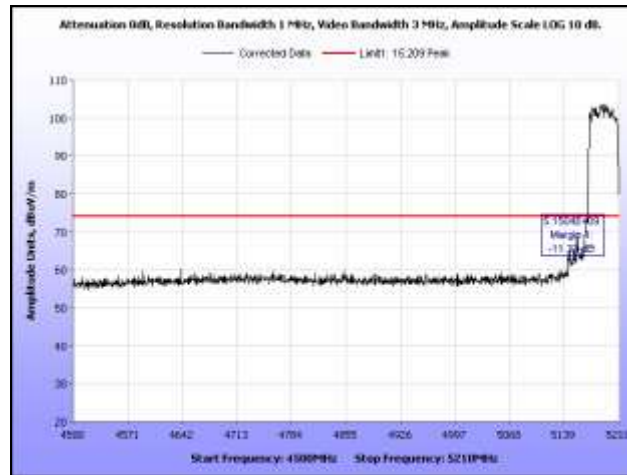
Plot 143. Radiated Band Edge, 802.11n 40 MHz, Low Channel, Peak
