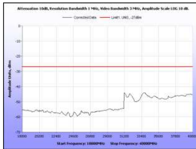
Plot 119. Radiated Spurious Emissions, 802.11n 20 MHz, Mid Channel, 18 GHz – 40 GHz
