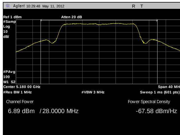
Plot 51. RF Power Output, Low Channel, 802.11n 20 MHz (A6)
