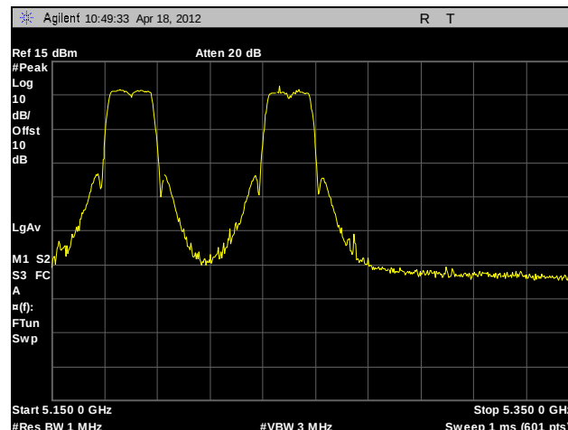
Plot 155. Frequency Stability, 5150 – 5250 MHz, 55°C, 120 V
