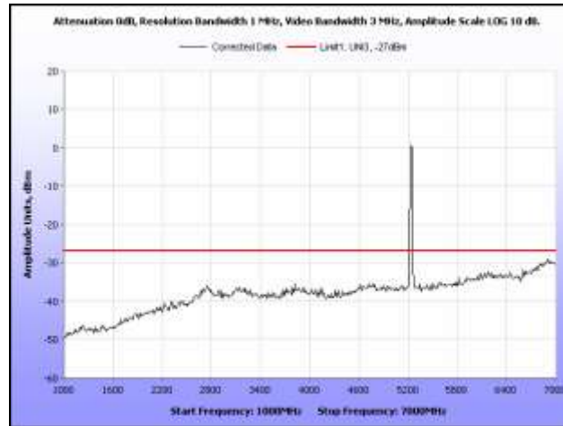
Plot 109. Radiated Spurious Emissions, 802.11a, High Channel, 1 GHz – 7 GHz
