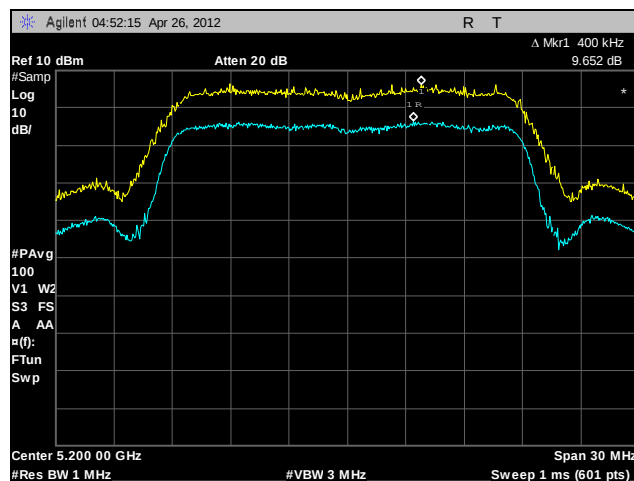
Plot 92. Peak Excursion Ratio, Mid Channel, 802.11n 20 MHz (A6)
