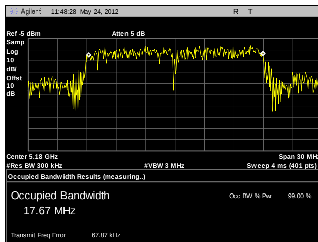
Plot 32. 99% Occupied Bandwidth, Low Channel, 802.11n 20 MHz (A5)
