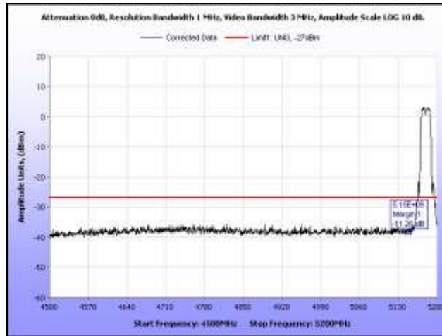
Plot 132. Radiated Band Edge, 802.11a, Low Channel
