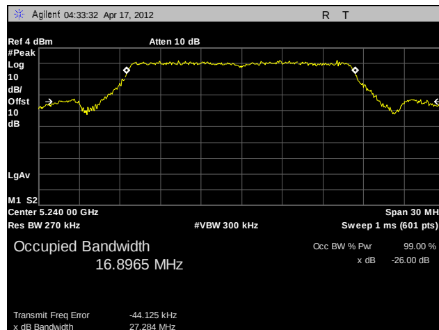
Plot 12. 26 dB Occupied Bandwidth, High Channel, 802.11a
