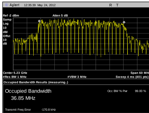
Plot 43. 99% Occupied Bandwidth, High Channel, 802.11n 40 MHz (A4)
