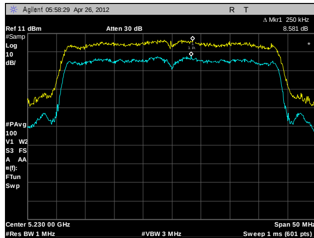
Plot 99. Peak Excursion Ratio, High Channel, 802.11n 40 MHz (A6)
