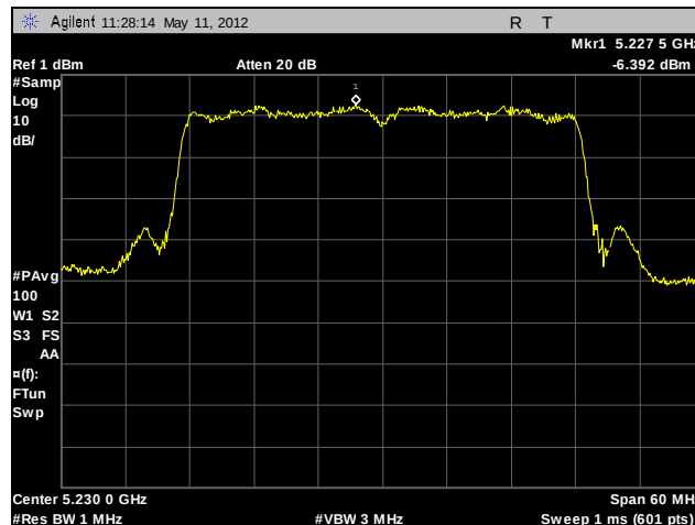
Plot 81. Power Spectral Density, High Channel, 802.11n 40 MHz (A6)
