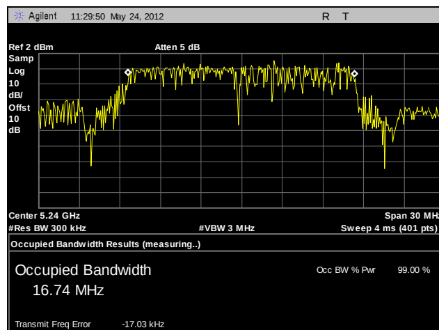
Plot 30. 99% Occupied Bandwidth, High Channel, 802.11a
