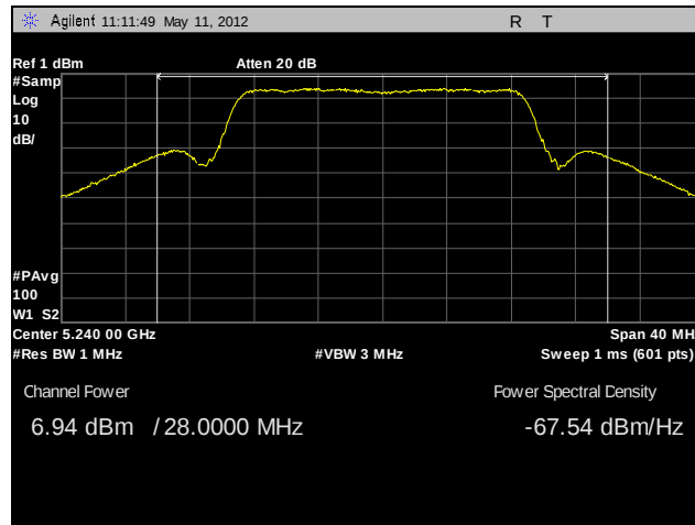
Plot 55. RF Power Output, High Channel, 802.11n 20 MHz (A4)
