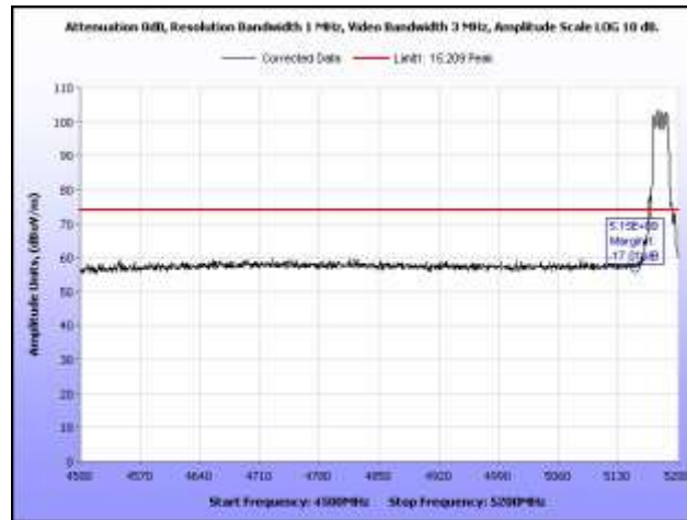
Plot 141. Radiated Band Edge, 802.11n 20 MHz, Low Channel, Peak
