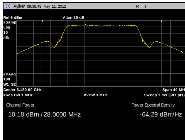
Plot 46. RF Power Output, Low Channel, 802.11a
