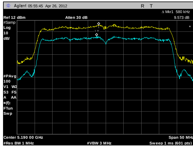
Plot 98. Peak Excursion Ratio, Low Channel, 802.11n 40 MHz (A6)
