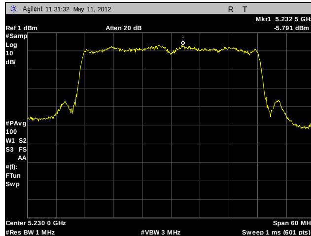
Plot 79. Power Spectral Density, High Channel, 802.11n 40 MHz (A4)
