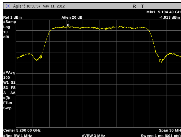
Plot 71. Power Spectral Density, Mid Channel, 802.11n 20 MHz (A5)
