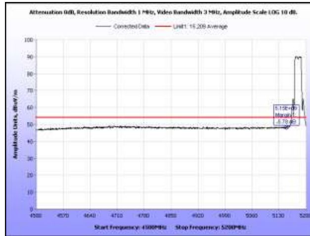
Plot 138. Radiated Band Edge, 802.11a, Low Channel, Average
