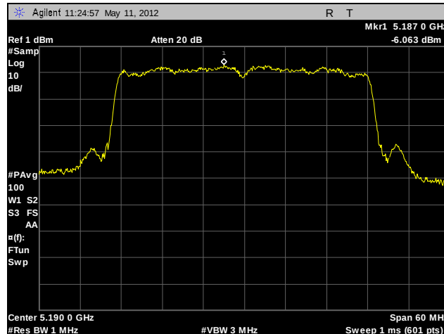
Plot 78. Power Spectral Density, Low Channel, 802.11n 40 MHz (A6)
