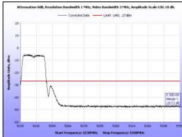
Plot 133. Radiated Band Edge, 802.11a, High Channel
