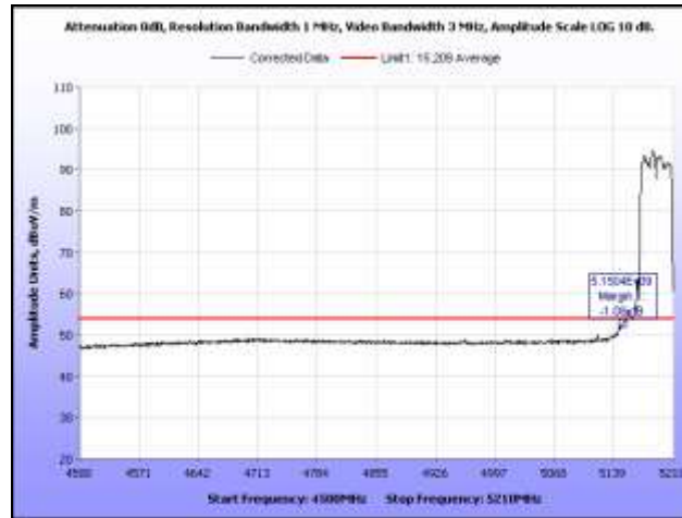
Plot 142. Radiated Band Edge, 802.11n 20 MHz, Low Channel, Average
