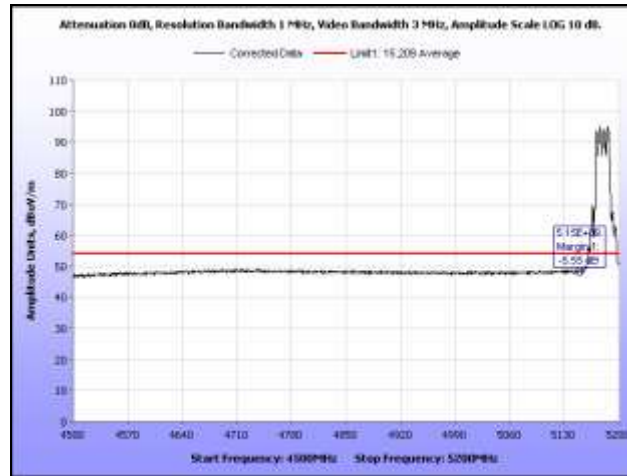
Plot 140. Radiated Band Edge, 802.11n 20 MHz, Low Channel, Average
