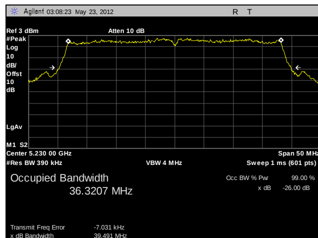
Plot 27. 26 dB Occupied Bandwidth, High Channel, 802.11n 40 MHz (A6)
