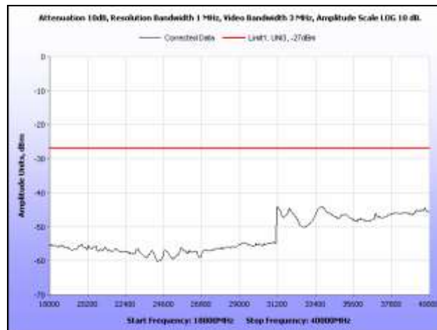
Plot 111. Radiated Spurious Emissions, 802.11a, High Channel, 18 GHz – 40 GHz
