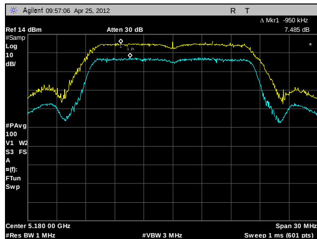
Plot 82. Peak Excursion Ratio, Low Channel, 802.11a
