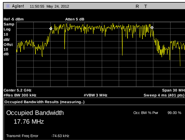
Plot 34. 99% Occupied Bandwidth, Mid Channel, 802.11n 20 MHz (A4)
