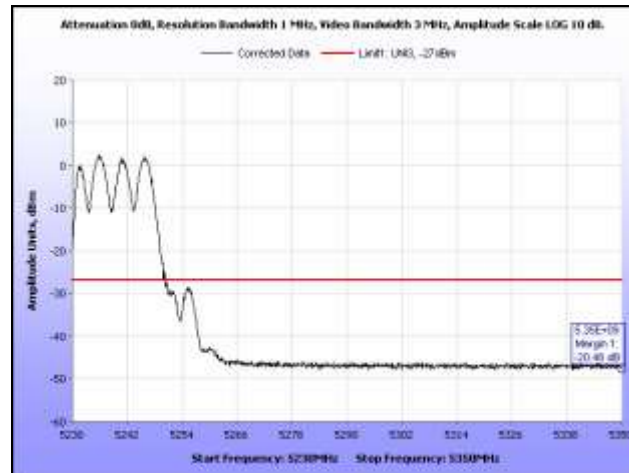
Plot 135. Radiated Band Edge, 802.11n 20 MHz, High Channel
