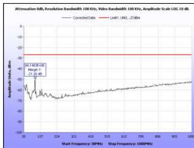
Plot 120. Radiated Spurious Emissions, 802.11n 20 MHz, High Channel, 30 MHz – 1 GHz
