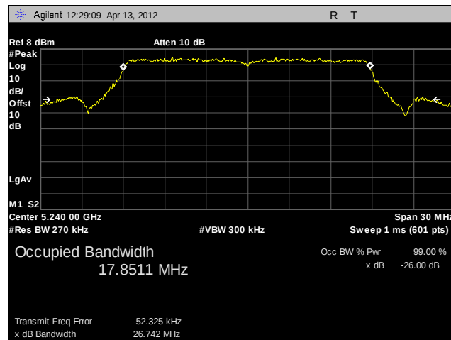
Plot 19. 26 dB Occupied Bandwidth, High Channel, 802.11n 20 MHz (A4)
