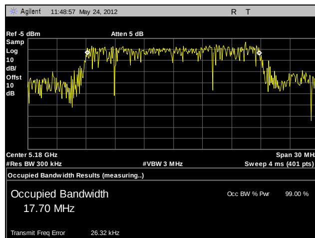
Plot 33. 99% Occupied Bandwidth, Low Channel, 802.11n 20 MHz (A6)
