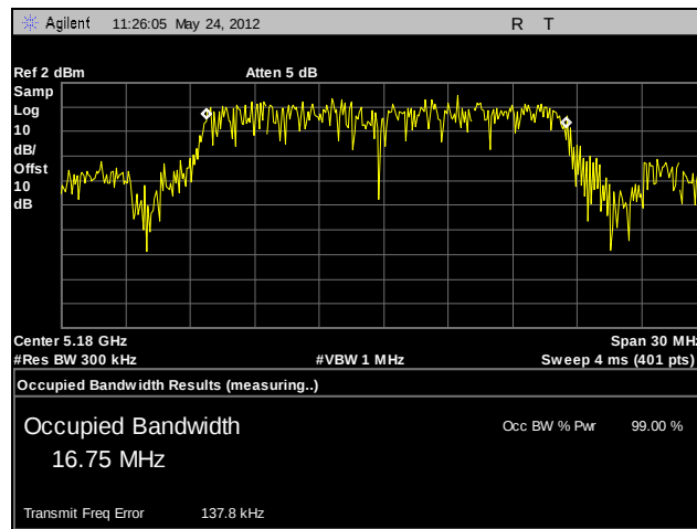
Plot 28. 99% Occupied Bandwidth, Low Channel, 802.11a
