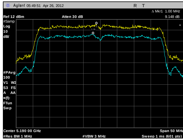
Plot 94. Peak Excursion Ratio, Low Channel, 802.11n 40 MHz (A4)
