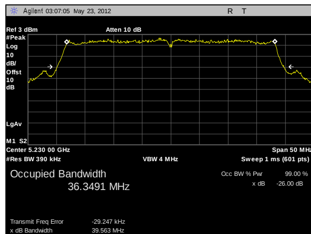
Plot 26. 26 dB Occupied Bandwidth, High Channel, 802.11n 40 MHz (A5)
