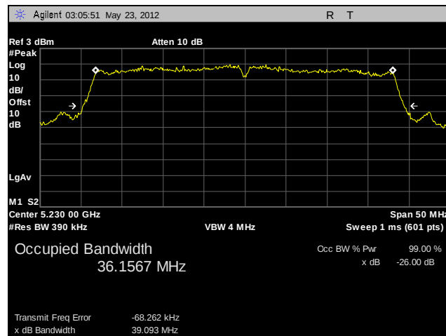
Plot 25. 26 dB Occupied Bandwidth, High Channel, 802.11n 40 MHz (A4)
