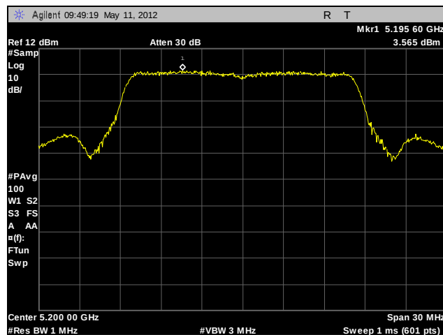
Plot 65. Power Spectral Density, Mid Channel, 802.11a
