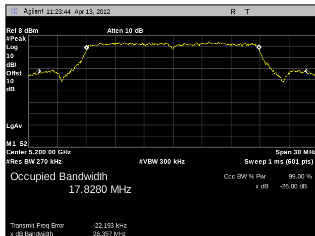
Plot 18. 26 dB Occupied Bandwidth, Mid Channel, 802.11n 20 MHz (A6)
