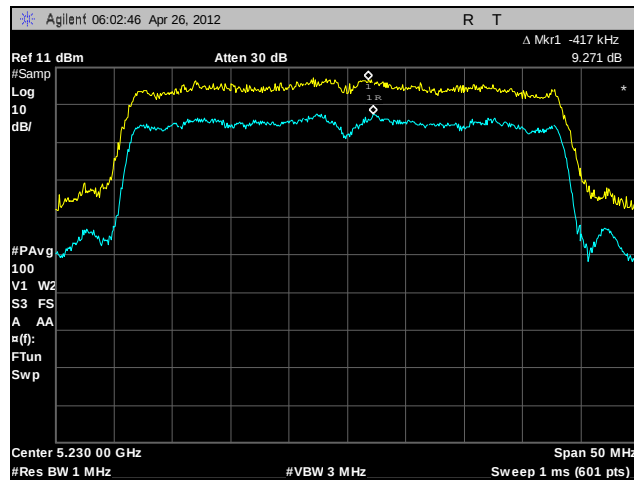
Plot 95. Peak Excursion Ratio, High Channel, 802.11n 40 MHz (A4)
