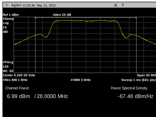
Plot 54. RF Power Output, Mid Channel, 802.11n 20 MHz (A6)
