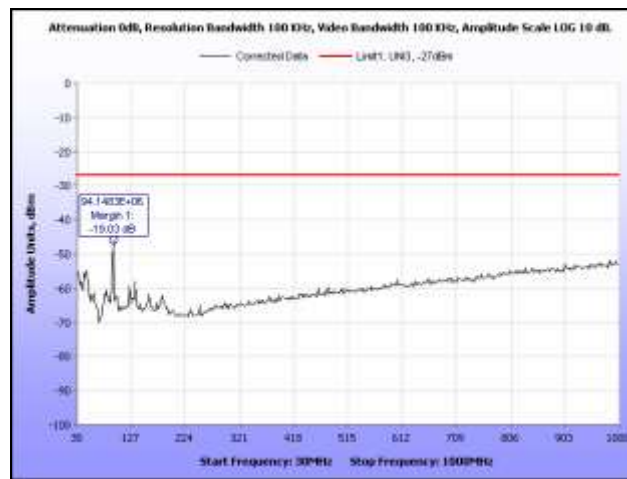
Plot 104. Radiated Spurious Emissions, 802.11a, Mid Channel, 30 MHz – 1 GHz
