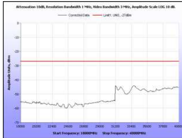
Plot 115. Radiated Spurious Emissions, 802.11n 20 MHz, Low Channel, 18 GHz – 40 GHz
