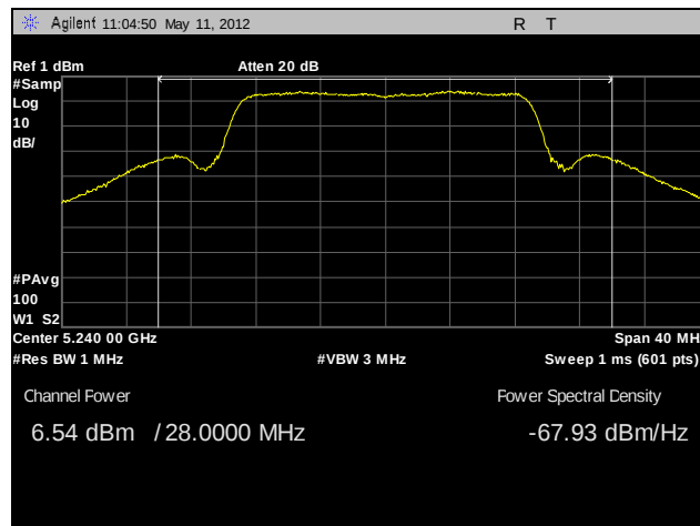
Plot 57. RF Power Output, High Channel, 802.11n 20 MHz (A6)
