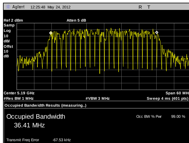
Plot 42. 99% Occupied Bandwidth, Low Channel, 802.11n 40 MHz (A6)
