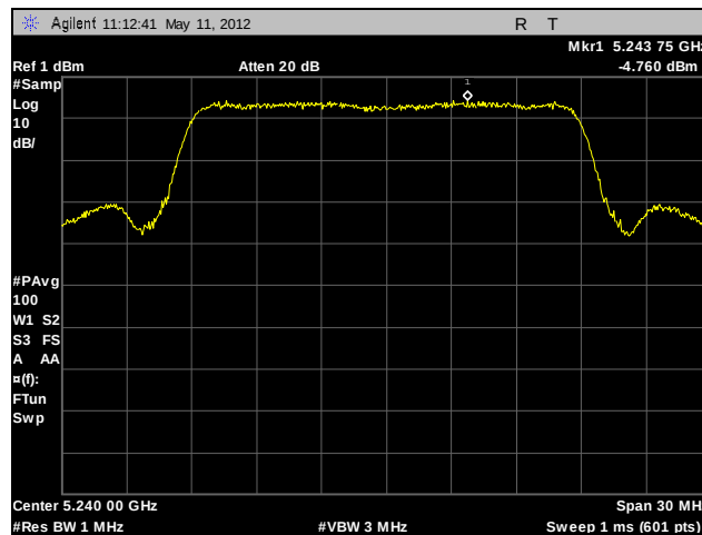
Plot 73. Power Spectral Density, High Channel, 802.11n 20 MHz (A4)
