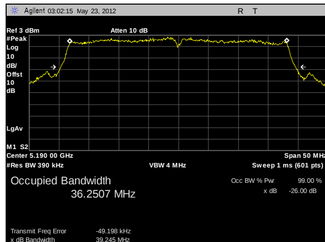
Plot 24. 26 dB Occupied Bandwidth, Low Channel, 802.11n 40 MHz (A6)
