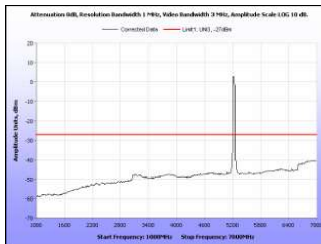
Plot 129. Radiated Spurious Emissions, 802.11n 40 MHz, High Channel, 1 GHz – 7 GHz
