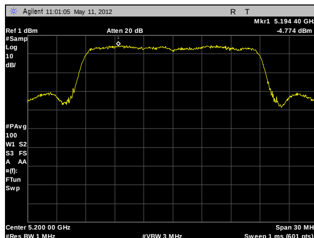
Plot 72. Power Spectral Density, Mid Channel, 802.11n 20 MHz (A6)
