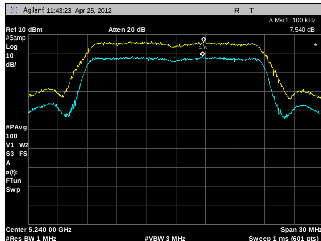
Plot 87. Peak Excursion Ratio, High Channel, 802.11n 20 MHz (A4)
