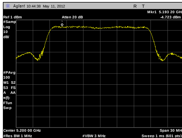
Plot 70. Power Spectral Density, Mid Channel, 802.11n 20 MHz (A4)
