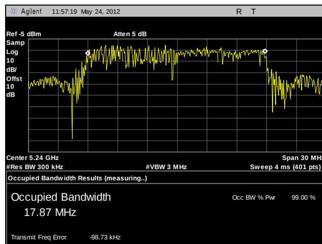
Plot 38. 99% Occupied Bandwidth, High Channel, 802.11n 20 MHz (A5)
