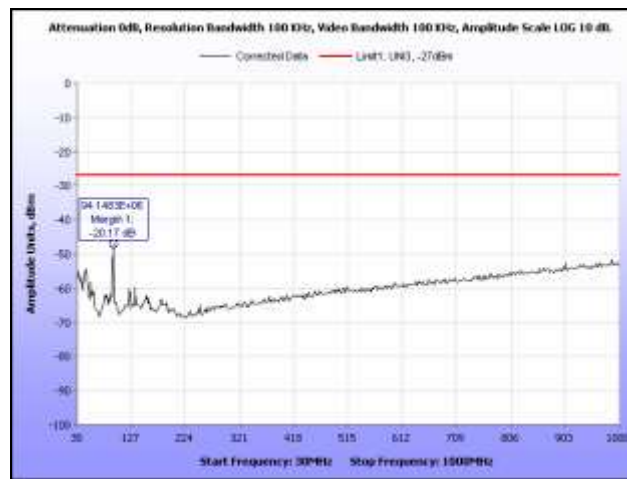
Plot 116. Radiated Spurious Emissions, 802.11n 20 MHz, Mid Channel, 30 MHz – 1 GHz
