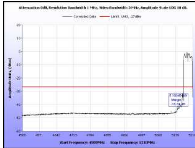
Plot 136. Radiated Band Edge, 802.11n 40 MHz, Low Channel
