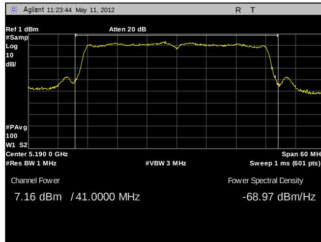
Plot 58. RF Power Output, Low Channel, 802.11n 40 MHz (A4)
