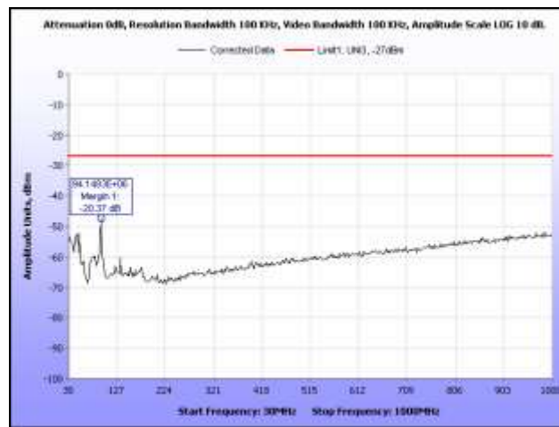
Plot 128. Radiated Spurious Emissions, 802.11n 40 MHz, High Channel, 30 MHz – 1 GHz
