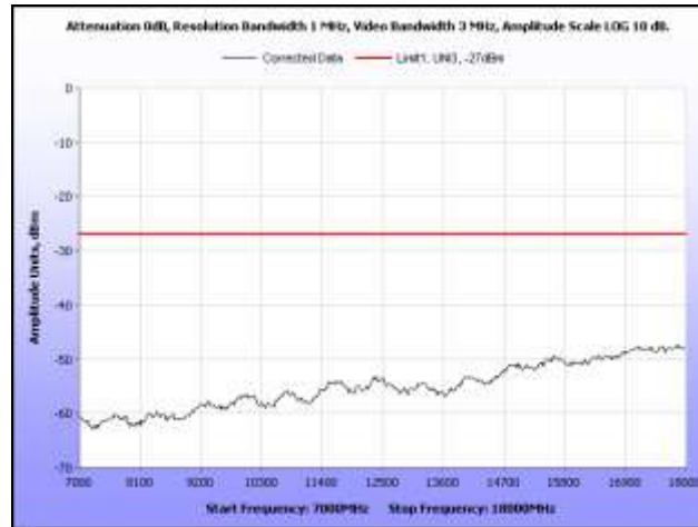
Plot 106. Radiated Spurious Emissions, 802.11a, Mid Channel, 7 GHz – 18 GHz
