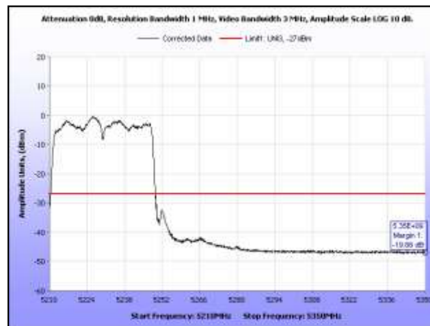
Plot 137. Radiated Band Edge, 802.11n 40 MHz, High Channel
