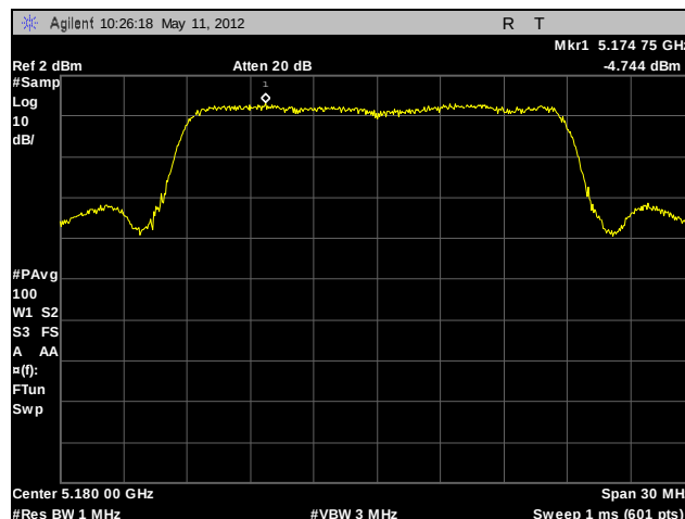
Plot 68. Power Spectral Density, Low Channel, 802.11n 20 MHz (A5)
