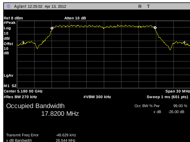
Plot 14. 26 dB Occupied Bandwidth, Low Channel, 802.11n 20 MHz (A5)
