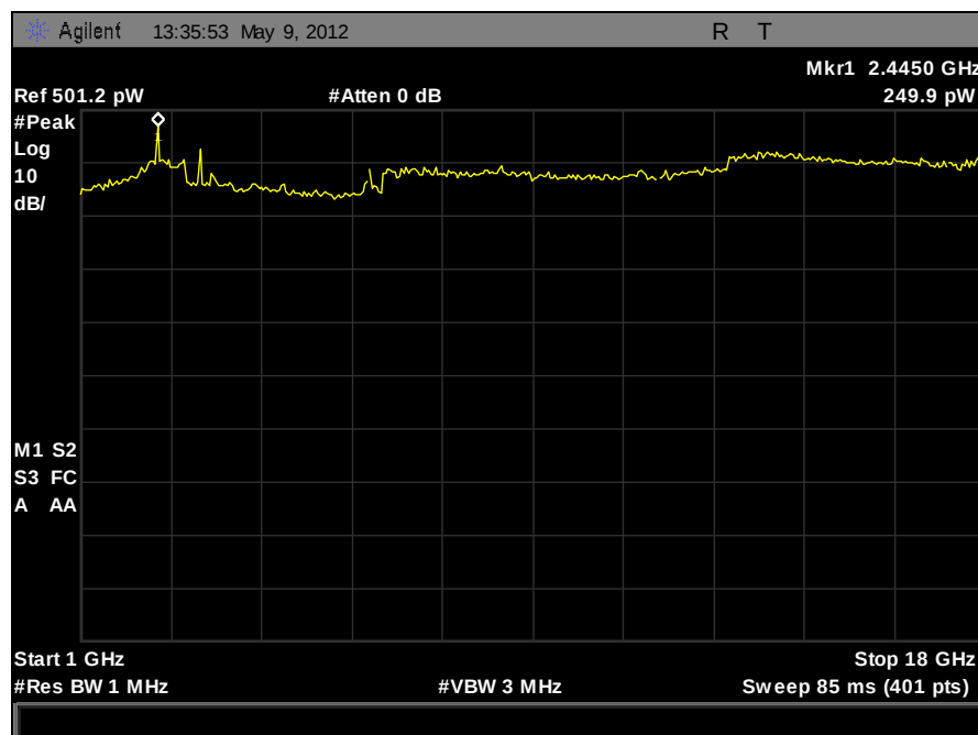
Plot 157. Receiver Spurious Emission, 1 GHz – 18 GHz (Port 1)
