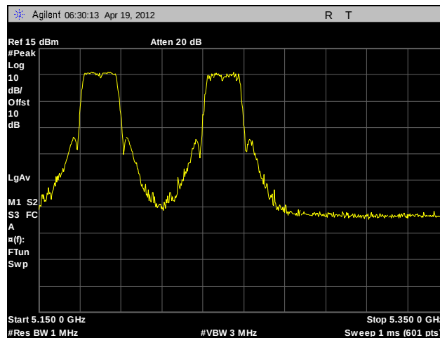
Plot 144. Frequency Stability, 5150 – 5250 MHz, -30°C, 120 V
