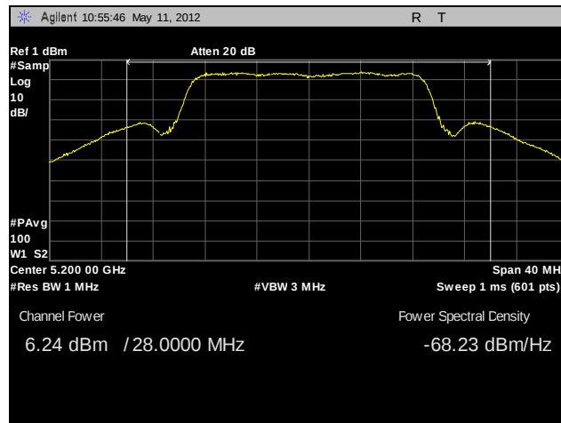
Plot 53. RF Power Output, Mid Channel, 802.11n 20 MHz (A5)
