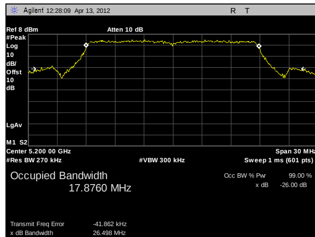
Plot 16. 26 dB Occupied Bandwidth, Mid Channel, 802.11n 20 MHz (A4)
