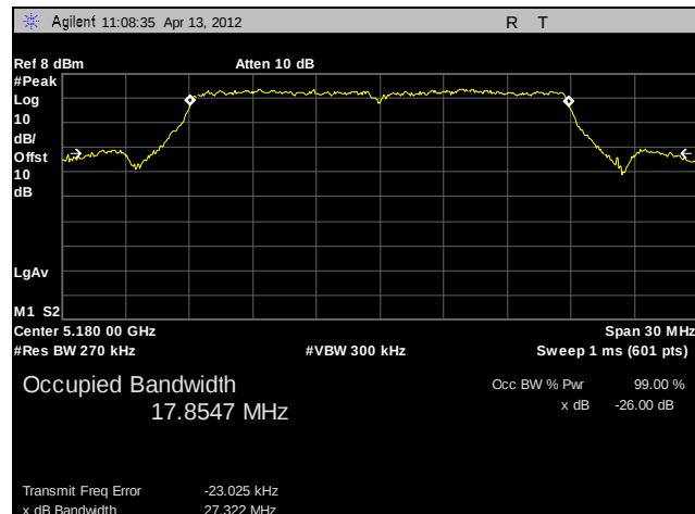
Plot 15. 26 dB Occupied Bandwidth, Low Channel, 802.11n 20 MHz (A6)
