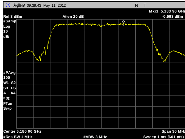
Plot 64. Power Spectral Density, Low Channel, 802.11a
