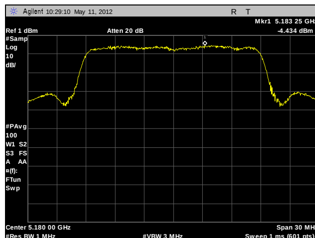
Plot 69. Power Spectral Density, Low Channel, 802.11n 20 MHz (A6)
