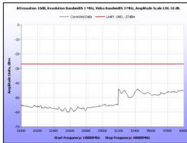
Plot 107. Radiated Spurious Emissions, 802.11a, Mid Channel, 18 GHz – 40 GHz
