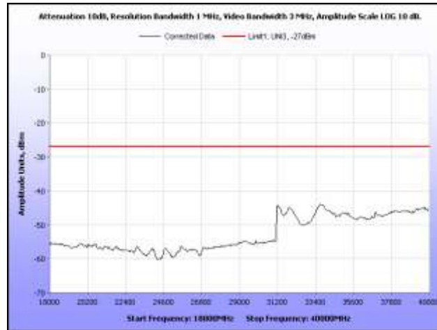
Plot 103. Radiated Spurious Emissions, 802.11a, Low Channel, 18 GHz – 40 GHz
