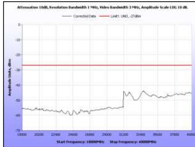
Plot 127. Radiated Spurious Emissions, 802.11n 40 MHz, Low Channel, 18 GHz – 40 GHz
