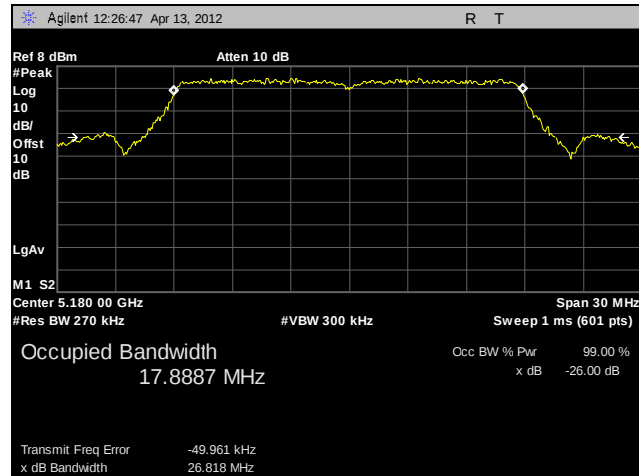
Plot 13. 26 dB Occupied Bandwidth, Low Channel, 802.11n 20 MHz (A4)
