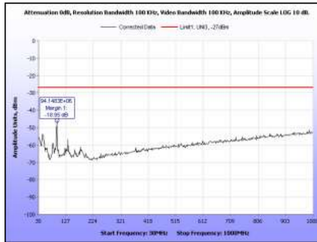
Plot 100. Radiated Spurious Emissions, 802.11a, Low Channel, 30 MHz – 1 GHz
