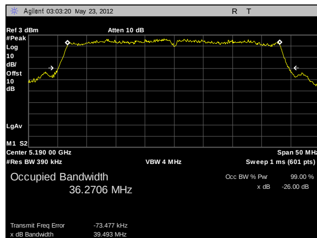
Plot 23. 26 dB Occupied Bandwidth, Low Channel, 802.11n 40 MHz (A5)
