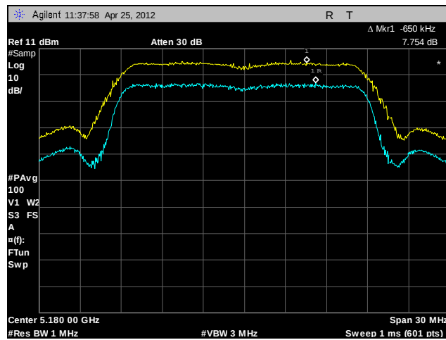
Plot 85. Peak Excursion Ratio, Low Channel, 802.11n 20 MHz (A4)
