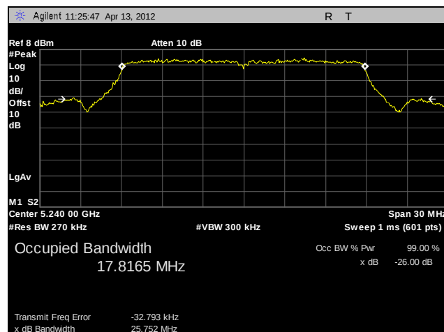
Plot 21. 26 dB Occupied Bandwidth, High Channel, 802.11n 20 MHz (A6)
