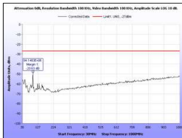
Plot 108. Radiated Spurious Emissions, 802.11a, High Channel, 30 MHz – 1 GHz
