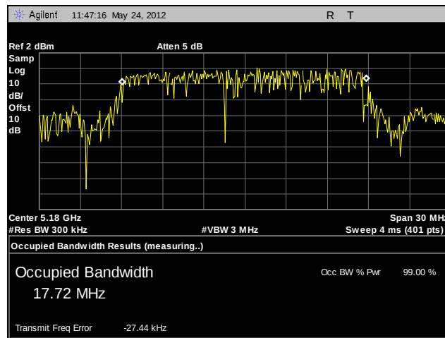
Plot 31. 99% Occupied Bandwidth, Low Channel, 802.11n 20 MHz (A4)
