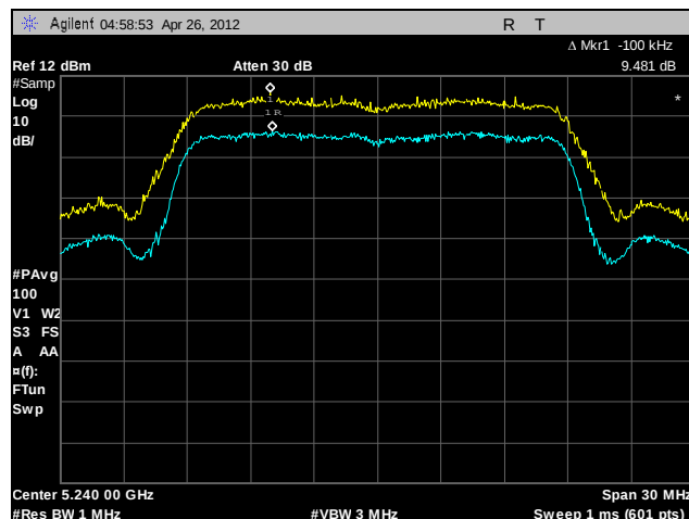
Plot 93. Peak Excursion Ratio, High Channel, 802.11n 20 MHz (A6)
