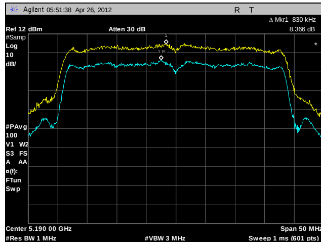
Plot 96. Peak Excursion Ratio, Low Channel, 802.11n 40 MHz (A5)
