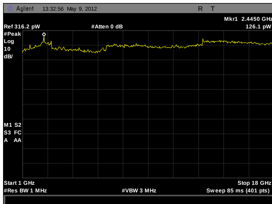
Plot 159. Receiver Spurious Emission, 1 GHz – 18 GHz (Port 2)
