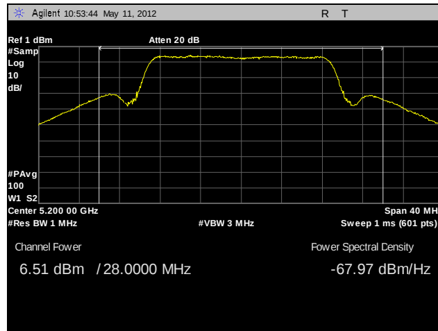
Plot 52. RF Power Output, Mid Channel, 802.11n 20 MHz (A4)
