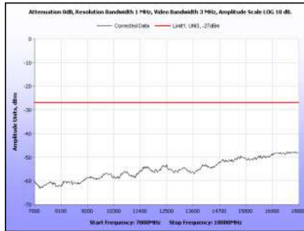
Plot 110. Radiated Spurious Emissions, 802.11a, High Channel, 7 GHz – 18 GHz
