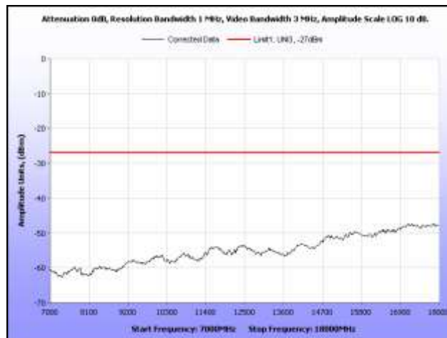
Plot 102. Radiated Spurious Emissions, 802.11a, Low Channel, 7 GHz – 18 GHz
