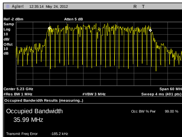
Plot 44. 99% Occupied Bandwidth, High Channel, 802.11n 40 MHz (A5)
