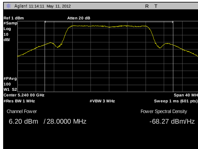
Plot 56. RF Power Output, High Channel, 802.11n 20 MHz (A5)
