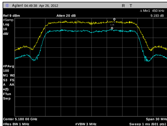
Plot 91. Peak Excursion Ratio, Low Channel, 802.11n 20 MHz (A6)
