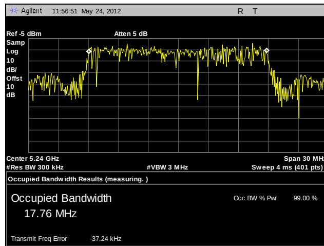
Plot 37. 99% Occupied Bandwidth, High Channel, 802.11n 20 MHz (A4)
