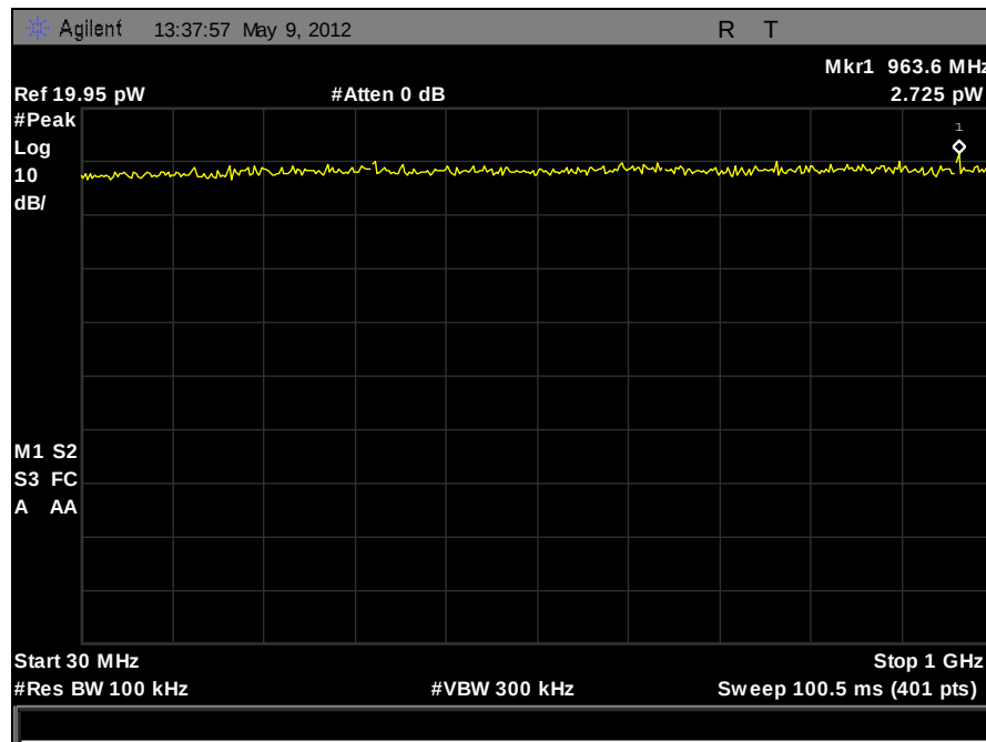
Plot 160. Receiver Spurious Emission, 30 MHz – 1 GHz (Port 3)
