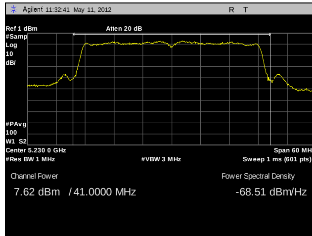
Plot 61. RF Power Output, High Channel, 802.11n 40 MHz (A4)
