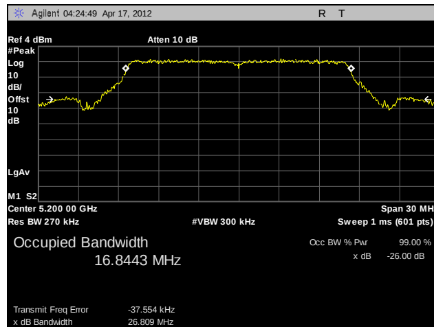
Plot 11. 26 dB Occupied Bandwidth, Mid Channel, 802.11a
