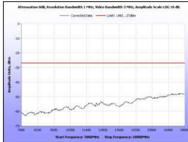
Plot 118. Radiated Spurious Emissions, 802.11n 20 MHz, Mid Channel, 7 GHz – 18 GHz
