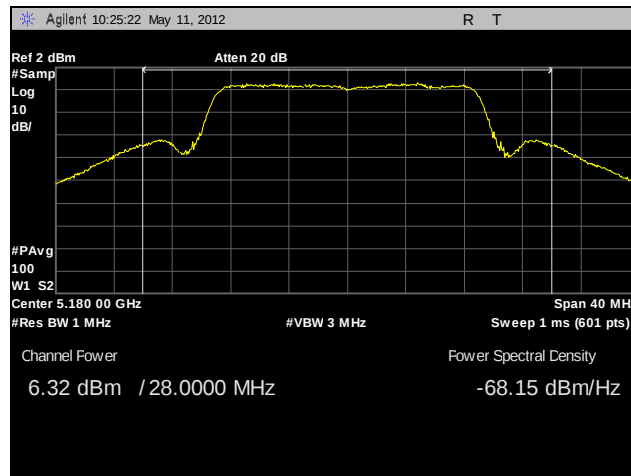
Plot 50. RF Power Output, Low Channel, 802.11n 20 MHz (A5)
