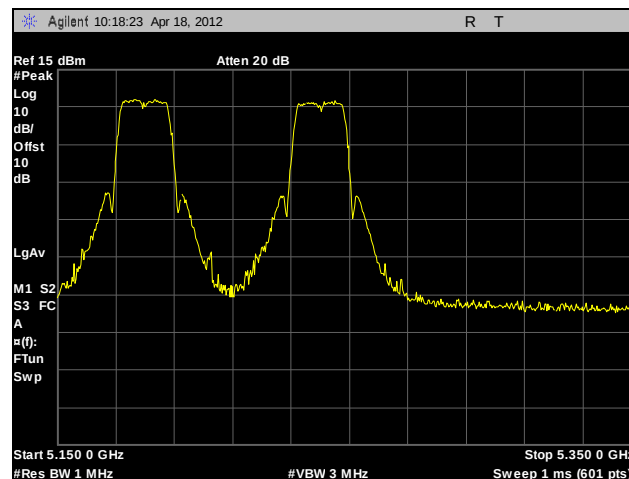
Plot 154. Frequency Stability, 5150 – 5250 MHz, 50°C, 120 V
