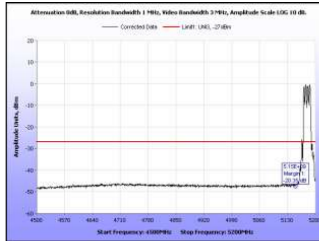
Plot 134. Radiated Band Edge, 802.11n 20 MHz, Low Channel
