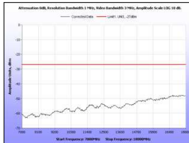
Plot 126. Radiated Spurious Emissions, 802.11n 40 MHz, Low Channel, 7 GHz – 18 GHz
