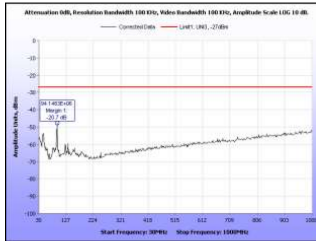
Plot 112. Radiated Spurious Emissions, 802.11n 20 MHz, Low Channel, 30 MHz – 1 GHz
