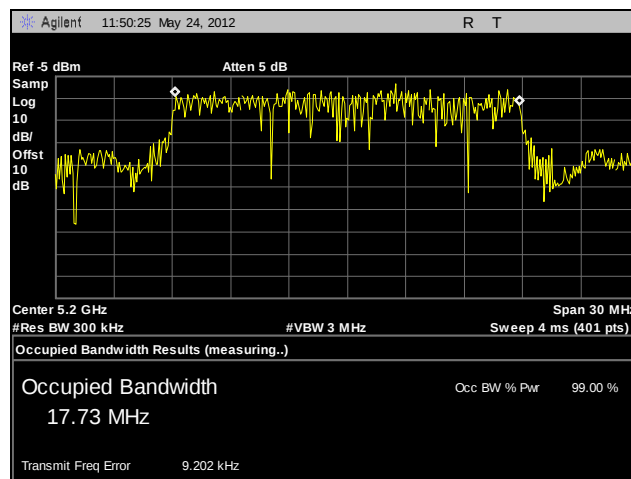
Plot 35. 99% Occupied Bandwidth, Mid Channel, 802.11n 20 MHz (A5)
