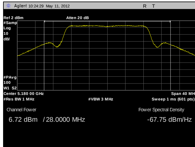
Plot 49. RF Power Output, Low Channel, 802.11n 20 MHz (A4)
