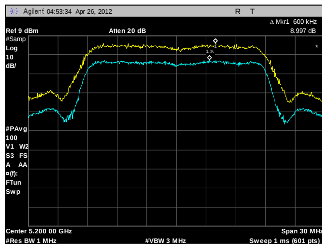
Plot 89. Peak Excursion Ratio, Mid Channel, 802.11n 20 MHz (A5)
