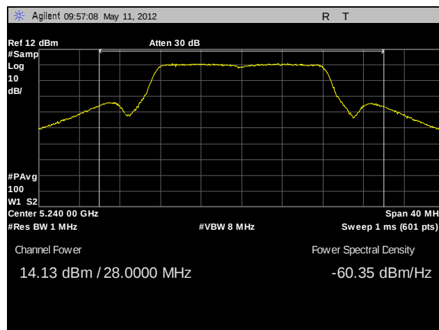
Plot 48. RF Power Output, High Channel, 802.11a
