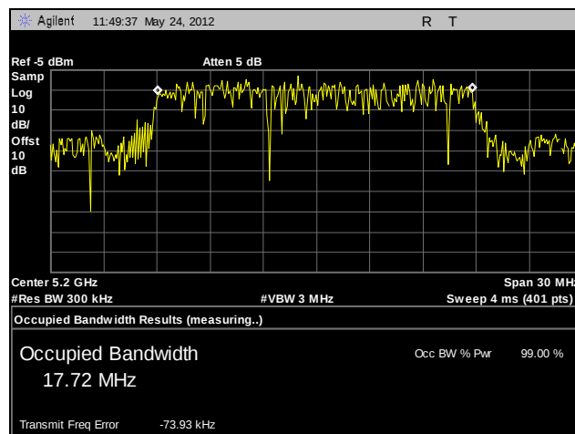
Plot 36. 99% Occupied Bandwidth, Mid Channel, 802.11n 20 MHz (A6)
