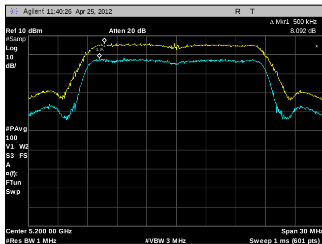
Plot 86. Peak Excursion Ratio, Mid Channel, 802.11n 20 MHz (A4)
