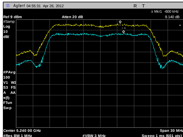
Plot 90. Peak Excursion Ratio, High Channel, 802.11n 20 MHz (A5)
