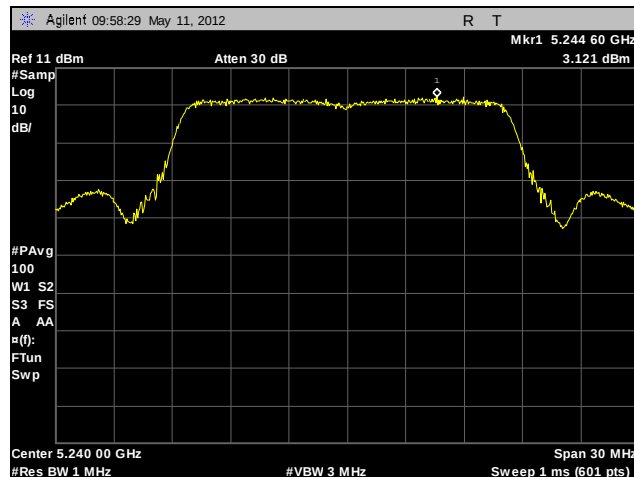
Plot 66. Power Spectral Density, High Channel, 802.11a
