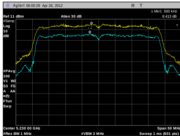
Plot 97. Peak Excursion Ratio, High Channel, 802.11n 40 MHz (A5)
