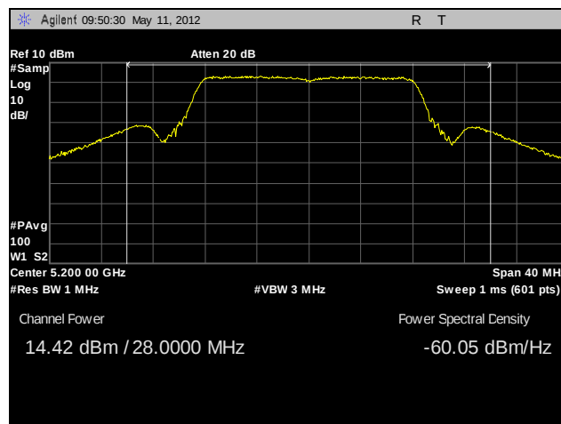
Plot 47. RF Power Output, Mid Channel, 802.11a
