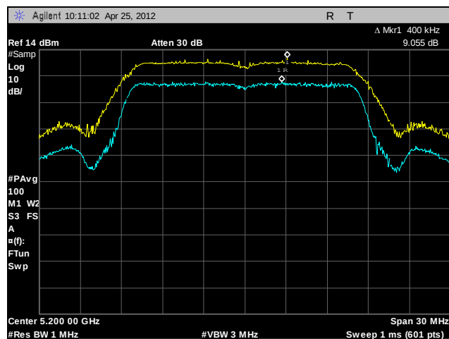
Plot 83. Peak Excursion Ratio, Mid Channel, 802.11a
