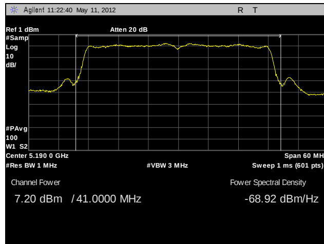
Plot 59. RF Power Output, Low Channel, 802.11n 40 MHz (A5)
