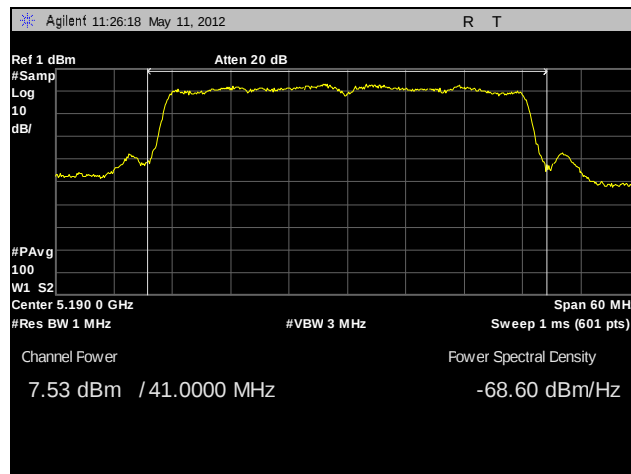
Plot 60. RF Power Output, Low Channel, 802.11n 40 MHz (A6)
