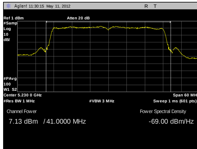
Plot 62. RF Power Output, High Channel, 802.11n 40 MHz (A5)
