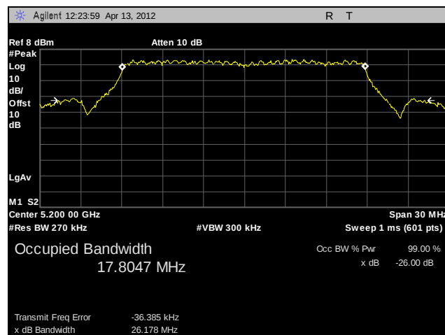
Plot 17. 26 dB Occupied Bandwidth, Mid Channel, 802.11n 20 MHz (A5)
