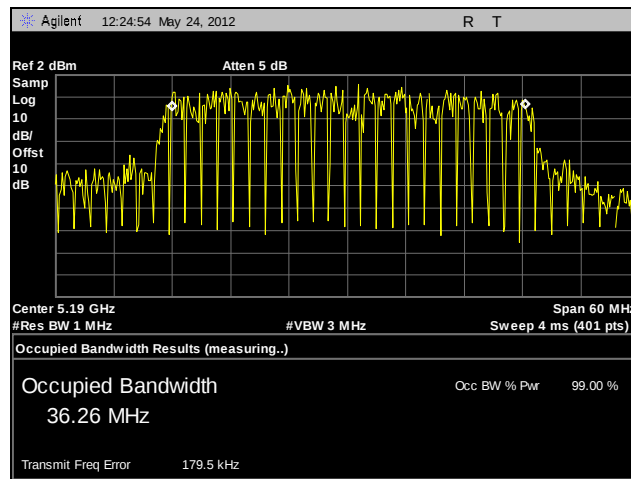
Plot 40. 99% Occupied Bandwidth, Low Channel, 802.11n 40 MHz (A4)
