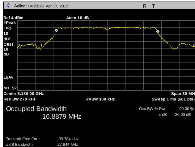
Plot 10. 26 dB Occupied Bandwidth, Low Channel, 802.11a
