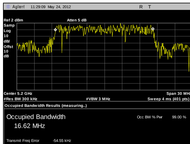
Plot 29. 99% Occupied Bandwidth, Mid Channel, 802.11a
