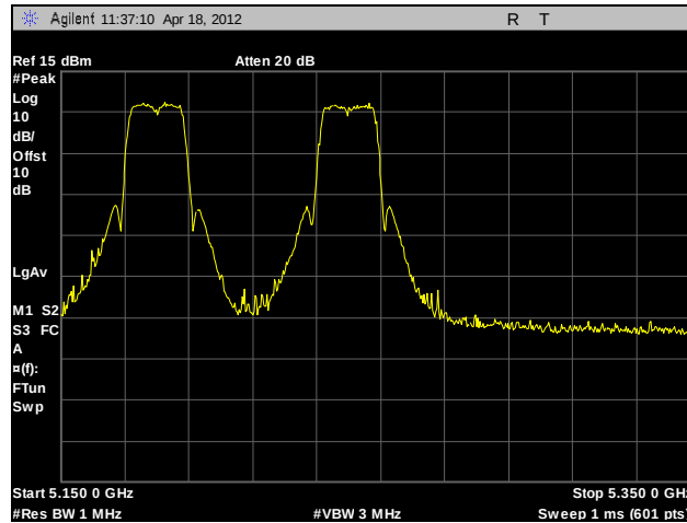
Plot 147. Frequency Stability, 5150 – 5250 MHz, 0°C, 120 V
