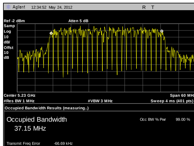
Plot 45. 99% Occupied Bandwidth, High Channel, 802.11n 40 MHz (A6)
