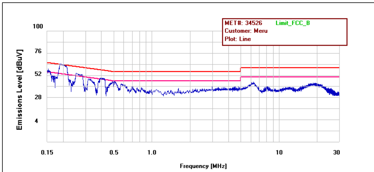
Plot 8. Conducted Emissions, 15.207(a), Phase Line
