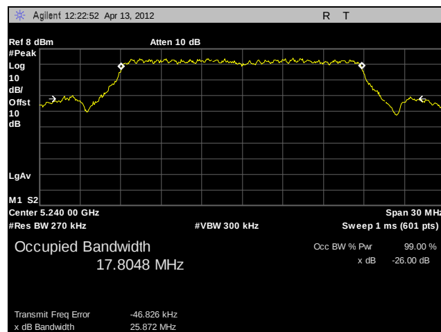
Plot 20. 26 dB Occupied Bandwidth, High Channel, 802.11n 20 MHz (A5)
