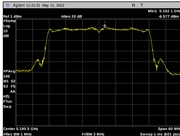
Plot 77. Power Spectral Density, Low Channel, 802.11n 40 MHz (A5)
