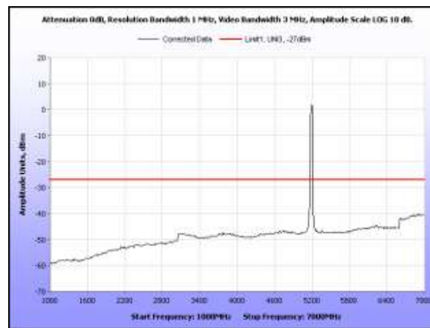
Plot 125. Radiated Spurious Emissions, 802.11n 40 MHz, Low Channel, 1 GHz – 7 GHz
