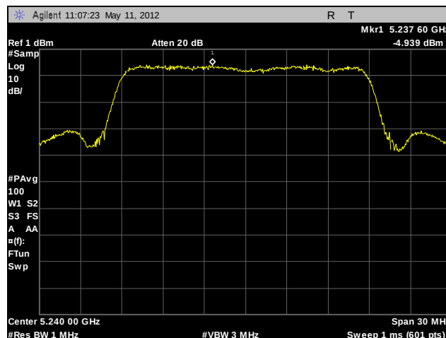
Plot 74. Power Spectral Density, High Channel, 802.11n 20 MHz (A5)
