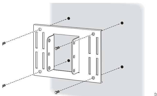
Figure 38: Mount OAP180 Bracket on Wall
