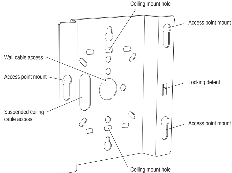
Figure 18: AP200 Bracket
