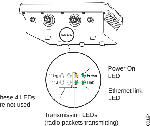
Figure 43: OAP180 LEDs
