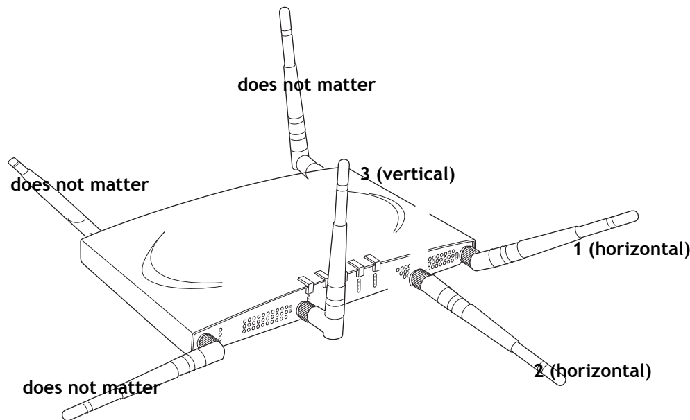
Figure 7: AP310/AP310-M Antennas 1-3
