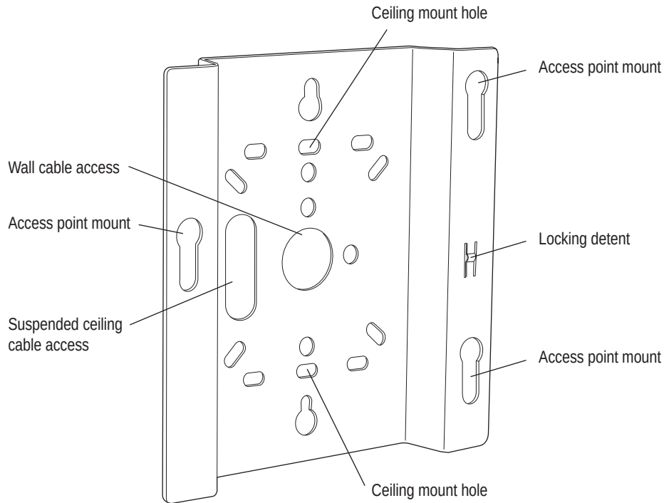
Figure 15: AP200 Mounting Bracket
