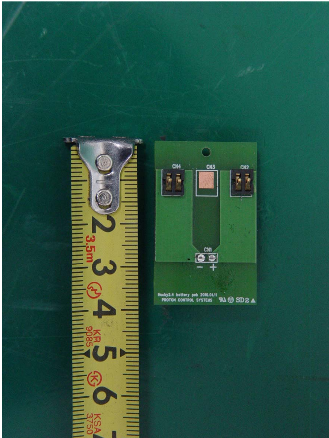
< Board #2 front >
