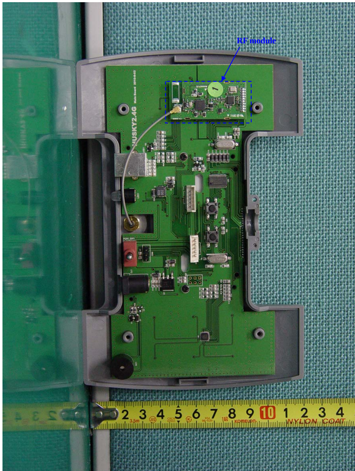
< Inside / RF module location >
