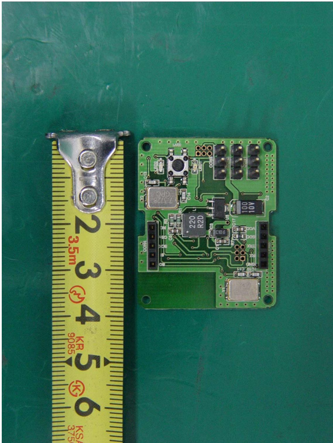
< Board #1 rear >
