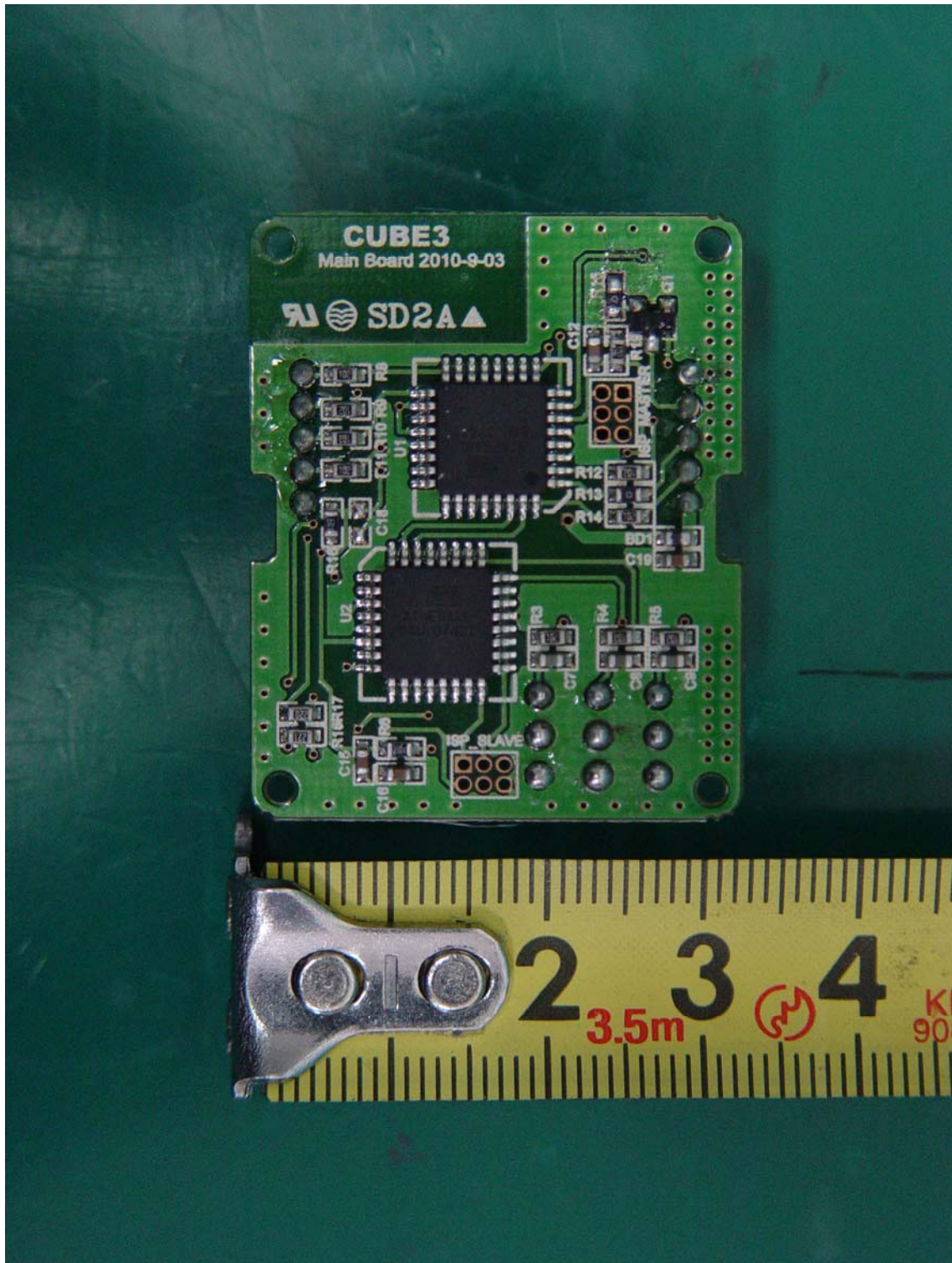
< Board #1 front >
