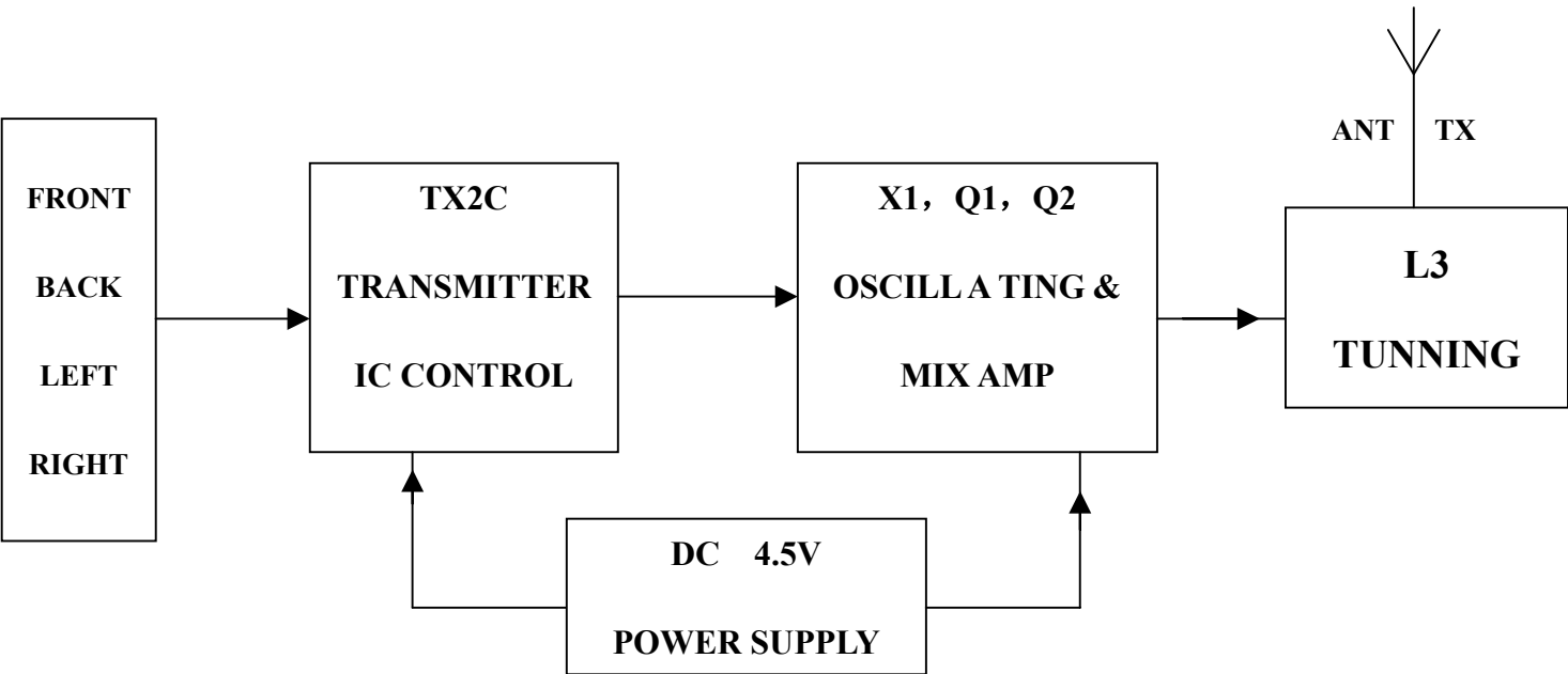
A>BLOCK DIAGRAM
