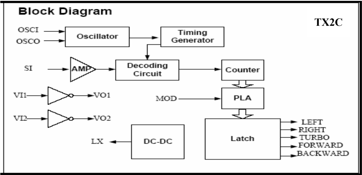
B> IC BLOCK DIAGRAM
