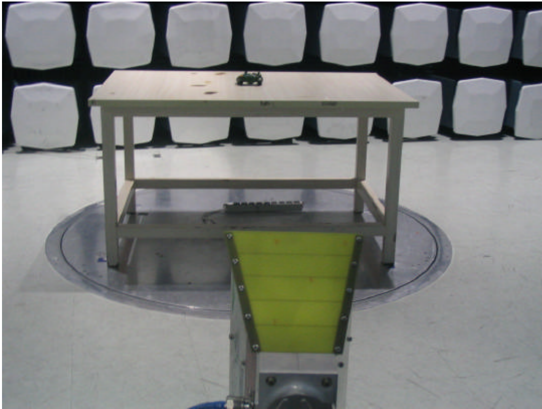
Setup Photo-4
