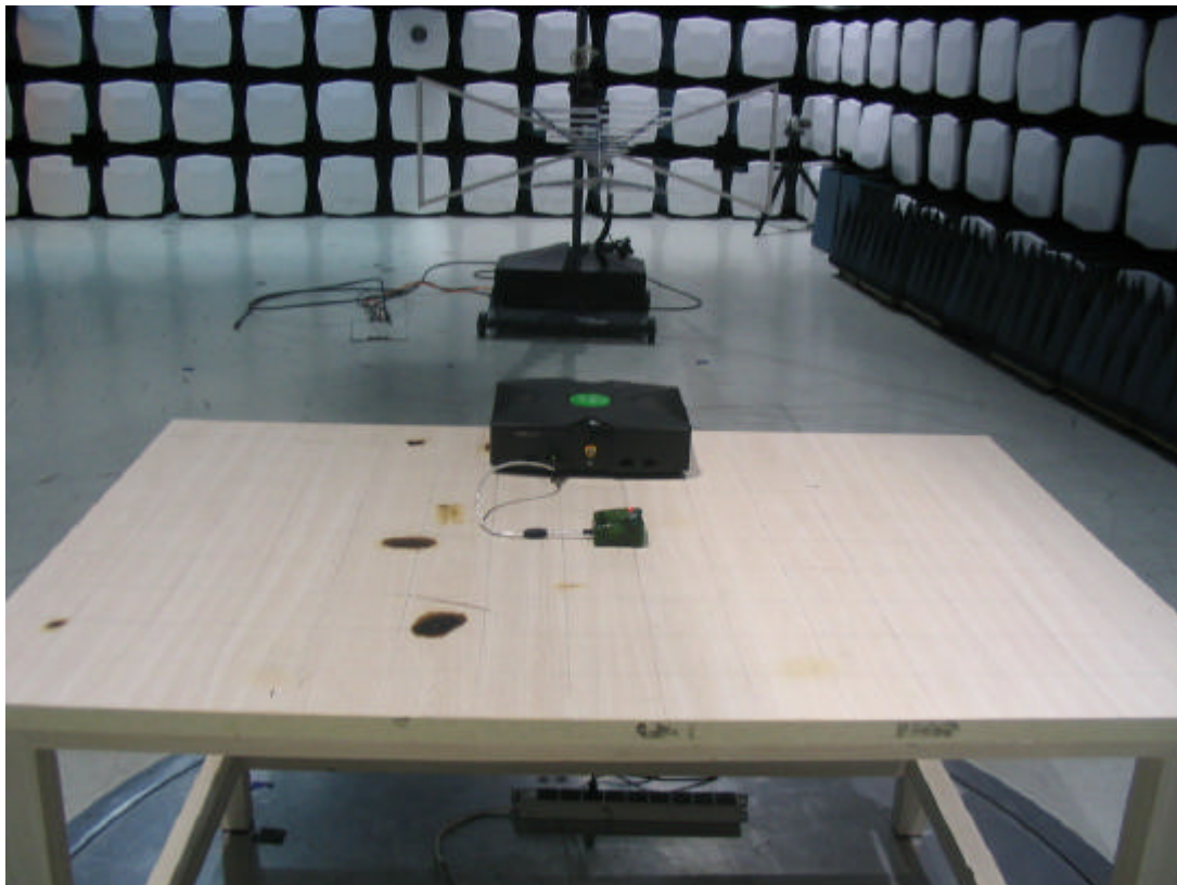
Setup Photo-4
