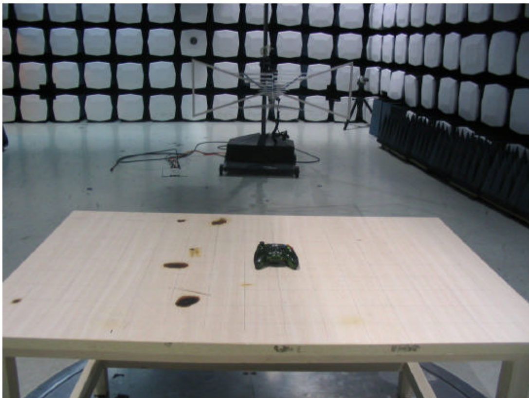
Setup Photo-2
