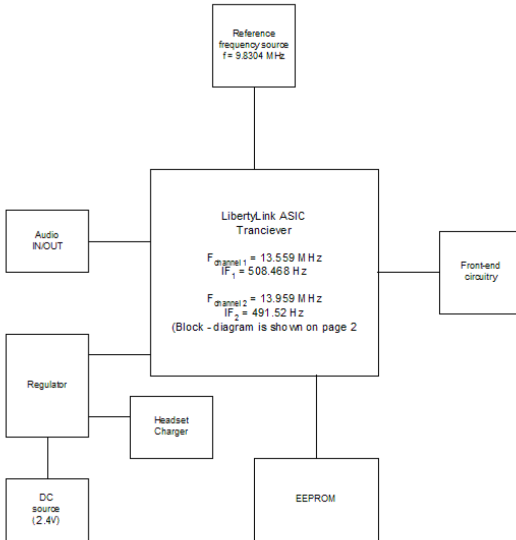
Wireless Headset System Base unit Block - Diagram
