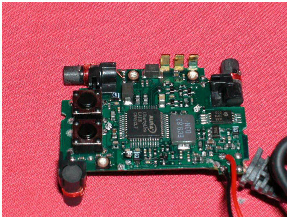
Base Main MCU PCB front side (View 2)
