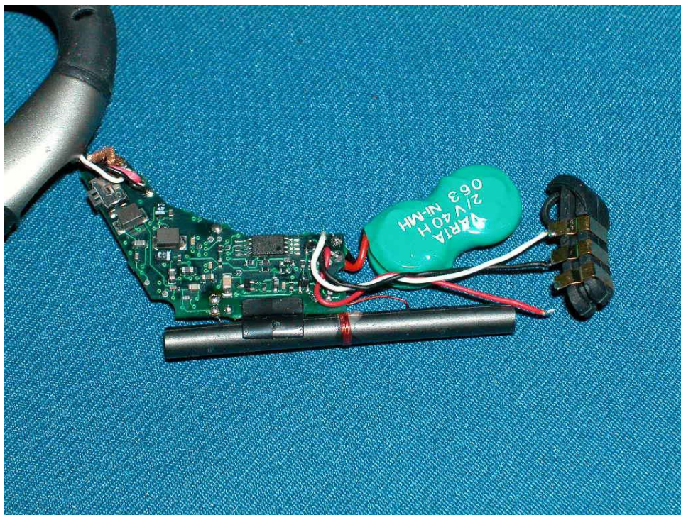
Headset Main MCU PCB rear side (View 1)
