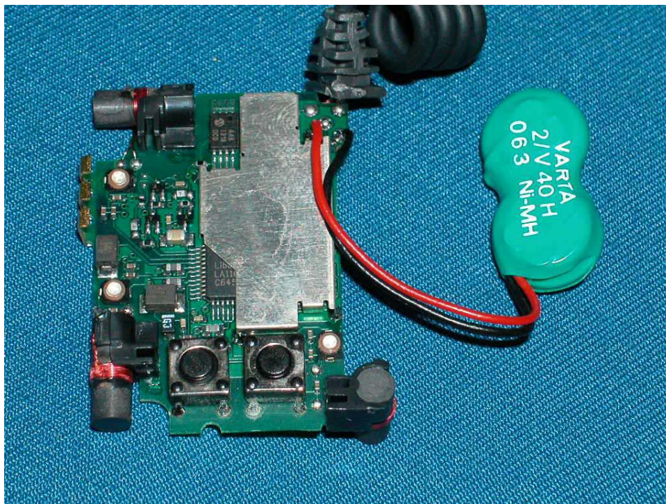
Base Main MCU PCB front side (View 1)
