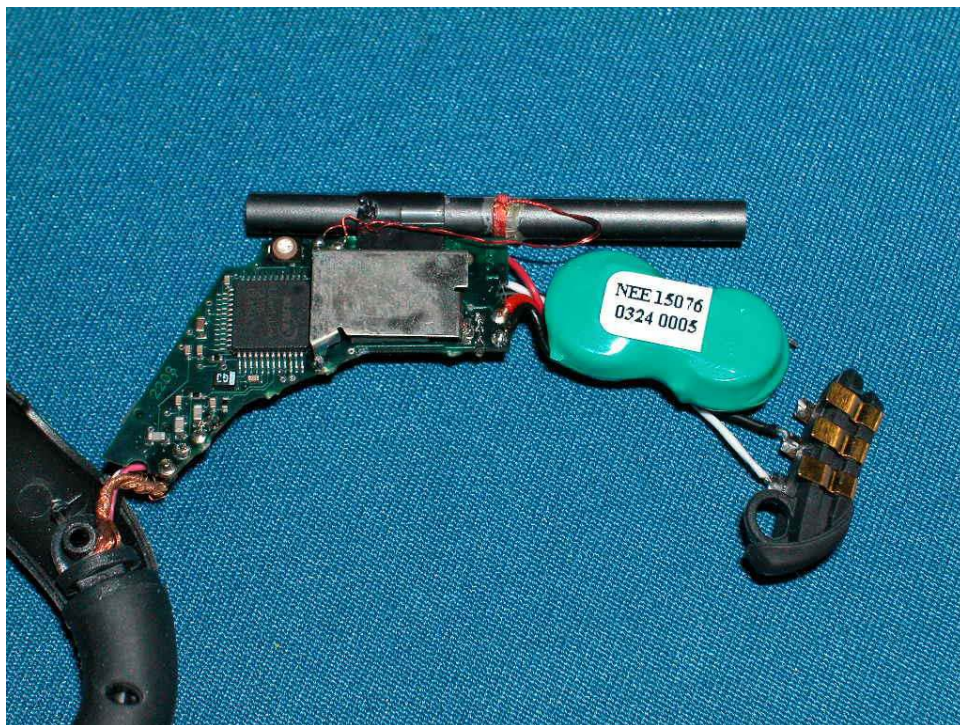
Headset Main MCU PCB front side (View 1)
