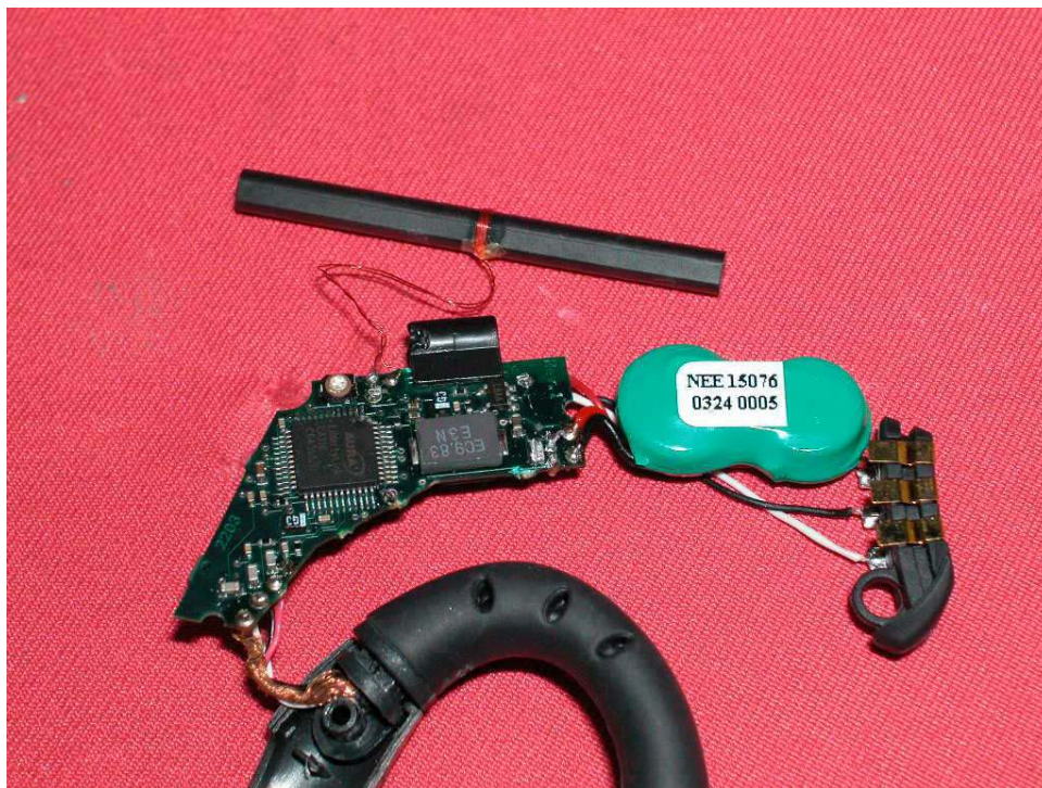
Headset Main MCU PCB front side (View 2)
