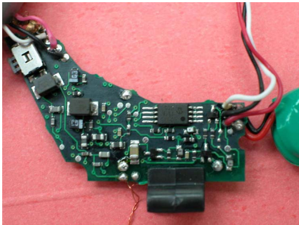
Headset Main MCU PCB rear side (View 2)
