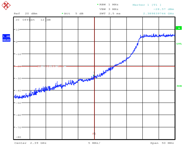
Figure 8.4-37: Conducted lower band edge emission within restricted bands for 802.11n HT20, peak measurement
