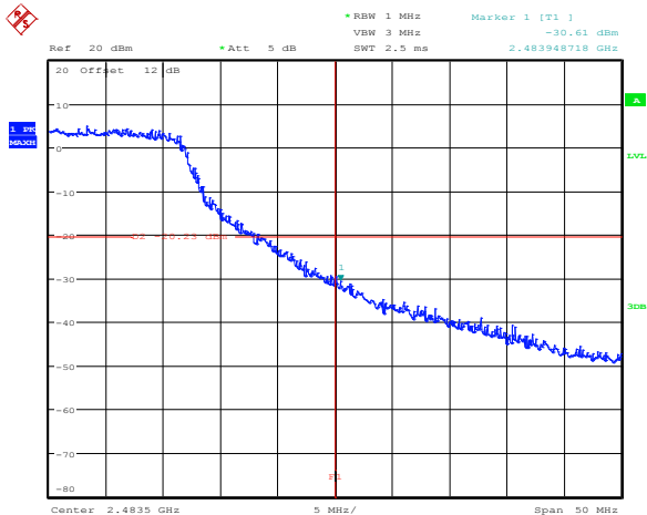
Figure 8.4-45: Conducted upper band edge emission within restricted bands for 802.11n HT20, peak measurement
