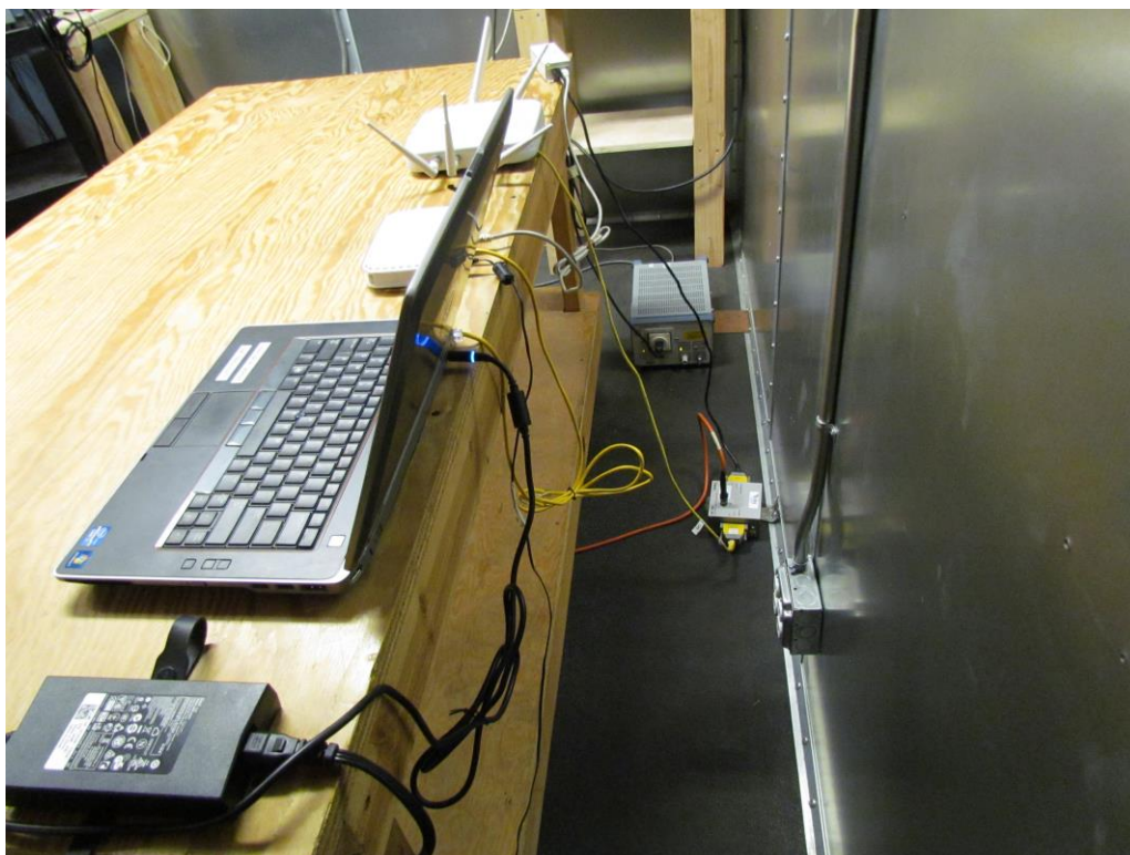
Conducted Emissions Signal Line Side View– SENSOR4-R1S1W1-E
