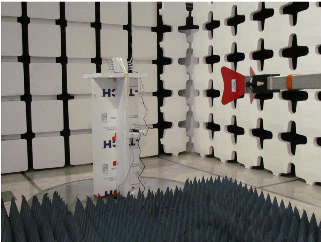
Radiated Emissions below 1GHz 80cm- SENSOR4-R1S1W1-E
