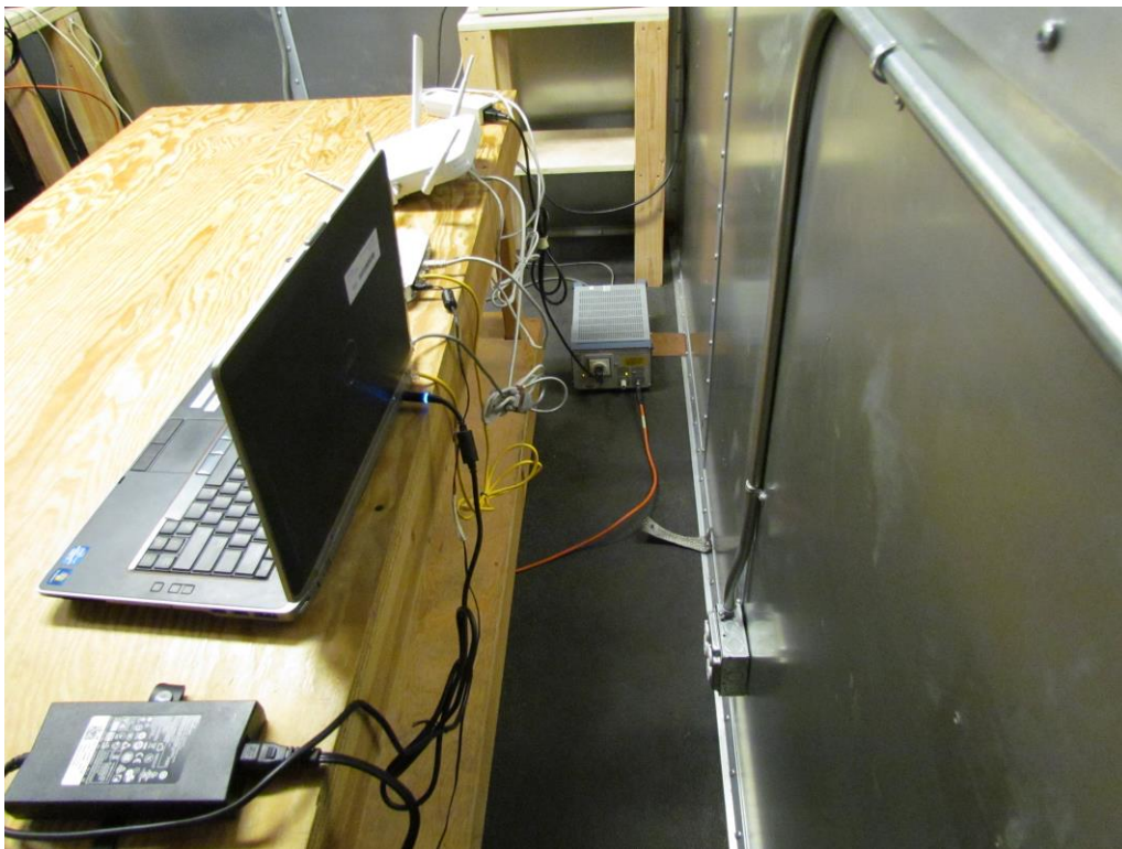
Conducted Emissions AC Line Side View- SENSOR4-R1S1W1-E
