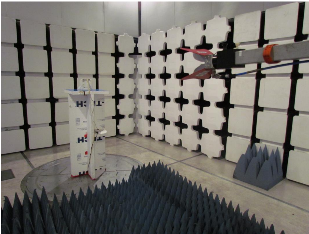
Radiated Emissions above 1GHz 80cm - SENSOR4-R1S1W1-E
