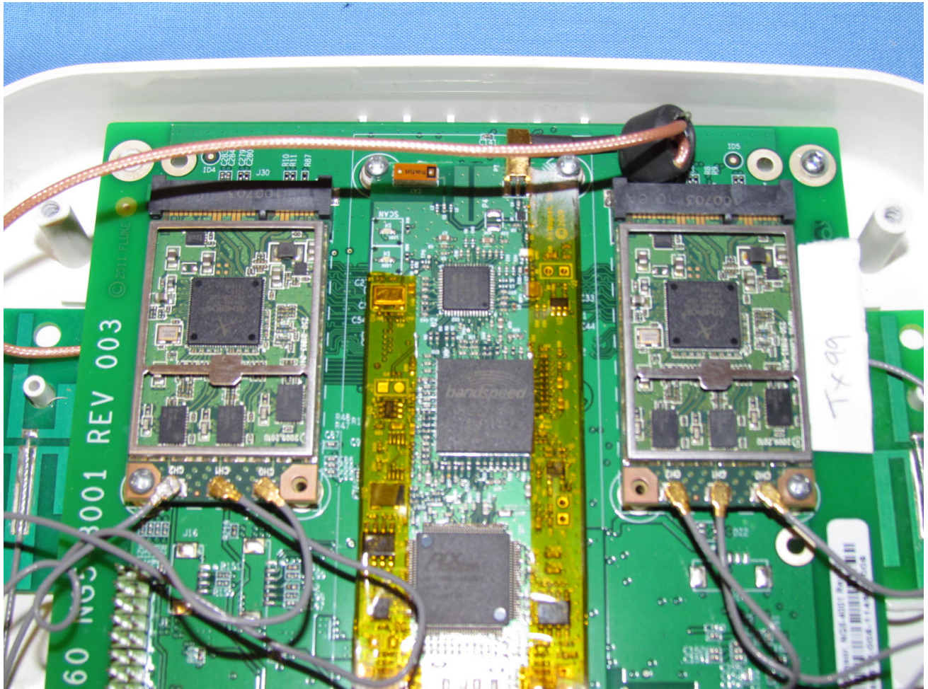
Main assy front with Shields removed
