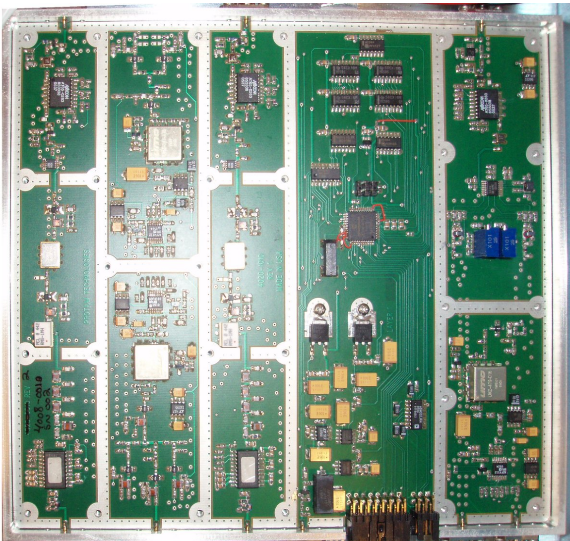
Figure 2: RF front
