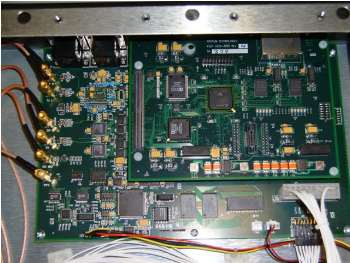
Figure 7: Assembled
