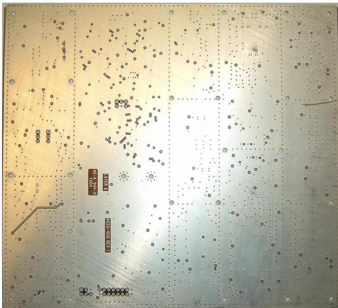
Figure 1: RF board back
