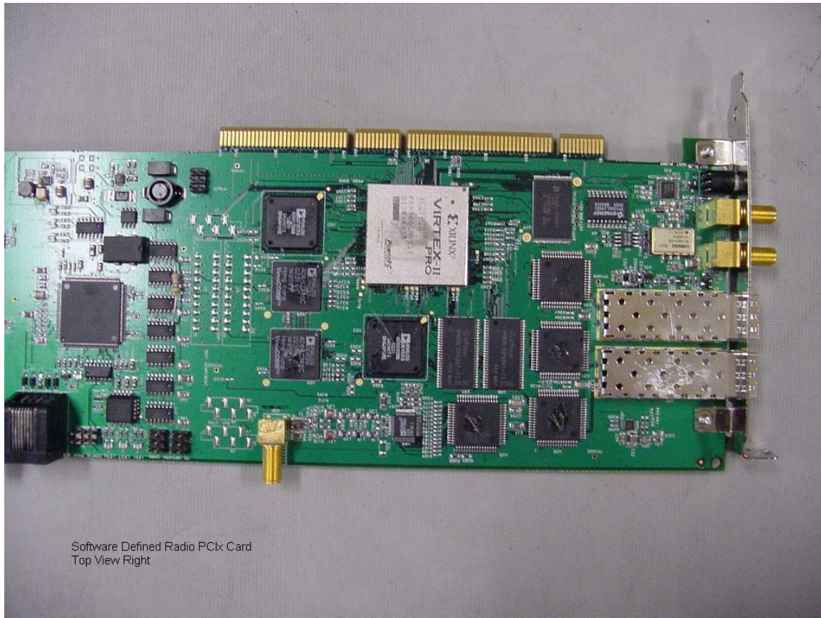
Figure 5 PCIX Card Top View Right
