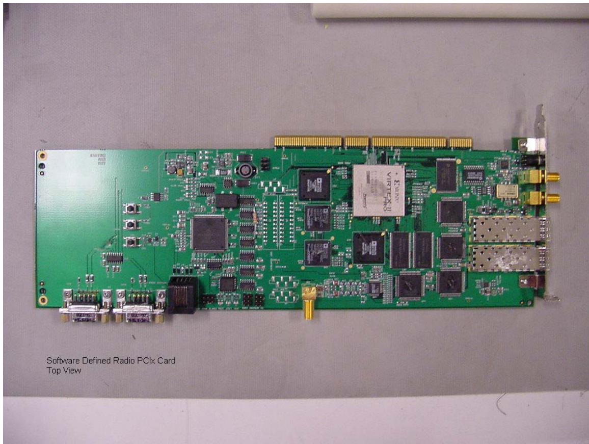
Figure 4 PCIX Card Top View
