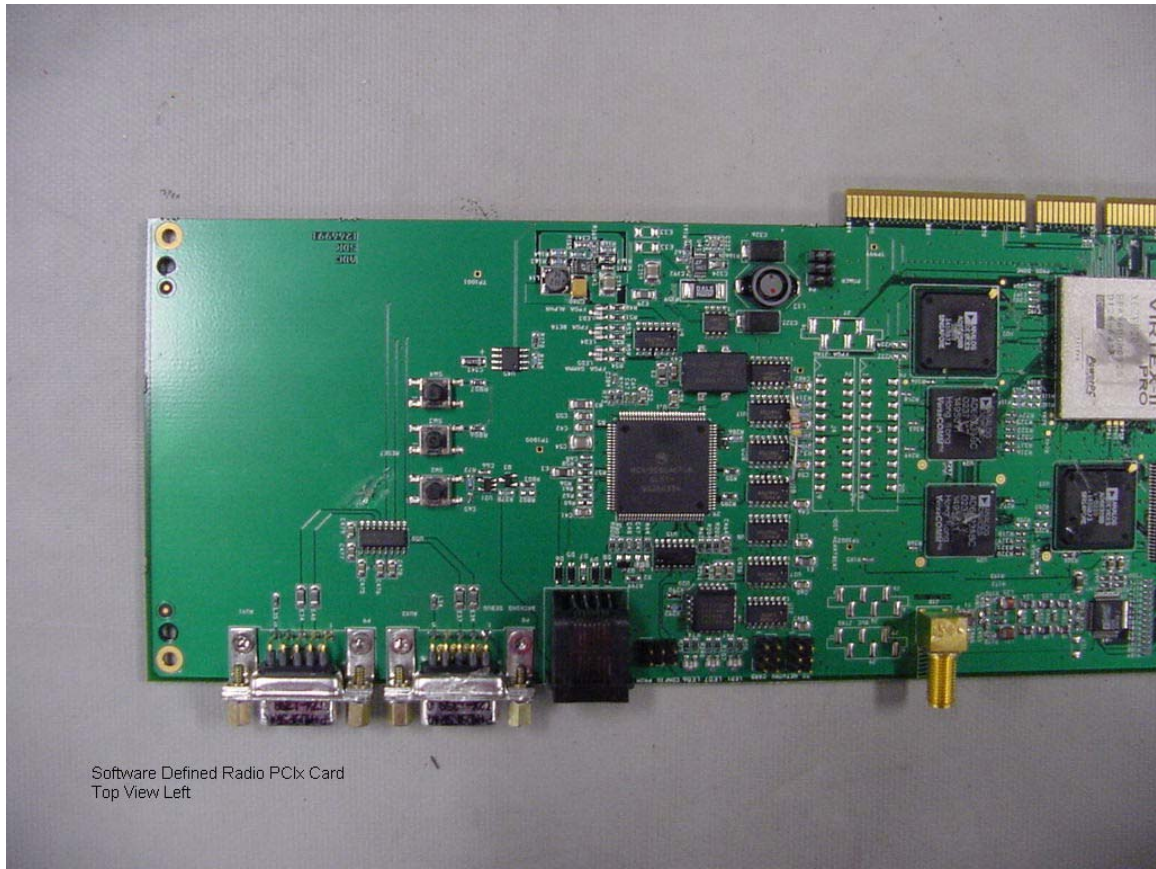
Figure 6 PCIX Card Top View Left
