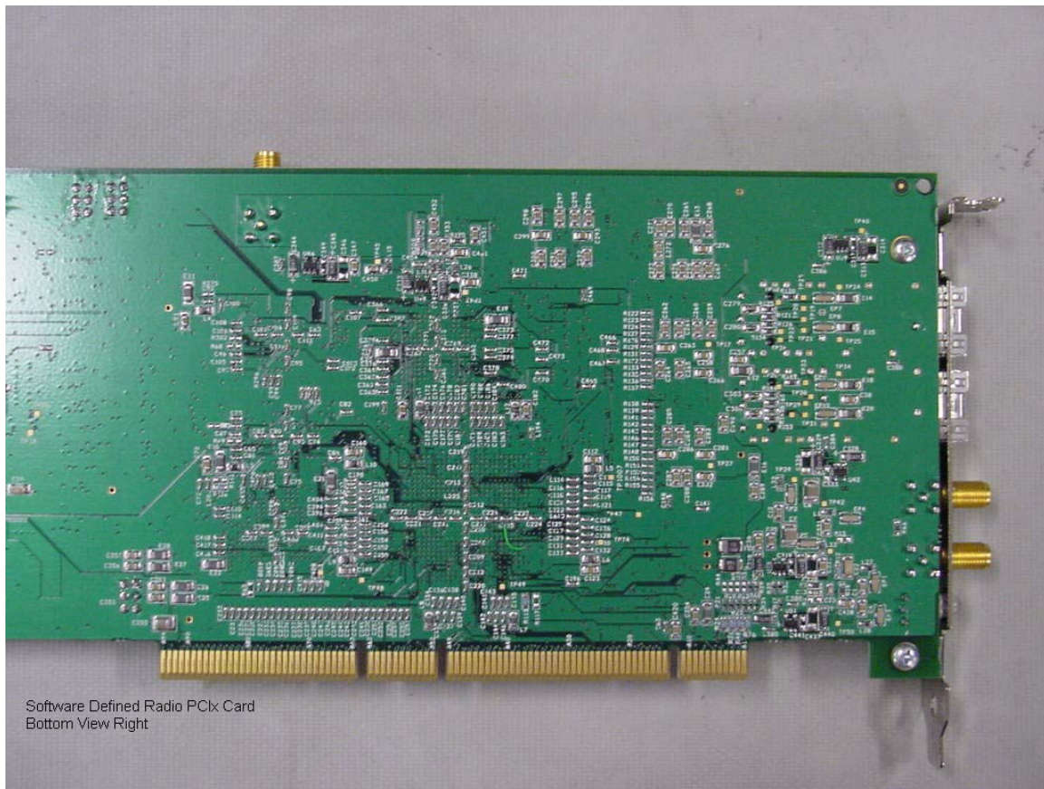
Figure 2 PCIX Card Bottom View Right
