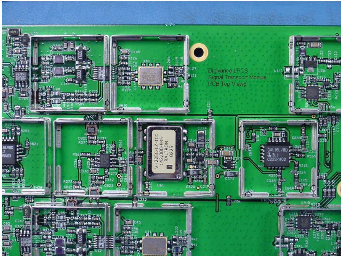
Figure 19 Digivance LRCS STM PCB Top View 8
