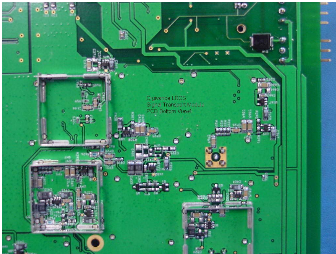
Figure 5 Digivance LRCS STM PCB Bottom View 4
