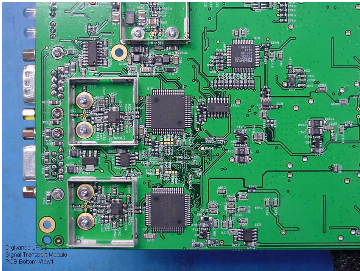
Figure 3 Digivance LRCS STM PCB Bottom View 1
