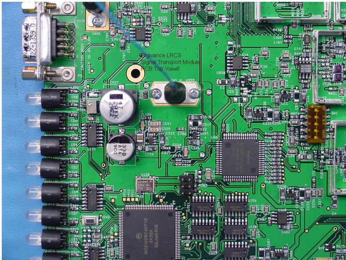
Figure 17 Digivance LRCS STM PCB Top View 6
