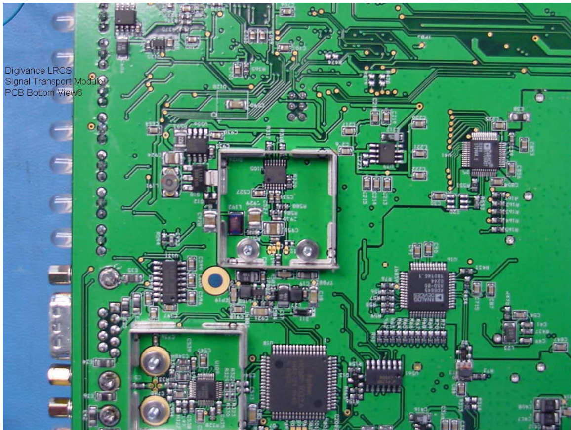
Figure 7 Digivance LRCS STM PCB Bottom View 6
