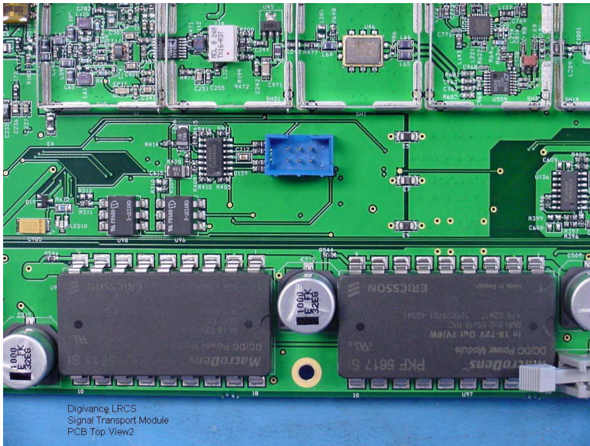
Figure 13 Digivance LRCS STM PCB Top View 2
