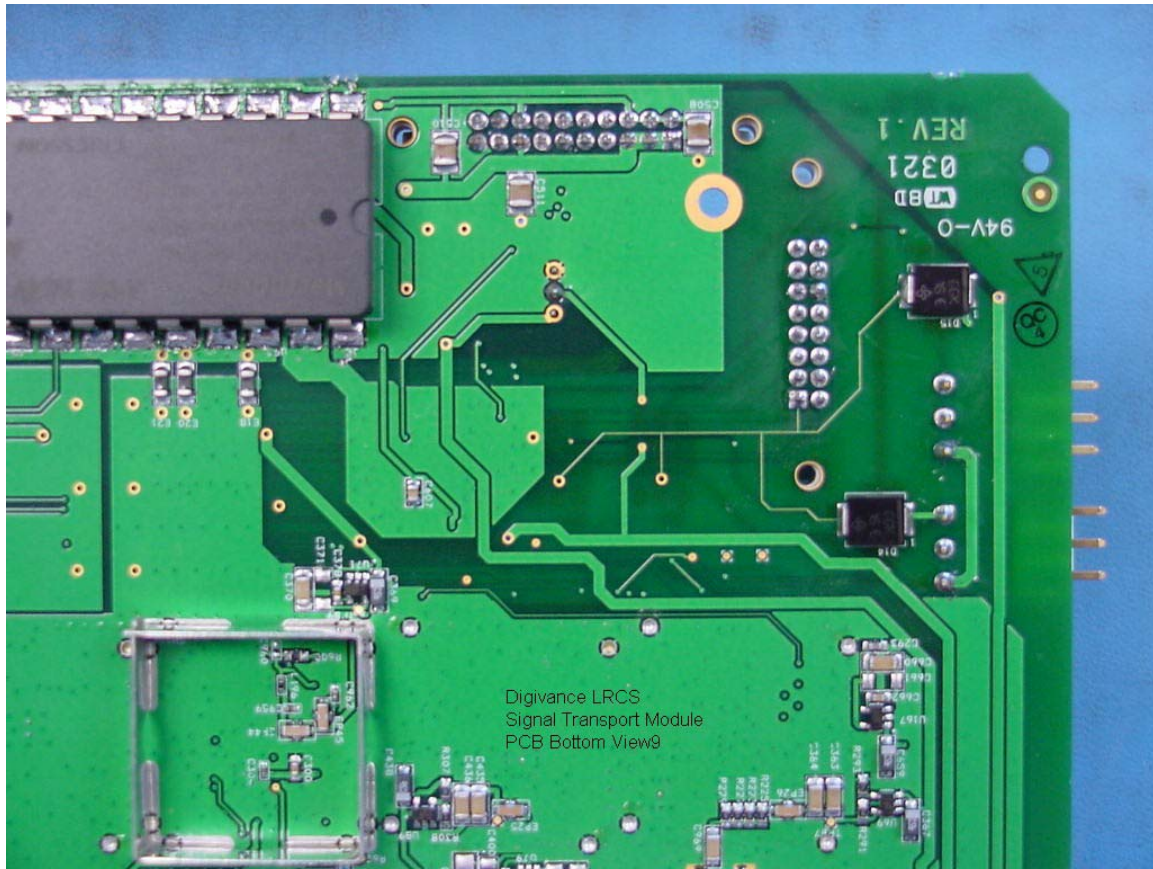
Figure 10 Digivance LRCS STM PCB Bottom View 9
