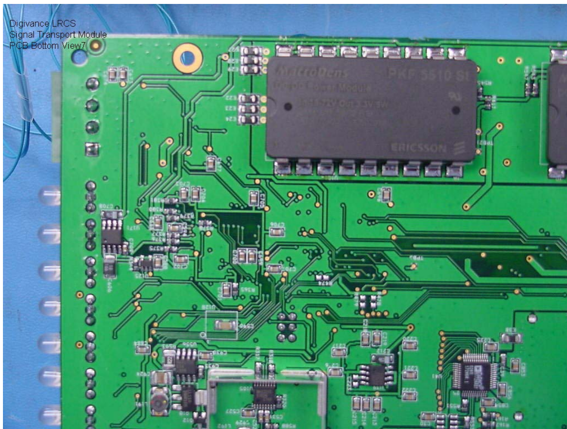
Figure 8 Digivance LRCS STM PCB Bottom View 7
