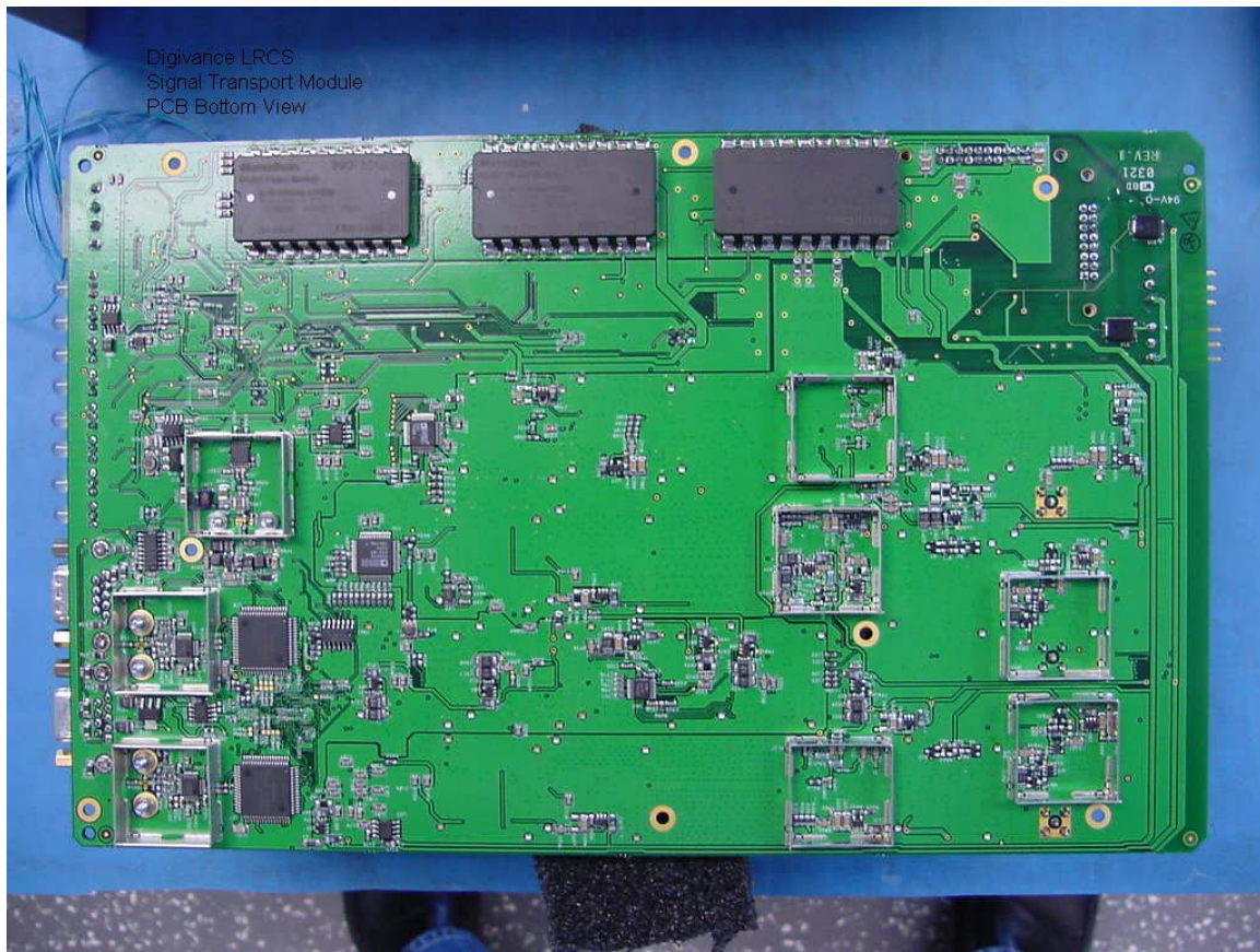
Figure 2 Digivance LRCS STM PCB Bottom View
