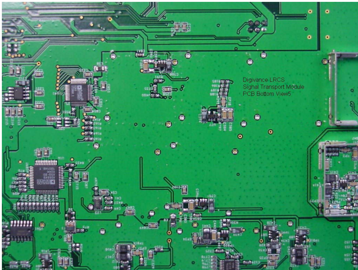
Figure 6 Digivance LRCS STM PCB Bottom View 5
