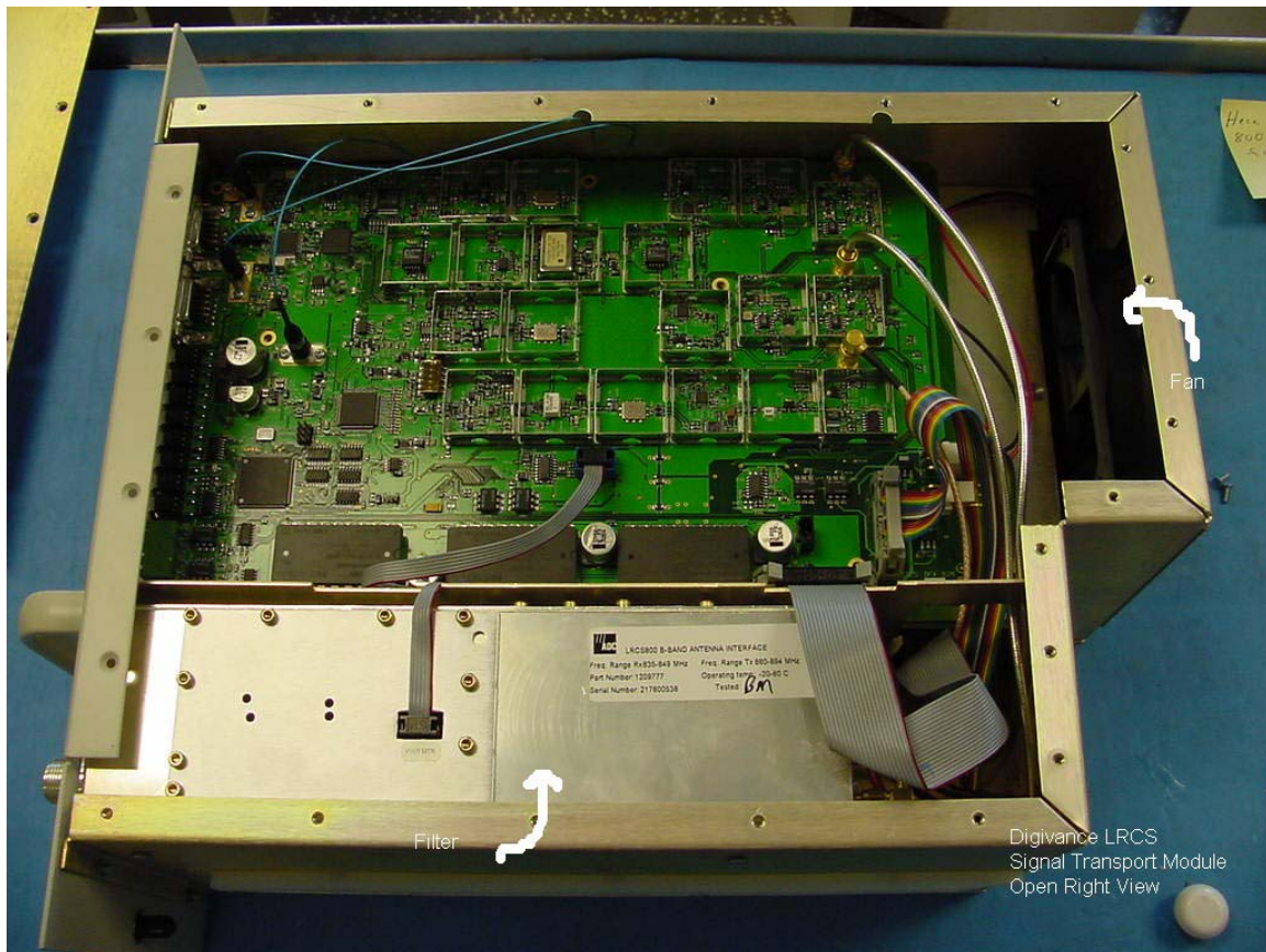
Figure 1 Digivance LRCS STM Open Right View
