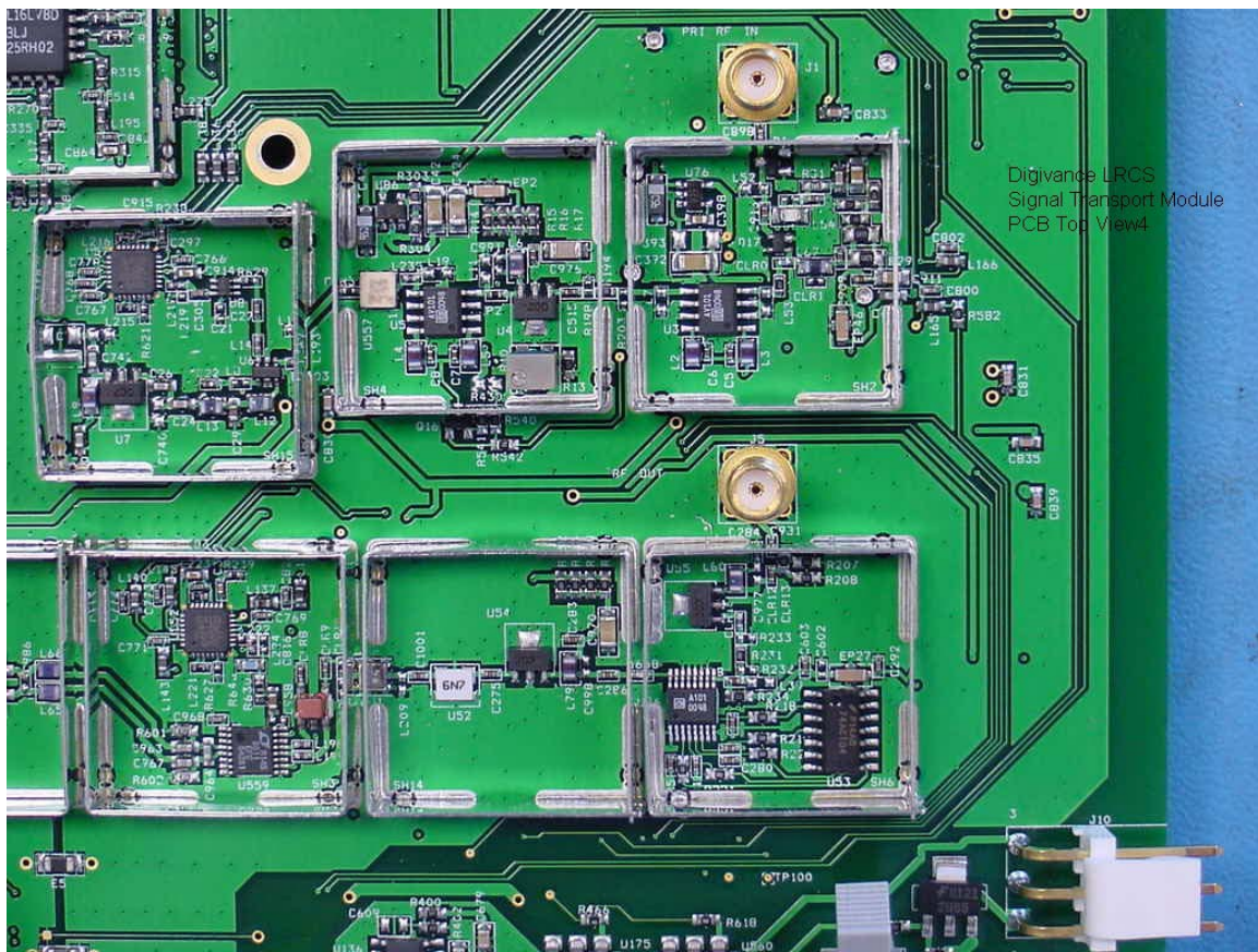
Figure 15 Digivance LRCS STM PCB Top View 4
