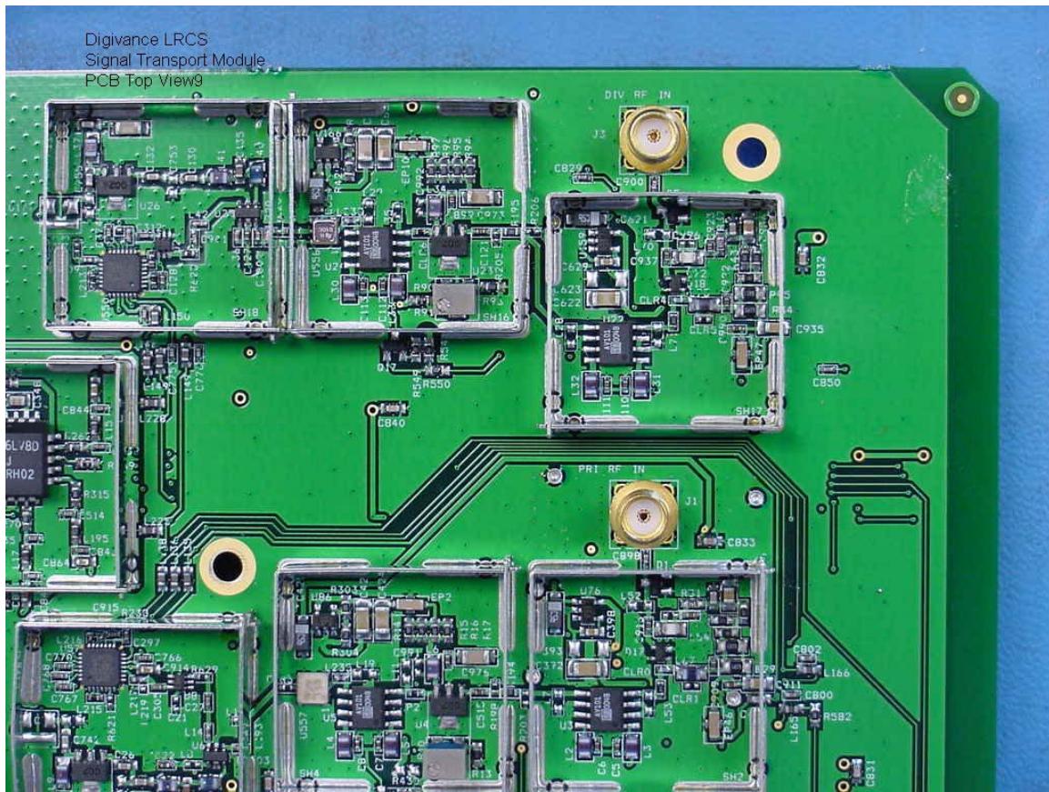
Figure 20 Digivance LRCS STM PCB Top View 9
