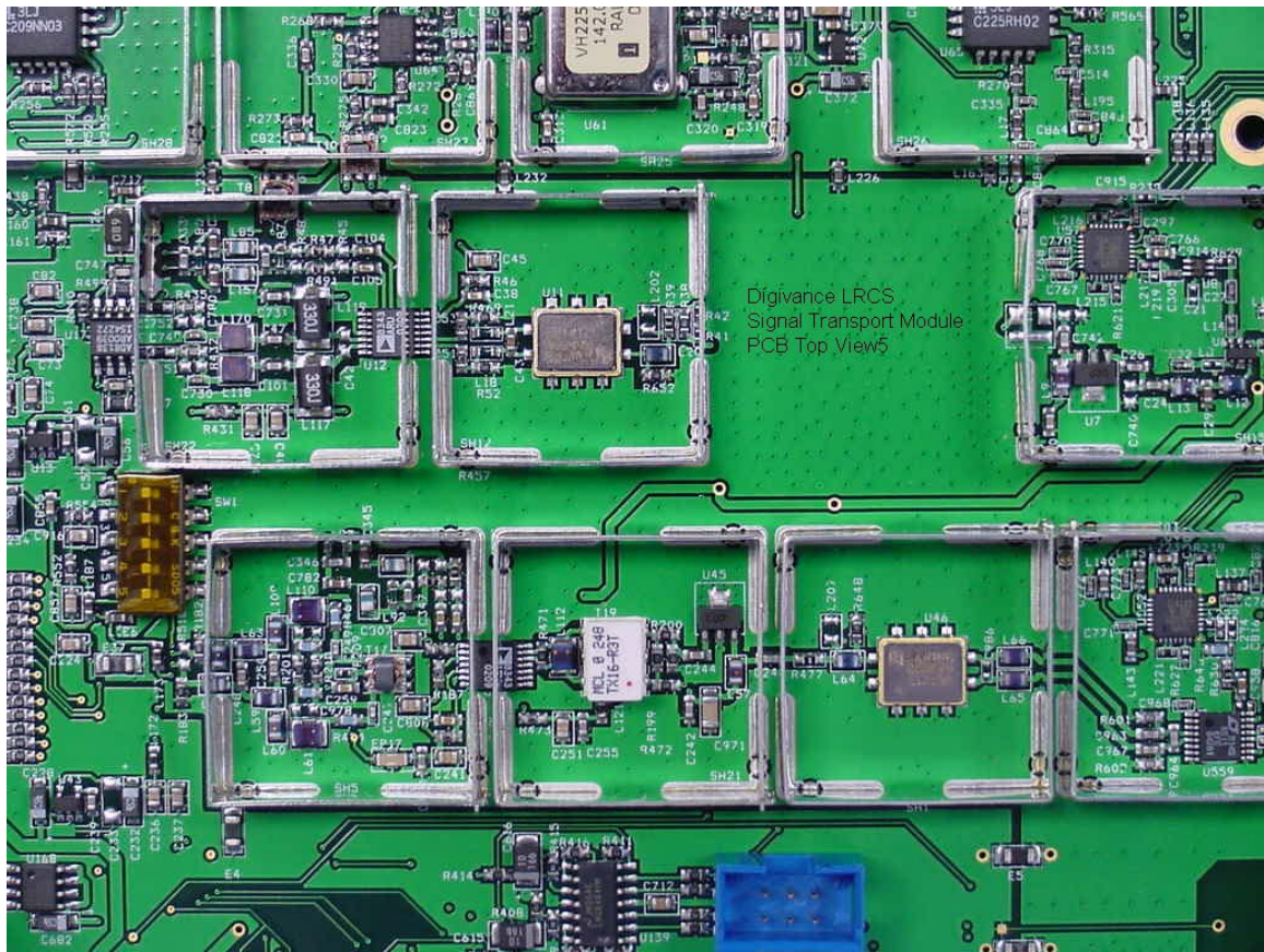
Figure 16 Digivance LRCS STM PCB Top View 5
