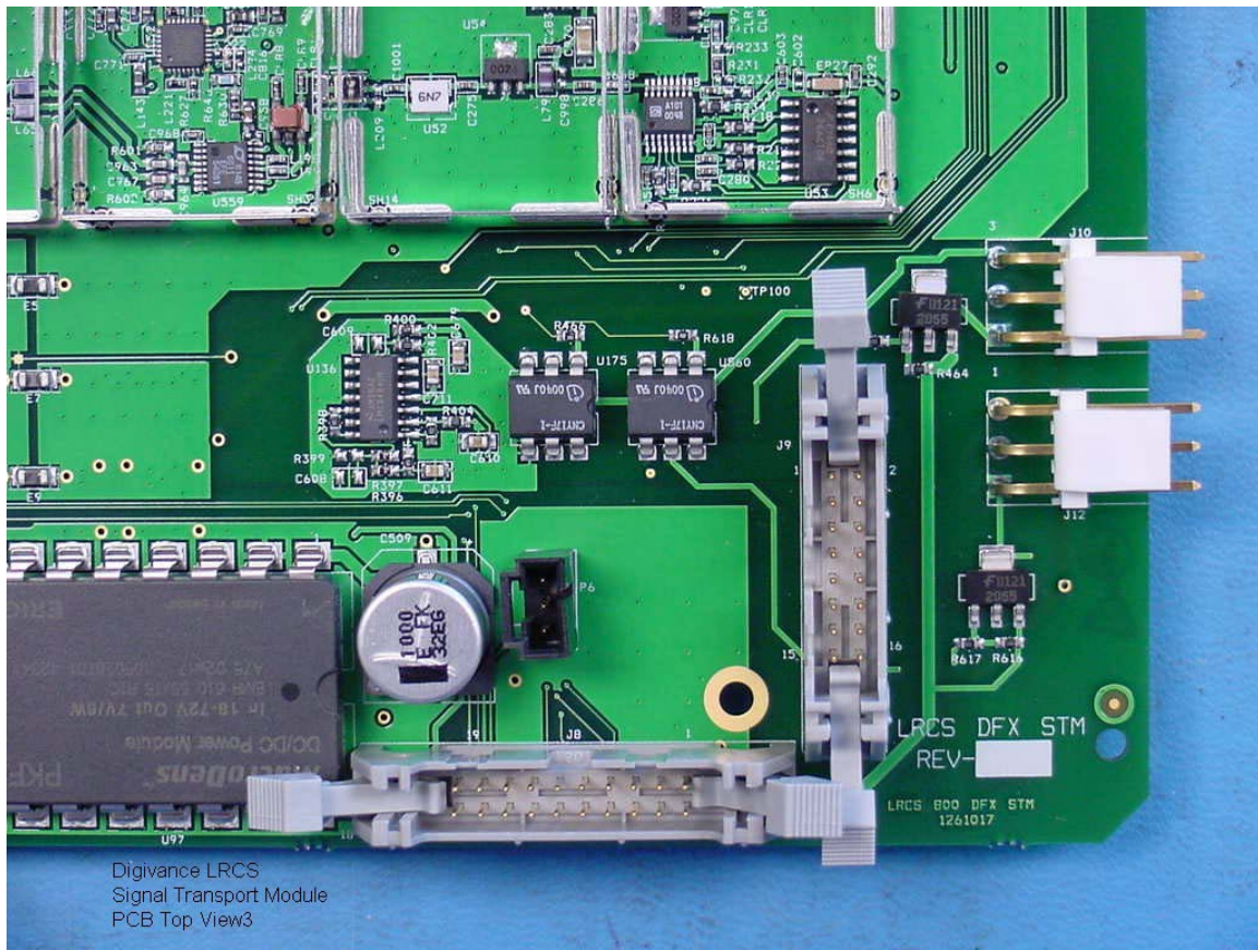
Figure 14 Digivance LRCS STM PCB Top View 3
