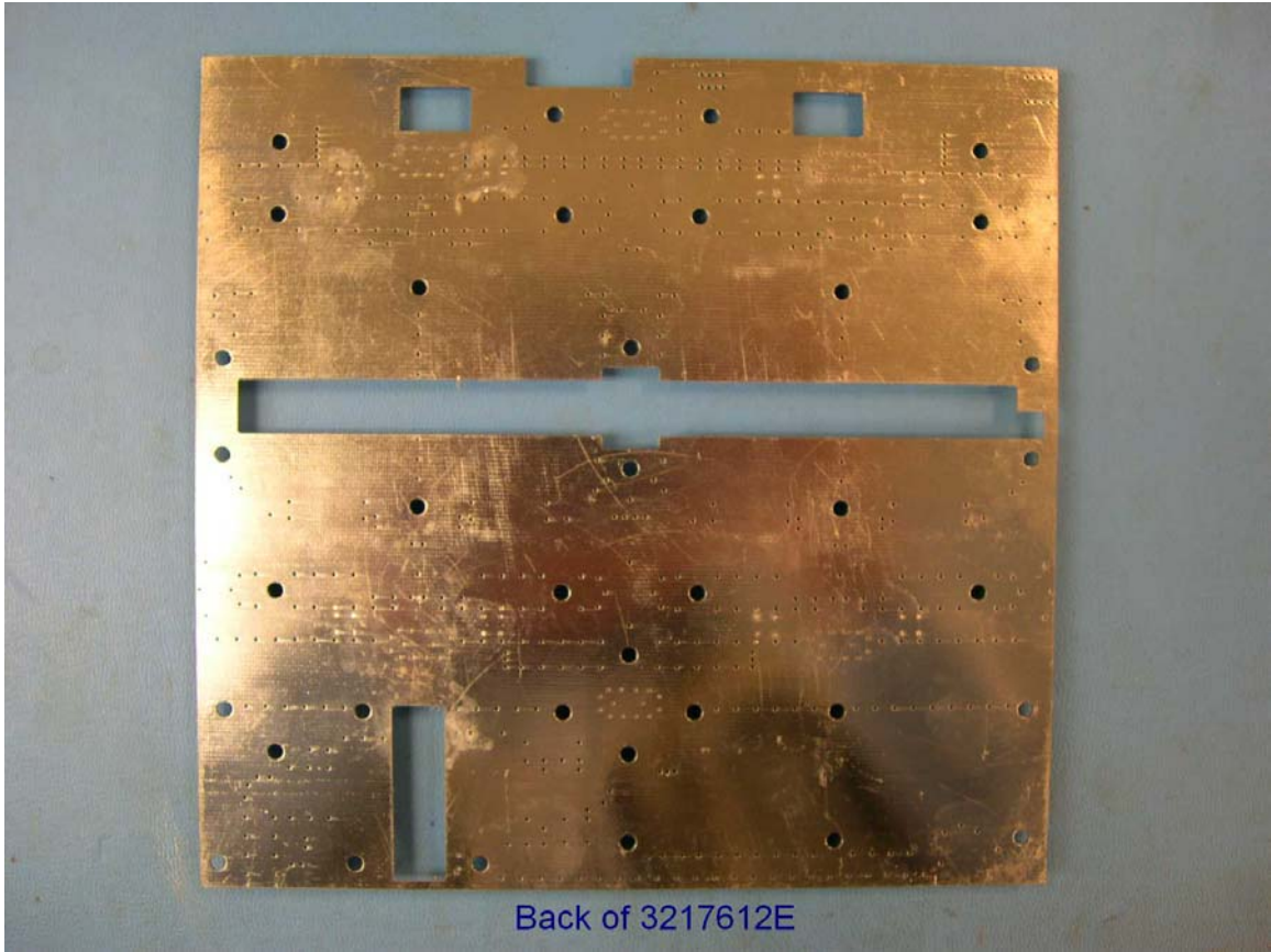
Figure 18 Main Amp Board Bottom View
