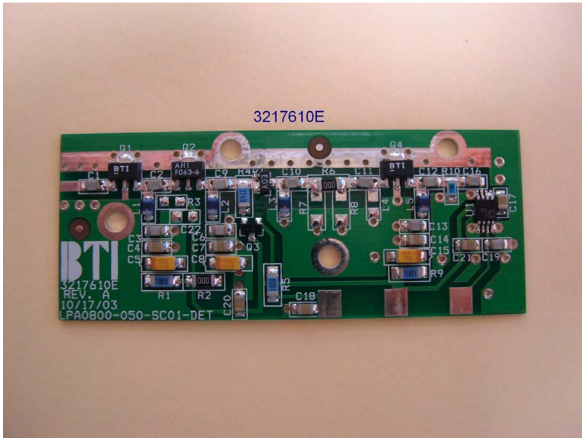
Figure 15 Detector Board Top View
