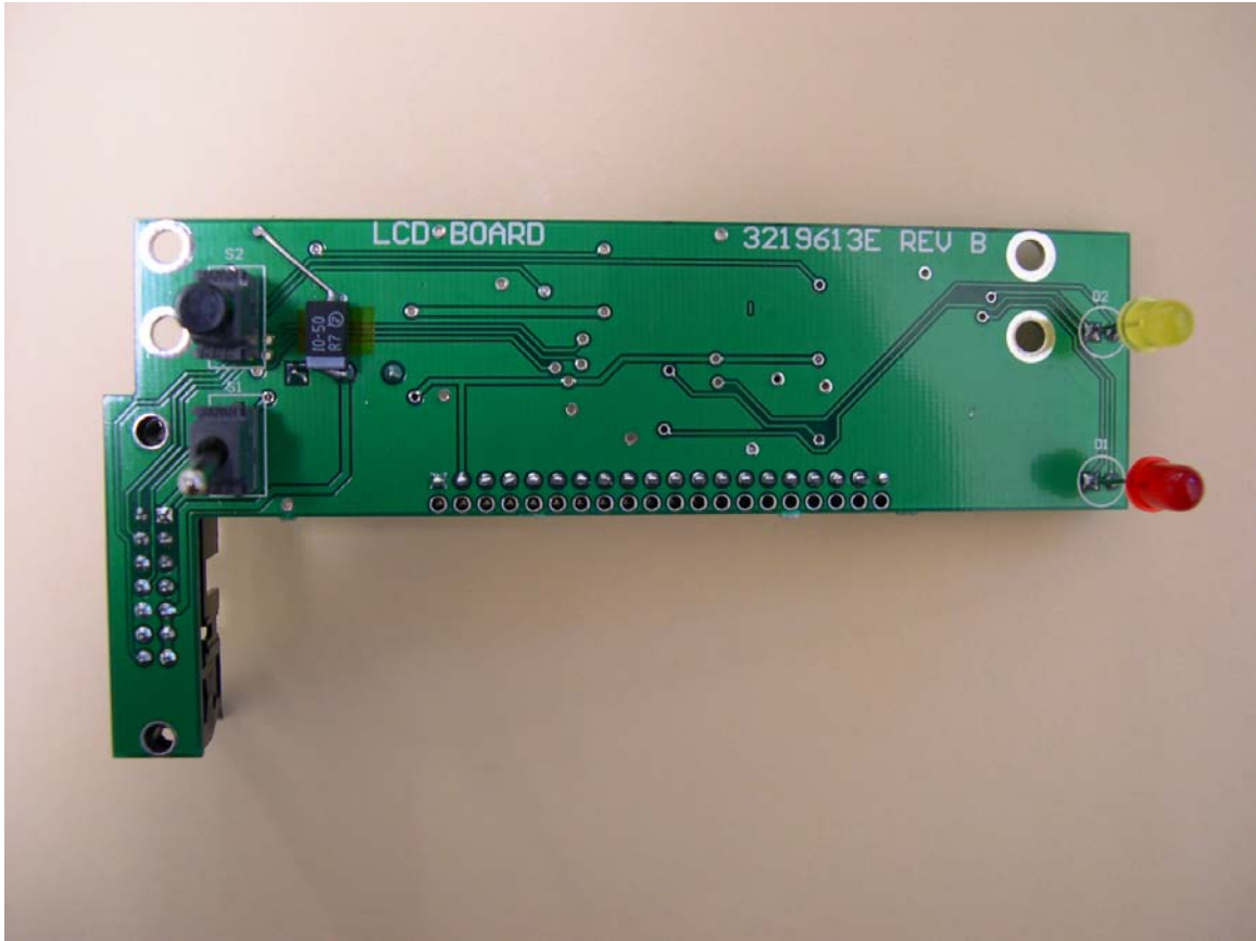
Figure 23 LCD Board Top View
