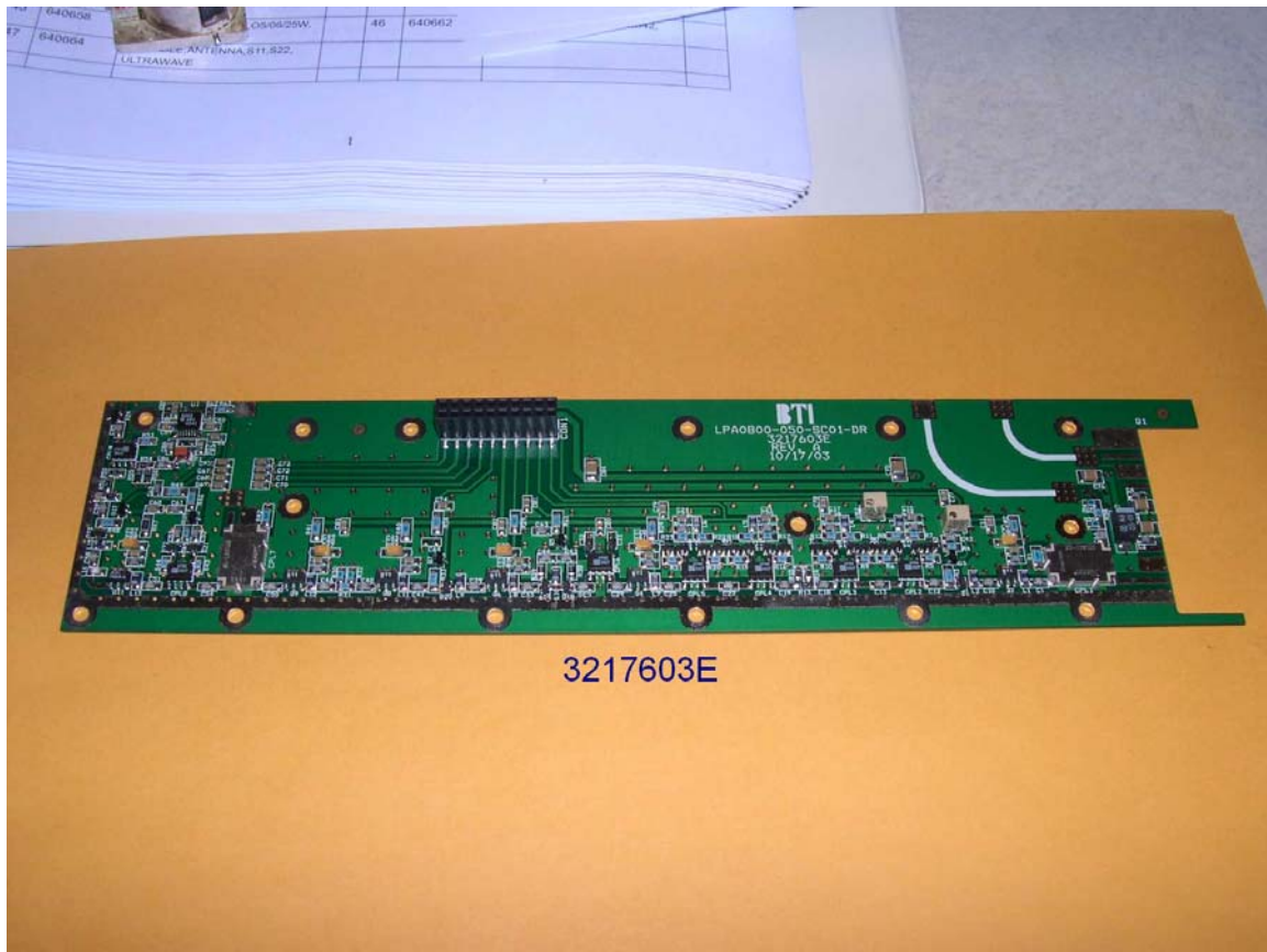
Figure 1 Driver Board Top View
