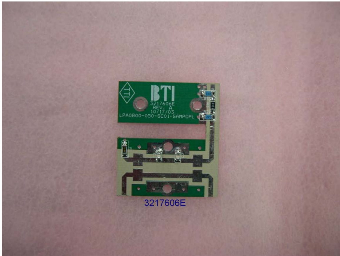
Figure 7 Sample Coupler Board Top View
