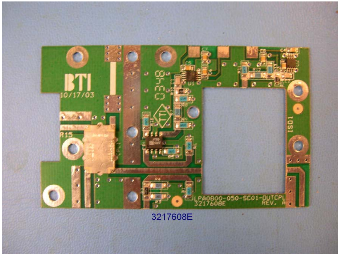
Figure 11 Output Coupler Board Top View
