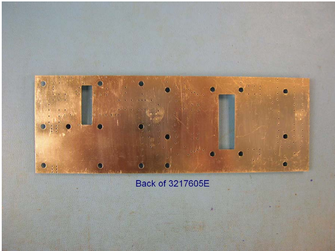
Figure 6 Error Amplifier Board Bottom View
