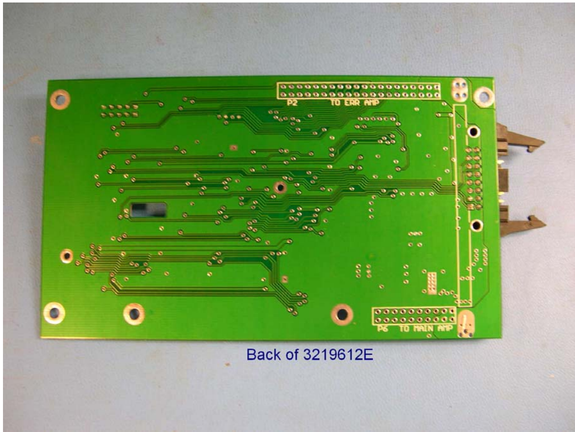
Figure 22 Main Mother Board Bottom View
