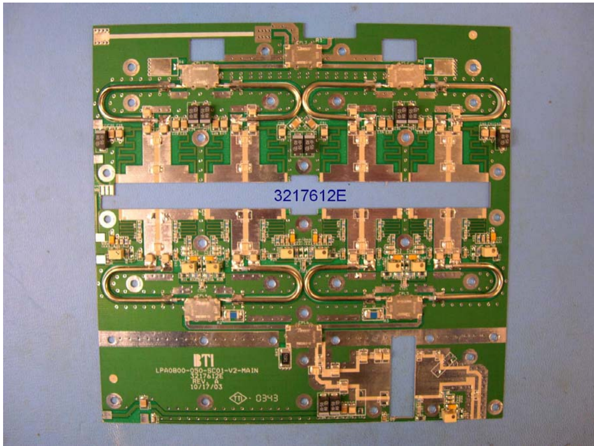
Figure 17 Main Amp Board Top View
