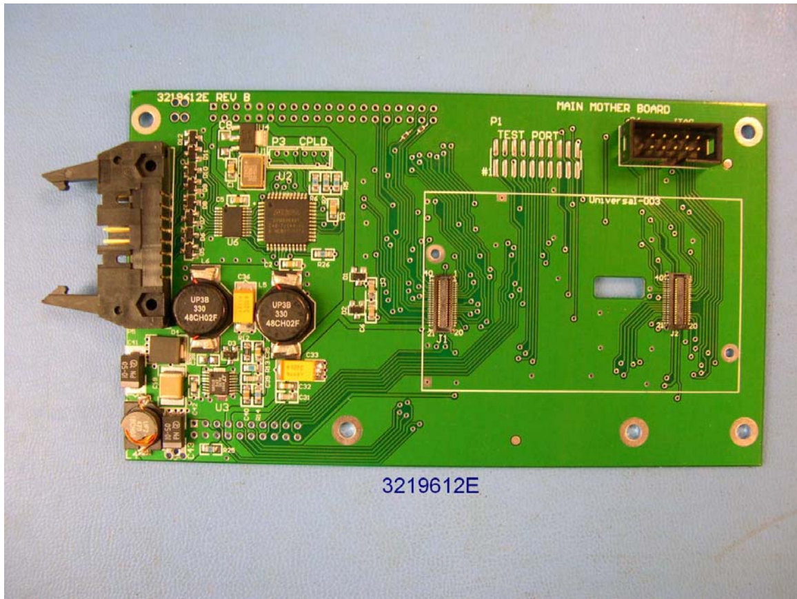
Figure 21 Main Mother Board Top View
