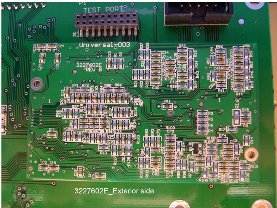
Figure 27 Control Board Top View
