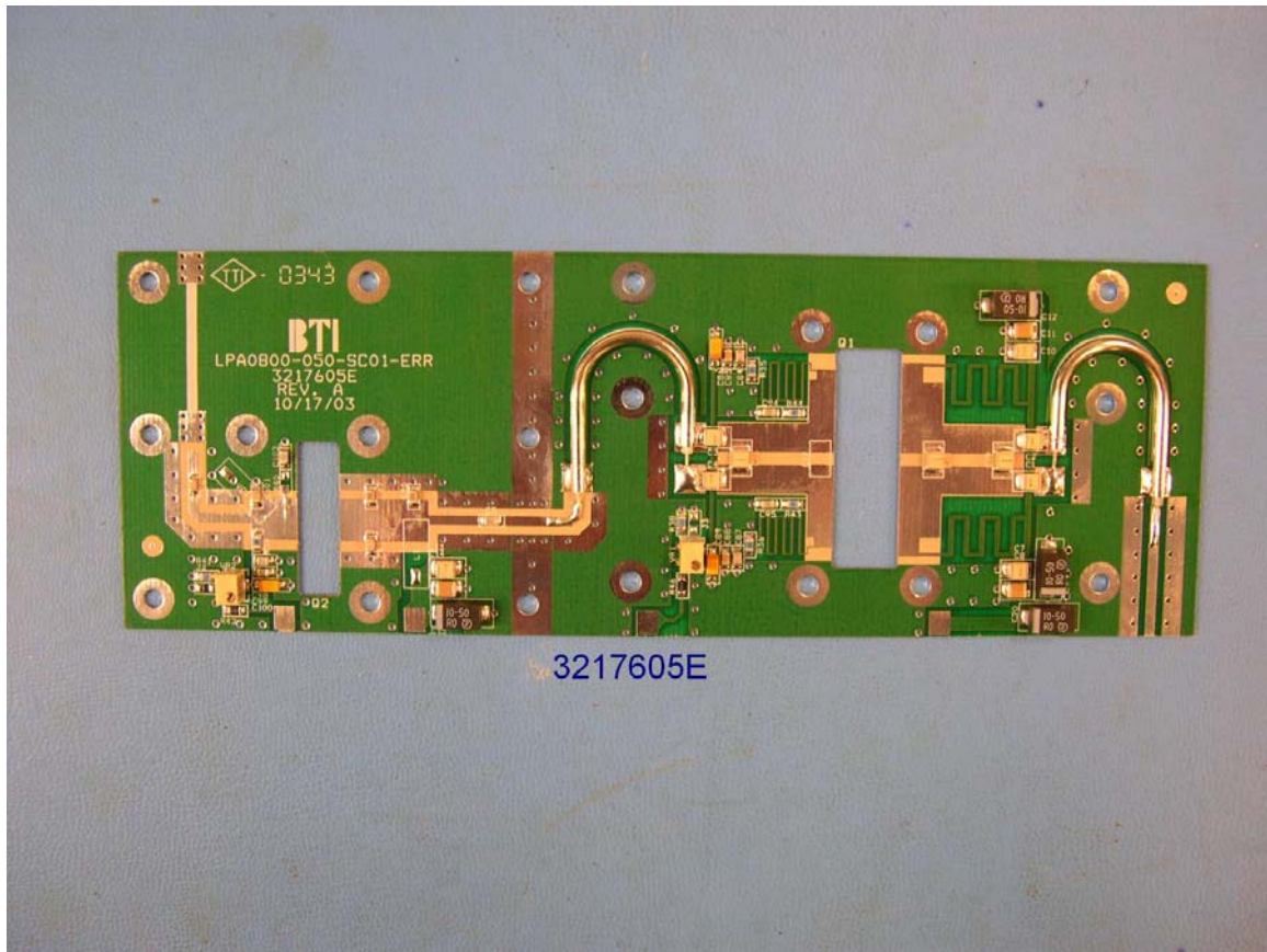
Figure 5 Error Amplifier Board Top View
