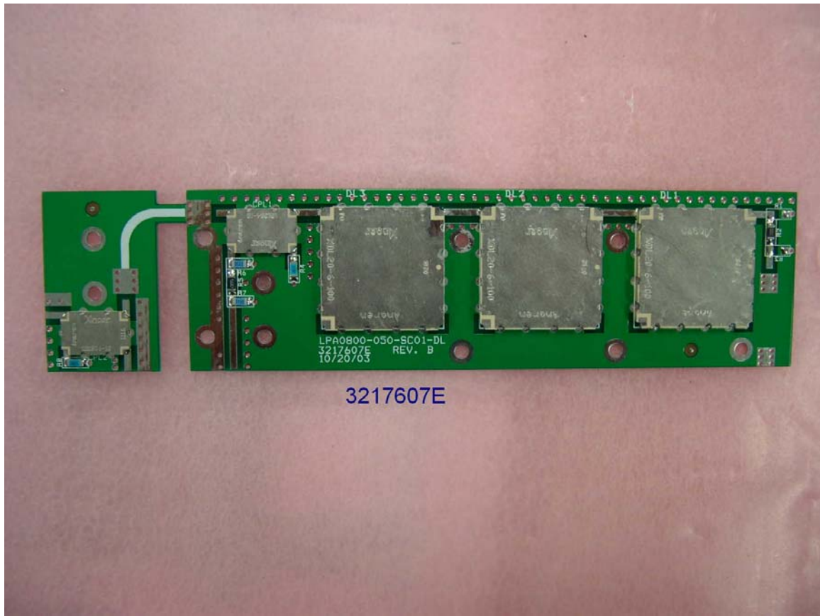
Figure 9 Delay Board Top View
