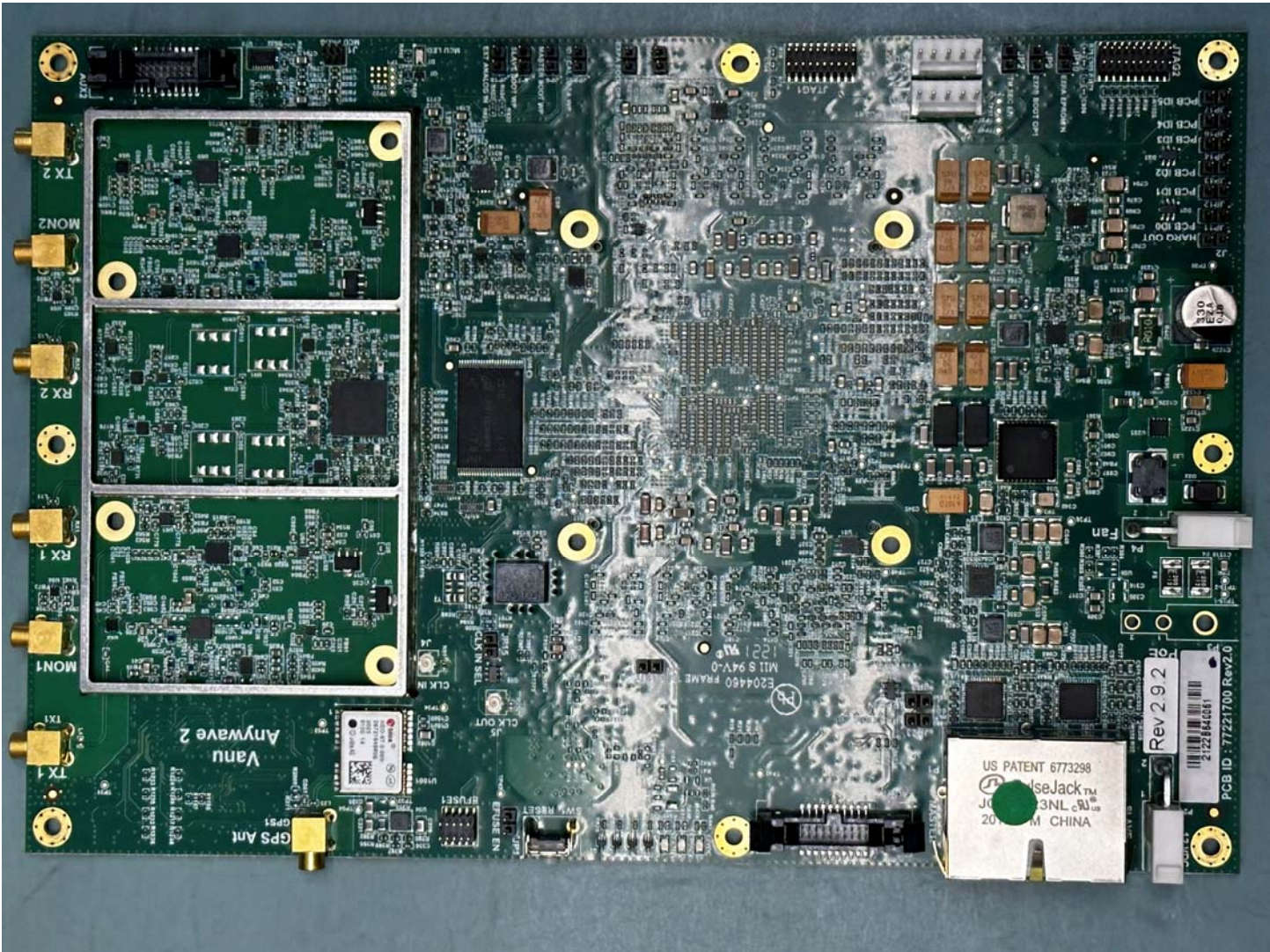
TOP WITH SHIELD CAN REMOVED
