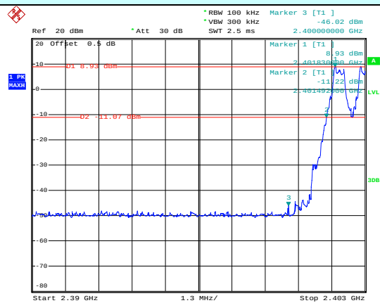
Hopping mode
