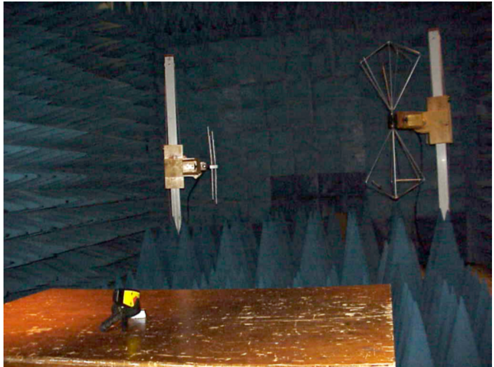
View of Radiated Emissions Prescan test setup 30MHz – 1 GHz
