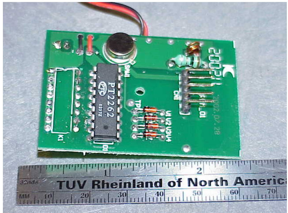
Close Up Top View of Transmitter Circuit Board
