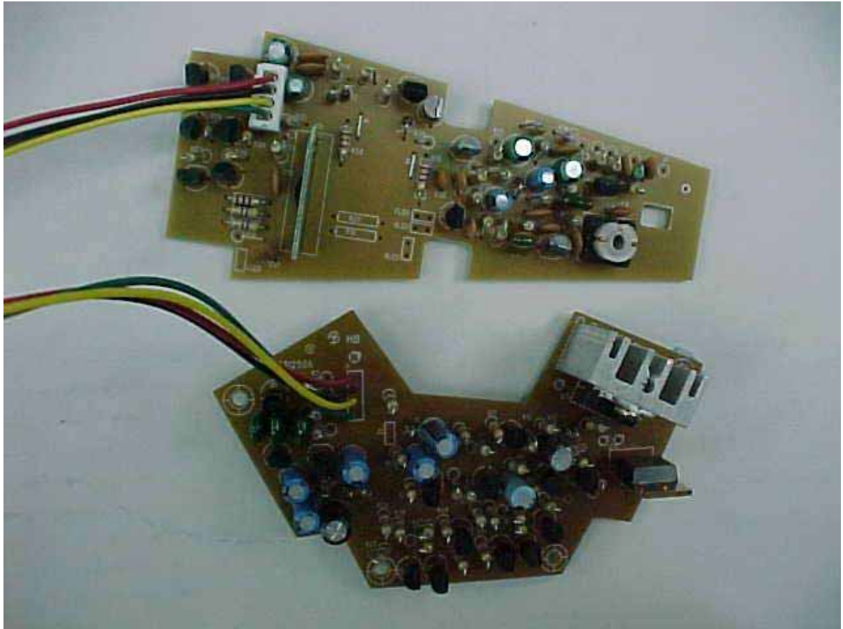
RCB231449_PCB6 (640x480x16M jpeg)
