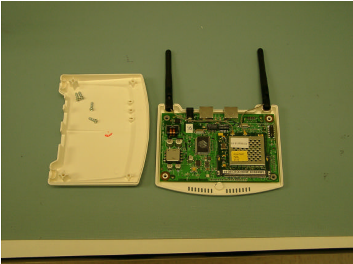
Main circuit board plus MINI PCI radio card
