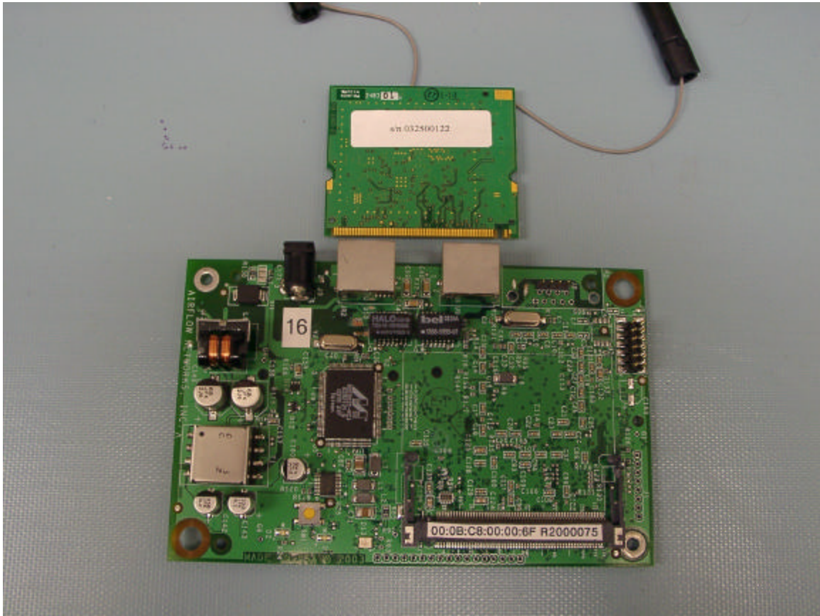
Top Side of the main circuit board and bottom side of the Mini PCI card removed
