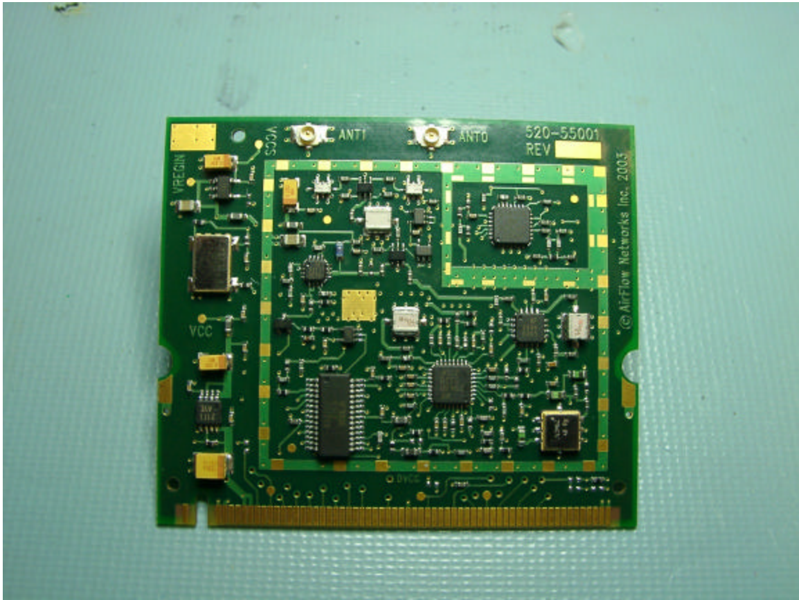
Top Side (component side of the main circuit board)
