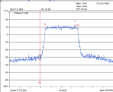
802.11ac(VHT80)_Chain0 / CH155
