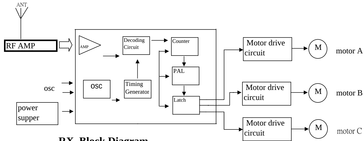
RX Block Diagram
