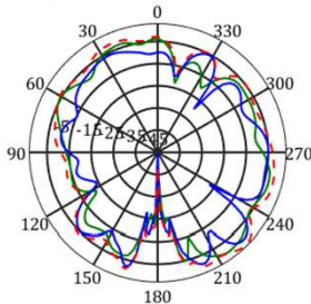
frequency=5470MHz, Y-Z Plane
