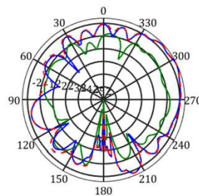
frequency=6525MHz, X-Z Plane
