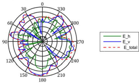
frequency=5470MHz, X-Y Plane
