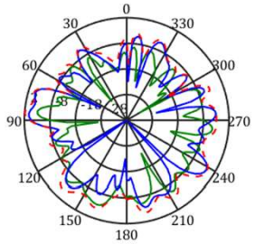
frequency=5850MHz, X-Y Plane
