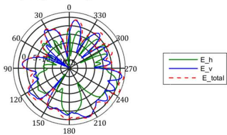
frequency=5850MHz, X-Y Plane
