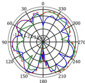
frequency=5850MHz, Y-Z Plane
