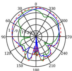
frequency=2450MHz, X-Z Plane
