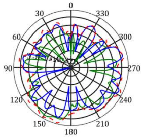
frequency=5470MHz, X-Y Plane
