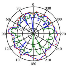
frequency=5150MHz, X-Y Plane
