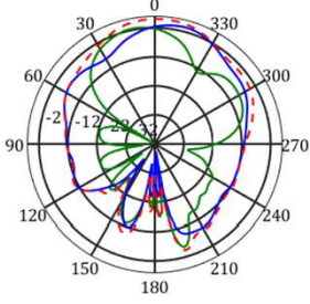
frequency=2500MHz, X-Z Plane
