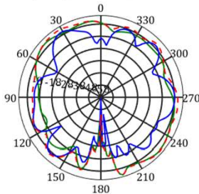
frequency=5150MHz, Y-Z Plane
