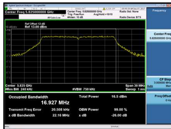
Channel 165 (5825MHz)
