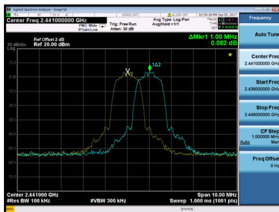
Channel 39 (2441MHz)
