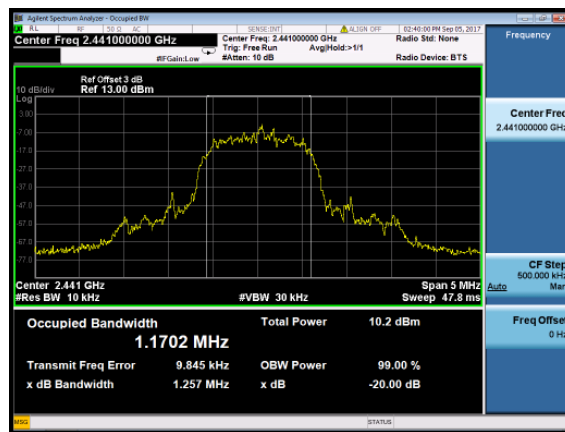
Channel 39 (2441MHz)
