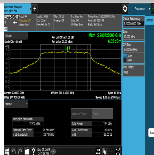
11AC20SISO-Ant1-5200
