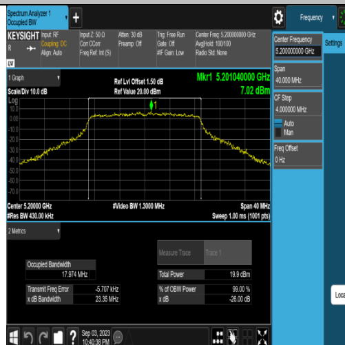
11N20SISO-Ant1-5200
