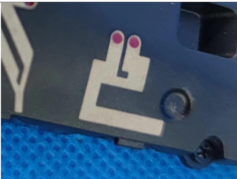
EUT Photo(12) - Antenna 6
