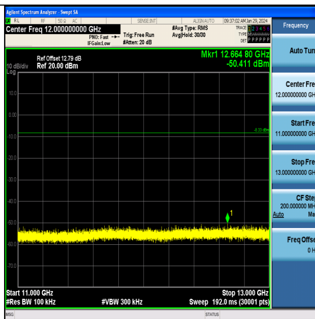
BLE_2M-Ant1-2402-11000~13000-PASS
