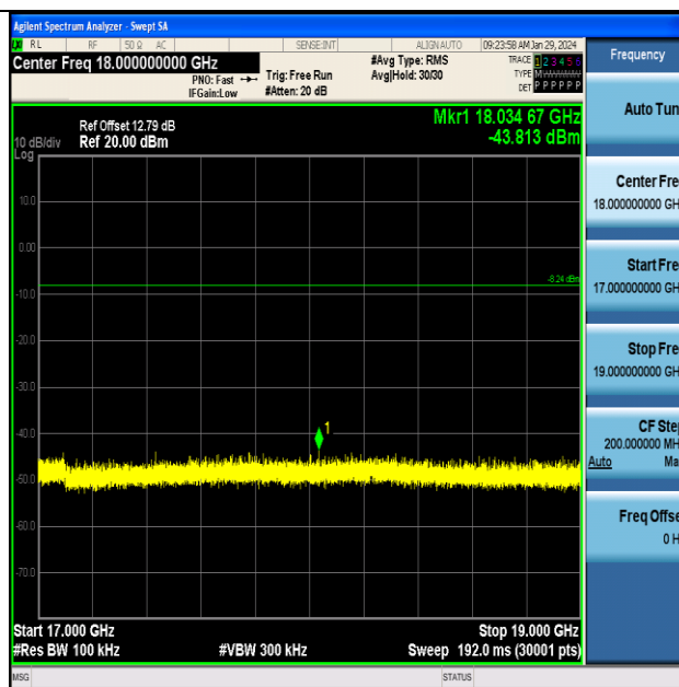
BLE_1M-Ant1-2402-17000~19000-PASS
