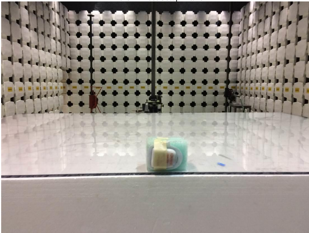
1-18 GHz Test Setup Y-axis
