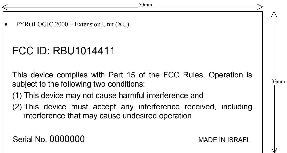
Figure 1. FCC Label
