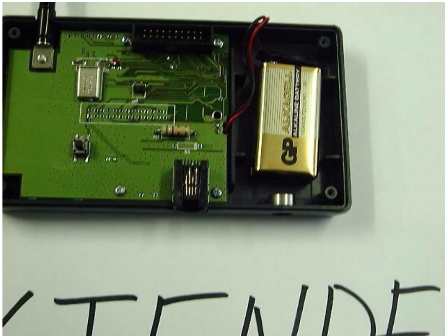
Figure 4 PCB (Side 1) in Unit
